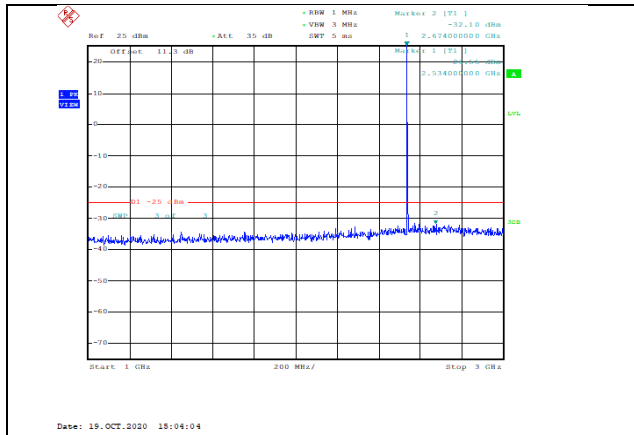
Band7-5MHz-16QAM-21100-1RB#0-Range2:1000~3000MHz--32.1-PASS
