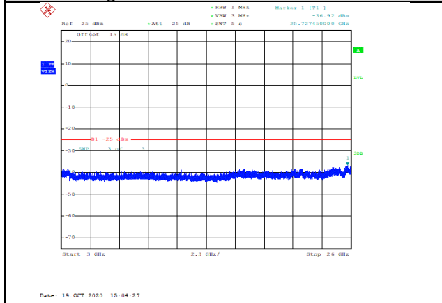
Band7-5MHz-16QAM-21100-1RB#0-Range3:3000~26000MHz--36.92-PASS
