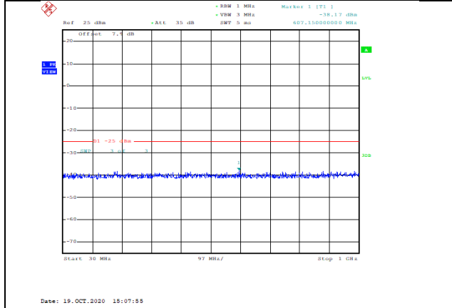
Band7-10MHz-QPSK-21100-1RB#0-Range1:30~1000MHz--38.17-PASS
