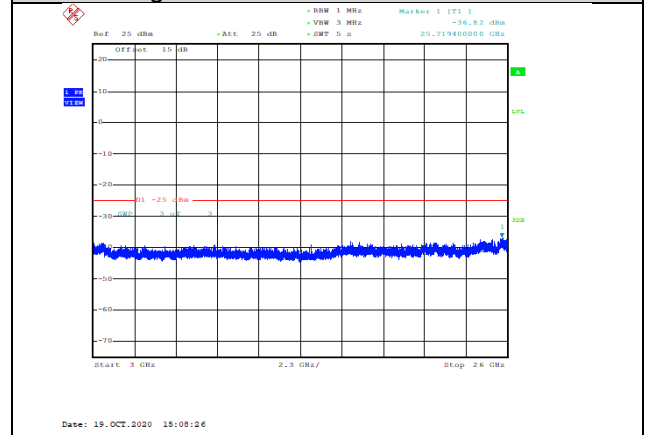
Band7-10MHz-QPSK-21100-1RB#0-Range3:3000~26000MHz--36.82-PASS
