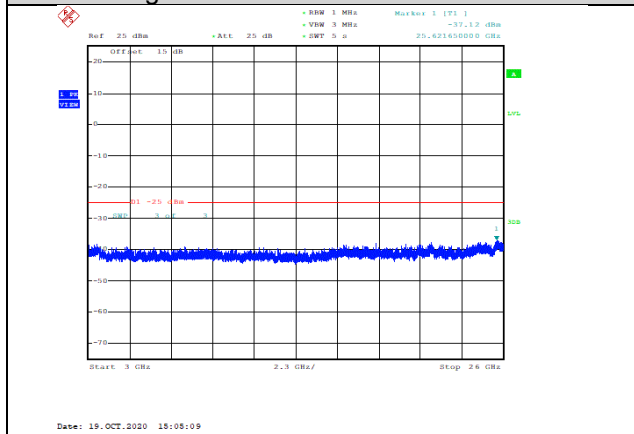
Band7-5MHz-QPSK-21425-1RB#0-Range3:3000~26000MHz--37.12-PASS
