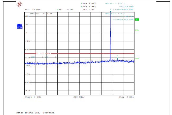
Band7-5MHz-16QAM-21425-1RB#0-Range2:1000~3000MHz--31.23-PASS
