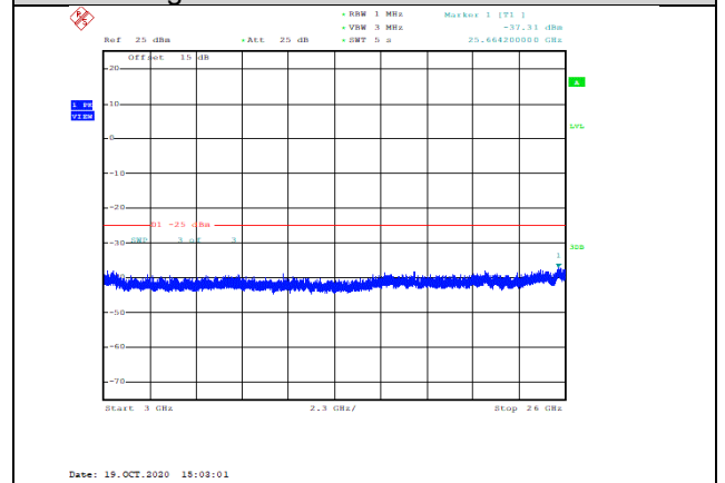
Band7-5MHz-16QAM-20775-1RB#0-Range3:3000~26000MHz--37.31-PASS
