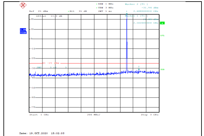
Band7-5MHz-16QAM-20775-1RB#0-Range2:1000~3000MHz--31.94-PASS
