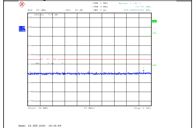
Band7-5MHz-16QAM-21100-1RB#0-Range1:30~1000MHz--37.95-PASS
