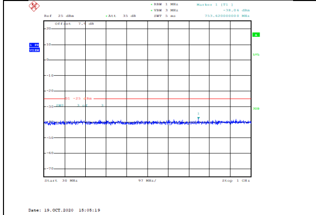
Band7-5MHz-16QAM-21425-1RB#0-Range1:30~1000MHz--38.06-PASS
