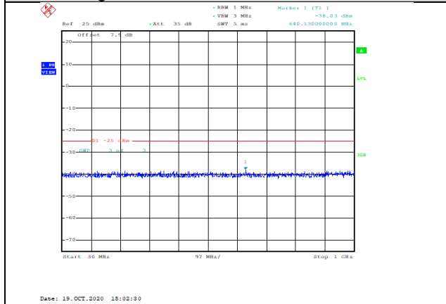
Band7-5MHz-16QAM-20775-1RB#0-Range1:30~1000MHz--38.03-PASS
