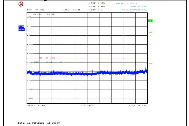
Band7-5MHz-16QAM-21425-1RB#0-Range3:3000~26000MHz--36.84-PASS
