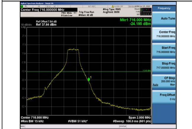
Band12-1.4MHz-QPSK-23173-1RB#5
