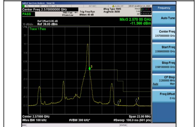
Band7-5MHz-16QAM-21425-1RB#24
