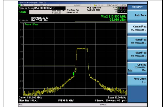
Band26-1.4MHz-16QAM-26697-6RB#0
