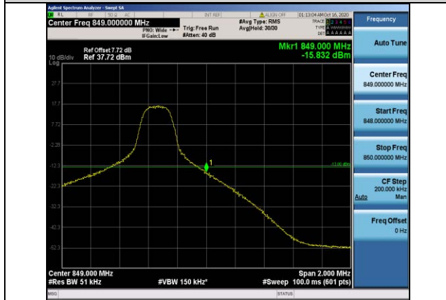
Band5-5MHz-16QAM-20625-1RB#24
