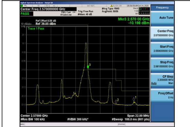
Band7-5MHz-QPSK-21425-1RB#24
