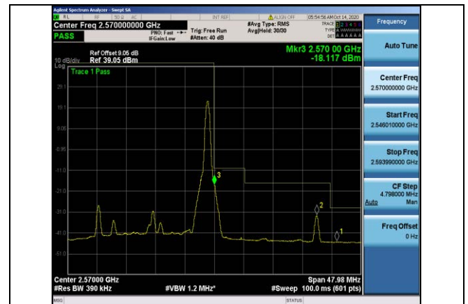
Band7-20MHz-QPSK-21350-1RB#99
