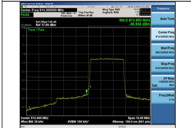
Band26-3MHz-QPSK-26705-15RB#0
