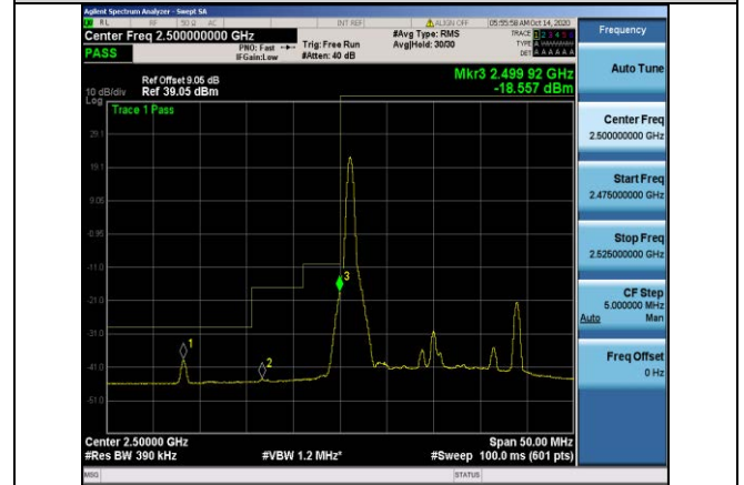
Band7-20MHz-QPSK-20850-1RB#0
