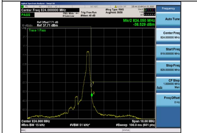
Band26-1.4MHz-QPSK-26783-1RB#5
