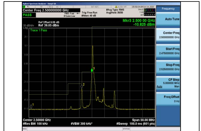
Band7-5MHz-16QAM-20775-1RB#0
