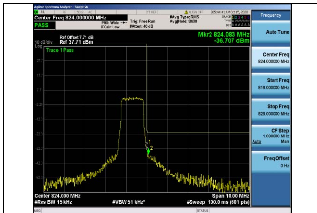
Band26-1.4MHz-16QAM-26783-6RB#0
