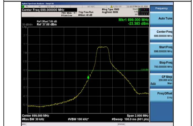
Band12-3MHz-16QAM-23025-1RB#0
