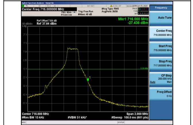
Band12-1.4MHz-16QAM-23173-1RB#5
