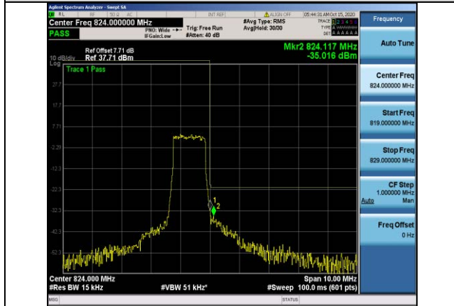
Band26-1.4MHz-QPSK-26783-6RB#0
