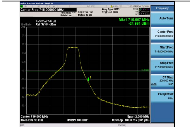
Band12-3MHz-16QAM-23165-1RB#14
