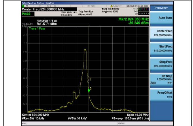
Band26-1.4MHz-16QAM-26783-1RB#5
