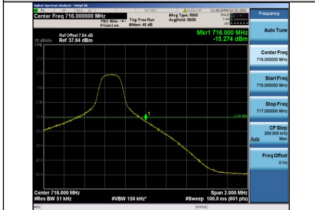
Band17-5MHz-16QAM-23825-1RB#24
