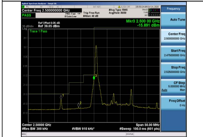
Band7-15MHz-16QAM-20825-1RB#0
