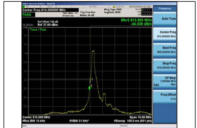
Band26-1.4MHz-16QAM-26697-1RB#0
