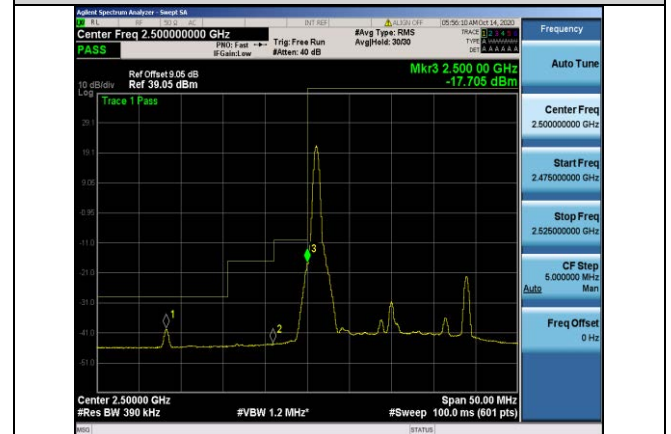
Band7-20MHz-16QAM-20850-1RB#0
