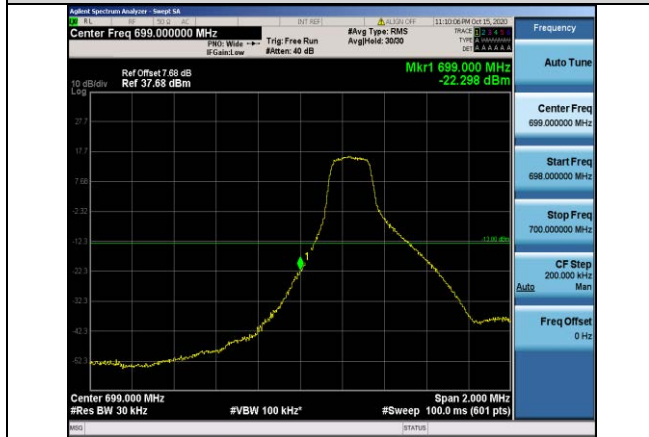
Band12-3MHz-QPSK-23025-1RB#0
