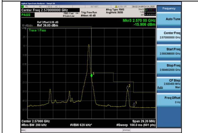
Band7-10MHz-16QAM-21400-1RB#49
