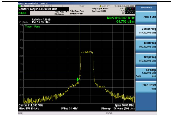
Band26-1.4MHz-QPSK-26697-6RB#0
