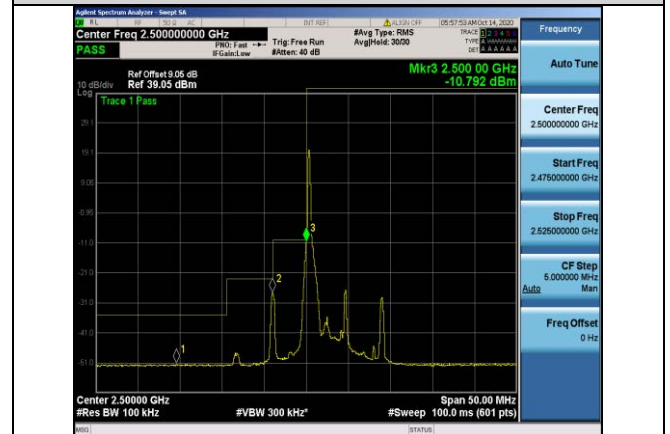
Band7-5MHz-QPSK-20775-1RB#0
