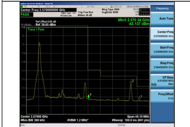
Band7-20MHz-16QAM-21350-1RB#0
