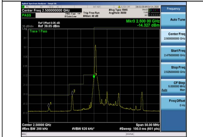
Band7-10MHz-QPSK-20800-1RB#0
