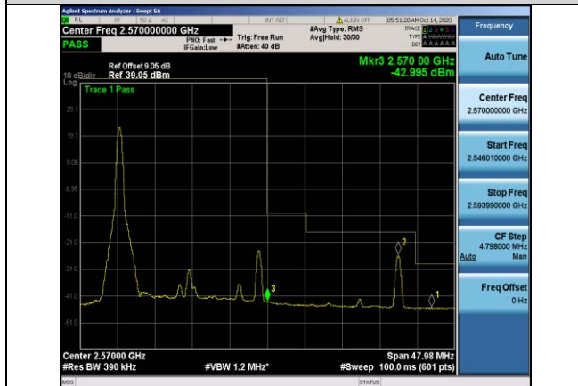
Band7-20MHz-QPSK-21350-1RB#0
