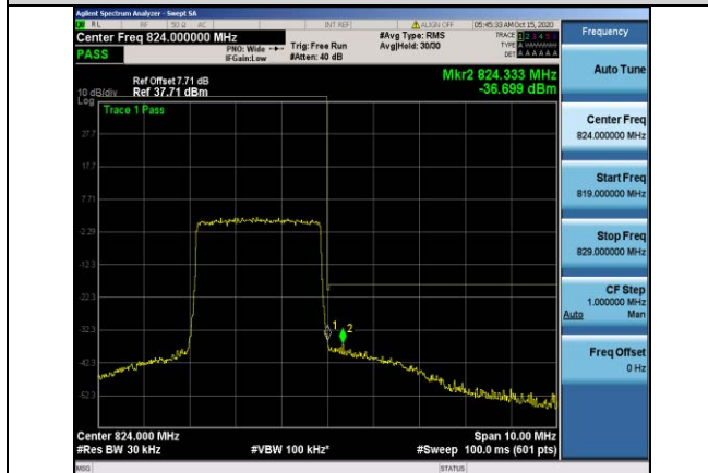
Band26-3MHz-16QAM-26775-15RB#0
