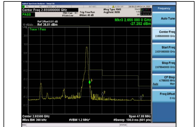
Band41-20MHz-16QAM-41140-1RB#99
