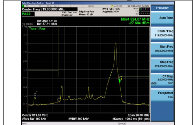
Band26-10MHz-16QAM-26740_Right-1RB#49
