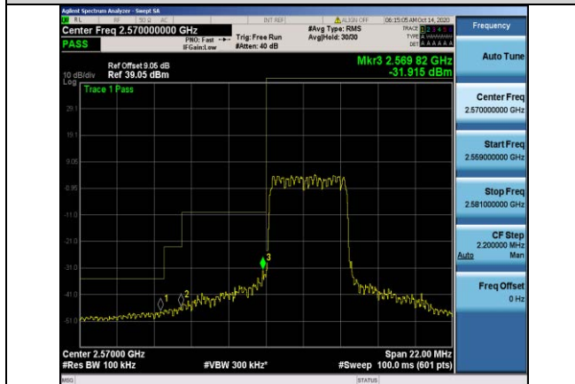
Band38-5MHz-QPSK-37775-25RB#0
