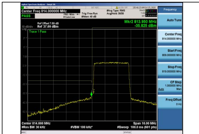
Band26-3MHz-16QAM-26705-15RB#0
