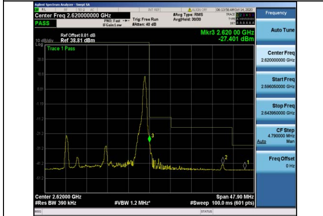
Band38-20MHz-16QAM-38150-100RB#0
