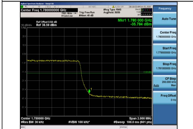
Band66-3MHz-16QAM-132657-15RB#0
