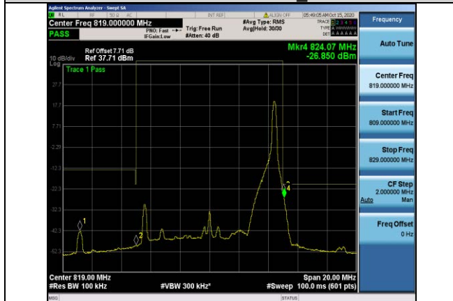
Band26-10MHz-QPSK-26740_Right-1RB#49
