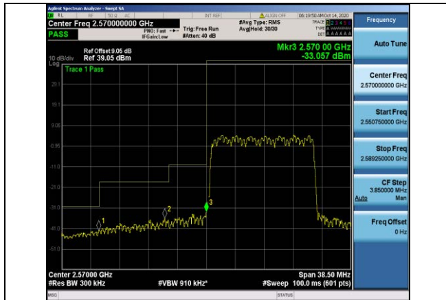
Band38-15MHz-QPSK-37825-75RB#0
