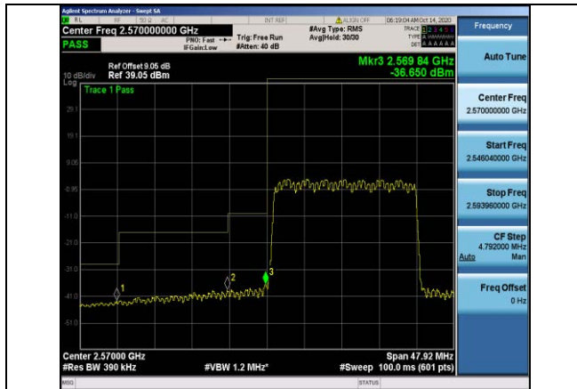
Band38-20MHz-16QAM-37850-100RB#0
