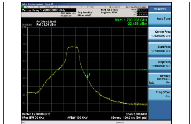
Band66-3MHz-QPSK-132657-1RB#14
