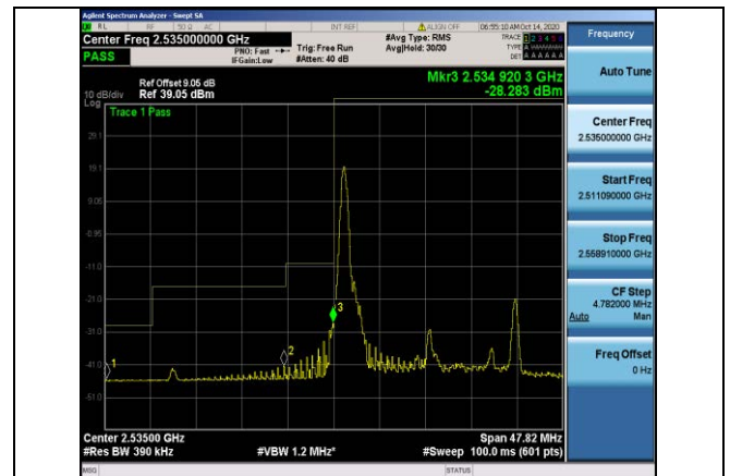
Band41-20MHz-QPSK-40140-1RB#0
