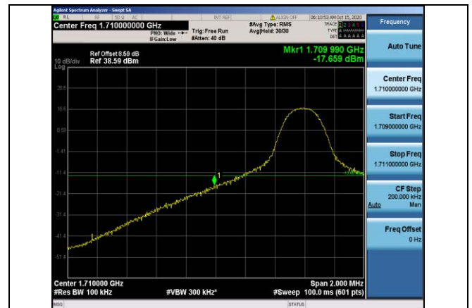
Band66-10MHz-16QAM-132022-1RB#0
