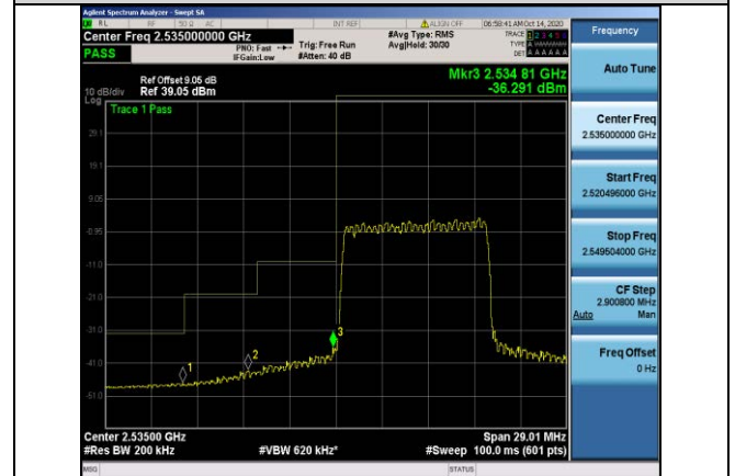
Band41-10MHz-16QAM-40090-50RB#0
