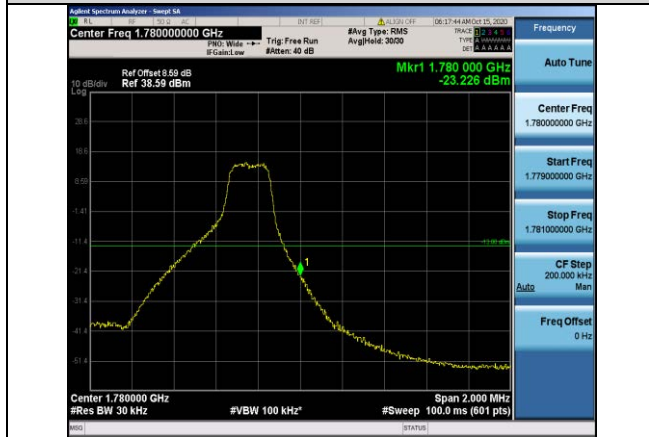
Band66-3MHz-16QAM-132657-1RB#14
