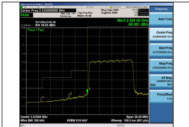
Band41-15MHz-16QAM-40115-75RB#0
