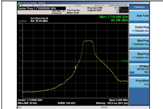
Band66-3MHz-QPSK-131987-1RB#0
