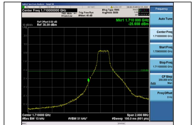
Band66-1.4MHz-16QAM-131979-1RB#0
