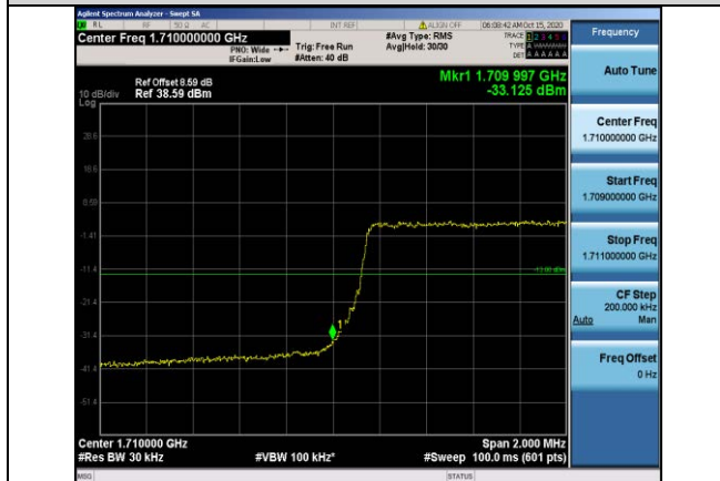
Band66-3MHz-QPSK-131987-15RB#0
