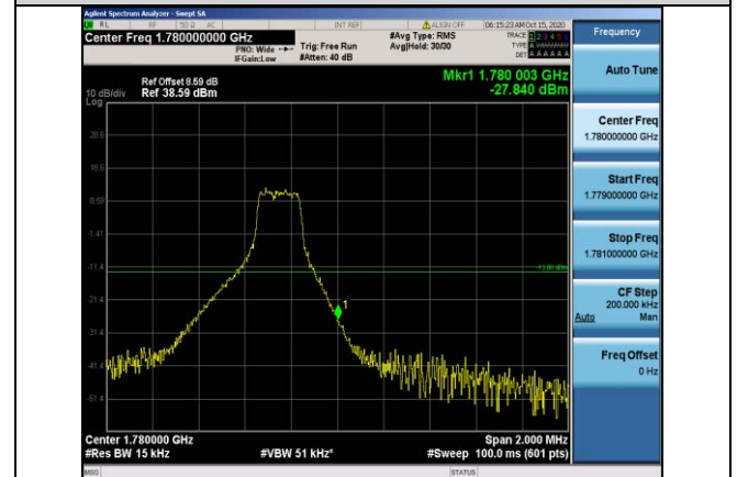
Band66-1.4MHz-16QAM-132665-1RB#5
