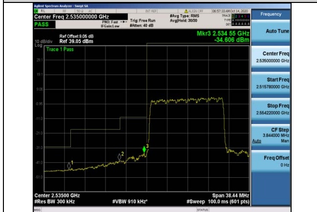
Band41-15MHz-QPSK-40115-75RB#0
