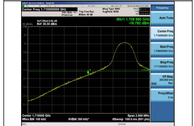
Band66-10MHz-QPSK-132022-1RB#0
