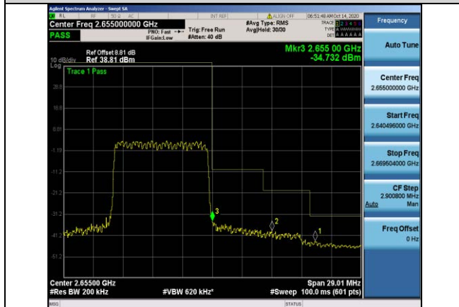
Band41-10MHz-QPSK-41190-50RB#0
