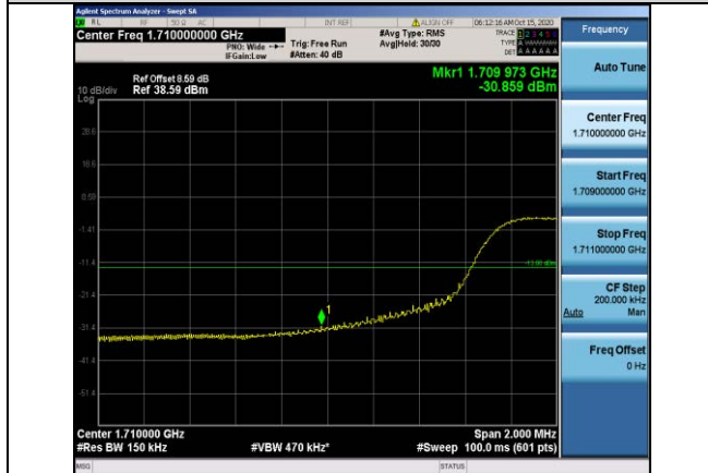
Band66-15MHz-QPSK-132047-75RB#0
