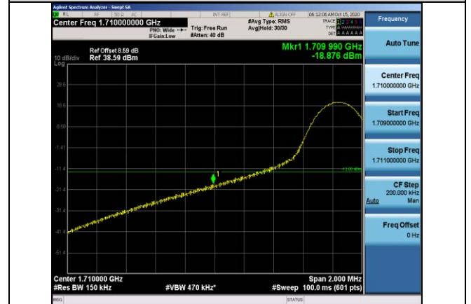
Band66-15MHz-16QAM-132047-1RB#0
