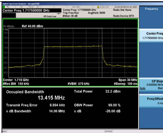
Band4-15MHz-16QAM-20025-75RB#0-13.415
