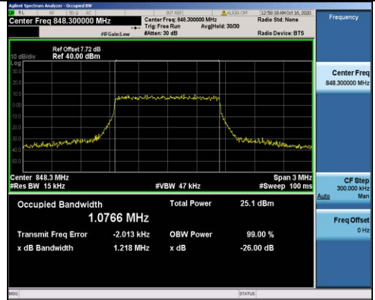
Band5-1.4MHz-QPSK-20643-6RB#0-1.0766
