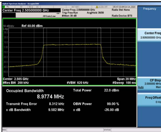
Band7-10MHz-16QAM-20800-50RB#0-8.9774
