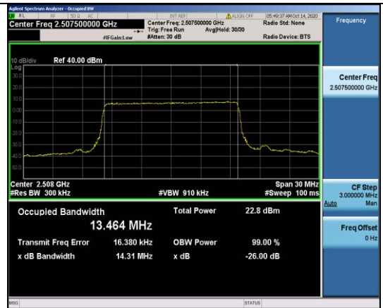
Band7-15MHz-QPSK-20825-75RB#0-13.464
