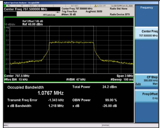
Band12-1.4MHz-QPSK-23095-6RB#0-1.0767
