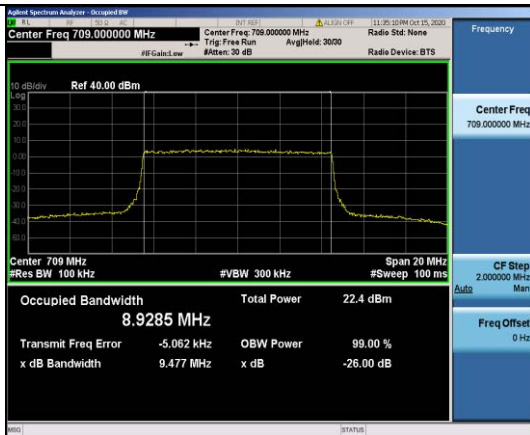
Band17-10MHz-16QAM-23780-50RB#0-8.9285
