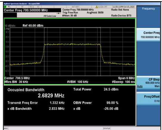
Band12-3MHz-QPSK-23025-15RB#0-2.6829
