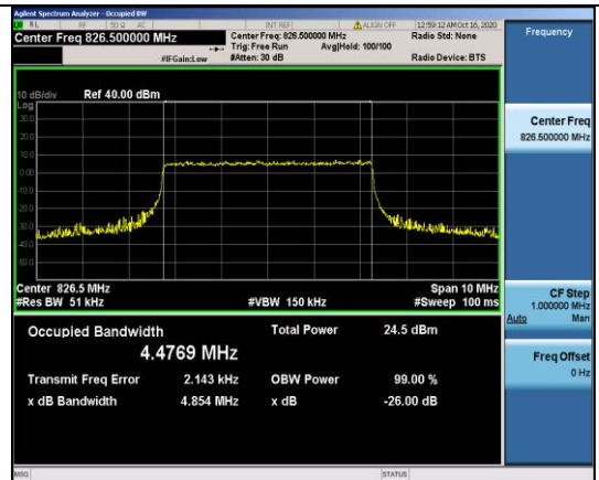
Band5-5MHz-QPSK-20425-25RB#0-4.4769
