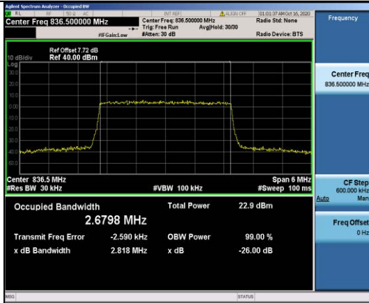
Band5-3MHz-16QAM-20525-15RB#0-2.6798
