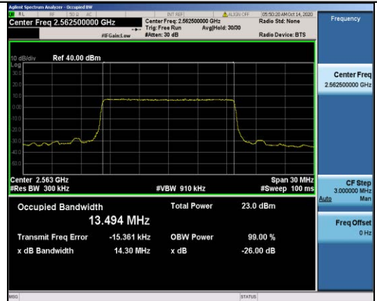
Band7-15MHz-QPSK-21375-75RB#0-13.494
