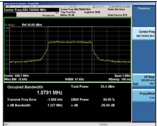
Band12-1.4MHz-QPSK-23017-6RB#0-1.0791
