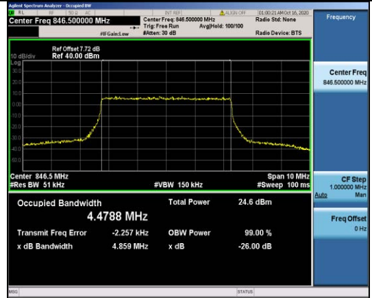
Band5-5MHz-QPSK-20625-25RB#0-4.4788
