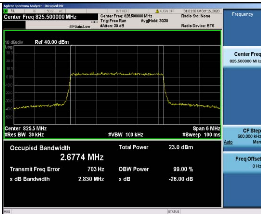
Band5-3MHz-16QAM-20415-15RB#0-2.6774
