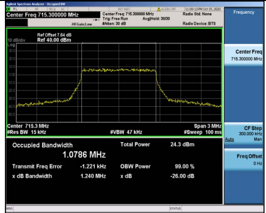
Band12-1.4MHz-QPSK-23173-6RB#0-1.0786
