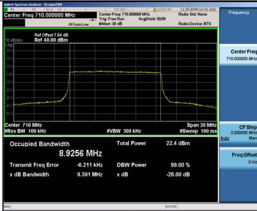
Band17-10MHz-16QAM-23790-50RB#0-8.9256
