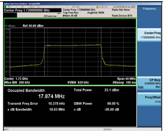
Band4-20MHz-QPSK-20050-100RB#0-17.874
