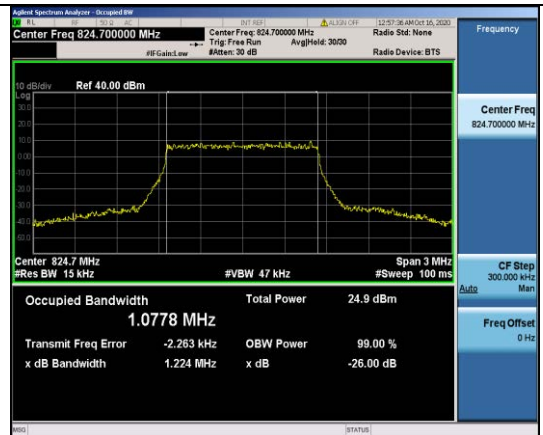
Band5-1.4MHz-QPSK-20407-6RB#0-1.0778
