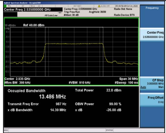
Band7-15MHz-QPSK-21100-75RB#0-13.486
