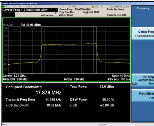
Band4-20MHz-16QAM-20050-100RB#0-17.879
