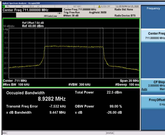
Band17-10MHz-16QAM-23800-50RB#0-8.9282
