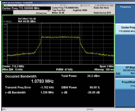
Band12-1.4MHz-16QAM-23173-6RB#0-1.0783
