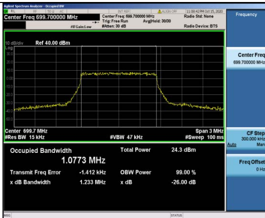
Band12-1.4MHz-16QAM-23017-6RB#0-1.0773
