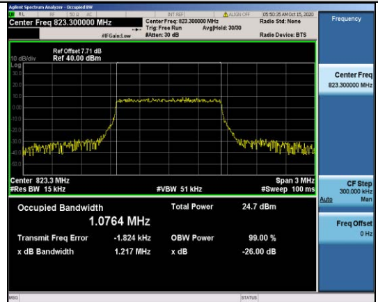
Band26-1.4MHz-QPSK-26783-6RB#0-1.0764
