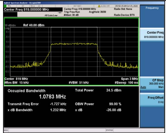
Band26-1.4MHz-QPSK-26740-6RB#0-1.0783
