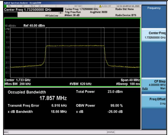
Band4-20MHz-QPSK-20175-100RB#0-17.857
