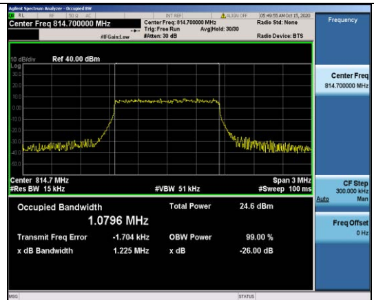
Band26-1.4MHz-QPSK-26697-6RB#0-1.0796
