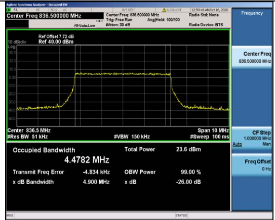
Band5-5MHz-QPSK-20525-25RB#0-4.4782
