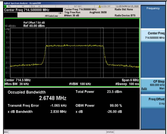
Band12-3MHz-QPSK-23165-15RB#0-2.6748
