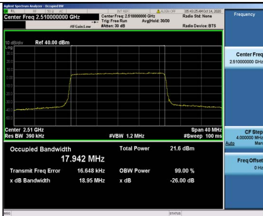
Band7-20MHz-16QAM-20850-100RB#0-17.942
