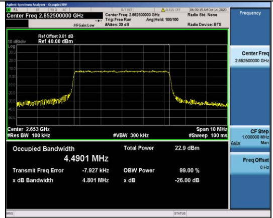
Band41-5MHz-16QAM-41215-25RB#0-4.4901
