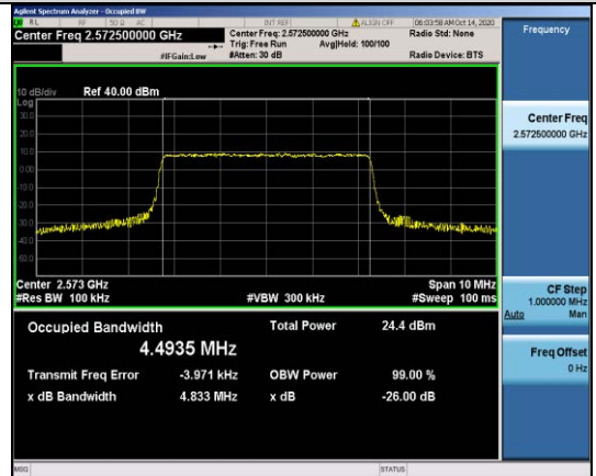
Band38-5MHz-QPSK-37775-25RB#0-4.4935
