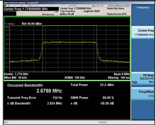
Band66-3MHz-16QAM-132657-15RB#0-2.6788
