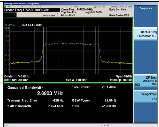
Band66-3MHz-16QAM-132322-15RB#0-2.6803
