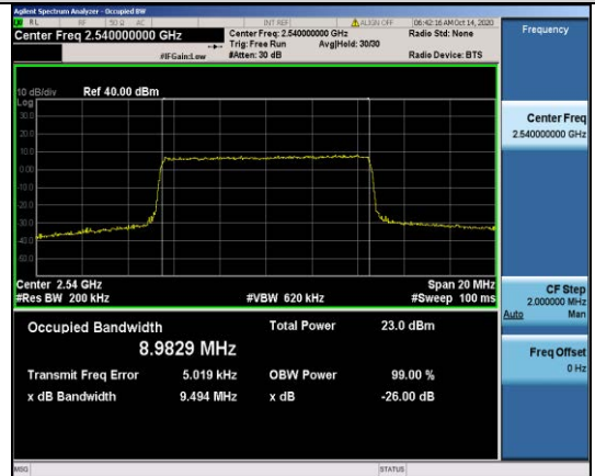
Band41-10MHz-QPSK-40090-50RB#0-8.9829
