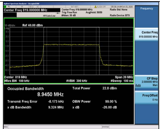
Band26-10MHz-QPSK-26740-50RB#0-8.9450
