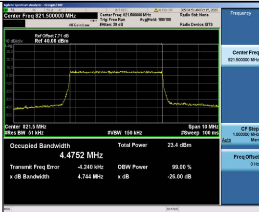
Band26-5MHz-16QAM-26765-25RB#0-4.4752
