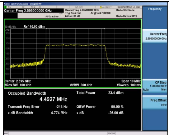
Band38-5MHz-16QAM-38000-25RB#0-4.4927
