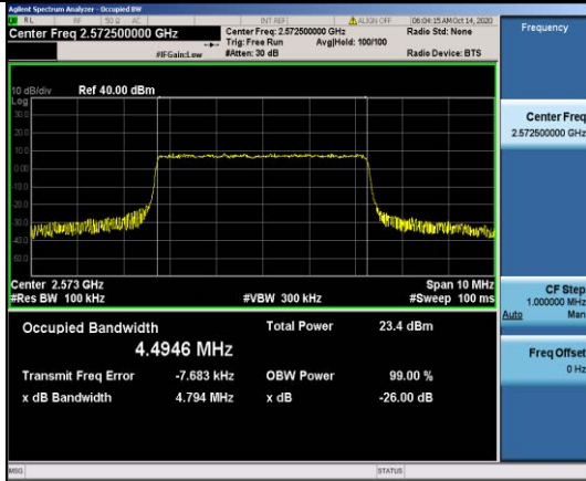
Band38-5MHz-16QAM-37775-25RB#0-4.4946
