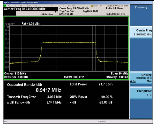
Band26-10MHz-16QAM-26740-50RB#0-8.9417
