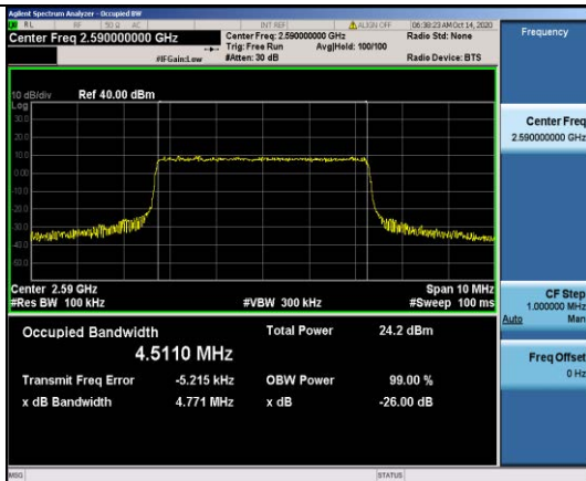
Band41-5MHz-QPSK-40590-25RB#0-4.5110
