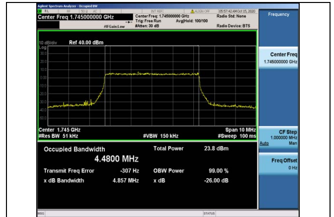
Band66-5MHz-16QAM-132322-25RB#0-4.4800
