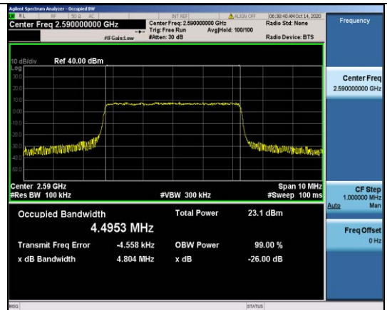
Band41-5MHz-16QAM-40590-25RB#0-4.4953
