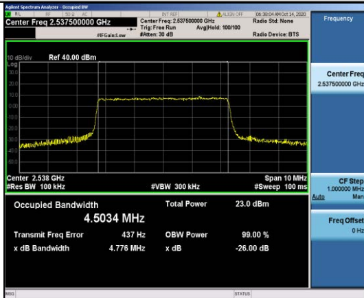
Band41-5MHz-16QAM-40065-25RB#0-4.5034
