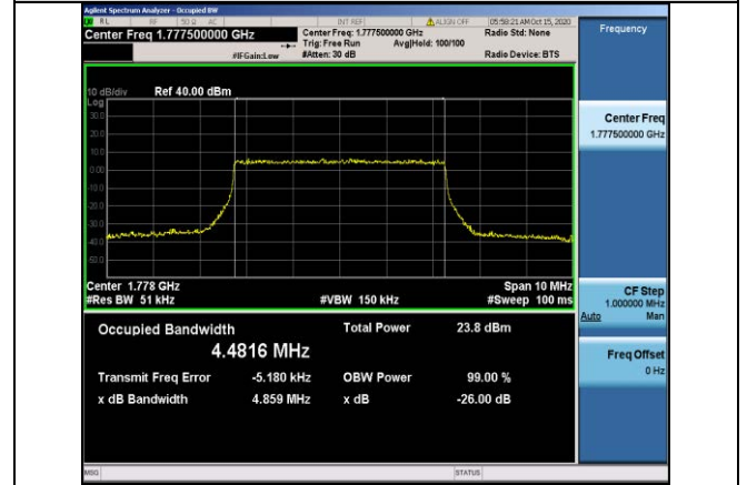
Band66-5MHz-16QAM-132647-25RB#0-4.4816
