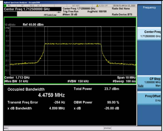
Band66-5MHz-QPSK-131997-25RB#0-4.4759
