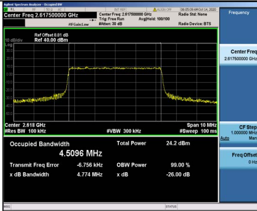
Band38-5MHz-QPSK-38225-25RB#0-4.5096
