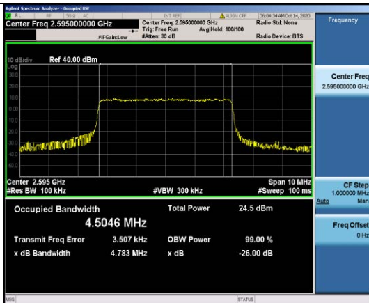
Band38-5MHz-QPSK-38000-25RB#0-4.5046
