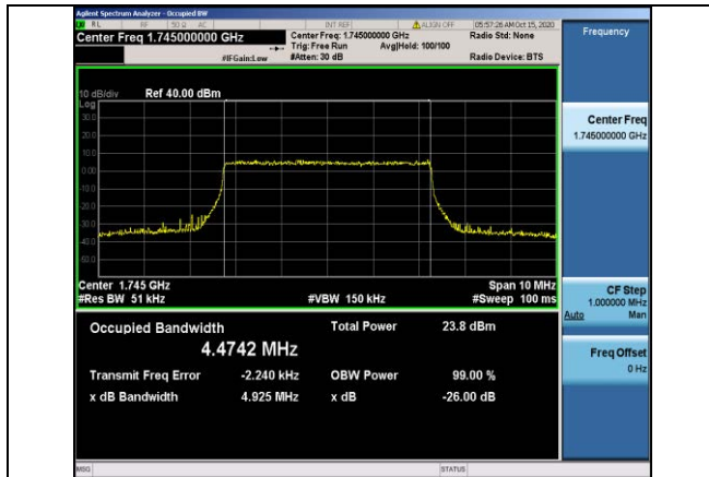
Band66-5MHz-QPSK-132322-25RB#0-4.4742
