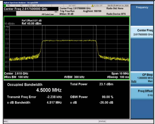
Band38-5MHz-16QAM-38225-25RB#0-4.5000
