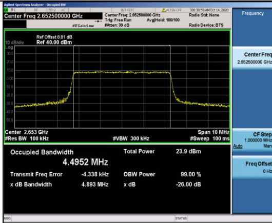
Band41-5MHz-QPSK-41215-25RB#0-4.4952
