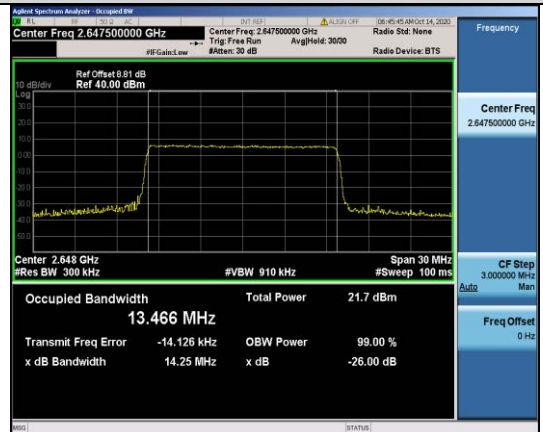
Band41-15MHz-16QAM-41165-75RB#0-13.466
