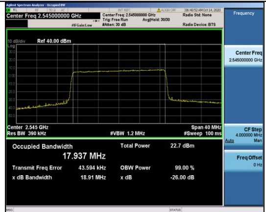
Band41-20MHz-QPSK-40140-100RB#0-17.937
