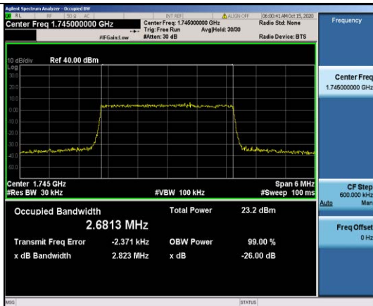
Band66-3MHz-QPSK-132322-15RB#0-2.6813
