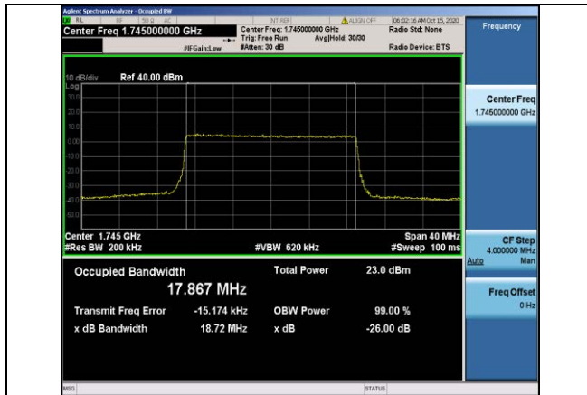
Band66-20MHz-QPSK-132322-100RB#0-17.867
