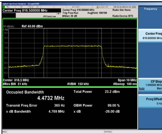
Band26-5MHz-16QAM-26715-25RB#0-4.4732
