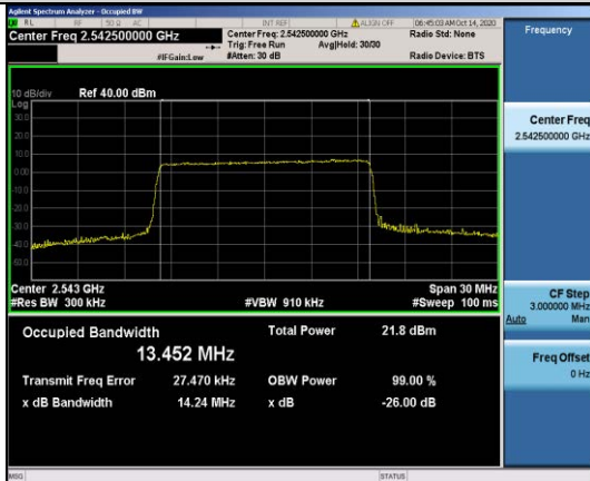
Band41-15MHz-16QAM-40115-75RB#0-13.452
