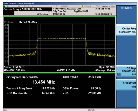
Band41-15MHz-16QAM-40590-75RB#0-13.454
