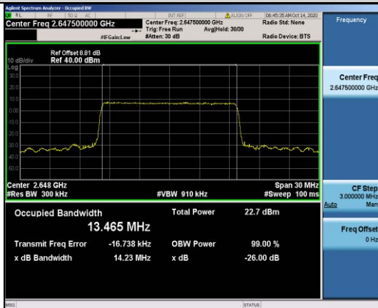
Band41-15MHz-QPSK-41165-75RB#0-13.465
