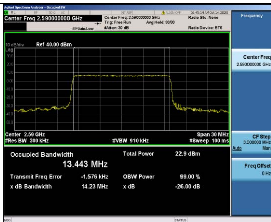
Band41-15MHz-QPSK-40590-75RB#0-13.443
