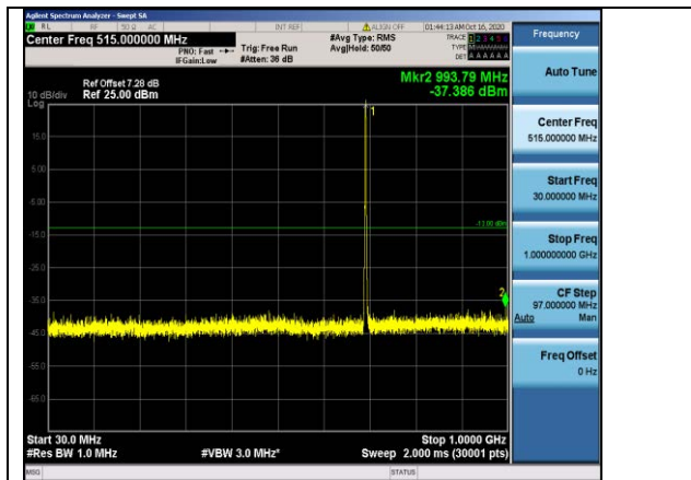
Band12-1.4MHz-16QAM-23017-1RB#0- Range1:30~1000MHz
