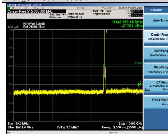
Band17-5MHz-QPSK-23825-1RB#0- Range1:30~1000MHz
