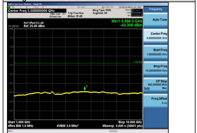
Band5-3MHz-QPSK-20635-1RB#0- Range2:1000~10000MHz
