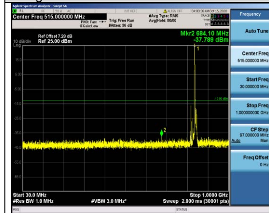
Band5-10MHz-QPSK-20600-1RB#0- Range1:30~1000MHz
