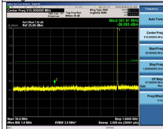
Band5-1.4MHz-16QAM-20525-1RB#0- Range1:30~1000MHz
