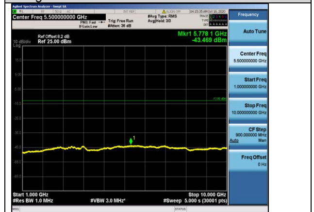
Band5-5MHz-QPSK-20625-1RB#0- Range2:1000~10000MHz
