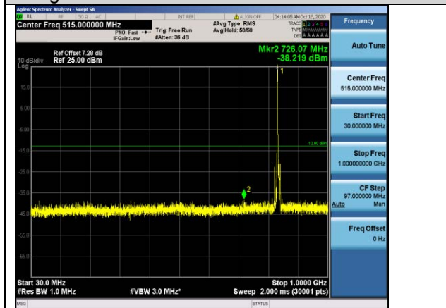
Band5-5MHz-QPSK-20525-1RB#0- Range1:30~1000MHz
