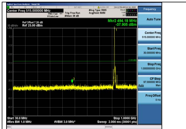
Band5-5MHz-QPSK-20425-1RB#0- Range1:30~1000MHz
