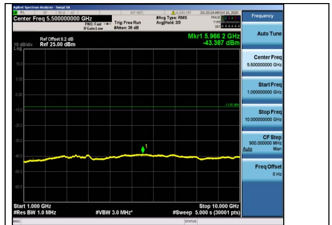
Band12-10MHz-QPSK-23060-1RB#0-Range2:1000~10000MHz
