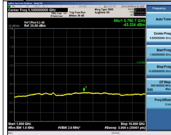
Band5-10MHz-QPSK-20600-1RB#0- Range2:1000~10000MHz
