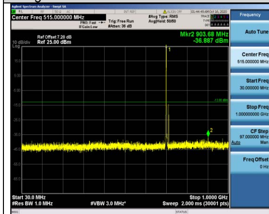
Band12-1.4MHz-QPSK-23095-1RB#0- Range1:30~1000MHz
