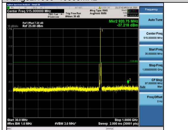
Band12-5MHz-QPSK-23095-1RB#0- Range1:30~1000MHz
