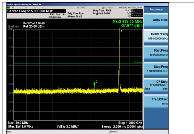
Band5-3MHz-16QAM-20415-1RB#0- Range1:30~1000MHz
