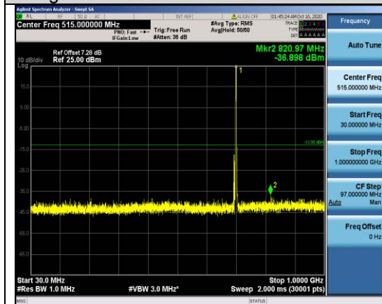
Band12-1.4MHz-16QAM-23095-1RB#0- Range1:30~1000MHz
