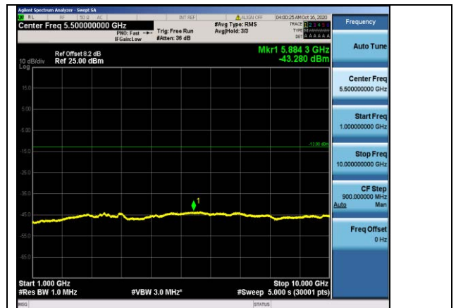
Band5-10MHz-16QAM-20525-1RB#0- Range2:1000~10000MHz
