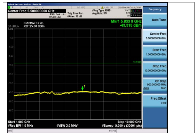
Band12-1.4MHz-16QAM-23095-1RB#0- Range2:1000~10000MHz
