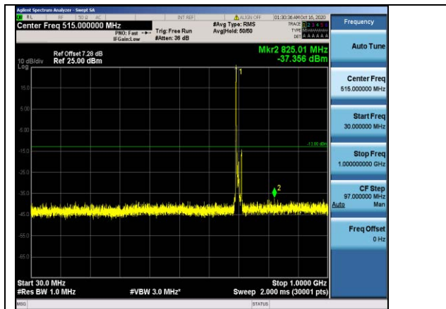
Band12-10MHz-QPSK-23060-1RB#0-Range2:30~1000MHz
