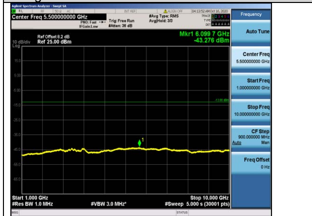
Band5-5MHz-16QAM-20425-1RB#0- Range2:1000~10000MHz
