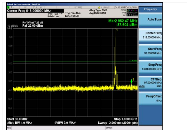
Band5-5MHz-16QAM-20425-1RB#0- Range1:30~1000MHz
