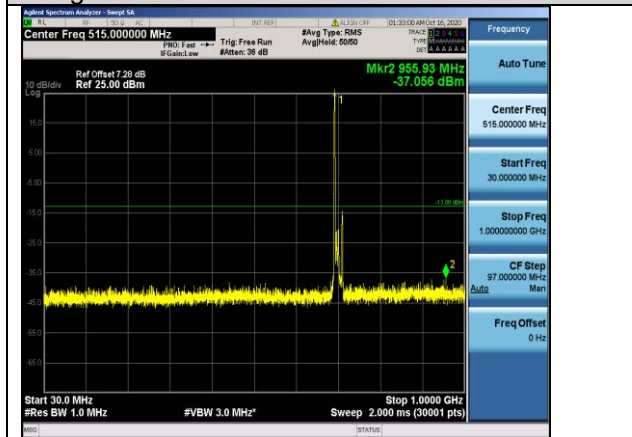
Band12-10MHz-QPSK-23060-1RB#0-Range1:30~1000MHz
