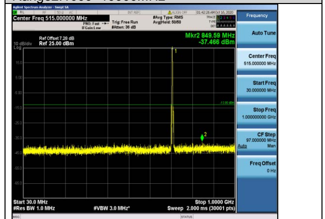
Band12-3MHz-QPSK-23165-1RB#0- Range1:30~1000MHz
