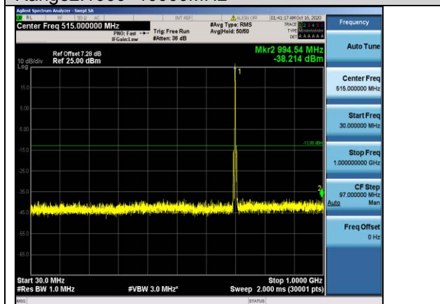
Band12-3MHz-QPSK-23095-1RB#0- Range1:30~1000MHz
