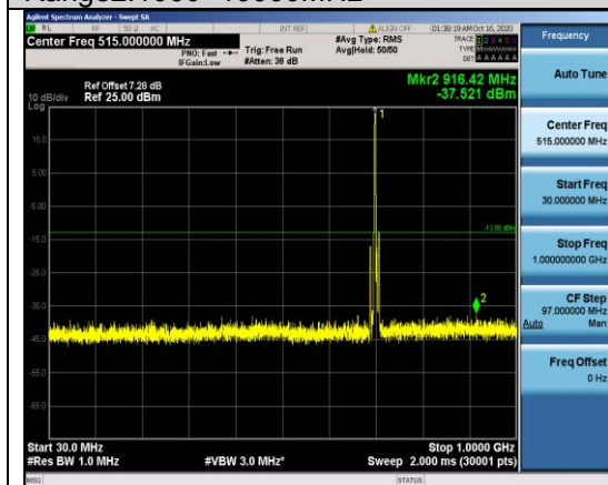
Band12-5MHz-16QAM-23095-1RB#0- Range1:30~1000MHz
