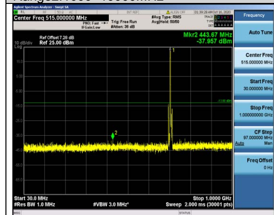
Band12-5MHz-16QAM-23155-1RB#0- Range1:30~1000MHz
