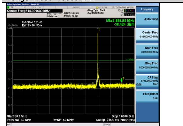
Band12-10MHz-16QAM-23130-1RB#0- Range1:30~1000MHz
