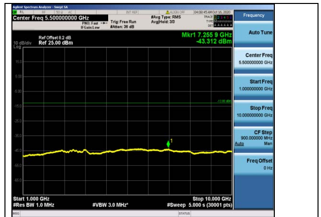
Band5-3MHz-16QAM-20525-1RB#0- Range2:1000~10000MHz
