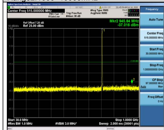
Band12-1.4MHz-QPSK-23173-1RB#0- Range1:30~1000MHz
