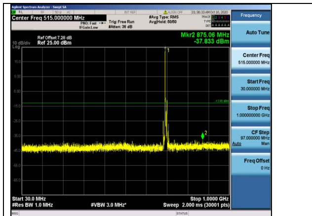
Band12-5MHz-QPSK-23035-1RB#0- Range1:30~1000MHz
