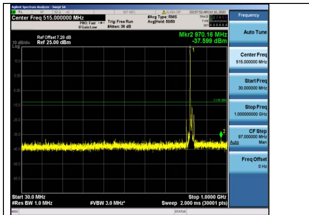
Band5-10MHz-QPSK-20450-1RB#0- Range1:30~1000MHz
