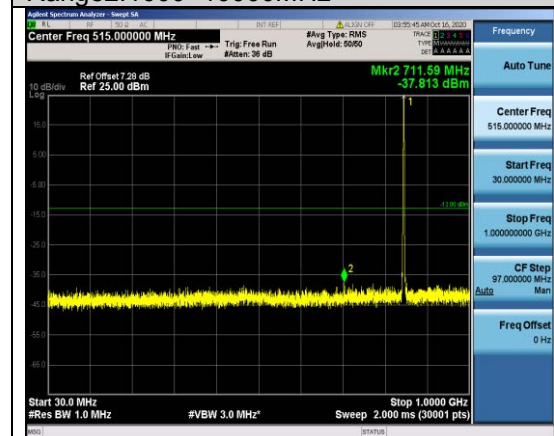
Band5-1.4MHz-16QAM-20643-1RB#0- Range1:30~1000MHz
