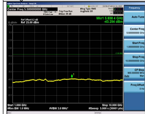
Band5-1.4MHz-16QAM-20643-1RB#0- Range2:1000~10000MHz
