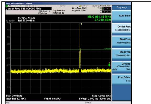
Band12-3MHz-16QAM-23025-1RB#0- Range1:30~1000MHz
