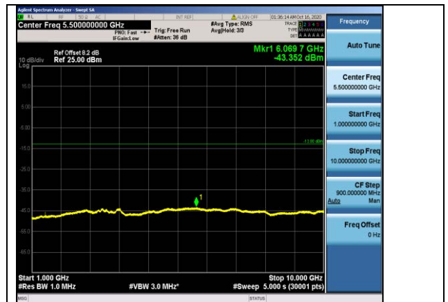
Band12-10MHz-16QAM-23130-1RB#0- Range2:1000~10000MHz
