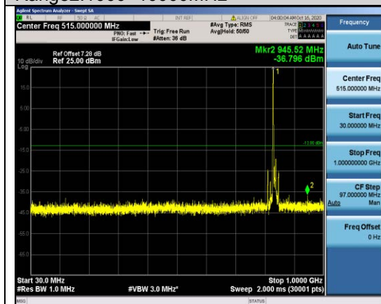
Band5-10MHz-16QAM-20525-1RB#0- Range1:30~1000MHz
