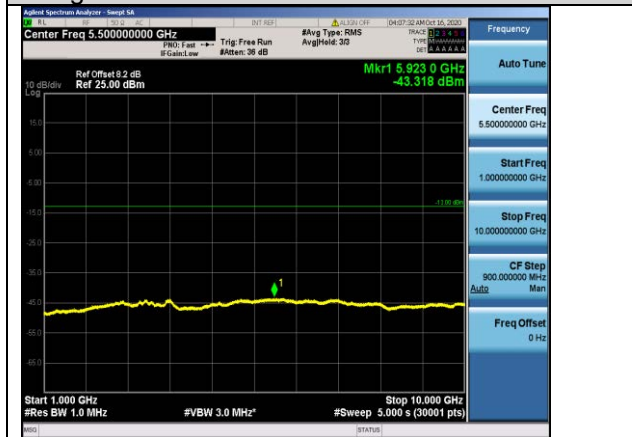
Band5-3MHz-16QAM-20415-1RB#0- Range2:1000~10000MHz
