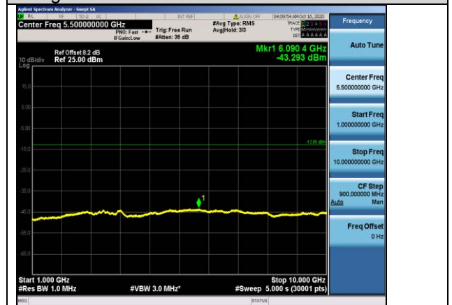
Band5-3MHz-16QAM-20635-1RB#0- Range2:1000~10000MHz
