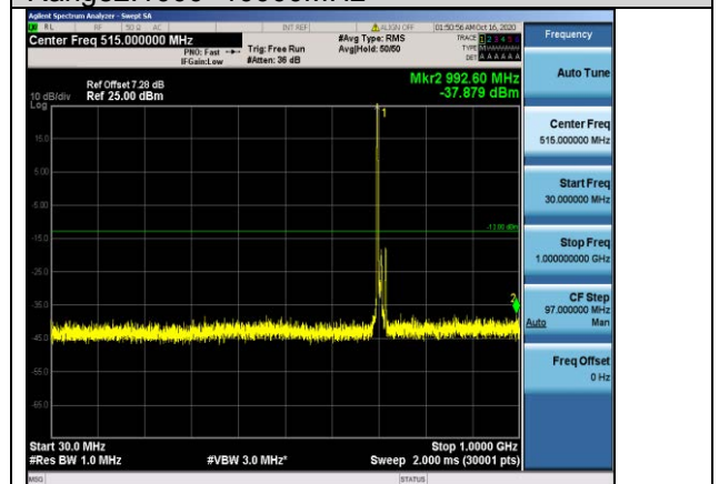
Band17-10MHz-QPSK-23780-1RB#0- Range1:30~1000MHz
