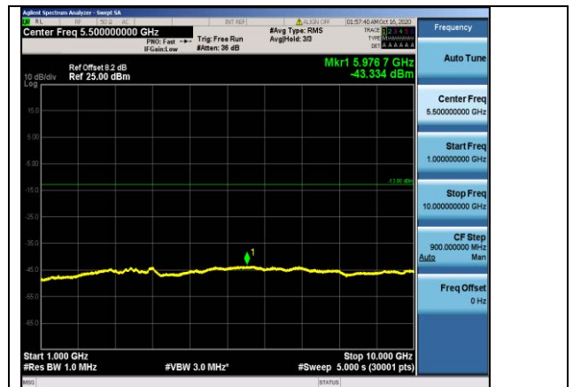
Band17-5MHz-16QAM-23825-1RB#0- Range2:1000~10000MHz
