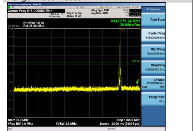
Band5-5MHz-QPSK-20625-1RB#0- Range1:30~1000MHz
