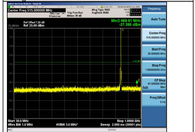
Band5-3MHz-16QAM-20635-1RB#0- Range1:30~1000MHz
