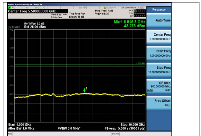
Band5-5MHz-16QAM-20525-1RB#0- Range2:1000~10000MHz
