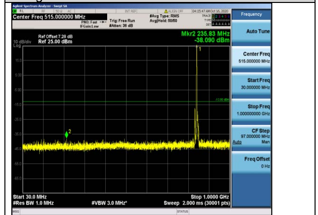
Band5-5MHz-16QAM-20625-1RB#0- Range1:30~1000MHz
