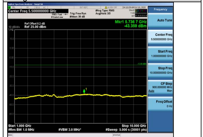
Band5-5MHz-16QAM-20625-1RB#0- Range2:1000~10000MHz
