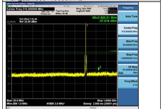
Band12-5MHz-QPSK-23155-1RB#0- Range1:30~1000MHz
