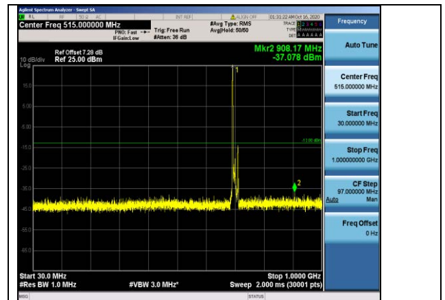
Band12-10MHz-16QAM-23060-1RB#0-Range2:30~1000MHz
