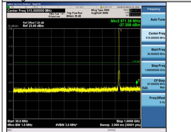
Band5-3MHz-16QAM-20525-1RB#0- Range1:30~1000MHz
