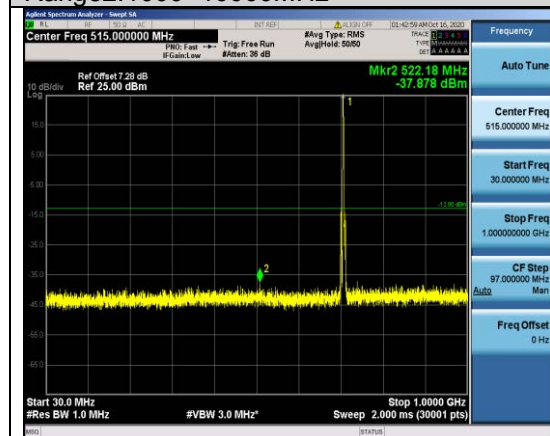
Band12-3MHz-16QAM-23165-1RB#0- Range1:30~1000MHz
