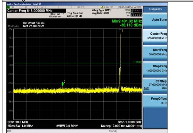
Band5-3MHz-QPSK-20525-1RB#0- Range1:30~1000MHz
