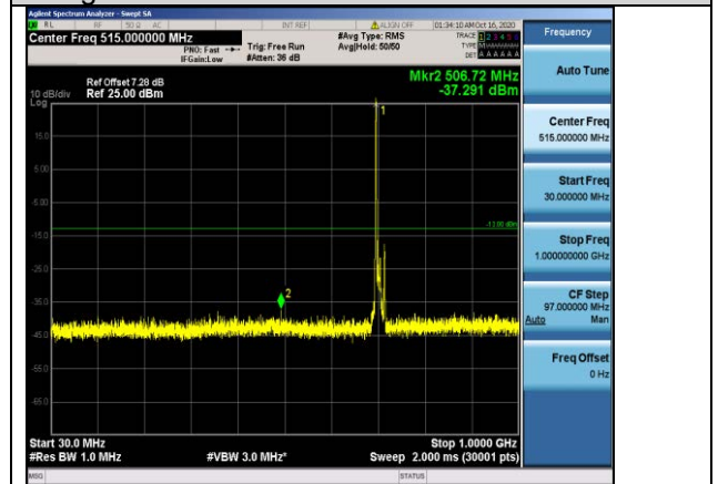
Band12-10MHz-QPSK-23095-1RB#0-Range1:30~1000MHz
