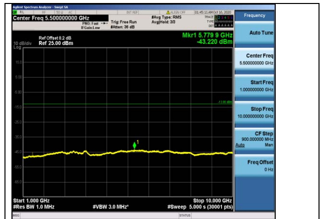
Band12-1.4MHz-QPSK-23095-1RB#0- Range2:1000~10000MHz
