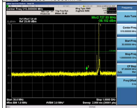
Band5-10MHz-16QAM-20600-1RB#0- Range1:30~1000MHz
