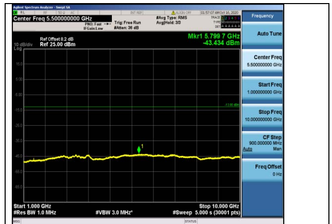
Band17-5MHz-QPSK-23825-1RB#0- Range2:1000~10000MHz
