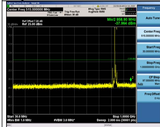
Band5-10MHz-QPSK-20525-1RB#0- Range1:30~1000MHz
