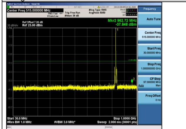
Band5-5MHz-16QAM-20525-1RB#0- Range1:30~1000MHz
