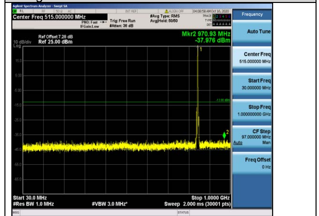
Band5-3MHz-QPSK-20635-1RB#0- Range1:30~1000MHz
