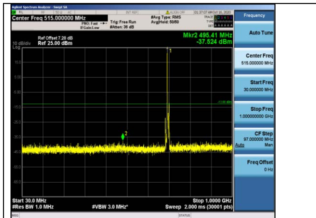
Band12-5MHz-16QAM-23035-1RB#0- Range1:30~1000MHz
