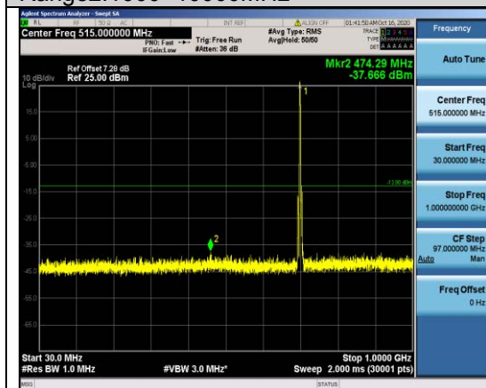
Band12-3MHz-16QAM-23095-1RB#0- Range1:30~1000MHz
