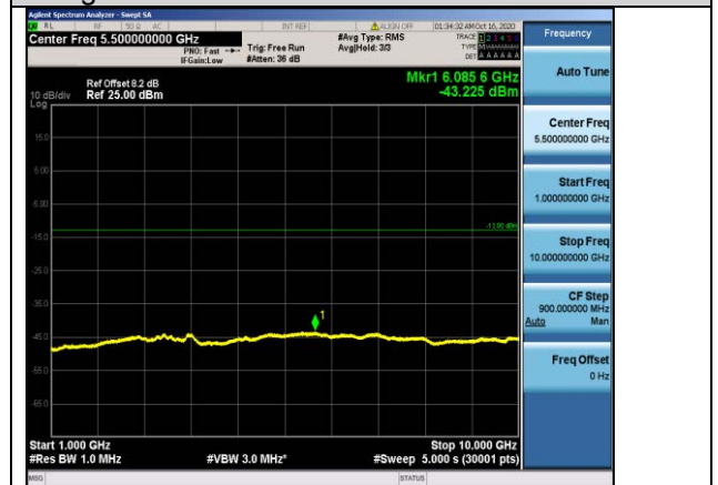
Band12-10MHz-QPSK-23095-1RB#0-Range2:1000~10000MHz
