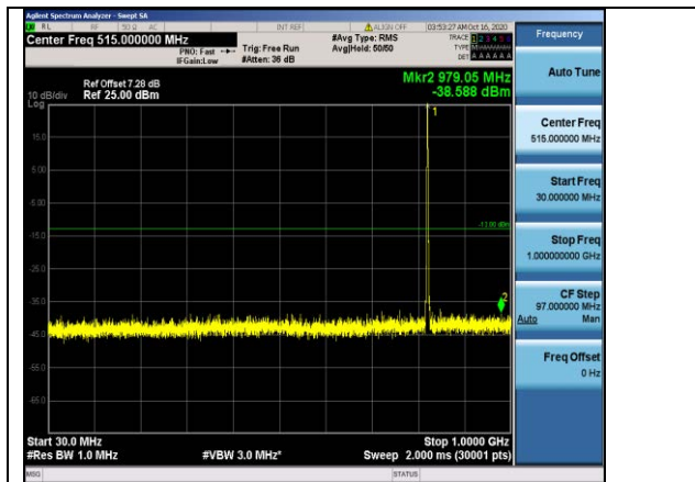
Band5-1.4MHz-16QAM-20407-1RB#0- Range1:30~1000MHz
