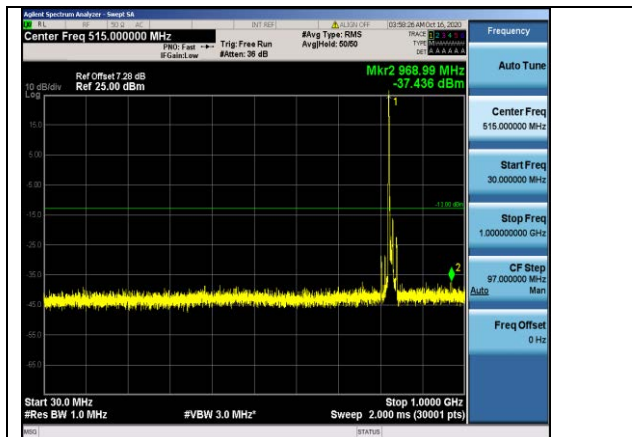
Band5-10MHz-16QAM-20450-1RB#0- Range1:30~1000MHz
