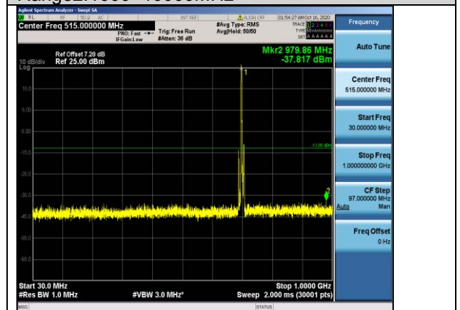
Band17-5MHz-QPSK-23755-1RB#0- Range1:30~1000MHz
