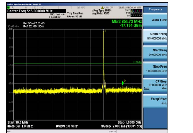
Band12-10MHz-QPSK-23130-1RB#0-Range1:30~1000MHz
