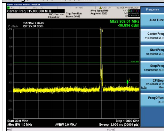
Band12-10MHz-16QAM-23060-1RB#0-Range1:30~1000MHz
