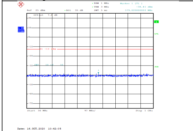
Band2-20MHz-QPSK-18700-1RB#0-Range1:30~1000MHz--38.45-PASS
