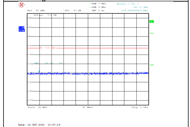
Band4-3MHz-16QAM-20175-1RB#0-Range1:30~1000MHz--38.73-PASS
