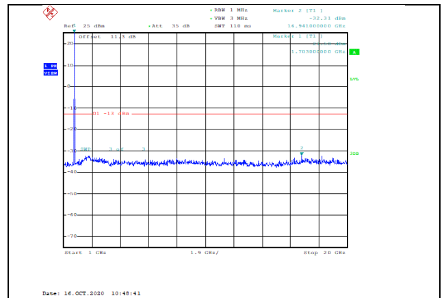
Band4-5MHz-QPSK-19975-1RB#0-Range2:1000~20000MHz--32.31-PASS
