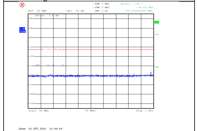
Band4-1.4MHz-QPSK-20175-1RB#0-Range1:30~1000MHz--38.24-PASS
