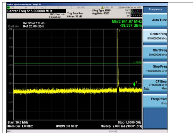
Band26-5MHz-QPSK-26740-1RB#0- Range1:30~1000MHz
