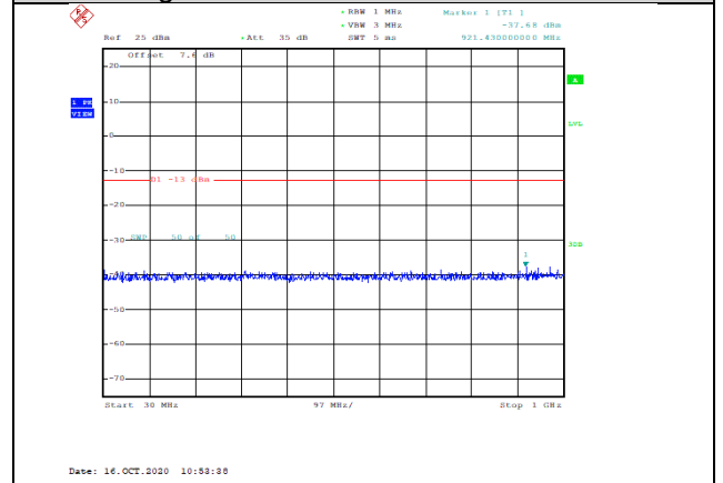
Band4-15MHz-QPSK-20175-1RB#0-Range1:30~1000MHz--37.68-PASS
