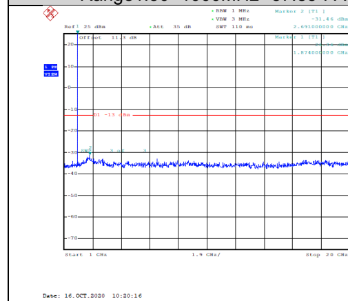
Band2-1.4MHz-QPSK-18900-1RB#0- Range2:1000~20000MHz--31.46-PASS
