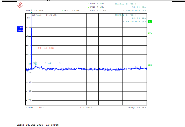
Band2-20MHz-16QAM-19100-1RB#0-Range2:1000~20000MHz--32.11-PASS
