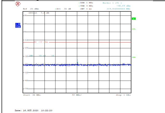
Band2-3MHz-QPSK-18615-1RB#0-Range1:30~1000MHz--38.39-PASS
