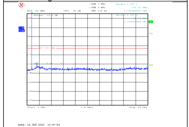
Band4-3MHz-16QAM-20175-1RB#0-Range2:1000~20000MHz--32.31-PASS
