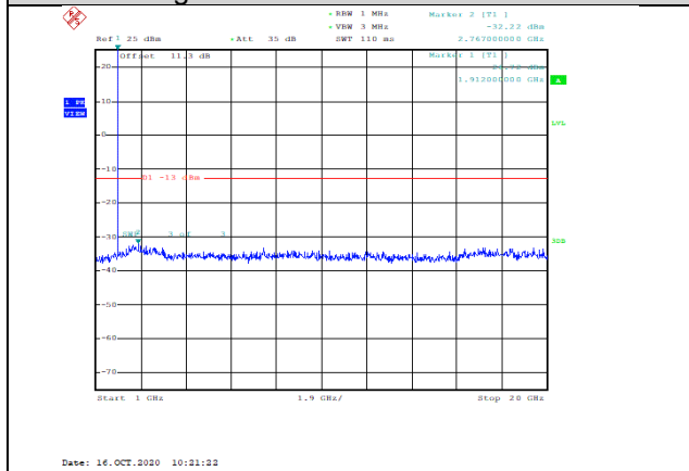
Band2-1.4MHz-QPSK-19193-1RB#0-Range2:1000~20000MHz--32.22-PASS
