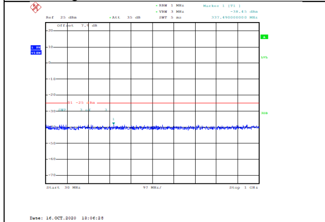
Band7-5MHz-QPSK-21425-1RB#0-Range1:30~1000MHz--38.45-PASS
