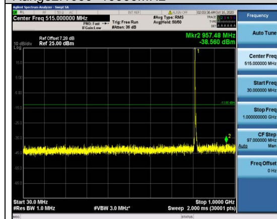
Band26-5MHz-QPSK-26715-1RB#0- Range1:30~1000MHz
