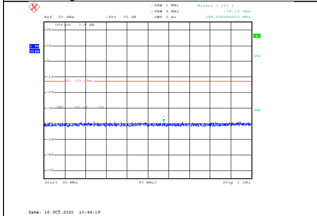
Band4-1.4MHz-16QAM-19957-1RB#0-Range1:30~1000MHz--38.52-PASS
