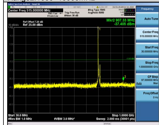
Band17-10MHz-16QAM-23780-1RB#0- Range1:30~1000MHz
