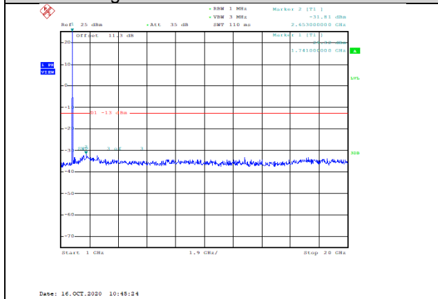
Band4-1.4MHz-QPSK-20393-1RB#0-Range2:1000~20000MHz--31.81-PASS
