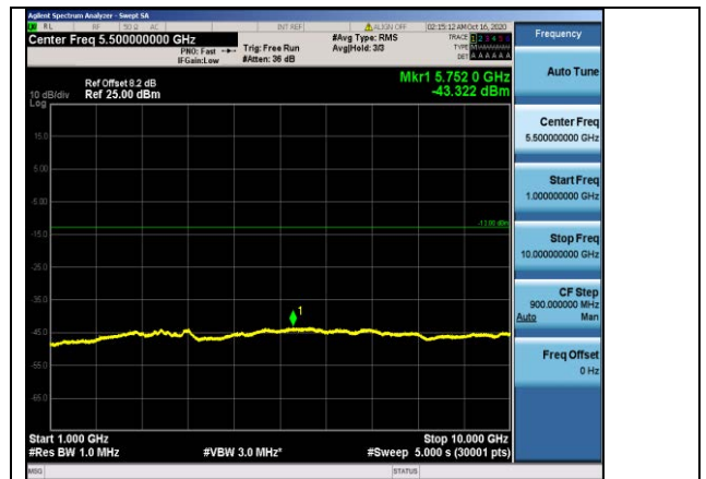
Band26-3MHz-16QAM-26775-1RB#0- Range2:1000~10000MHz
