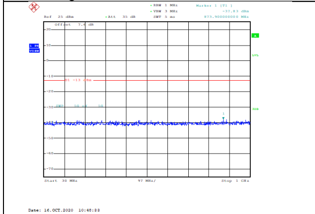
Band4-5MHz-QPSK-19975-1RB#0-Range1:30~1000MHz--37.83-PASS
