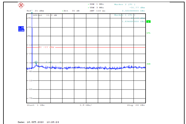
Band2-10MHz-QPSK-18650-1RB#0-Range2:1000~20000MHz--31.77-PASS
