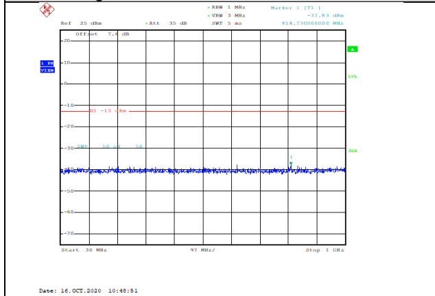
Band4-5MHz-16QAM-19975-1RB#0-Range1:30~1000MHz--37.83-PASS
