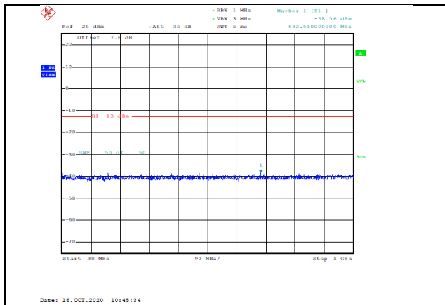
Band4-1.4MHz-16QAM-20393-1RB#0-Range1:30~1000MHz--38.56-PASS
