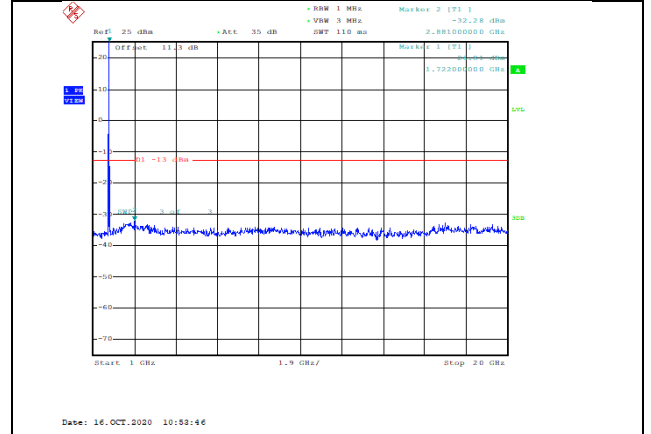
Band4-15MHz-QPSK-20175-1RB#0-Range2:1000~20000MHz--32.28-PASS
