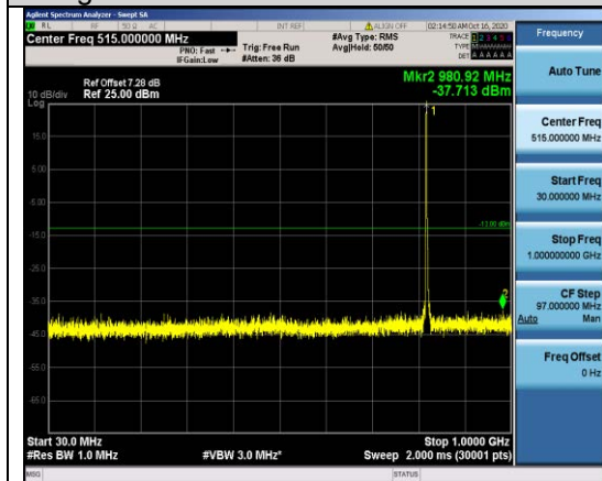
Band26-3MHz-16QAM-26775-1RB#0- Range1:30~1000MHz
