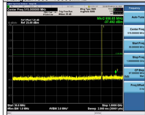
Band26-1.4MHz-16QAM-26697-1RB#0- Range1:30~1000MHz
