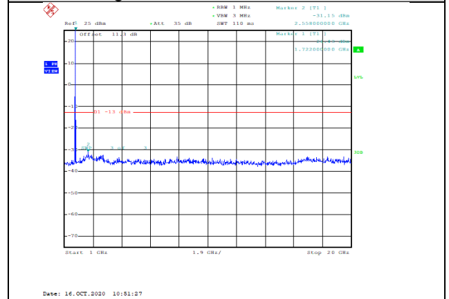
Band4-10MHz-QPSK-20175-1RB#0-Range2:1000~20000MHz--31.15-PASS
