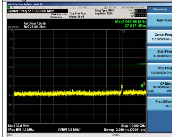
Band26-1.4MHz-QPSK-26783-1RB#0- Range1:30~1000MHz
