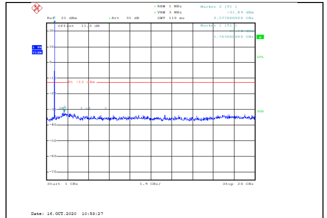
Band4-15MHz-16QAM-20025-1RB#0-Range2:1000~20000MHz--31.89-PASS
