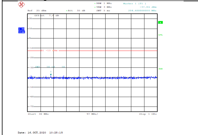
Band2-10MHz-QPSK-18650-1RB#0-Range1:30~1000MHz--37.86-PASS
