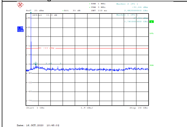
Band4-3MHz-16QAM-20385-1RB#0-Range2:1000~20000MHz--31.66-PASS
