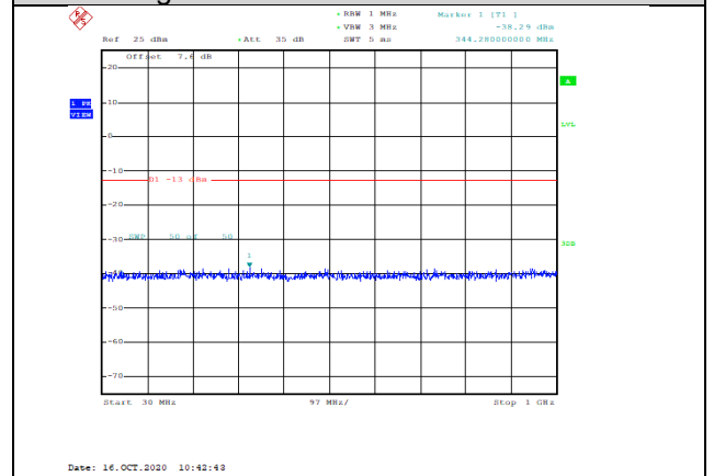
Band2-20MHz-QPSK-18900-1RB#0-Range1:30~1000MHz--38.29-PASS
