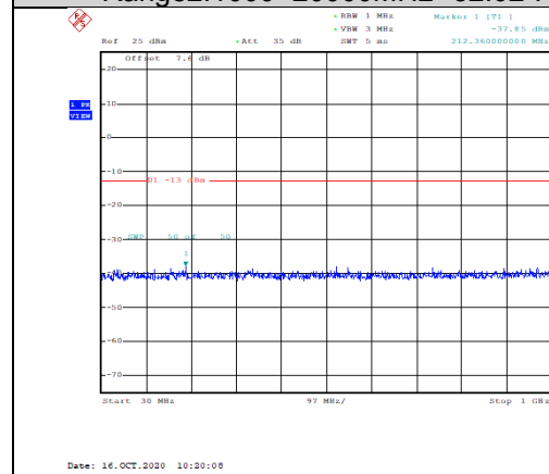
Band2-1.4MHz-QPSK-18900-1RB#0- Range1:30~1000MHz--37.85-PASS
