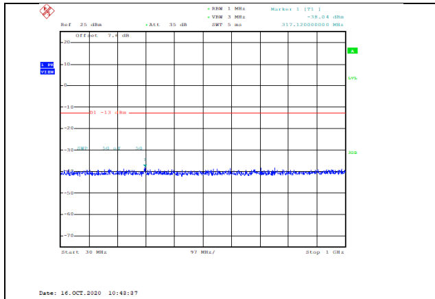
Band2-20MHz-16QAM-19100-1RB#0-Range1:30~1000MHz--38.04-PASS
