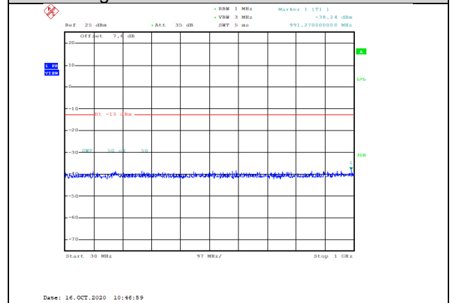
Band4-3MHz-QPSK-20175-1RB#0-Range1:30~1000MHz--38.24-PASS
