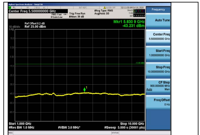
Band26-1.4MHz-QPSK-26783-1RB#0- Range2:1000~10000MHz
