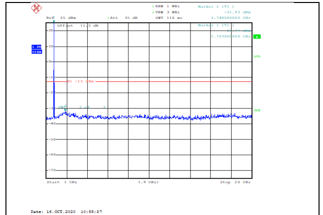
Band4-20MHz-16QAM-20050-1RB#0-Range2:1000~20000MHz--31.93-PASS
