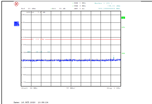
Band4-20MHz-QPSK-20300-1RB#0-Range1:30~1000MHz--38.31-PASS
