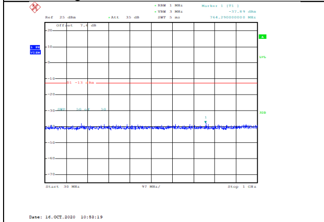
Band4-15MHz-16QAM-20025-1RB#0-Range1:30~1000MHz--37.89-PASS
