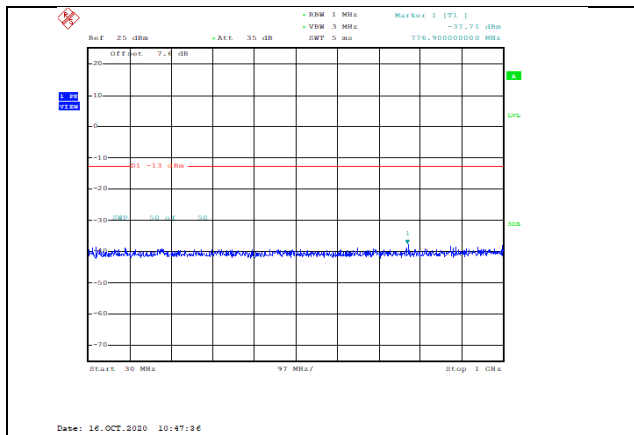
Band4-3MHz-QPSK-20385-1RB#0-Range1:30~1000MHz--37.71-PASS
