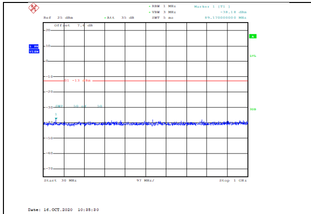
Band2-15MHz-QPSK-19125-1RB#0-Range1:30~1000MHz--38.18-PASS
