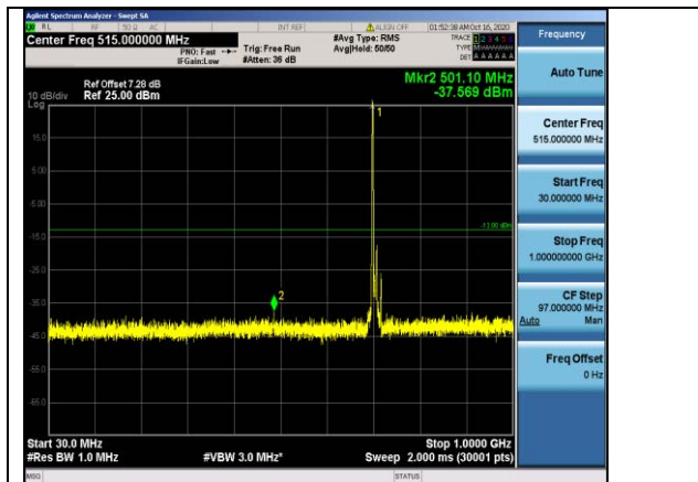
Band17-10MHz-16QAM-23790-1RB#0- Range1:30~1000MHz
