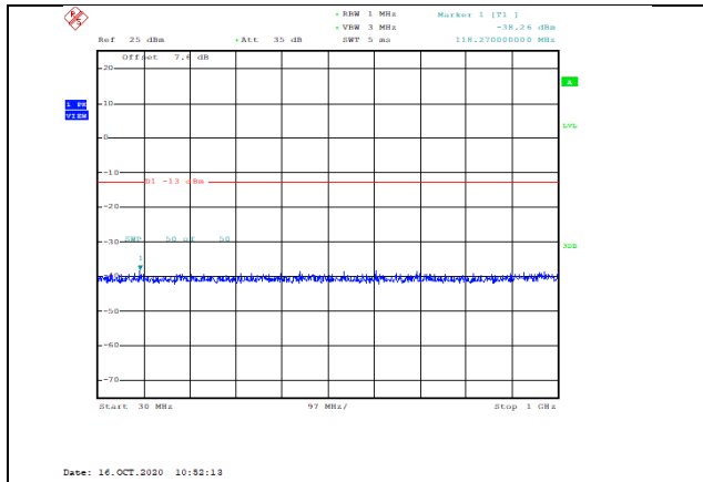
Band4-10MHz-16QAM-20350-1RB#0-Range1:30~1000MHz--38.26-PASS
