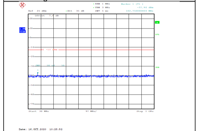
Band2-10MHz-QPSK-18900-1RB#0-Range1:30~1000MHz--37.9-PASS
