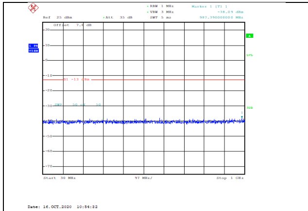
Band4-15MHz-16QAM-20325-1RB#0-Range1:30~1000MHz--38.09-PASS
