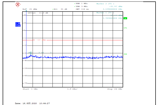
Band4-1.4MHz-16QAM-19957-1RB#0-Range2:1000~20000MHz--31.97-PASS
