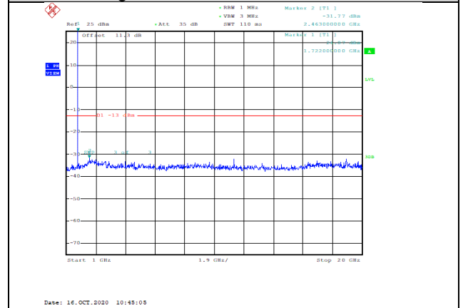
Band4-1.4MHz-16QAM-20175-1RB#0-Range2:1000~20000MHz--31.77-PASS
