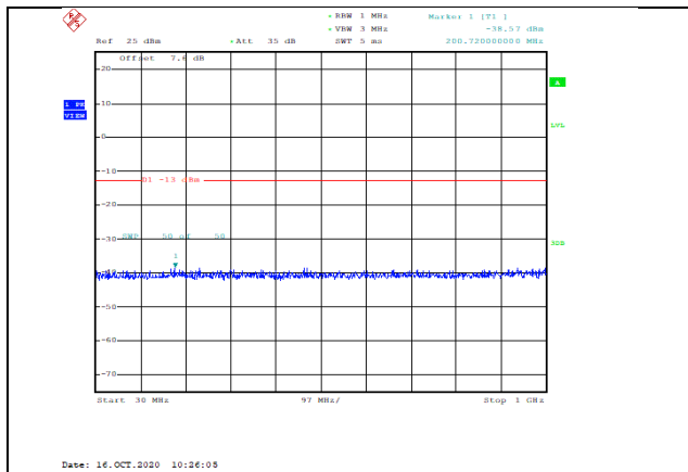
Band2-5MHz-16QAM-19175-1RB#0-Range1:30~1000MHz--38.57-PASS
