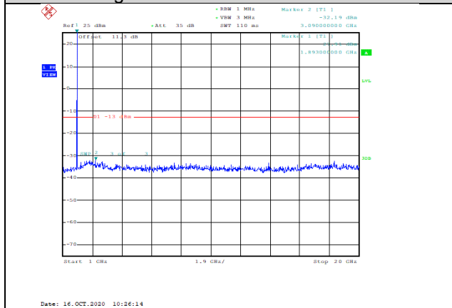
Band2-5MHz-16QAM-19175-1RB#0-Range2:1000~20000MHz--32.19-PASS
