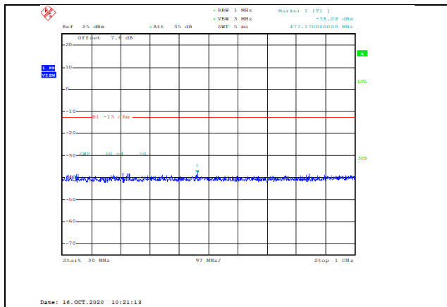
Band2-1.4MHz-QPSK-19193-1RB#0-Range1:30~1000MHz--38.08-PASS
