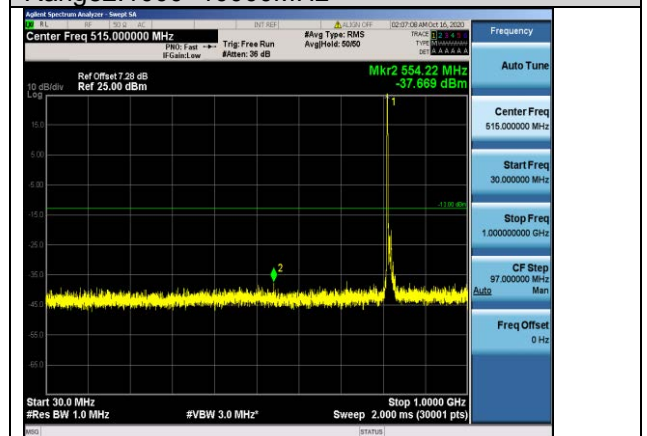
Band26-10MHz-QPSK-26740-1RB#0- Range1:30~1000MHz
