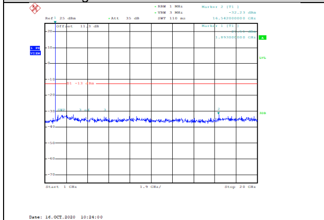
Band2-3MHz-16QAM-19185-1RB#0-Range2:1000~20000MHz--32.23-PASS
