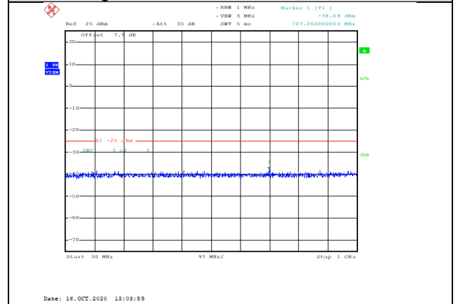
Band7-5MHz-16QAM-20775-1RB#0-Range1:30~1000MHz--38.08-PASS
