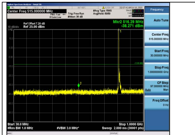
Band26-10MHz-16QAM-26740-1RB#0- Range1:30~1000MHz
