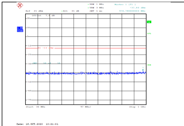
Band2-1.4MHz-16QAM-19193-1RB#0-Range1:30~1000MHz--37.8-PASS
