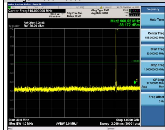
Band26-1.4MHz-QPSK-26697-1RB#0- Range1:30~1000MHz
