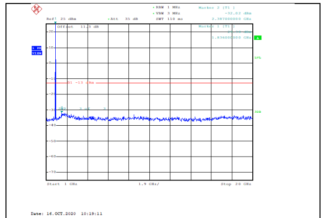
Band2-1.4MHz-QPSK-18607-1RB#0- Range2:1000~20000MHz--32.02-PASS
