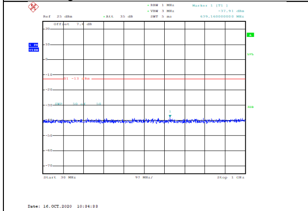
Band2-15MHz-16QAM-18675-1RB#0-Range1:30~1000MHz--37.91-PASS
