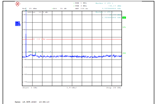
Band4-1.4MHz-QPSK-19957-1RB#0-Range2:1000~20000MHz--32.17-PASS
