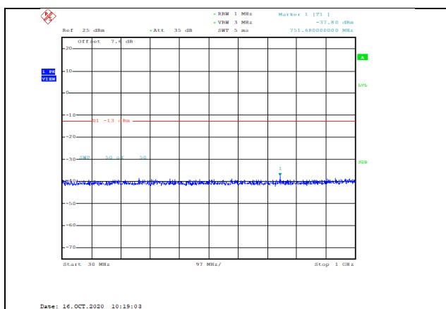
Band2-1.4MHz-QPSK-18607-1RB#0- Range1:30~1000MHz--37.8-PASS
