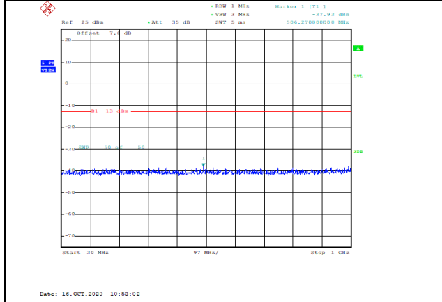
Band4-15MHz-QPSK-20025-1RB#0-Range1:30~1000MHz--37.93-PASS
