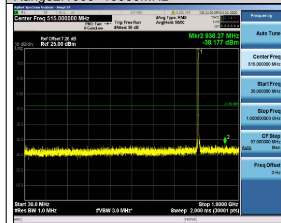
Band26-3MHz-QPSK-26705-1RB#0- Range1:30~1000MHz
