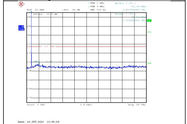
Band4-5MHz-16QAM-20175-1RB#0-Range2:1000~20000MHz--32.28-PASS
