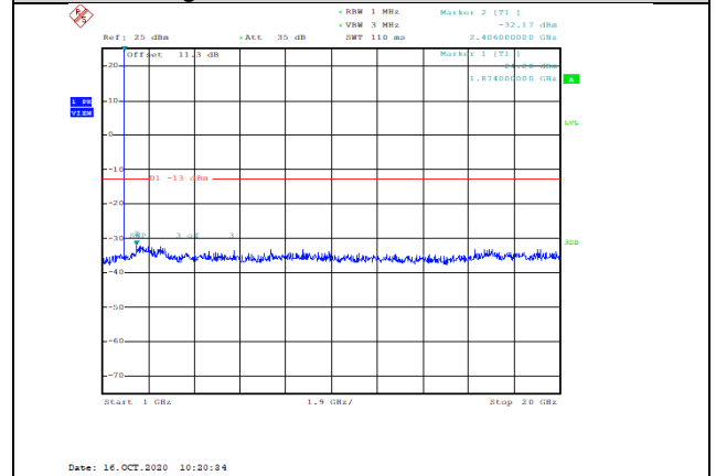
Band2-1.4MHz-16QAM-18900-1RB#0-Range2:1000~20000MHz--32.17-PASS
