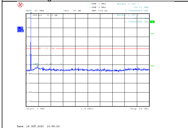
Band4-20MHz-QPSK-20300-1RB#0-Range2:1000~20000MHz--32.37-PASS
