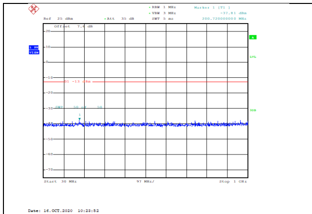
Band2-3MHz-16QAM-19185-1RB#0-Range1:30~1000MHz--37.81-PASS
