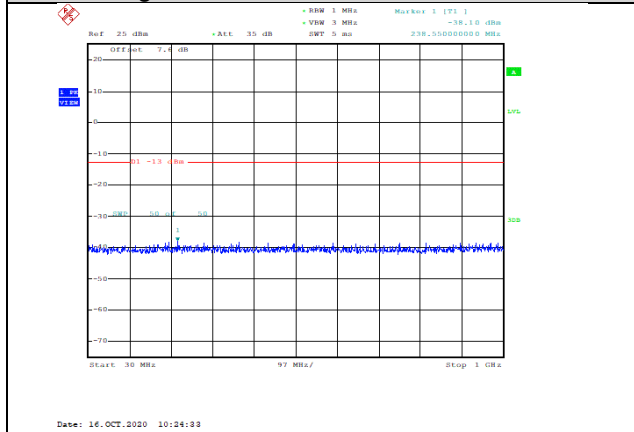
Band2-5MHz-QPSK-18625-1RB#0-Range1:30~1000MHz--38.1-PASS
