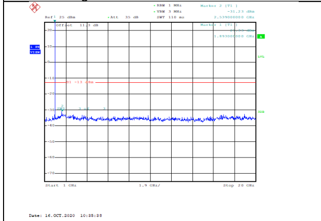
Band2-15MHz-QPSK-19125-1RB#0-Range2:1000~20000MHz--31.23-PASS
