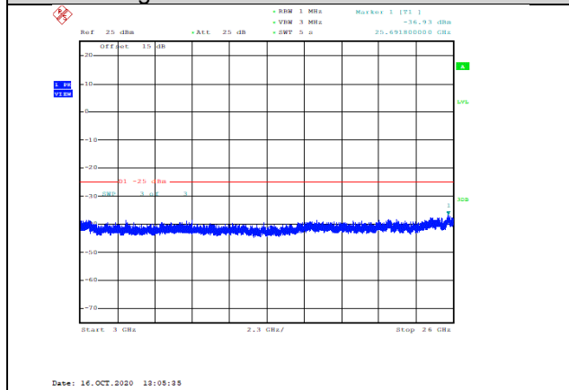
Band7-5MHz-QPSK-21100-1RB#0-Range3:3000~26000MHz--36.93-PASS
