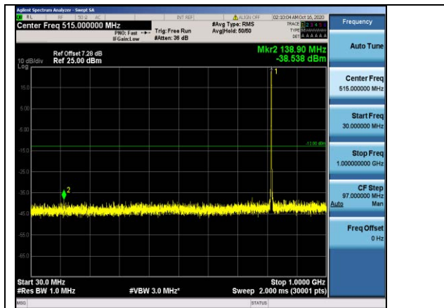
Band26-1.4MHz-16QAM-26740-1RB#0- Range1:30~1000MHz
