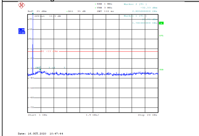
Band4-3MHz-QPSK-20385-1RB#0-Range2:1000~20000MHz--32.33-PASS
