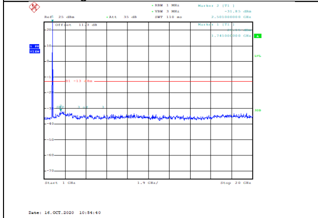
Band4-15MHz-16QAM-20325-1RB#0-Range2:1000~20000MHz--31.85-PASS
