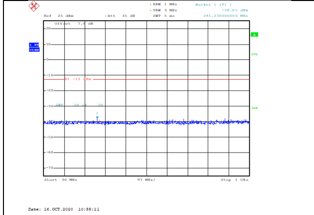
Band4-20MHz-QPSK-20050-1RB#0-Range1:30~1000MHz--38.05-PASS
