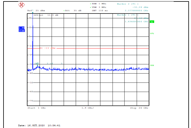
Band2-15MHz-16QAM-18675-1RB#0-Range2:1000~20000MHz--32.28-PASS
