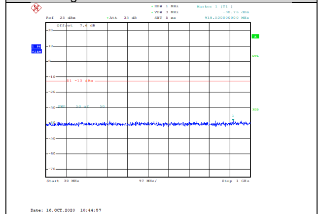
Band4-1.4MHz-16QAM-20175-1RB#0-Range1:30~1000MHz--38.76-PASS
