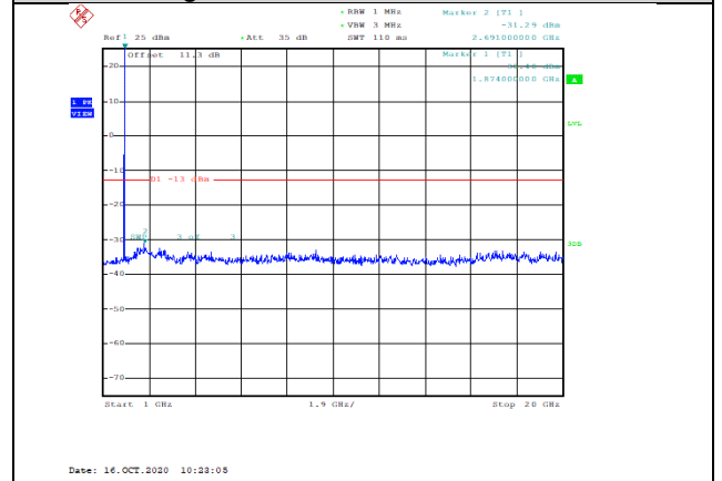
Band2-3MHz-QPSK-18900-1RB#0-Range2:1000~20000MHz--31.29-PASS
