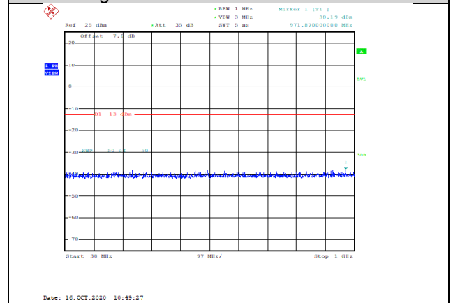
Band4-5MHz-16QAM-20175-1RB#0-Range1:30~1000MHz--38.19-PASS
