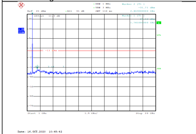
Band4-1.4MHz-16QAM-20393-1RB#0-Range2:1000~20000MHz--31.71-PASS
