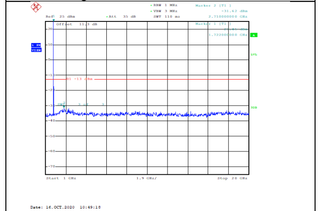
Band4-5MHz-QPSK-20175-1RB#0-Range2:1000~20000MHz--31.62-PASS
