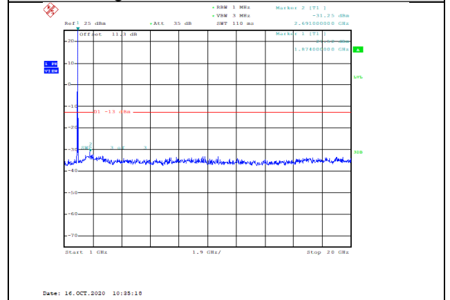
Band2-15MHz-16QAM-18900-1RB#0-Range2:1000~20000MHz--31.25-PASS
