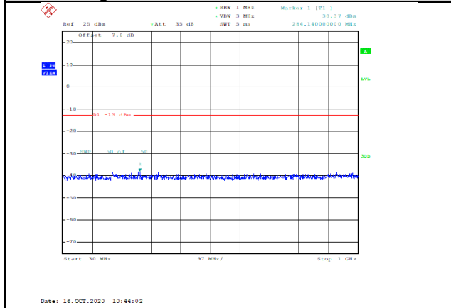
Band4-1.4MHz-QPSK-19957-1RB#0-Range1:30~1000MHz--38.37-PASS
