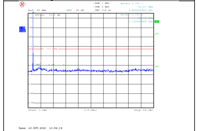
Band4-15MHz-16QAM-20175-1RB#0-Range2:1000~20000MHz--32.01-PASS
