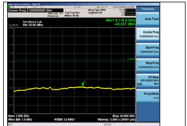
Band17-10MHz-QPSK-23800-1RB#0- Range2:1000~10000MHz
