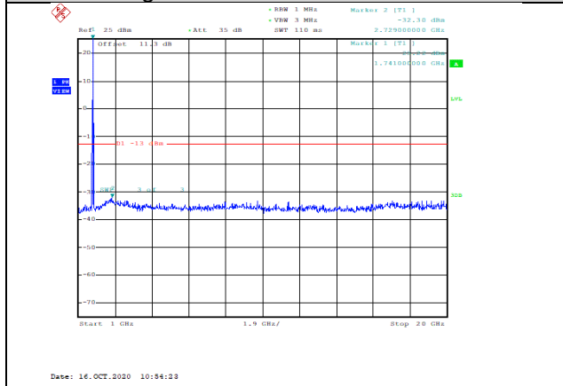
Band4-15MHz-QPSK-20325-1RB#0-Range2:1000~20000MHz--32.3-PASS
