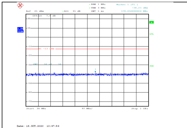
Band4-3MHz-16QAM-20385-1RB#0-Range1:30~1000MHz--38.25-PASS
