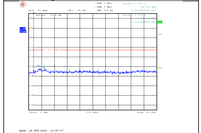
Band4-3MHz-QPSK-20175-1RB#0-Range2:1000~20000MHz--32.18-PASS
