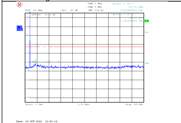
Band4-5MHz-16QAM-20375-1RB#0-Range2:1000~20000MHz--31.25-PASS
