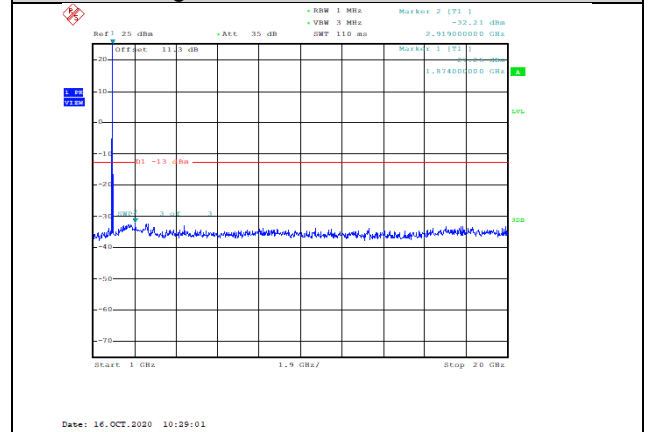
Band2-10MHz-QPSK-18900-1RB#0-Range2:1000~20000MHz--32.21-PASS
