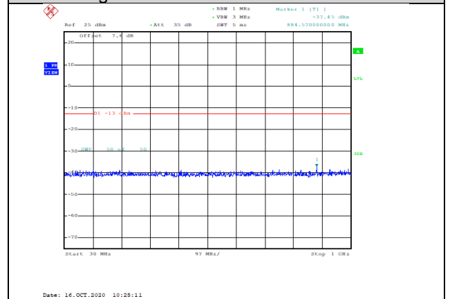
Band2-5MHz-QPSK-18900-1RB#0-Range1:30~1000MHz--37.45-PASS
