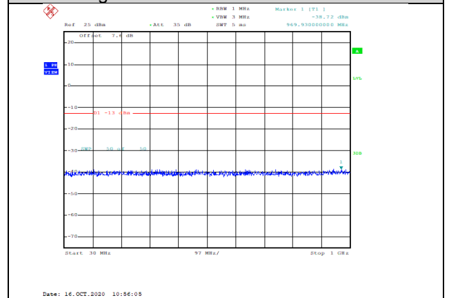
Band4-20MHz-16QAM-20175-1RB#0-Range1:30~1000MHz--38.72-PASS
