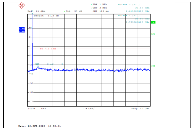
Band4-10MHz-QPSK-20000-1RB#0-Range2:1000~20000MHz--32.53-PASS
