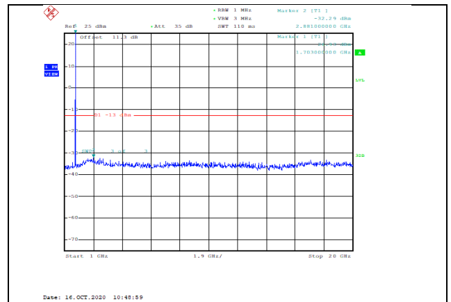
Band4-5MHz-16QAM-19975-1RB#0-Range2:1000~20000MHz--32.29-PASS
