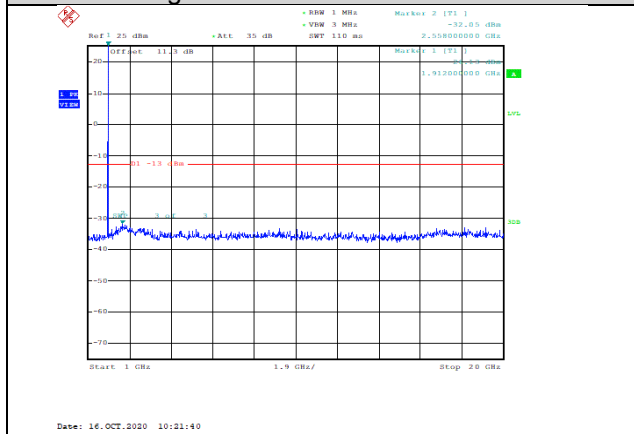
Band2-1.4MHz-16QAM-19193-1RB#0-Range2:1000~20000MHz--32.05-PASS
