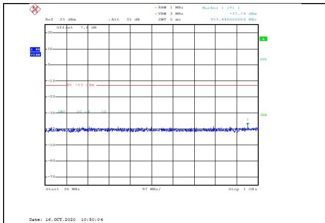
Band4-5MHz-16QAM-20375-1RB#0-Range1:30~1000MHz--37.76-PASS
