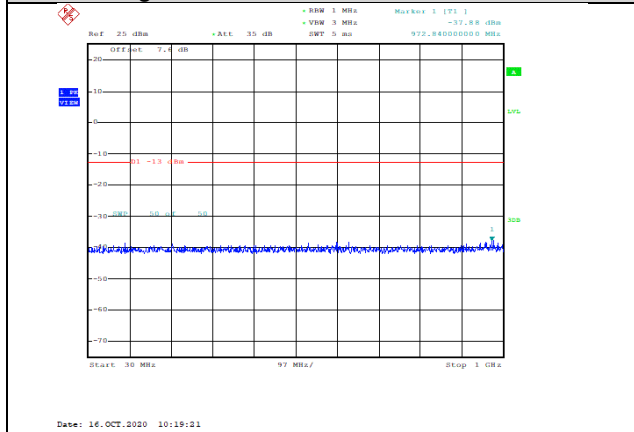
Band2-1.4MHz-16QAM-18607-1RB#0-Range1:30~1000MHz--37.88-PASS
