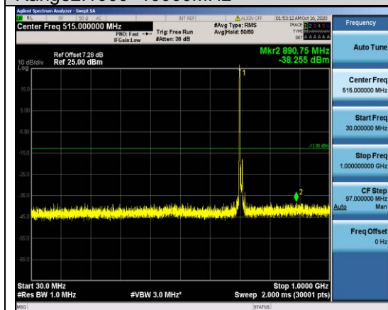
Band17-10MHz-QPSK-23800-1RB#0- Range1:30~1000MHz
