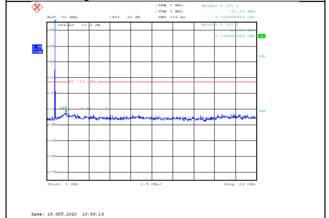
Band4-20MHz-16QAM-20175-1RB#0-Range2:1000~20000MHz--32.32-PASS
