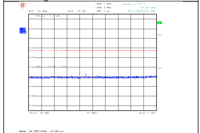
Band4-5MHz-QPSK-20175-1RB#0-Range1:30~1000MHz--38.08-PASS
