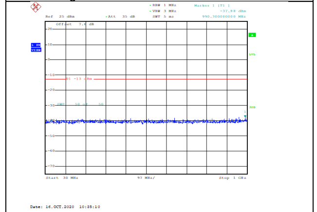
Band2-15MHz-16QAM-18900-1RB#0-Range1:30~1000MHz--37.88-PASS
