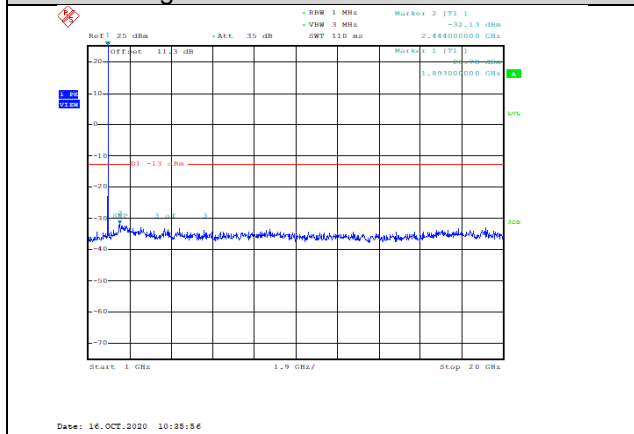
Band2-15MHz-16QAM-19125-1RB#0-Range2:1000~20000MHz--32.13-PASS
