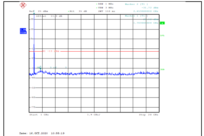
Band4-20MHz-QPSK-20050-1RB#0-Range2:1000~20000MHz--31.72-PASS
