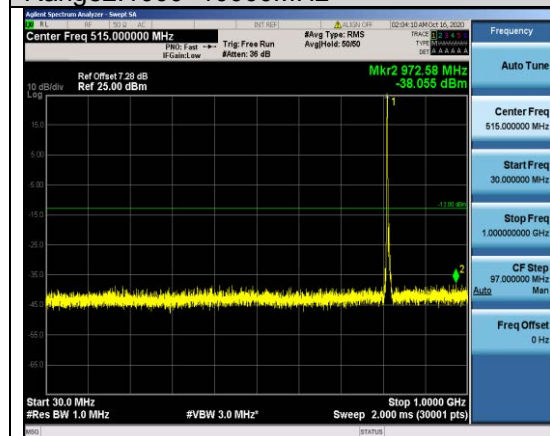
Band26-5MHz-16QAM-26715-1RB#0- Range1:30~1000MHz
