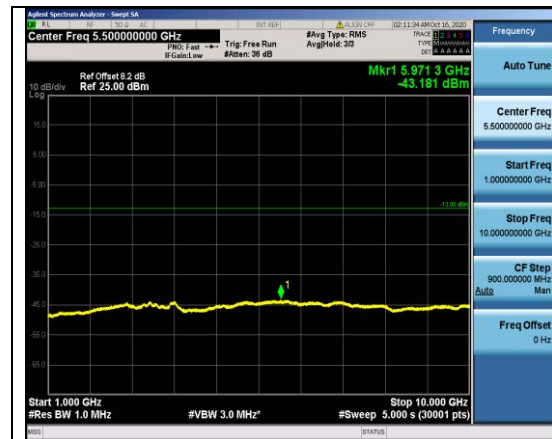
Band26-1.4MHz-16QAM-26783-1RB#0- Range2:1000~10000MHz
