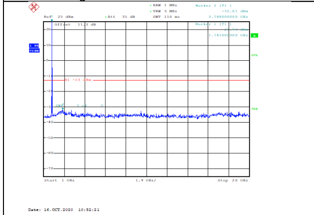
Band4-10MHz-16QAM-20350-1RB#0-Range2:1000~20000MHz--32.01-PASS
