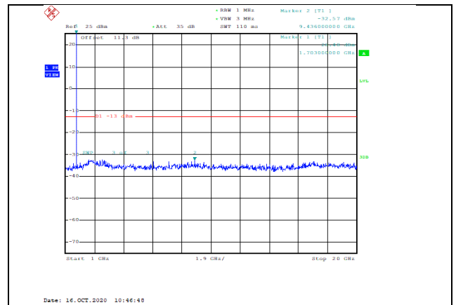
Band4-3MHz-16QAM-19965-1RB#0-Range2:1000~20000MHz--32.57-PASS
