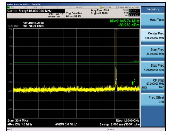
Band26-3MHz-QPSK-26740-1RB#0- Range1:30~1000MHz
