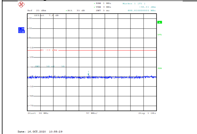
Band4-20MHz-16QAM-20050-1RB#0-Range1:30~1000MHz--38.31-PASS
