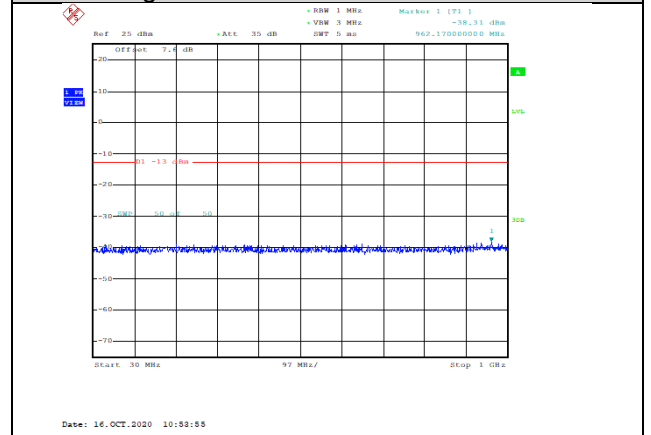
Band4-15MHz-16QAM-20175-1RB#0-Range1:30~1000MHz--38.31-PASS
