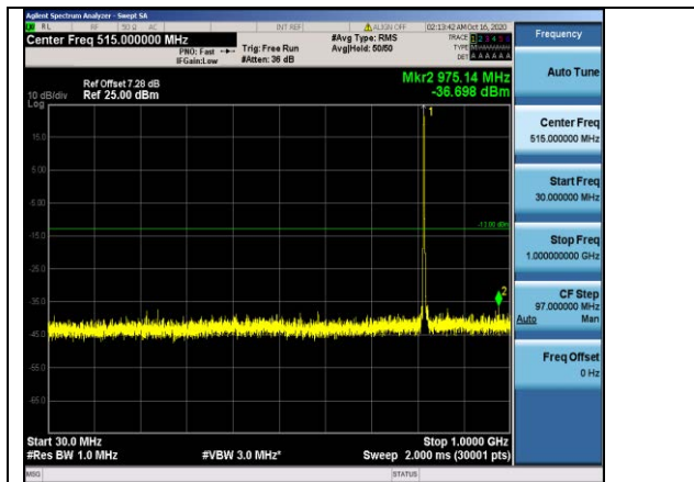
Band26-3MHz-16QAM-26740-1RB#0- Range1:30~1000MHz
