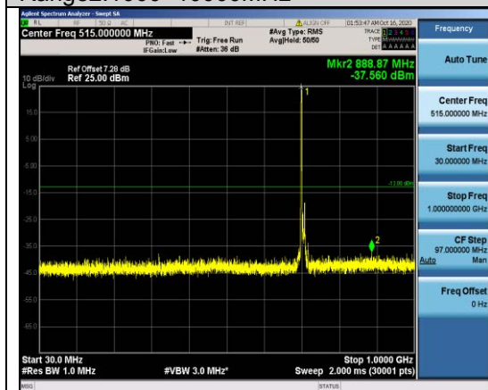
Band17-10MHz-16QAM-23800-1RB#0- Range1:30~1000MHz
