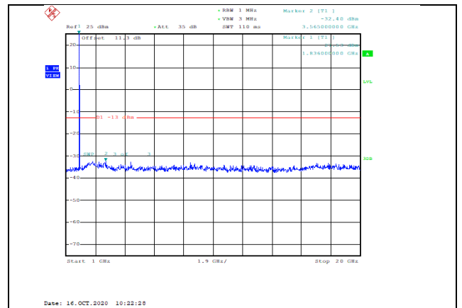
Band2-3MHz-QPSK-18615-1RB#0-Range2:1000~20000MHz--32.4-PASS
