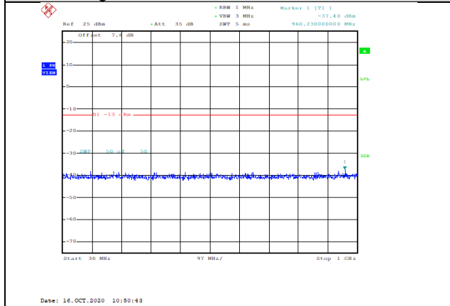
Band4-10MHz-QPSK-20000-1RB#0-Range1:30~1000MHz--37.4-PASS
