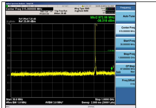
Band26-5MHz-16QAM-26740-1RB#0- Range1:30~1000MHz
