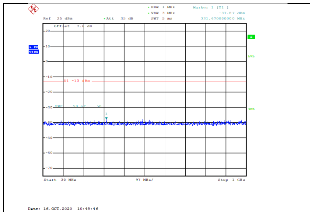
Band4-5MHz-QPSK-20375-1RB#0-Range1:30~1000MHz--37.87-PASS
