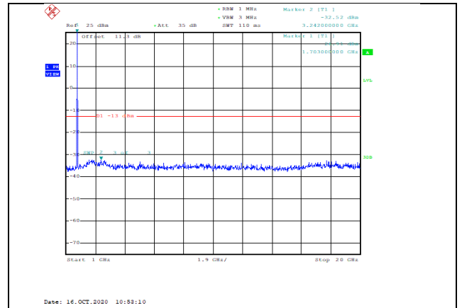
Band4-15MHz-QPSK-20025-1RB#0-Range2:1000~20000MHz--32.52-PASS
