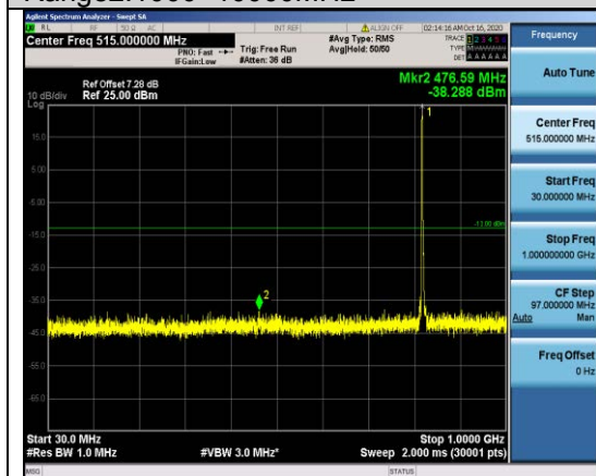
Band26-3MHz-QPSK-26775-1RB#0- Range1:30~1000MHz
