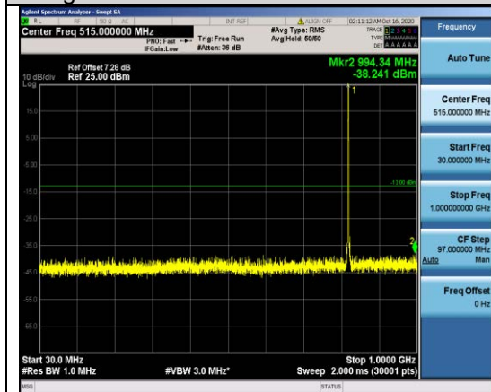
Band26-1.4MHz-16QAM-26783-1RB#0- Range1:30~1000MHz
