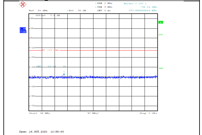
Band4-20MHz-QPSK-20175-1RB#0-Range1:30~1000MHz--38.36-PASS
