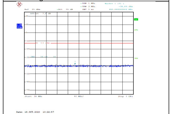
Band2-3MHz-QPSK-18900-1RB#0-Range1:30~1000MHz--38.49-PASS
