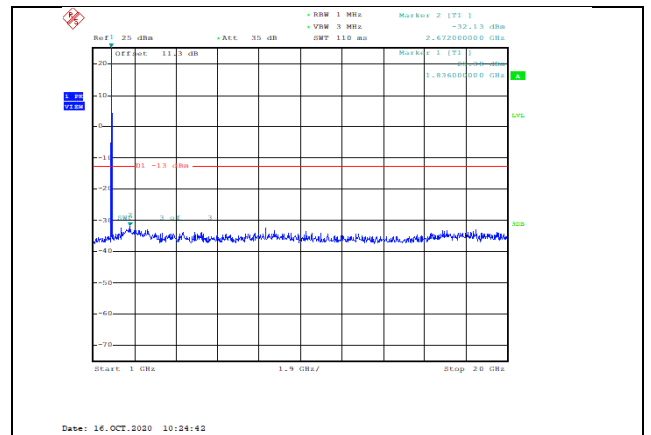
Band2-5MHz-QPSK-18625-1RB#0-Range2:1000~20000MHz--32.13-PASS
