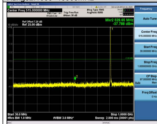
Band26-3MHz-16QAM-26705-1RB#0- Range1:30~1000MHz
