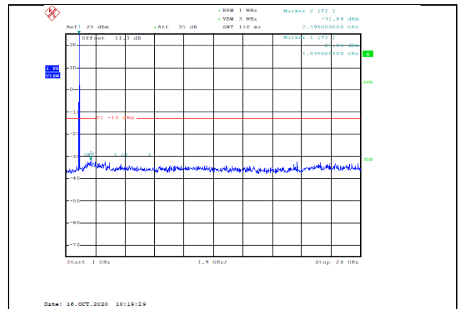
Band2-1.4MHz-16QAM-18607-1RB#0-Range2:1000~20000MHz--31.84-PASS
