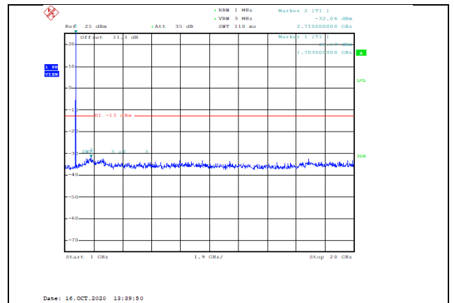
Band66-1.4MHz-16QAM-131979-1RB#0-Range2:1000~20000MHz--32.06-PASS
