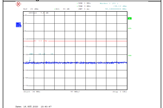
Band66-1.4MHz-16QAM-132322-1RB#0-Range1:30~1000MHz--38.12-PASS
