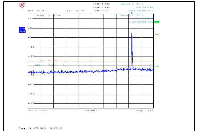
Band41-5MHz-QPSK-41215-1RB#0-Range2:1000~3000MHz--32.48-PASS
