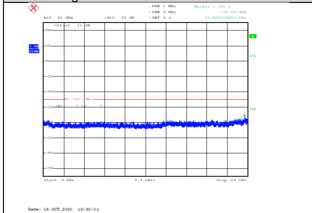
Band38-15MHz-16QAM-37825-1RB#0-Range3:3000~26000MHz--36.64-PASS
