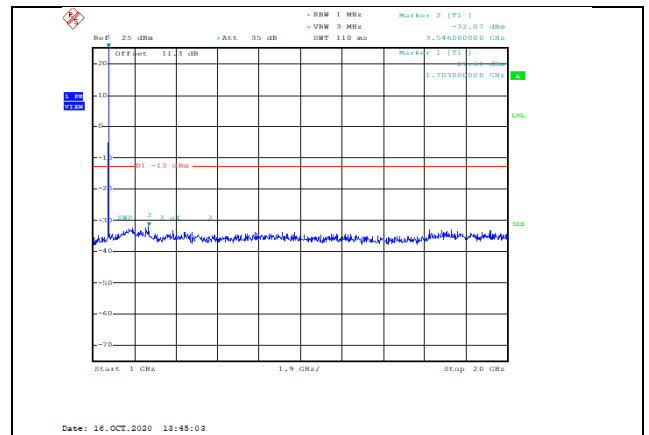
Band66-5MHz-QPSK-131997-1RB#0-Range2:1000~20000MHz--32.07-PASS
