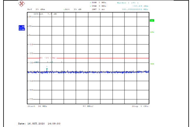
Band41-20MHz-QPSK-40590-1RB#0-Range1:30~1000MHz--37.69-PASS
