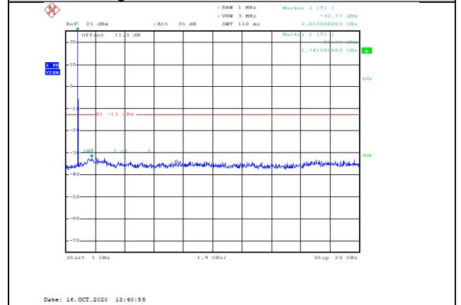
Band66-1.4MHz-16QAM-132322-1RB#0-Range2:1000~20000MHz--32.37-PASS
