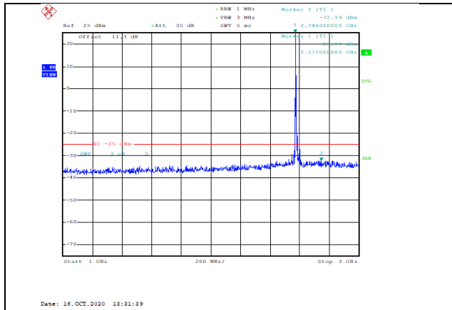
Band38-15MHz-16QAM-37825-1RB#0-Range2:1000~3000MHz--32.39-PASS
