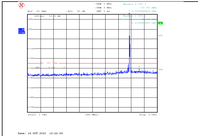
Band38-5MHz-16QAM-37775-1RB#0-Range2:1000~3000MHz--31.95-PASS
