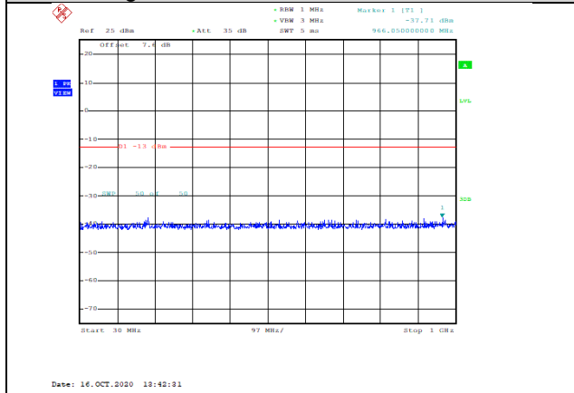
Band66-3MHz-QPSK-131987-1RB#0-Range1:30~1000MHz--37.71-PASS
