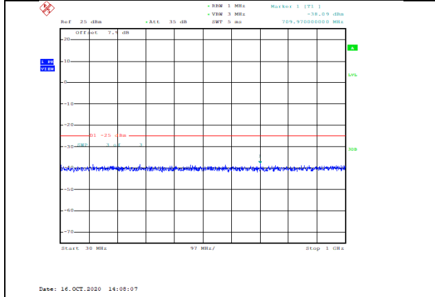
Band41-20MHz-QPSK-40140-1RB#0-Range1:30~1000MHz--38.09-PASS
