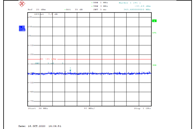
Band41-15MHz-QPSK-40590-1RB#0-Range1:30~1000MHz--37.69-PASS
