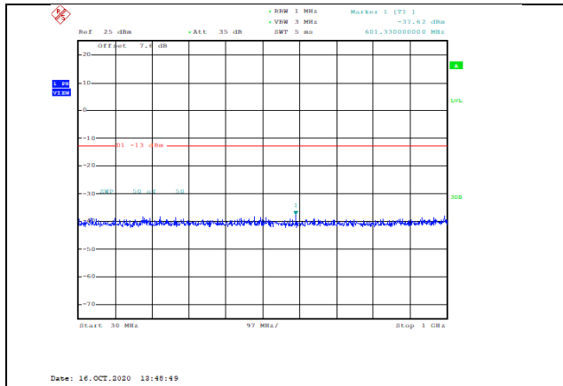
Band66-10MHz-QPSK-132622-1RB#0-Range1:30~1000MHz--37.62-PASS
