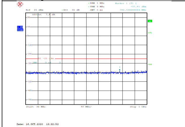
Band38-15MHz-16QAM-38000-1RB#0-Range1:30~1000MHz--37.91-PASS
