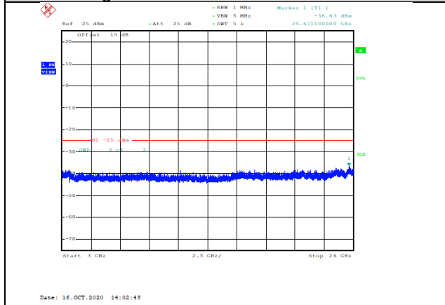
Band41-10MHz-16QAM-41190-1RB#0-Range3:3000~26000MHz--36.63-PASS
