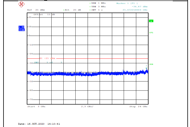
Band41-20MHz-16QAM-40590-1RB#0-Range3:3000~26000MHz--36.47-PASS
