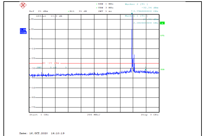
Band41-20MHz-16QAM-40590-1RB#0-Range2:1000~3000MHz--32.36-PASS
