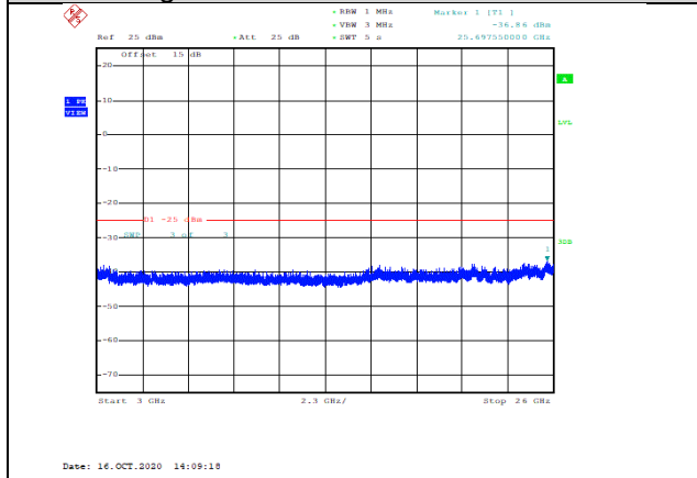
Band41-20MHz-16QAM-40140-1RB#0-Range3:3000~26000MHz--36.86-PASS
