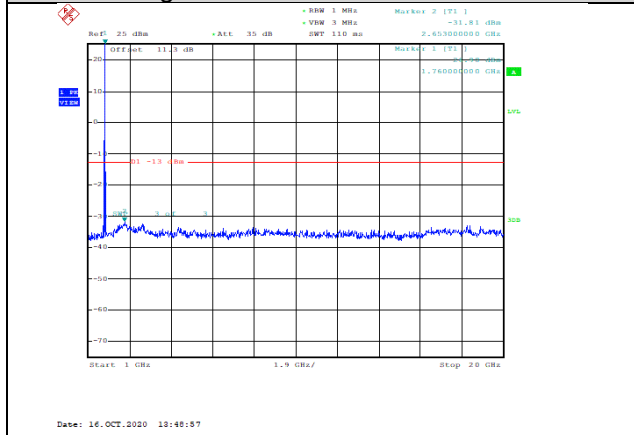
Band66-10MHz-QPSK-132622-1RB#0-Range2:1000~20000MHz--31.81-PASS
