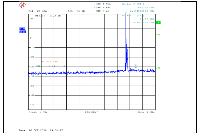
Band41-15MHz-QPSK-40115-1RB#0-Range2:1000~3000MHz--32.02-PASS
