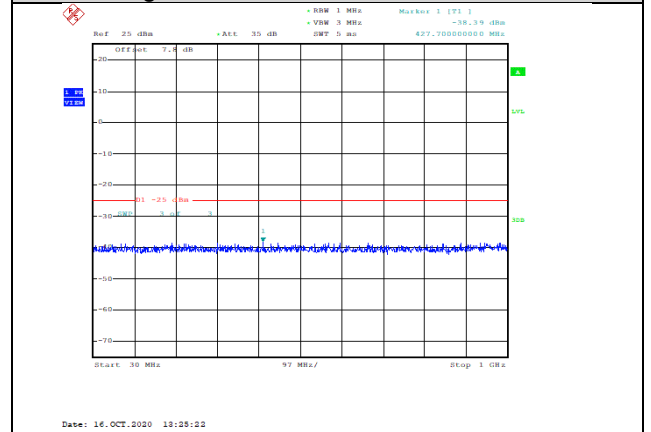
Band38-5MHz-16QAM-38225-1RB#0-Range1:30~1000MHz--38.39-PASS
