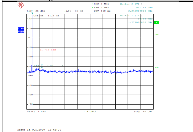
Band66-1.4MHz-16QAM-132665-1RB#0-Range2:1000~20000MHz--31.74-PASS
