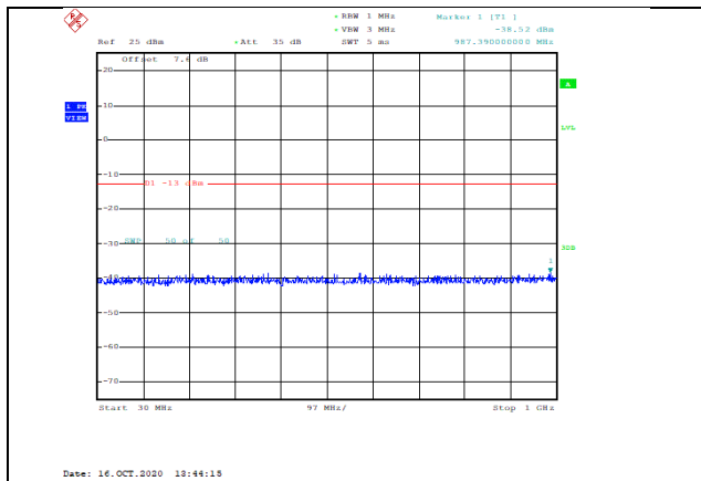
Band66-3MHz-16QAM-132657-1RB#0-Range1:30~1000MHz--38.52-PASS
