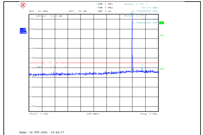
Band38-5MHz-16QAM-38000-1RB#0-Range2:1000~3000MHz--31.51-PASS
