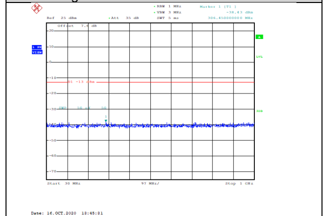
Band66-5MHz-QPSK-132322-1RB#0-Range1:30~1000MHz--38.43-PASS
