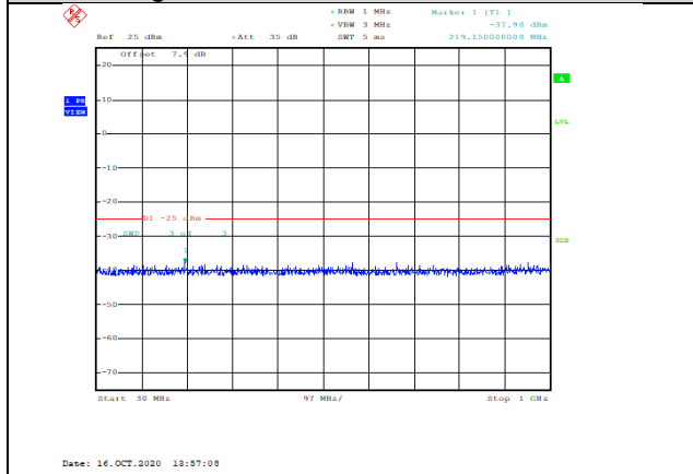
Band41-5MHz-QPSK-41215-1RB#0-Range1:30~1000MHz--37.9-PASS
