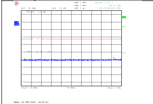
Band66-10MHz-QPSK-132022-1RB#0-Range1:30~1000MHz--38.54-PASS
