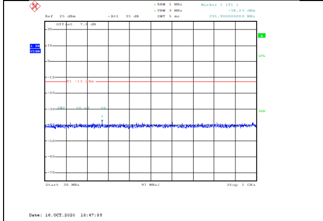
Band66-10MHz-16QAM-132022-1RB#0-Range1:30~1000MHz--38.23-PASS
