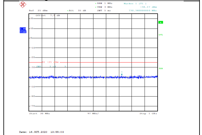
Band41-5MHz-16QAM-40065-1RB#0-Range1:30~1000MHz--38.37-PASS
