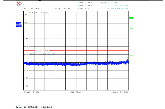
Band38-5MHz-16QAM-38000-1RB#0-Range3:3000~26000MHz--37.23-PASS
