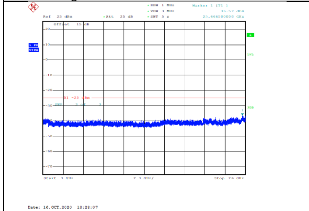
Band38-5MHz-16QAM-37775-1RB#0-Range3:3000~26000MHz--36.57-PASS
