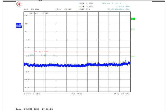
Band41-10MHz-16QAM-40590-1RB#0-Range3:3000~26000MHz--36.66-PASS
