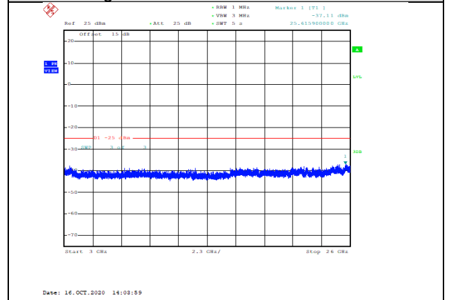
Band41-15MHz-QPSK-40115-1RB#0-Range3:3000~26000MHz--37.11-PASS
