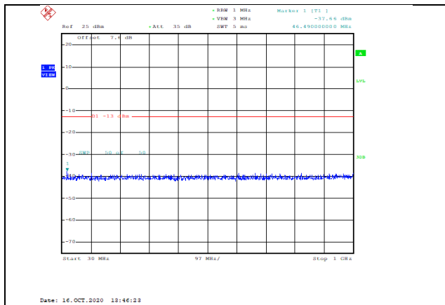
Band66-5MHz-QPSK-132647-1RB#0-Range1:30~1000MHz--37.66-PASS
