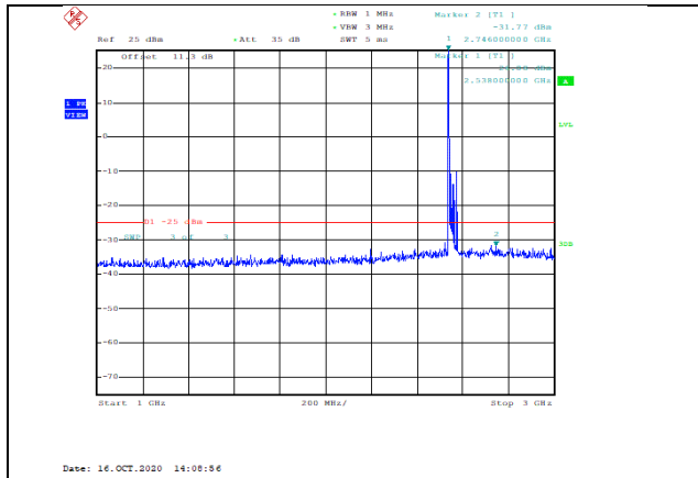
Band41-20MHz-16QAM-40140-1RB#0-Range2:1000~3000MHz--31.77-PASS
