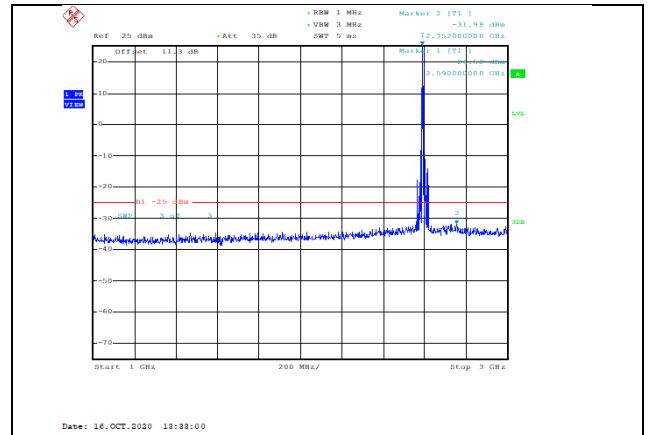
Band38-15MHz-16QAM-38000-1RB#0-Range2:1000~3000MHz--31.98-PASS
