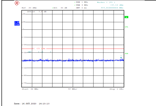
Band41-20MHz-16QAM-40590-1RB#0-Range1:30~1000MHz--37.52-PASS
