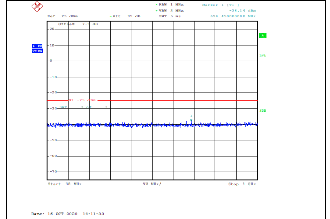
Band41-20MHz-16QAM-41140-1RB#0-Range1:30~1000MHz--38.14-PASS
