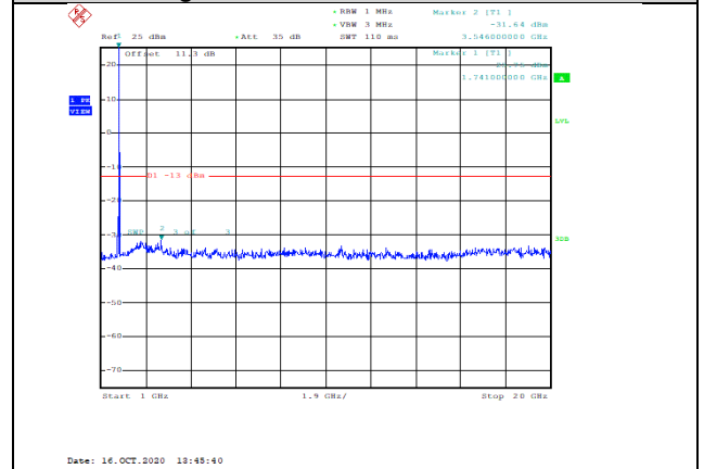
Band66-5MHz-QPSK-132322-1RB#0-Range2:1000~20000MHz--31.64-PASS
