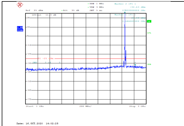
Band41-10MHz-16QAM-41190-1RB#0-Range2:1000~3000MHz--32.63-PASS
