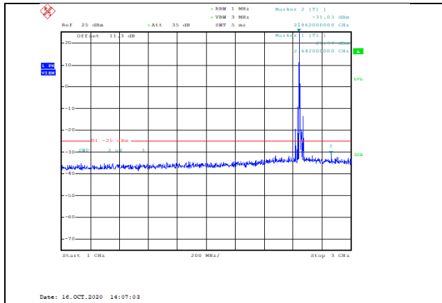
Band41-15MHz-16QAM-41165-1RB#0-Range2:1000~3000MHz--31.03-PASS
