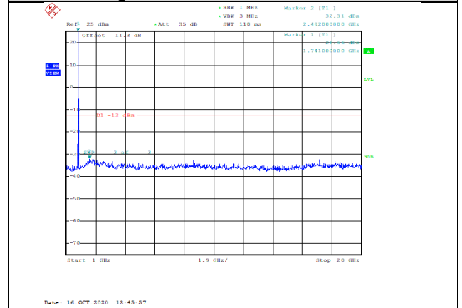
Band66-5MHz-16QAM-132322-1RB#0-Range2:1000~20000MHz--32.31-PASS
