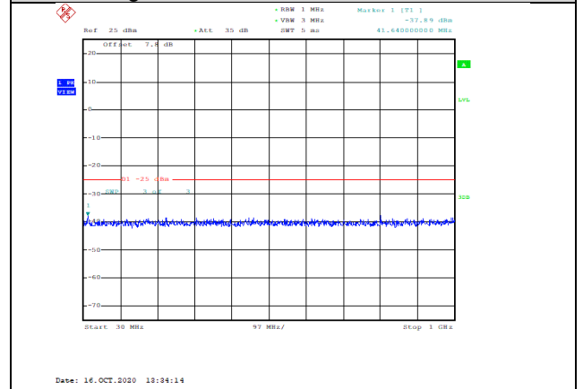
Band38-15MHz-16QAM-38175-1RB#0-Range1:30~1000MHz--37.89-PASS
