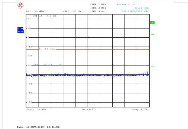
Band66-1.4MHz-16QAM-132665-1RB#0-Range1:30~1000MHz--38.38-PASS
