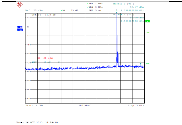
Band41-10MHz-16QAM-40090-1RB#0-Range2:1000~3000MHz--32.17-PASS
