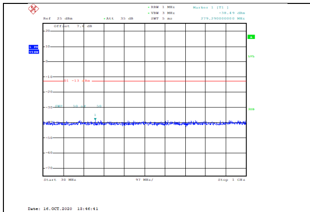
Band66-5MHz-16QAM-132647-1RB#0-Range1:30~1000MHz--38.49-PASS
