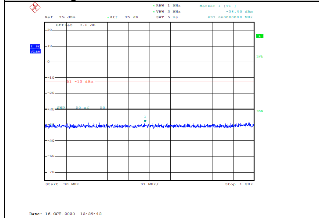
Band66-1.4MHz-16QAM-131979-1RB#0-Range1:30~1000MHz--38.4-PASS
