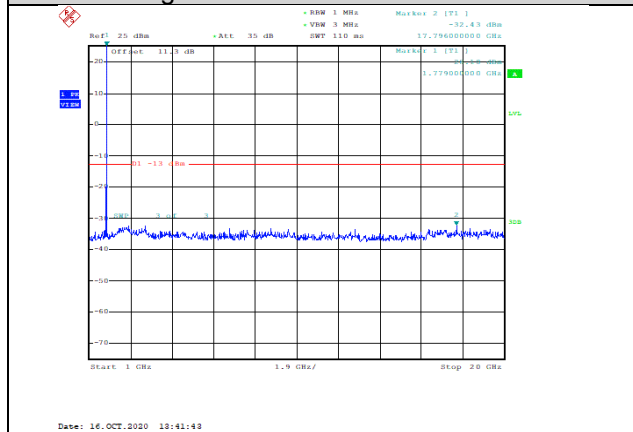
Band66-1.4MHz-QPSK-132665-1RB#0-Range2:1000~20000MHz--32.43-PASS
