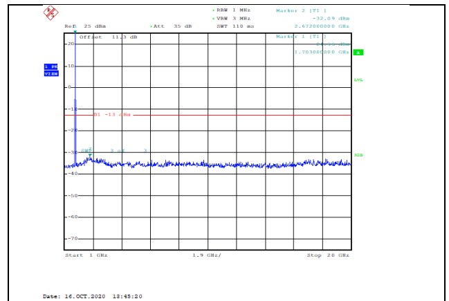
Band66-5MHz-16QAM-131997-1RB#0-Range2:1000~20000MHz--32.09-PASS
