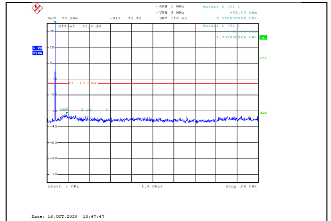
Band66-10MHz-16QAM-132022-1RB#0-Range2:1000~20000MHz--32.23-PASS
