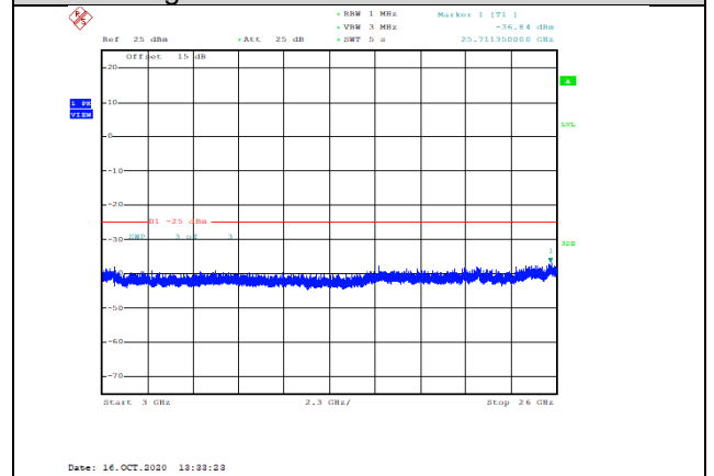
Band38-15MHz-16QAM-38000-1RB#0-Range3:3000~26000MHz--36.84-PASS
