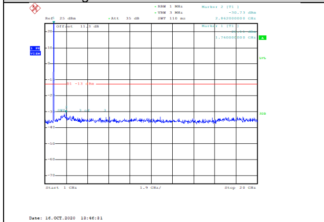
Band66-5MHz-QPSK-132647-1RB#0-Range2:1000~20000MHz--30.73-PASS
