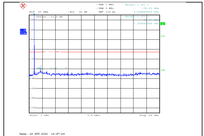
Band66-10MHz-QPSK-132022-1RB#0-Range2:1000~20000MHz--30.93-PASS
