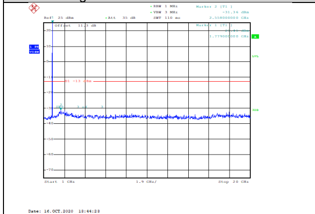
Band66-3MHz-16QAM-132657-1RB#0-Range2:1000~20000MHz--31.36-PASS
