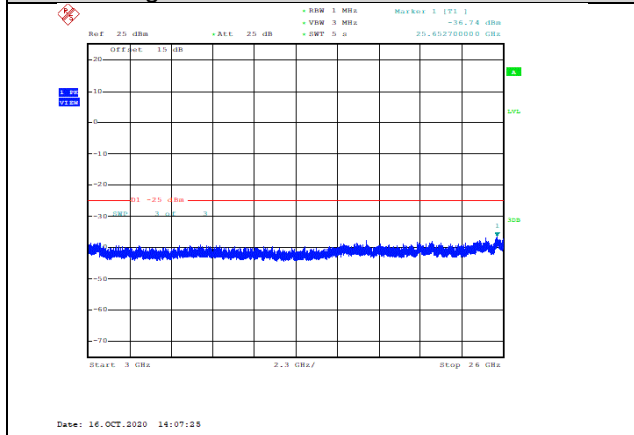
Band41-15MHz-16QAM-41165-1RB#0-Range3:3000~26000MHz--36.74-PASS
