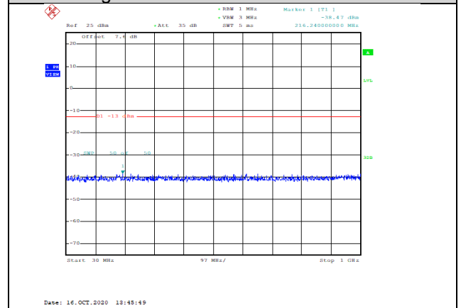
Band66-5MHz-16QAM-132322-1RB#0-Range1:30~1000MHz--38.47-PASS
