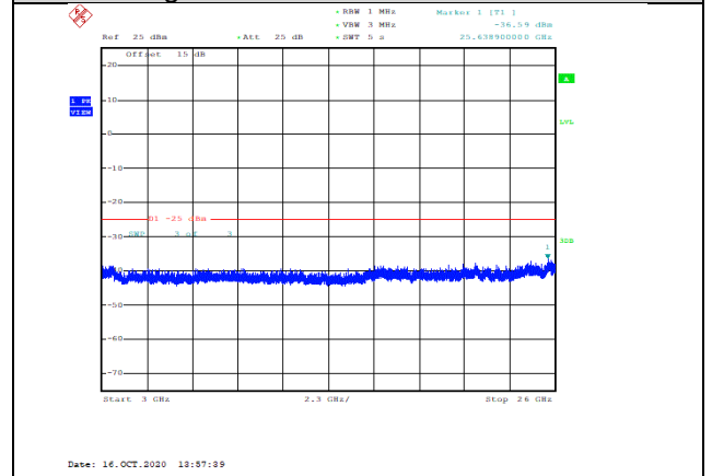
Band41-5MHz-QPSK-41215-1RB#0-Range3:3000~26000MHz--36.59-PASS
