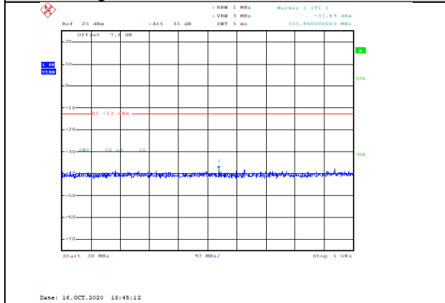
Band66-5MHz-16QAM-131997-1RB#0-Range1:30~1000MHz--37.89-PASS
