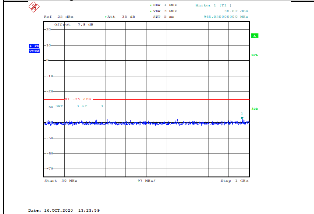
Band38-5MHz-16QAM-38000-1RB#0-Range1:30~1000MHz--38.02-PASS
