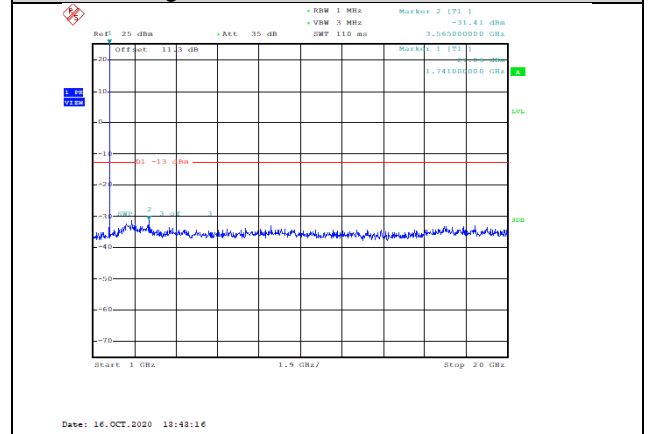
Band66-3MHz-QPSK-132322-1RB#0-Range2:1000~20000MHz--31.41-PASS
