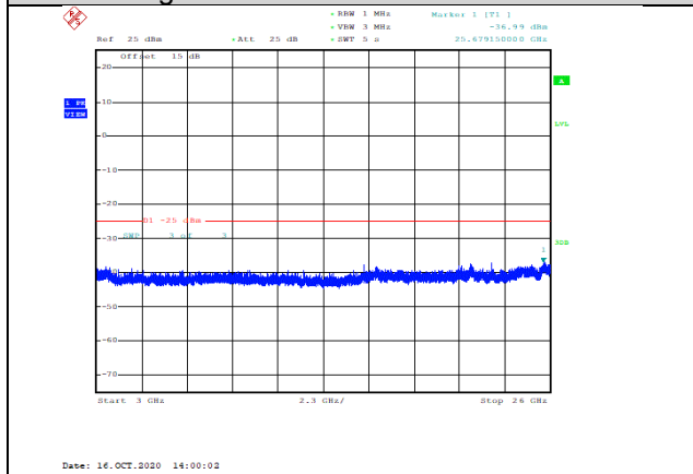
Band41-10MHz-16QAM-40090-1RB#0-Range3:3000~26000MHz--36.99-PASS
