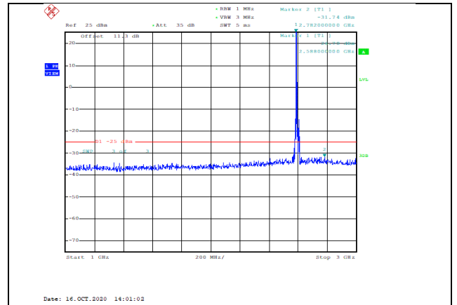
Band41-10MHz-16QAM-40590-1RB#0-Range2:1000~3000MHz--31.74-PASS
