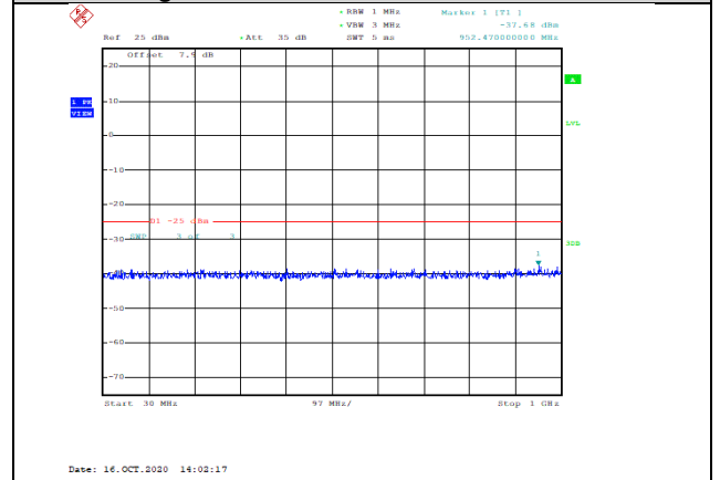
Band41-10MHz-16QAM-41190-1RB#0-Range1:30~1000MHz--37.68-PASS
