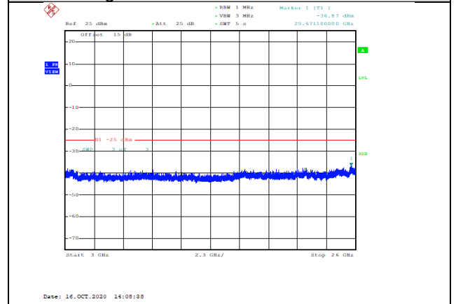
Band41-20MHz-QPSK-40140-1RB#0-Range3:3000~26000MHz--36.87-PASS
