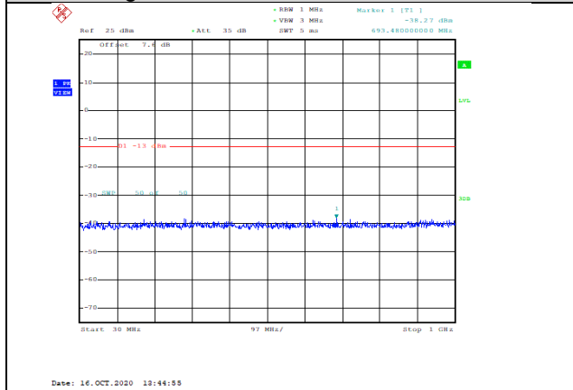
Band66-5MHz-QPSK-131997-1RB#0-Range1:30~1000MHz--38.27-PASS
