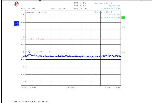
Band66-5MHz-16QAM-132647-1RB#0-Range2:1000~20000MHz--31.91-PASS
