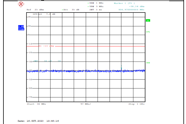
Band66-10MHz-16QAM-132322-1RB#0-Range1:30~1000MHz--38.34-PASS
