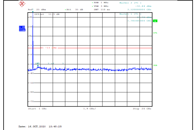
Band66-10MHz-16QAM-132322-1RB#0-Range2:1000~20000MHz--32.44-PASS
