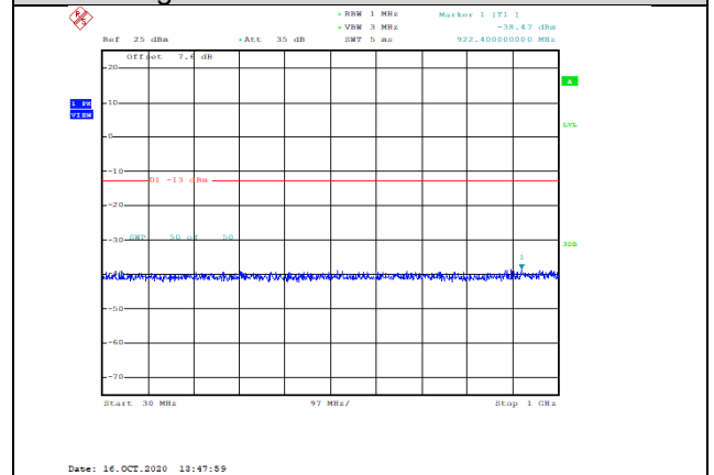
Band66-10MHz-QPSK-132322-1RB#0-Range1:30~1000MHz--38.47-PASS
