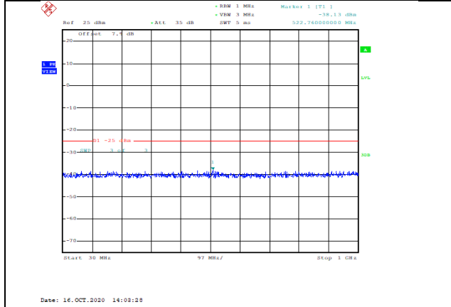
Band41-15MHz-QPSK-40115-1RB#0-Range1:30~1000MHz--38.13-PASS
