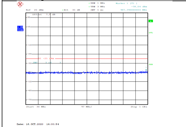
Band41-10MHz-16QAM-40590-1RB#0-Range1:30~1000MHz--38.06-PASS
