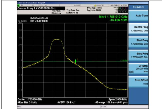
Band4-5MHz-16QAM-20375-1RB#24
