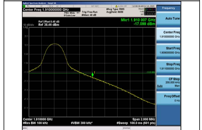
Band2-10MHz-QPSK-19150-1RB#49
