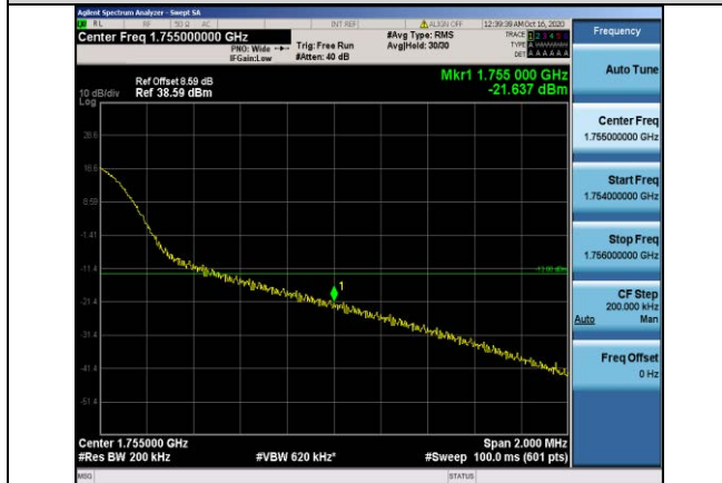
Band4-20MHz-16QAM-20300-1RB#99
