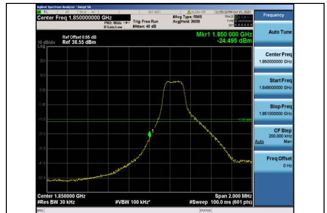
Band2-3MHz-16QAM-18615-1RB#0
