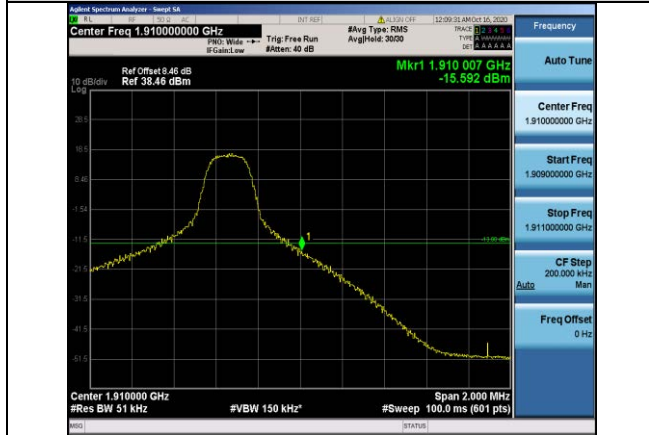
Band2-5MHz-16QAM-19175-1RB#24
