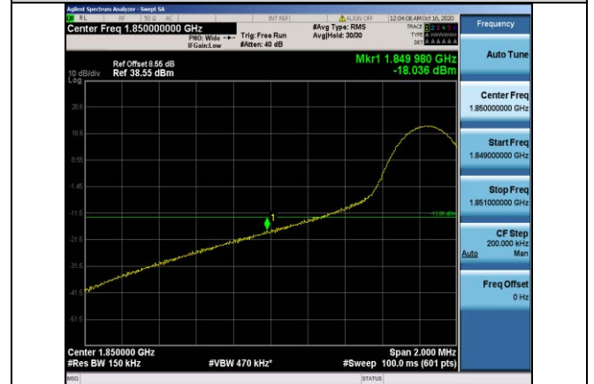
Band2-15MHz-QPSK-18675-1RB#0
