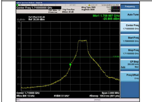
Band4-1.4MHz-16QAM-19957-1RB#0
