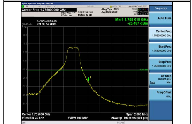
Band4-3MHz-16QAM-20385-1RB#14
