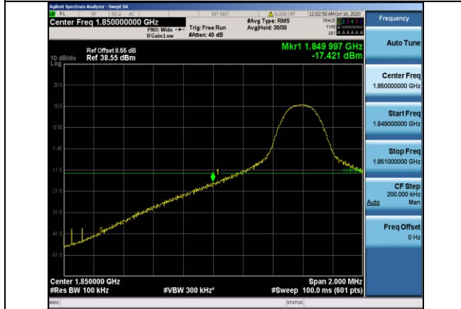
Band2-10MHz-16QAM-18650-1RB#0
