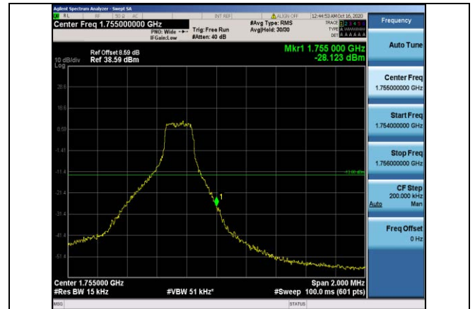
Band4-1.4MHz-16QAM-20393-1RB#5
