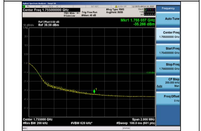
Band4-20MHz-QPSK-20300-100RB#0
