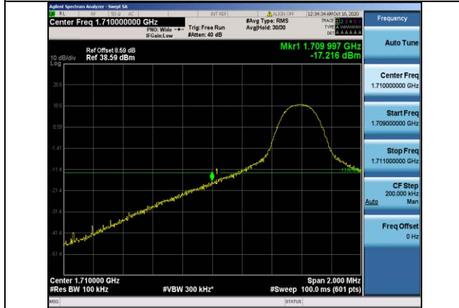
Band4-10MHz-16QAM-20000-1RB#0
