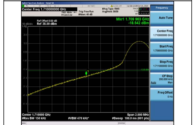
Band4-15MHz-QPSK-20025-1RB#0
