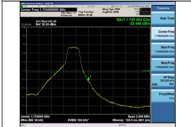
Band4-3MHz-QPSK-20385-1RB#14
