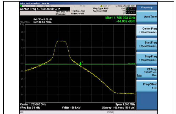
Band4-5MHz-QPSK-20375-1RB#24
