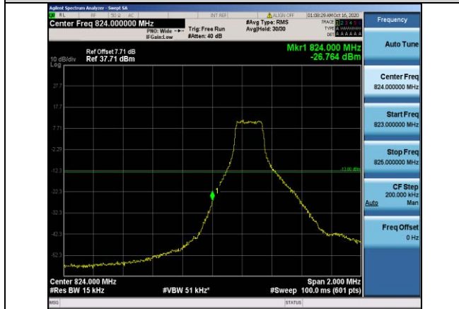
Band5-1.4MHz-16QAM-20407-1RB#0
