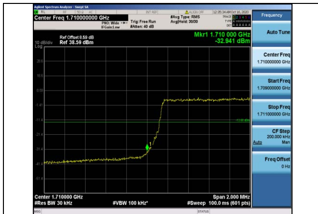
Band4-3MHz-QPSK-19965-15RB#0
