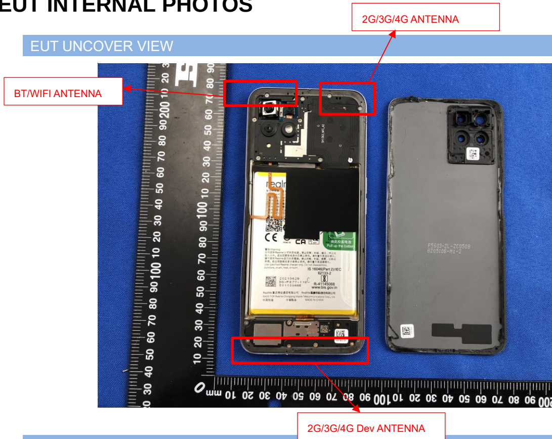
EUT UNCOVER VIEW
