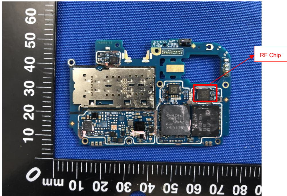
MAIN BOARD REAR VIEW (WITHOUT SHIELDING)
