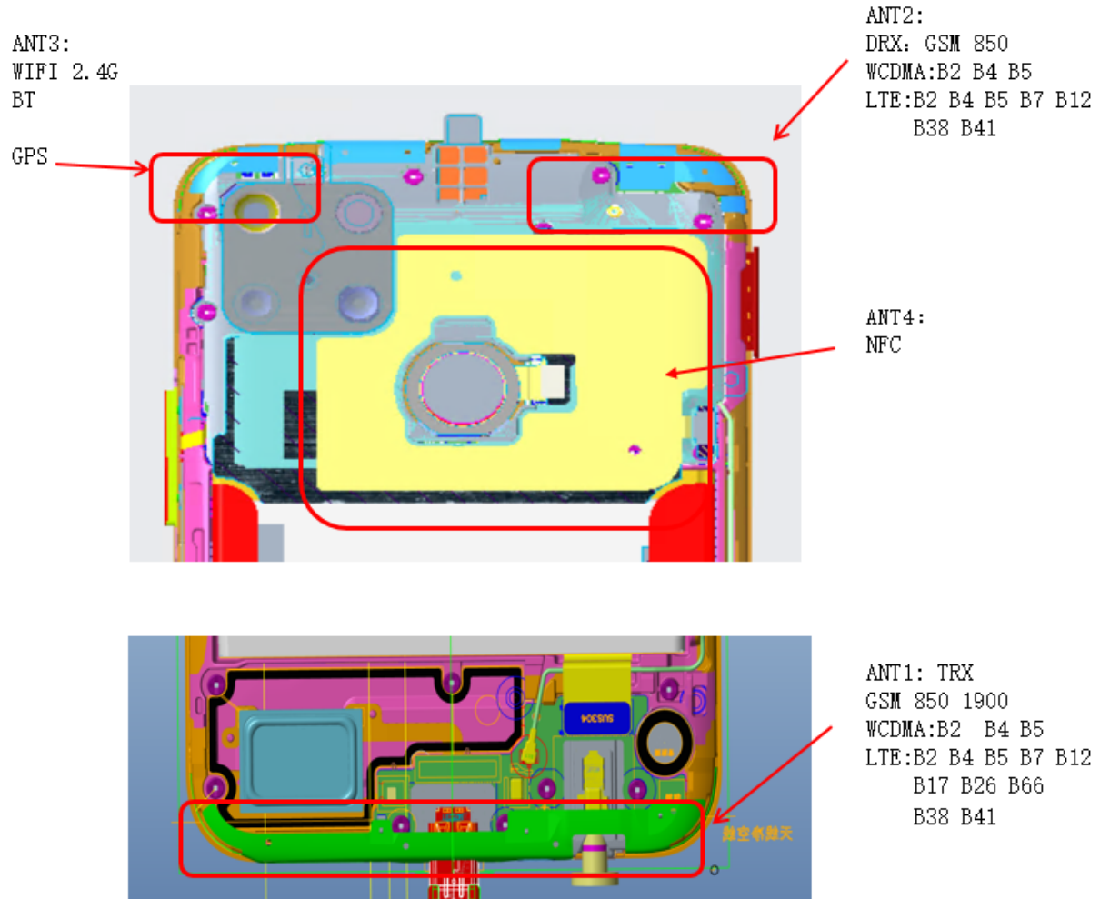
Figure: The location of the antennas
