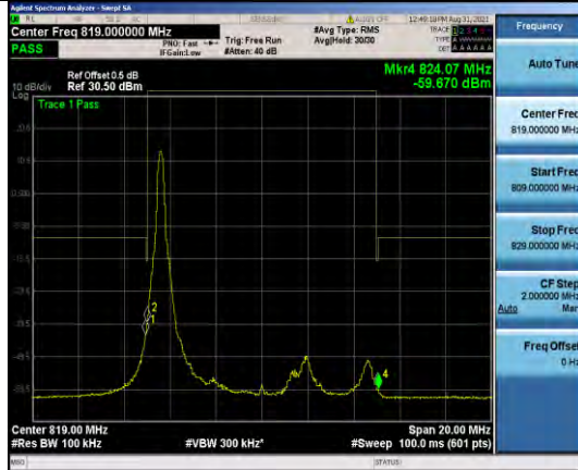
Band26-10MHz-QPSK-26740_Left-50RB#0
