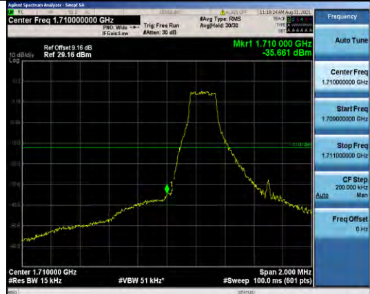
Band66-1.4MHz-QPSK-131979-6RB#0
