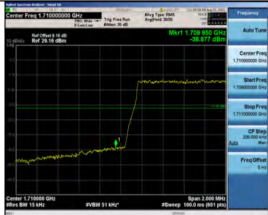
Band66-1.4MHz-QPSK-131979-6RB#0
