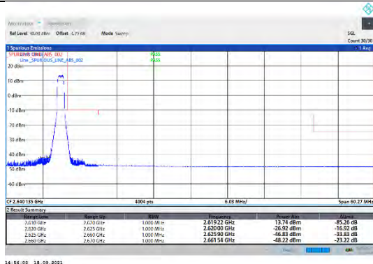
CA_38C-20MHz-20MHz-16QAM-16QAM-37952-38150-0RB#0-1RB#99
