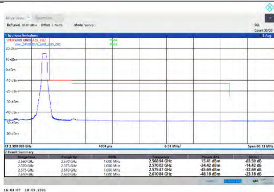
CA_7C-20MHz-20MHz-QPSK-QPSK-21152-21350-0RB#0-1RB#99
