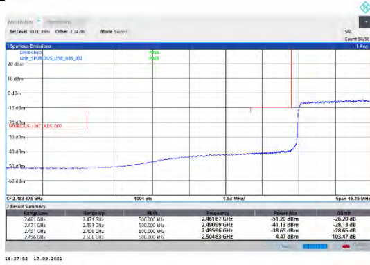
CA_41C-20MHz-5MHz-QPSK-QPSK-39750-39867-100RB#0-25RB#0
