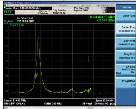
Band26-10MHz-16QAM-26740_Left-50RB#0
