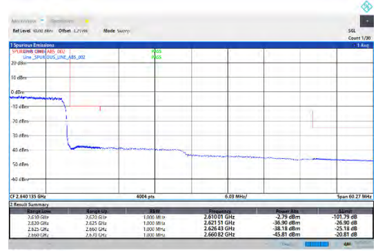
CA_38C-20MHz-20MHz-QPSK-QPSK-37952-38150-100RB#0-100RB#0
