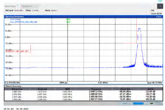
CA_41C-20MHz-20MHz-16QAM-16QAM-39750-39948-1RB#0-0RB#0
