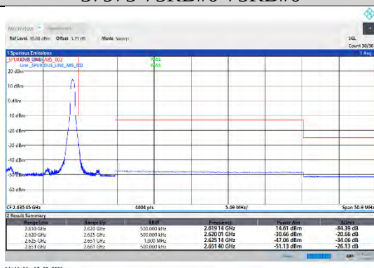
CA_38C-15MHz-15MHz-QPSK-QPSK-38025-38175-0RB#0-1RB#74
