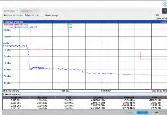
CA_41C-20MHz-20MHz-QPSK-QPSK-41292-41490-100RB#0-100RB#0
