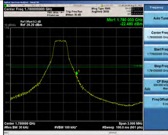
Band66-3MHz-16QAM-132657-15RB#0
