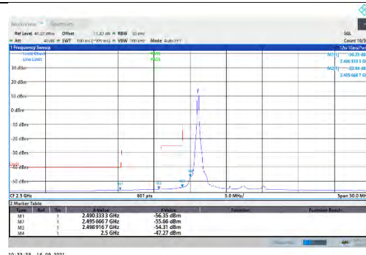
CA_7C-10MHz-20MHz-16QAM-16QAM-20805-20949-1RB#0-0RB#0
