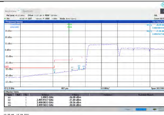
CA_7C-10MHz-20MHz-16QAM-16QAM-20805-20949-50RB#0-100RB#0
