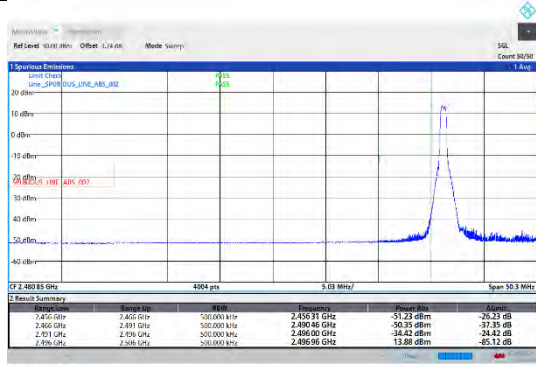
CA_41C-20MHz-10MHz-16QAM-16QAM-39750-39894-1RB#0-0RB#0
