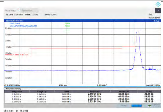
CA_7C-20MHz-20MHz-16QAM-16QAM-20850-21048-1RB#0-0RB#0
