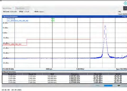
CA_38C-15MHz-15MHz-QPSK-QPSK-37825-37975-1RB#0-0RB#0
