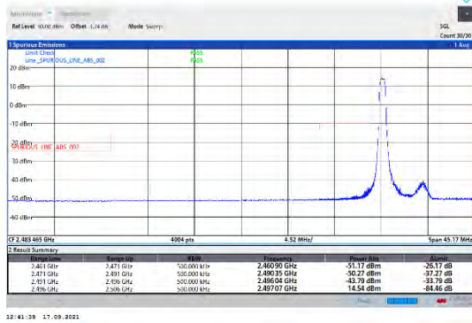
CA_41C-5MHz-20MHz-QPSK-QPSK-39683-39800-1RB#0-0RB#0
