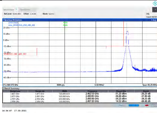
CA_41C-20MHz-5MHz-QPSK-QPSK-39750-39867-1RB#0-0RB#0
