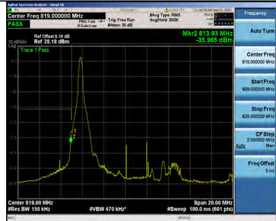
Band26-15MHz-16QAM-26765-75RB#0
