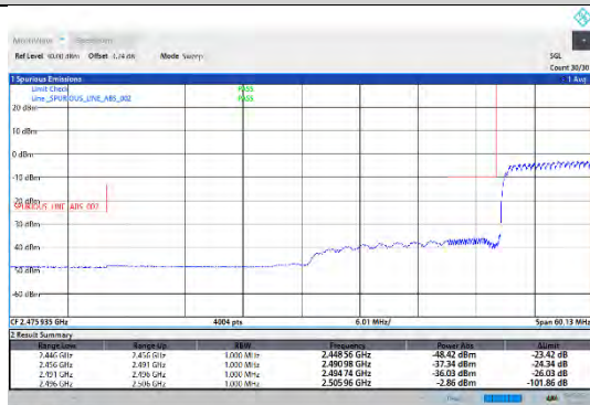
CA_41C-20MHz-20MHz-16QAM-16QAM-39750-39948-100RB#0-100RB#0
