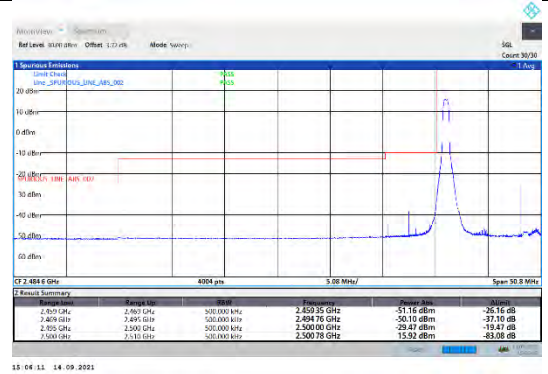
CA_7C-15MHz-15MHz-16QAM-16QAM-20825-20975-1RB#0-0RB#0
