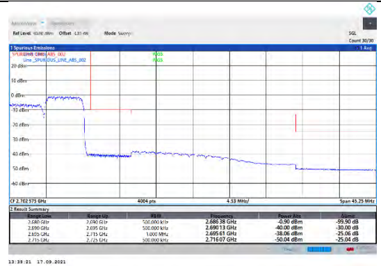
CA_41C-20MHz-5MHz-16QAM-16QAM-41440-41557-100RB#0-25RB#0
