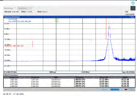
CA_41C-20MHz-5MHz-16QAM-16QAM-39750-39867-1RB#0-0RB#0
