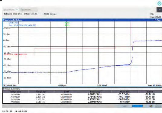
CA_7C-15MHz-15MHz-QPSK-QPSK-20825-20975-75RB#0-75RB#0
