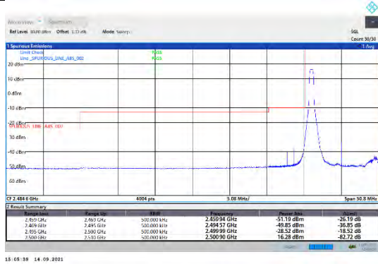
CA_7C-15MHz-15MHz-QPSK-QPSK-20825-20975-1RB#0-0RB#0
