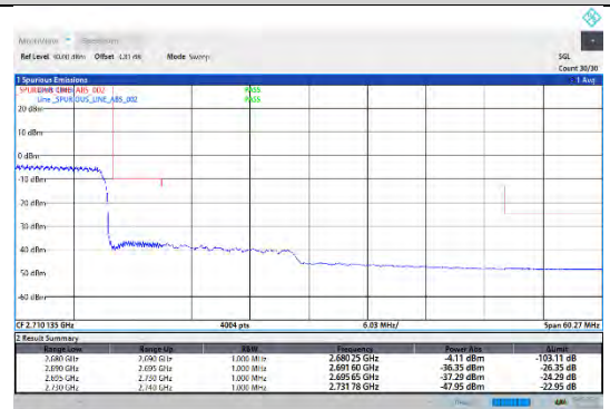
CA_41C-20MHz-20MHz-16QAM-16QAM-41292-41490-100RB#0-100RB#0
