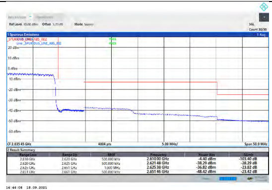
CA_38C-15MHz-15MHz-QPSK-QPSK-38025-38175-75RB#0-75RB#0
