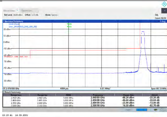
CA_7C-20MHz-20MHz-QPSK-QPSK-20850-21048-1RB#0-0RB#0
