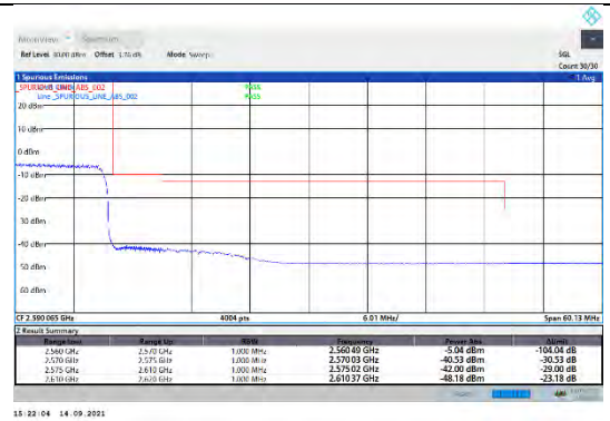
CA_7C-20MHz-20MHz-QPSK-QPSK-21152-21350-100RB#0-100RB#0
