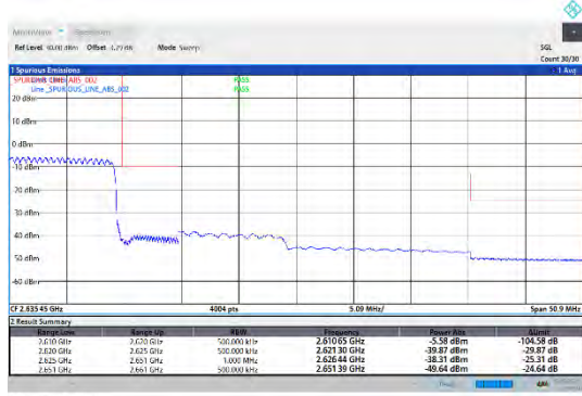
CA_38C-15MHz-15MHz-16QAM-16QAM-38025-38175-75RB#0-75RB#0
