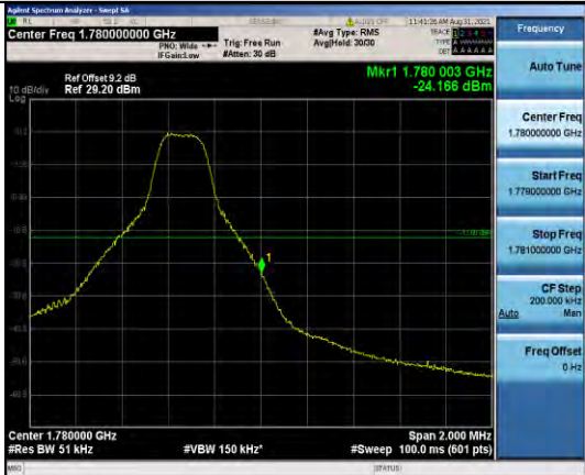
Band66-5MHz-QPSK-132647-25RB#0
