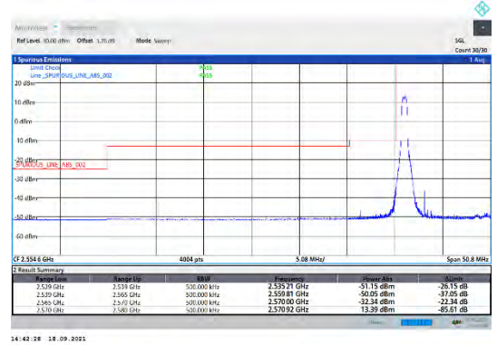
CA_38C-15MHz-15MHz-16QAM-16QAM-37825-37975-1RB#0-0RB#0
