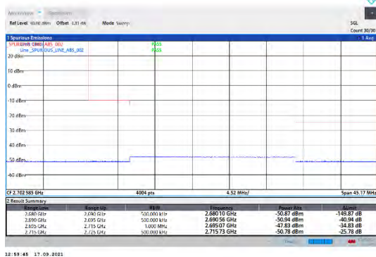
CA_41C-5MHz-20MHz-QPSK-QPSK-41373-41490-25RB#0-100RB#0
