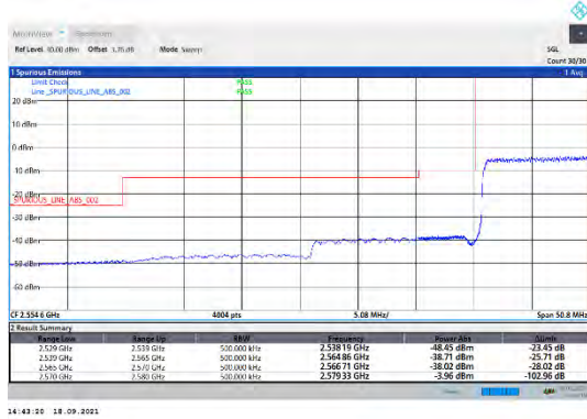
CA_38C-15MHz-15MHz-QPSK-QPSK-37825-37975-75RB#0-75RB#0
