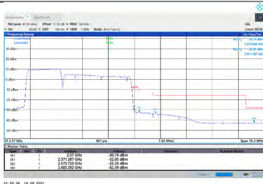
CA_7C-10MHz-20MHz-QPSK-QPSK-21206-21350-50RB#0-100RB#0
