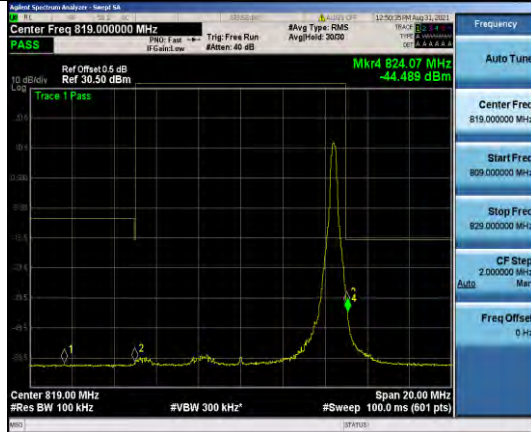
Band26-10MHz-16QAM-26740_Right-50RB#0
