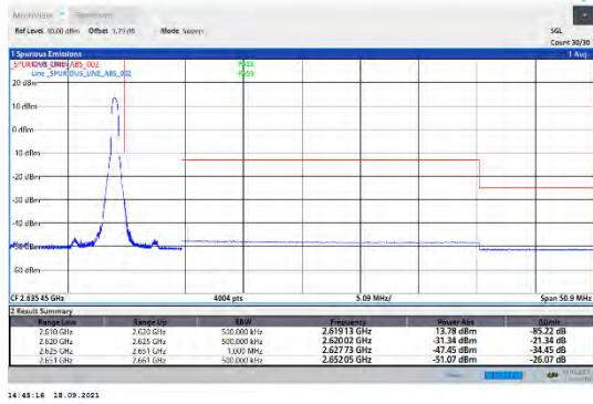
CA_38C-15MHz-15MHz-16QAM-16QAM-38025-38175-0RB#0-1RB#74
