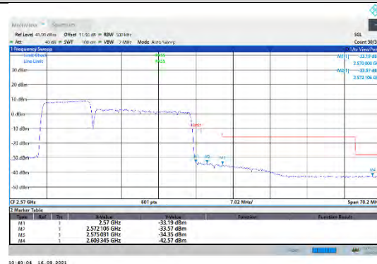
CA_7C-10MHz-20MHz-16QAM-16QAM-21206-21350-50RB#0-100RB#0
