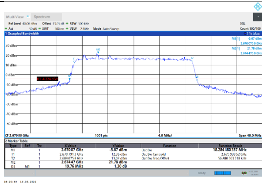
N41-30kHz-20MHz-CP-QPSK-High-Outer_Full---PASS
