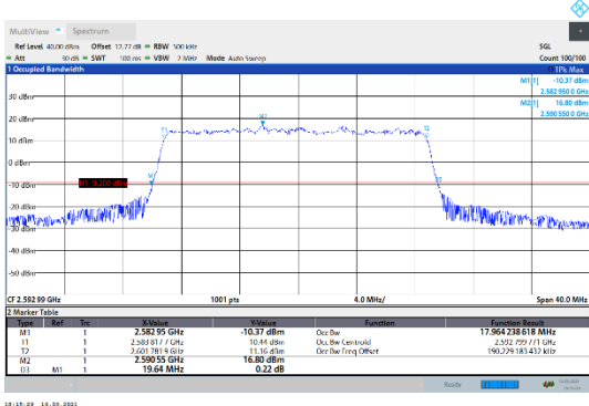
N41-30kHz-20MHz-DFT-256QAM-Mid-Outer_Full---PASS
