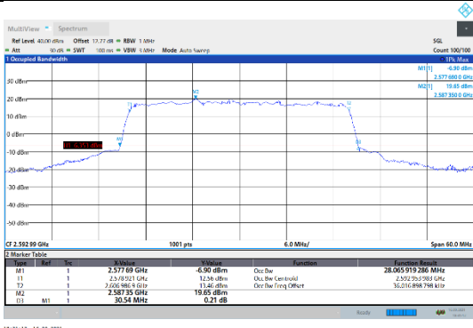
N41-30kHz-30MHz-CP-64QAM-Mid-Outer_Full---PASS
