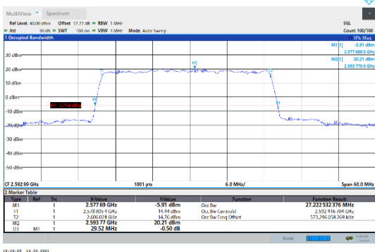
N41-30kHz-30MHz-DFT-64QAM-Mid-Outer_Full--- PASS
