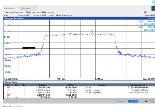
N41-30kHz-20MHz-DFT-256QAM-Low-Outer_Full---PASS
