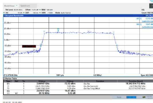
N41-30kHz-20MHz-CP-256QAM-High-Outer_Full---PASS
