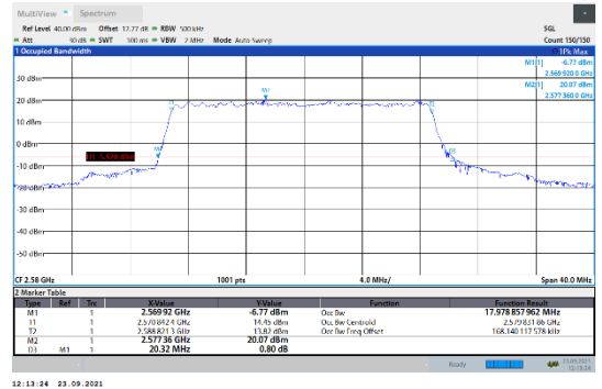
N38-30kHz-20MHz-DFT-QPSK-Low-Outer_Full--Ant1-PASS
