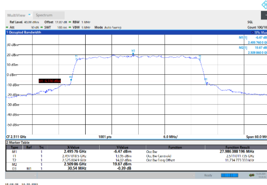
N41-30kHz-30MHz-CP-64QAM-Low-Outer_Full---PASS
