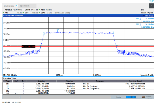
N41-30kHz-20MHz-CP-256QAM-Mid-Outer_Full---PASS
