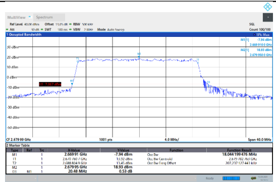
N41-30kHz-20MHz-DFT-16QAM-High-Outer_Full---PASS
