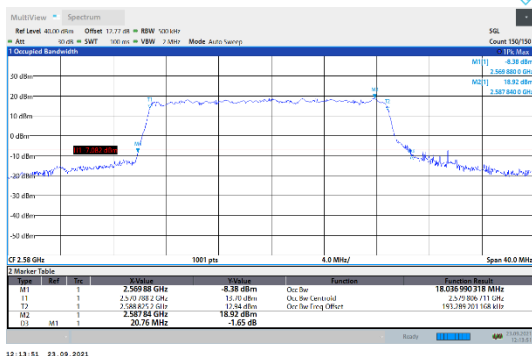
N38-30kHz-20MHz-DFT-16QAM-Low-Outer_Full-- Ant1-PASS
