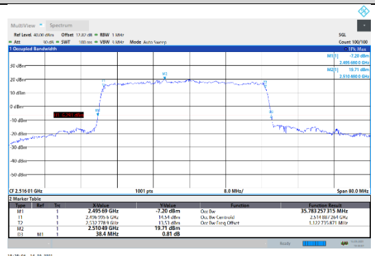
N41-30kHz-40MHz-DFT-16QAM-Low-Outer_Full---PASS
