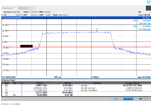
N41-30kHz-20MHz-CP-QPSK-Low-Outer_Full---PASS
