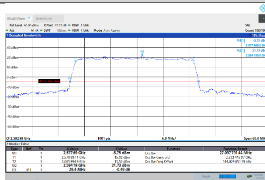
N41-30kHz-30MHz-DFT-16QAM-Mid-Outer_Full---PASS
