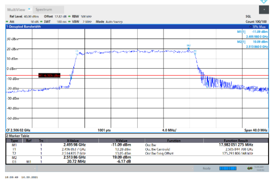
N41-30kHz-20MHz-DFT-16QAM-Low-Outer_Full---PASS
