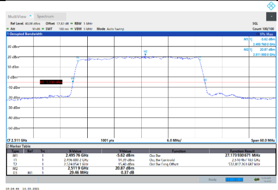
N41-30kHz-30MHz-DFT-64QAM-Low-Outer_Full--- PASS
