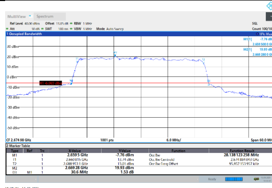
N41-30kHz-30MHz-CP-64QAM-High-Outer_Full---PASS
