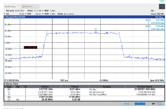
N41-30kHz-30MHz-DFT-256QAM-Mid-Outer_Full--- PASS
