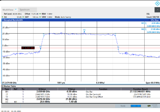
N41-30kHz-30MHz-DFT-16QAM-High-Outer_Full--- PASS
