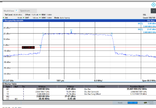
N41-30kHz-40MHz-DFT-QPSK-High-Outer_Full---PASS
