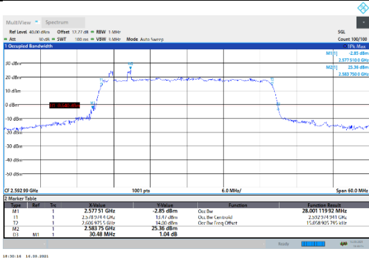
N41-30kHz-30MHz-CP-QPSK-Mid-Outer_Full---PASS
