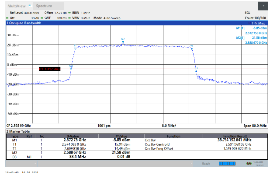
N41-30kHz-40MHz-DFT-QPSK-Mid-Outer_Full---PASS
