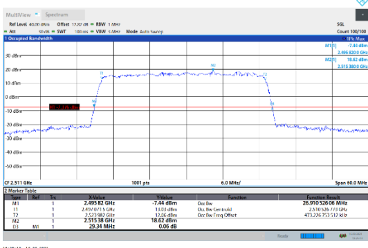
N41-30kHz-30MHz-DFT-256QAM-Low-Outer_Full--- PASS
