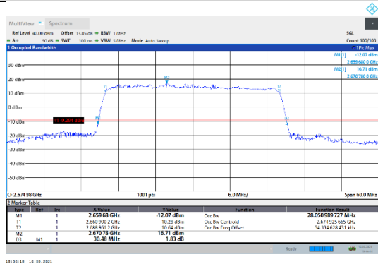
N41-30kHz-30MHz-CP-256QAM-High-Outer_Full---PASS
