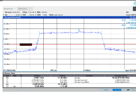
N41-30kHz-20MHz-CP-256QAM-Low-Outer_Full---PASS
