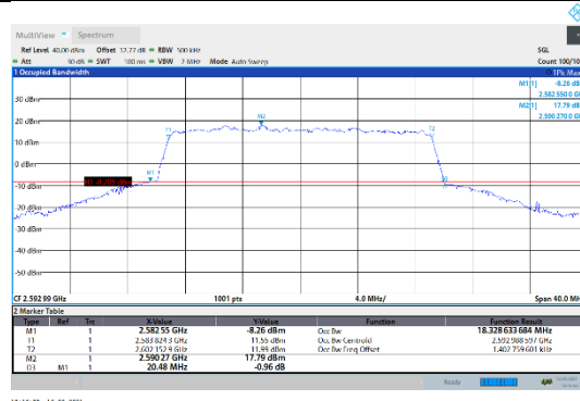
N41-30kHz-20MHz-CP-64QAM-Mid-Outer_Full---PASS
