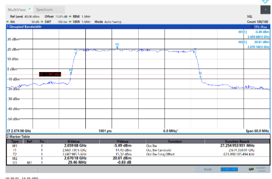
N41-30kHz-30MHz-DFT-64QAM-High-Outer_Full--- PASS
