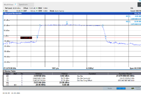
N41-30kHz-30MHz-DFT-QPSK-High-Outer_Full---PASS
