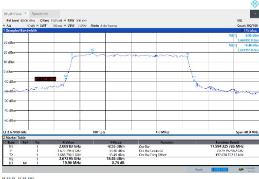
N41-30kHz-20MHz-DFT-64QAM-High-Outer_Full---PASS
