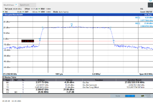
N41-30kHz-30MHz-DFT-QPSK-Mid-Outer_Full---PASS
