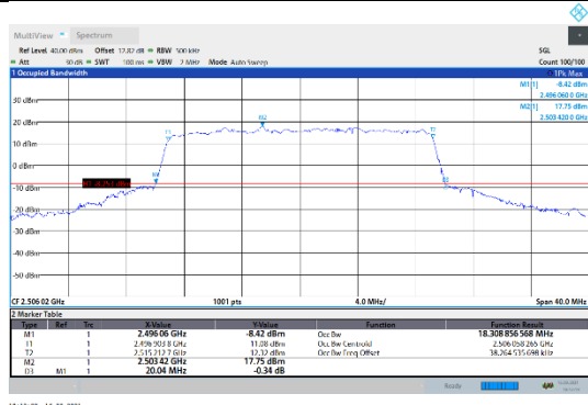
N41-30kHz-20MHz-CP-64QAM-Low-Outer_Full---PASS
