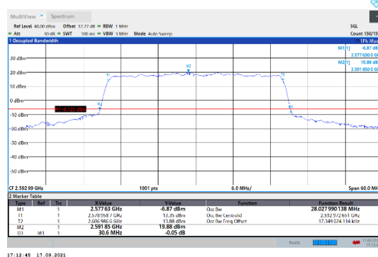
N41-30kHz-30MHz-CP-16QAM-Mid-Outer_Full---PASS
