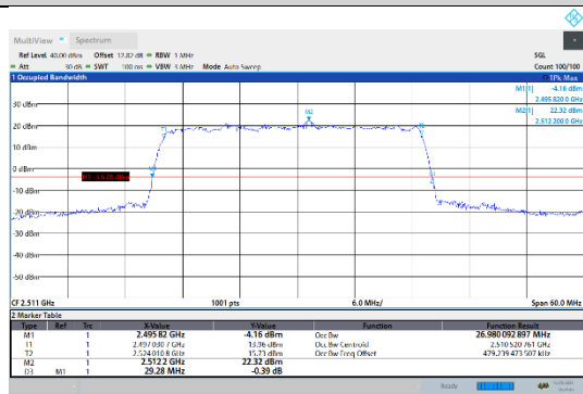
N41-30kHz-30MHz-DFT-16QAM-Low-Outer_Full---PASS
