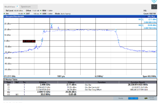
N41-30kHz-30MHz-CP-QPSK-Low-Outer_Full---PASS
