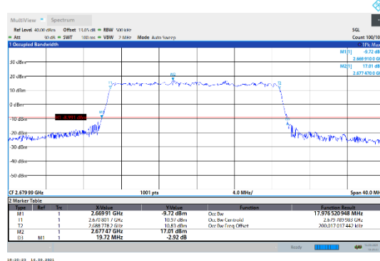
N41-30kHz-20MHz-DFT-256QAM-High-Outer_Full---PASS
