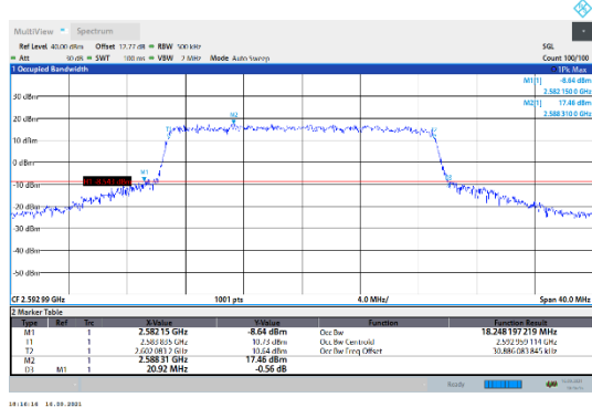
N41-30kHz-20MHz-CP-16QAM-Mid-Outer_Full---PASS
