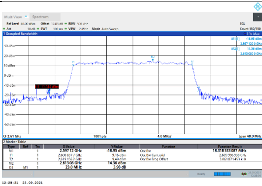
N38-30kHz-20MHz-CP-256QAM-High-Outer_Full--Ant1-PASS
