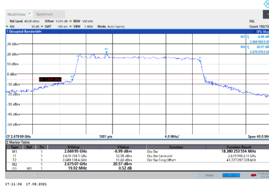
N41-30kHz-20MHz-CP-16QAM-High-Outer_Full---PASS
