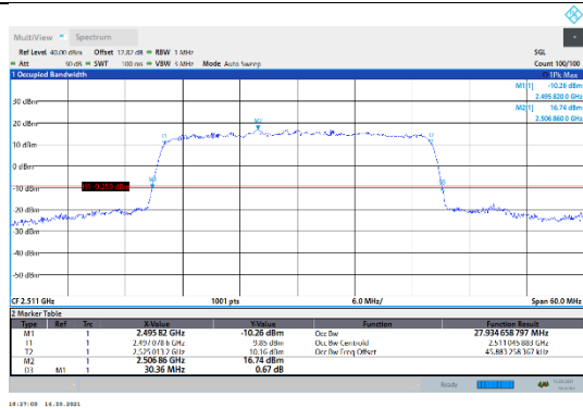
N41-30kHz-30MHz-CP-256QAM-Low-Outer_Full---PASS
