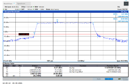
N38-30kHz-20MHz-DFT-QPSK-High-Outer_Full--Ant1-PASS
