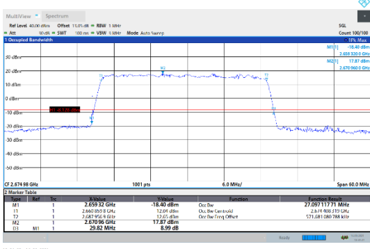
N41-30kHz-30MHz-DFT-256QAM-High-Outer_Full--- PASS
