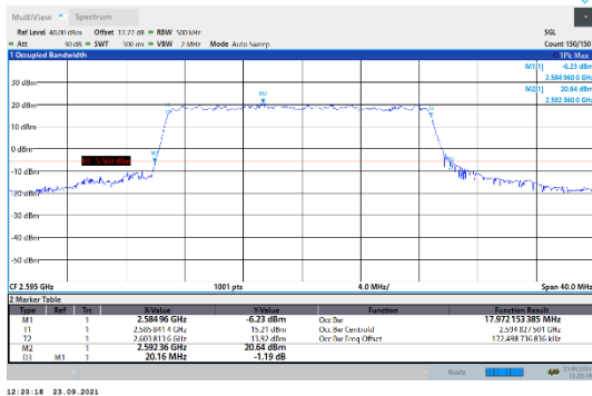
N38-30kHz-20MHz-DFT-QPSK-Mid-Outer_Full--Ant1- PASS
