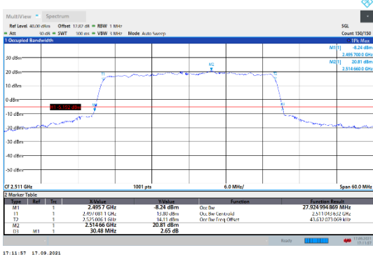
N41-30kHz-30MHz-CP-16QAM-Low-Outer_Full---PASS
