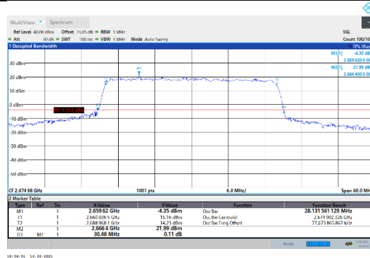
N41-30kHz-30MHz-CP-QPSK-High-Outer_Full---PASS
