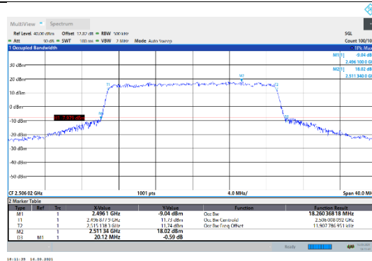
N41-30kHz-20MHz-CP-16QAM-Low-Outer_Full---PASS
