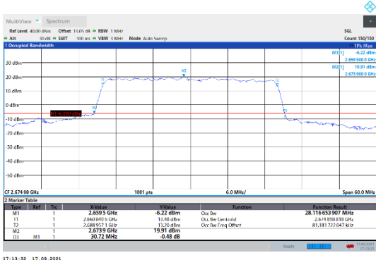
N41-30kHz-30MHz-CP-16QAM-High-Outer_Full---PASS
