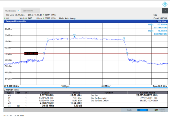
N41-30kHz-30MHz-CP-256QAM-Mid-Outer_Full---PASS
