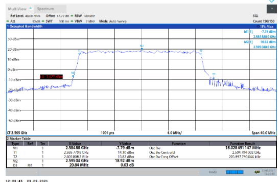
N38-30kHz-20MHz-DFT-16QAM-Mid-Outer_Full-- Ant1-PASS
