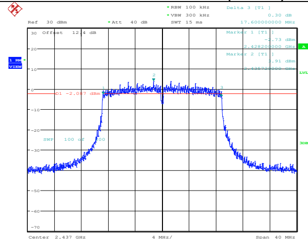
Channel 6, 802.11ac (VHT20)
