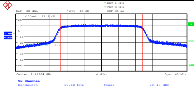
2412MHz, 802.11ax (HEW20),ANT 0
