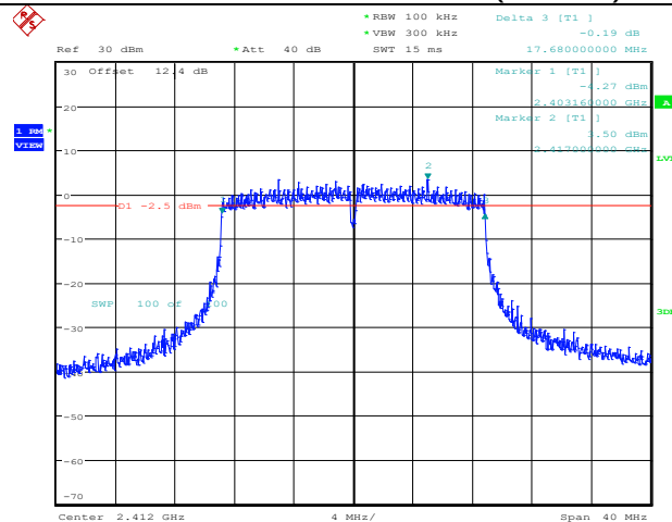
Channel 1, 802.11ac (VHT20)
