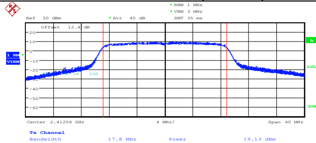
2412MHz, 802.11ax (HEW20),ANT 1
