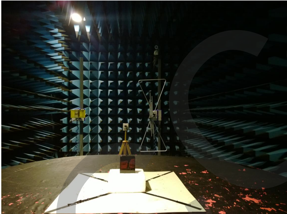
FCC Part15C Radiated Emission above 18-26GHz -Front
