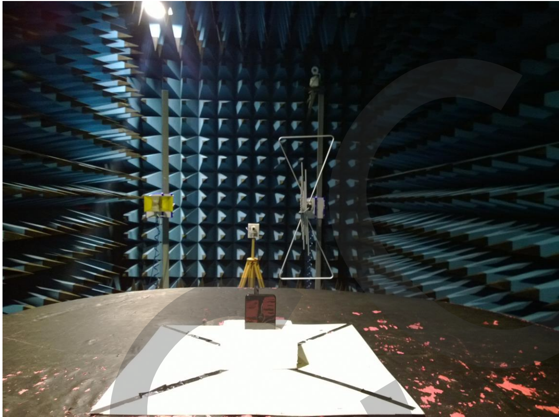
FCC Part15C Radiated Emission above 26-40GHz -Front
