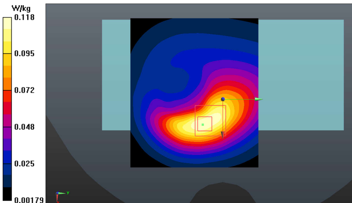
Fig.3 GSM 850 Body-worn
