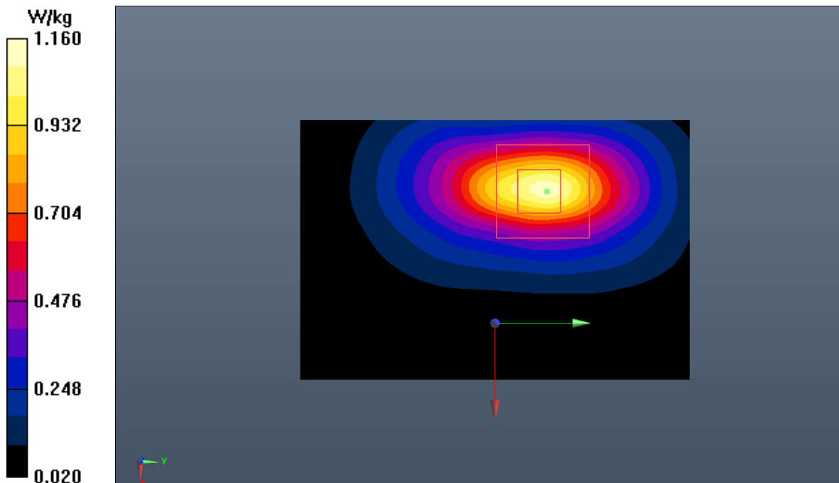
Fig.5 GSM 1900 Hotspot
