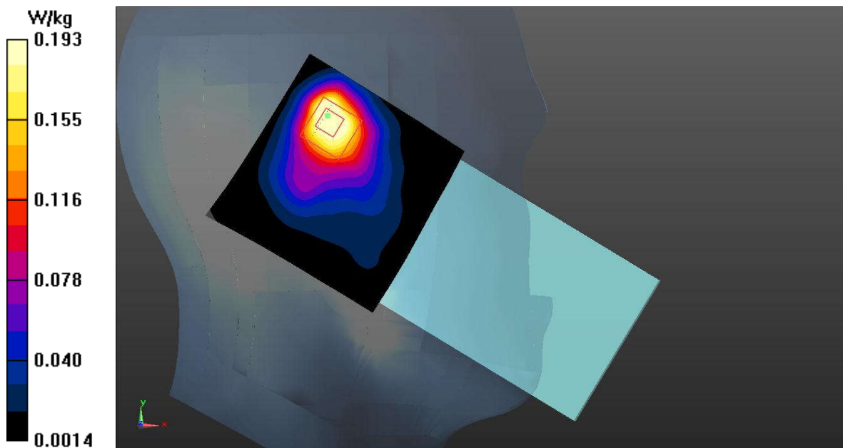
Fig.61 Bluetooth Head
