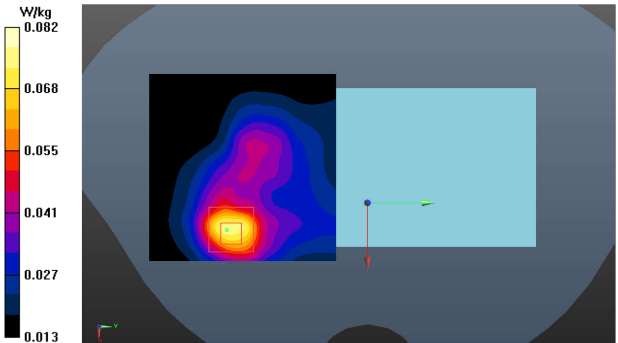
Fig.62 Bluetooth Hotspot
