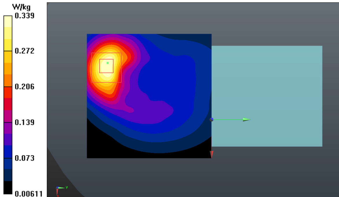
Fig.45 LTE Band 66 Body worn
