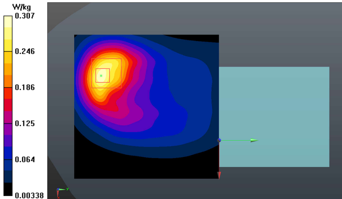
Fig.6 GSM 1900 Body-worn
