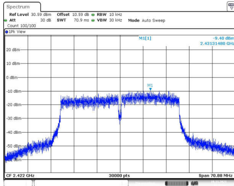
Fig.19 Power Spectral Density (802.11-VHT40, CH 3)
