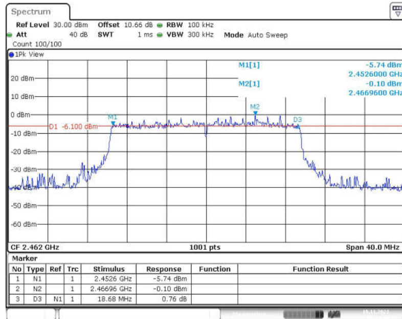
Fig.39 6dB Bandwidth (802.11ax-HE20, CH 11)
