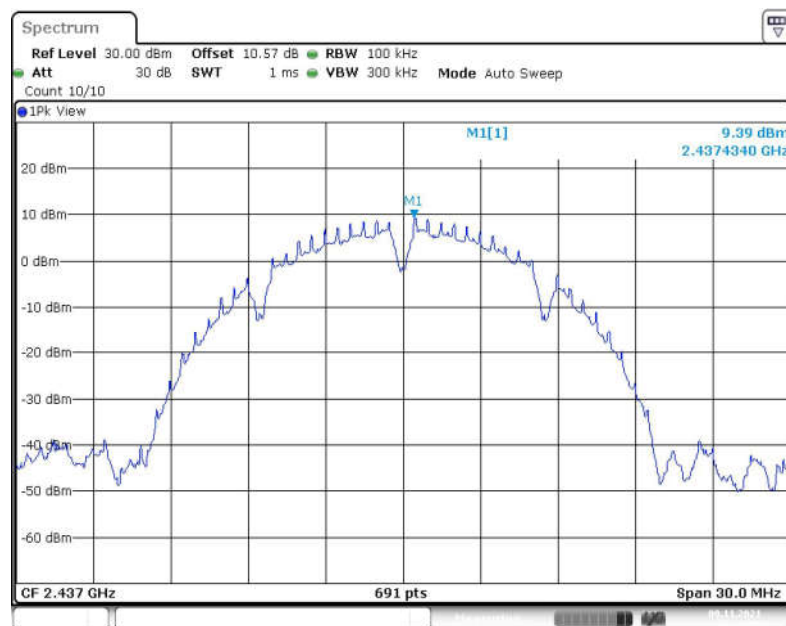
Fig.68 Conducted Spurious Emission (Center Frequency, 802.11b, CH6)
