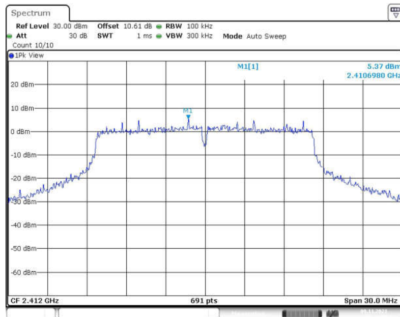
Fig.74 Conducted Spurious Emission (Center Frequency, 802.11g, CH1)
