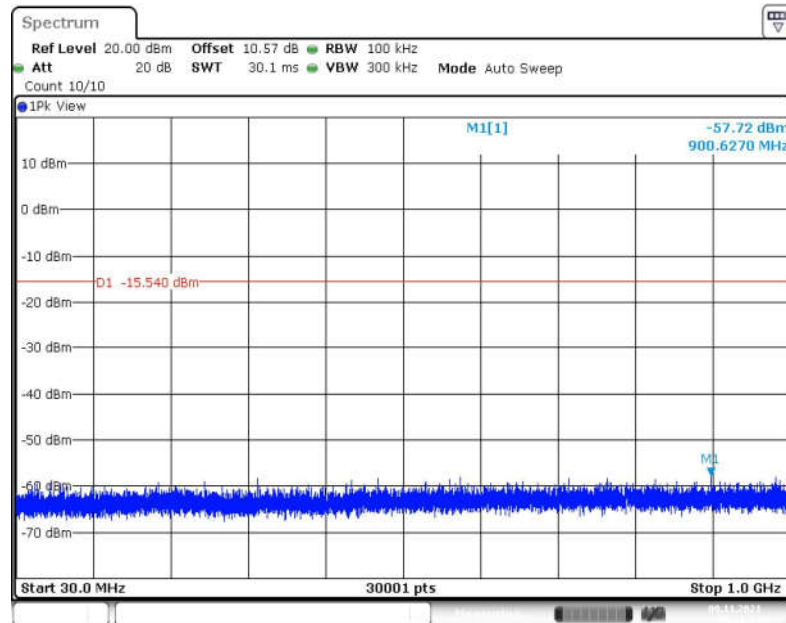
Fig.87 Conducted Spurious Emission (30MHz -1GHz, 802.11n-HT20, CH6)
