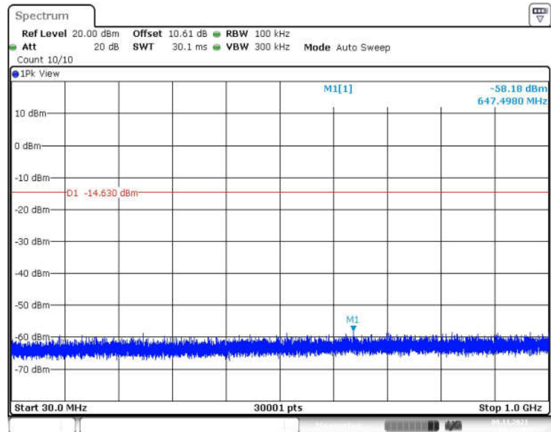
Fig.75 Conducted Spurious Emission (30MHz -1GHz, 802.11g, CH1)
