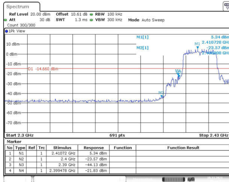
Fig.57 Band Edges (802.11ax-HE20, CH 1)
