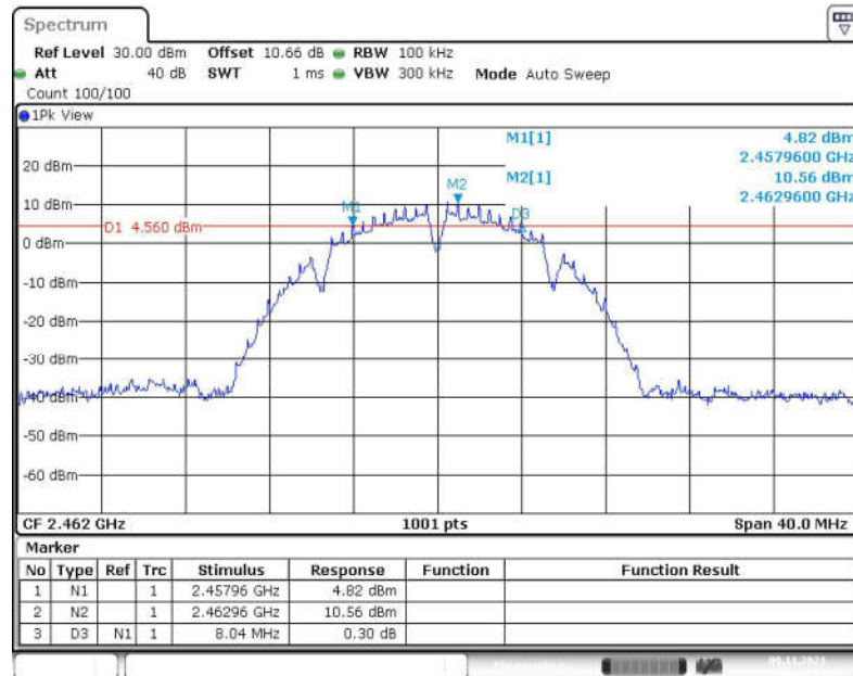
Fig.27 6dB Bandwidth (802.11b, CH 11)
