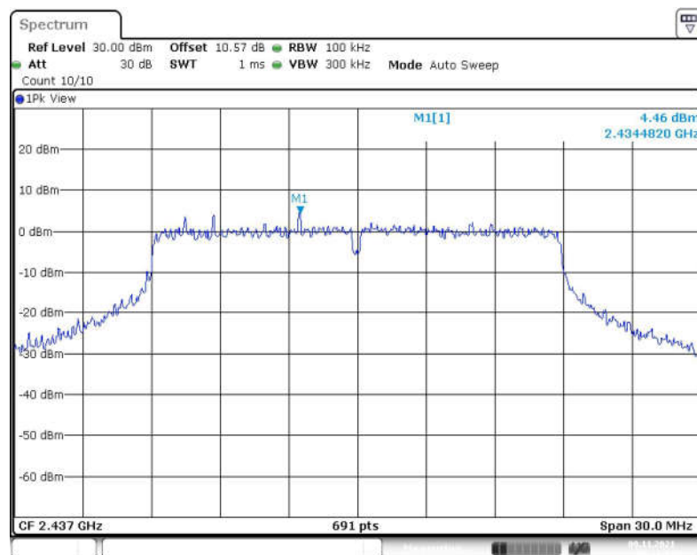
Fig.86 Conducted Spurious Emission (Center Frequency, 802.11n-HT20, CH6)
