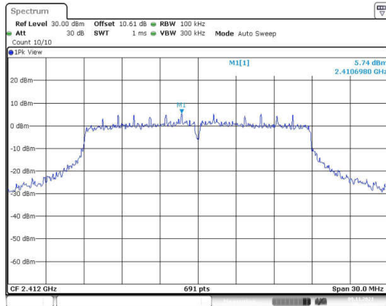
Fig.83 Conducted Spurious Emission (Center Frequency, 802.11n-HT20, CH1)
