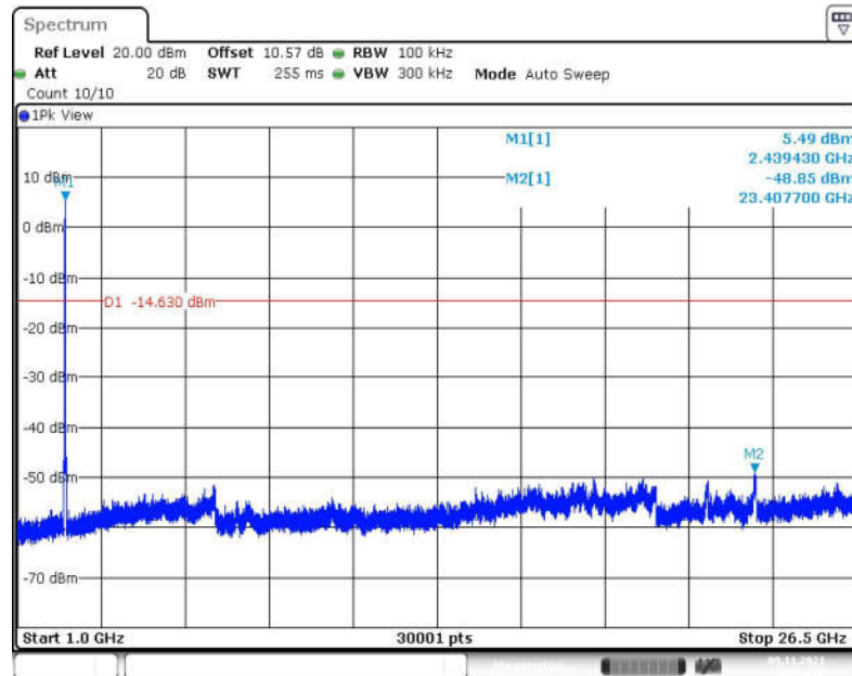
Fig.79 Conducted Spurious Emission (1GHz-26.5GHz, 802.11g, CH6)
