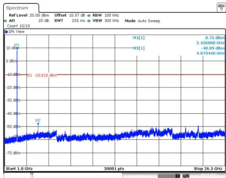
Fig.70 Conducted Spurious Emission (1GHz-26.5GHz, 802.11b, CH6)
