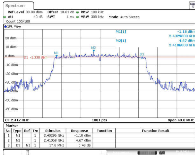
Fig.37 6dB Bandwidth (802.11ax-HE20, CH 1)
