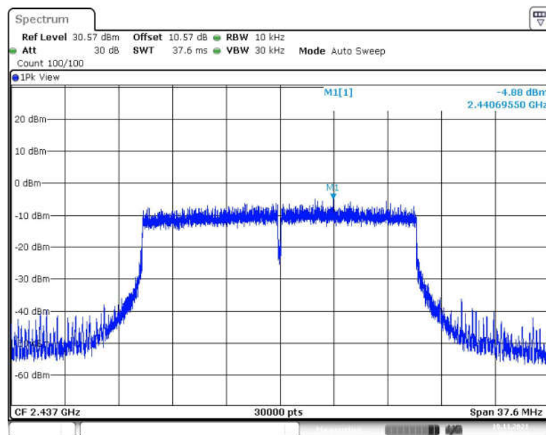
Fig.14 Power Spectral Density (802.11ax-HE20, CH 6)
