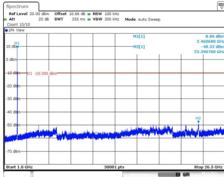
Fig.73 Conducted Spurious Emission (1GHz-26.5GHz, 802.11b, CH11)
