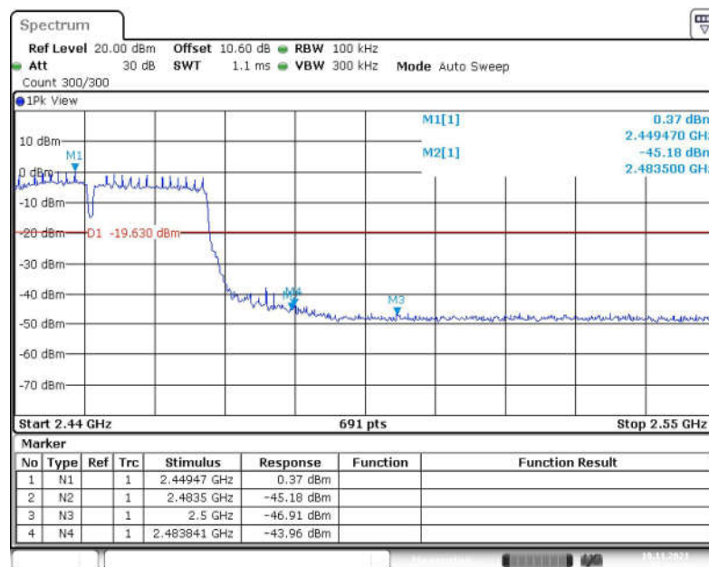
Fig.62 Band Edges (802.11-VHT40, CH 9)
