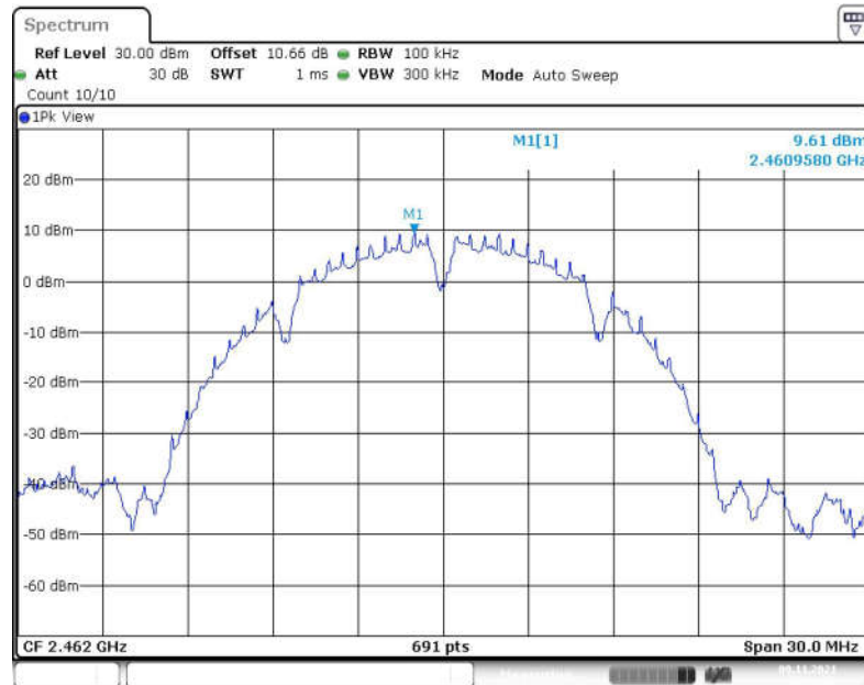
Fig.71 Conducted Spurious Emission (Center Frequency, 802.11b, CH11)
