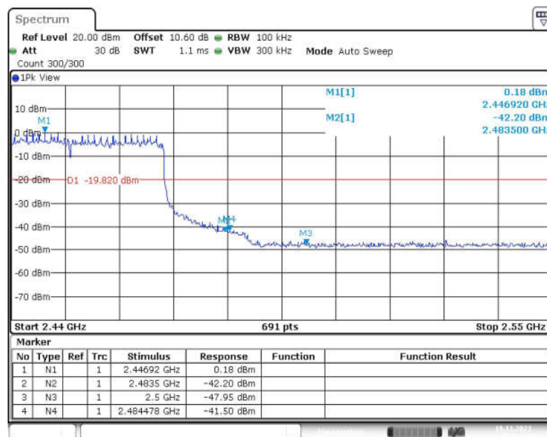
Fig.64 Band Edges (802.11ax-HE40, CH 9)
