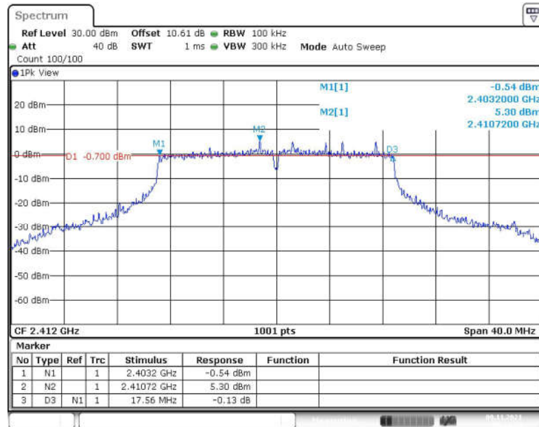
Fig.31 6dB Bandwidth (802.11n-HT20, CH 1)
