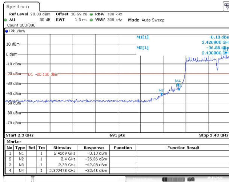
Fig.61 Band Edges (802.11-VHT40, CH 3)
