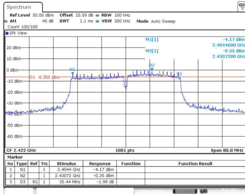
Fig.43 6dB Bandwidth (802.11-VHT40, CH 3)
