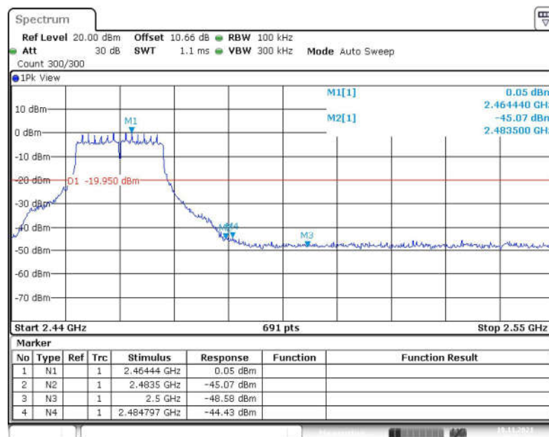
Fig.56 Band Edges (802.11-VHT20, CH 11)
