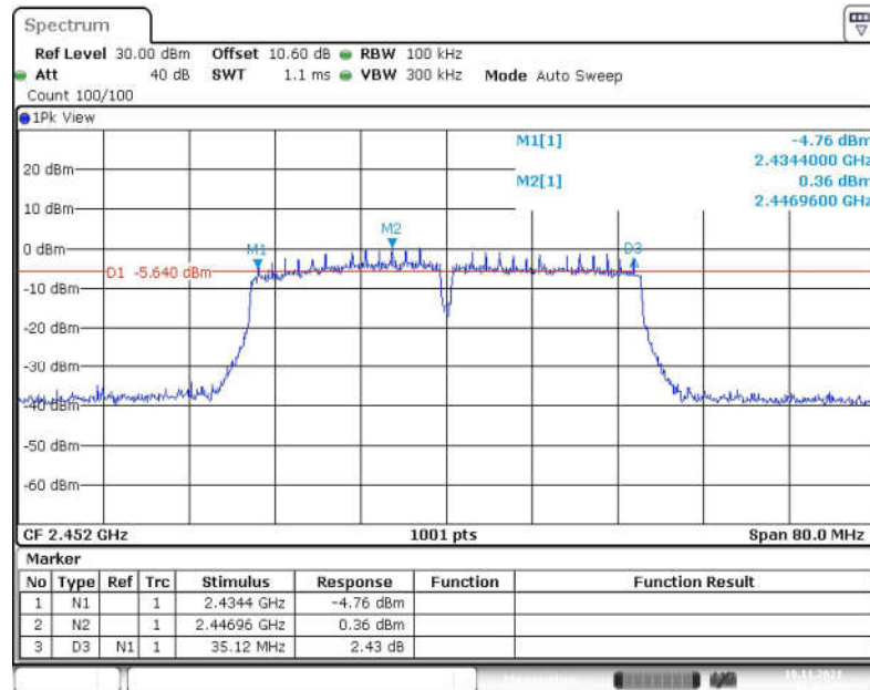
Fig.45 6dB Bandwidth (802.11-VHT40, CH 9)
