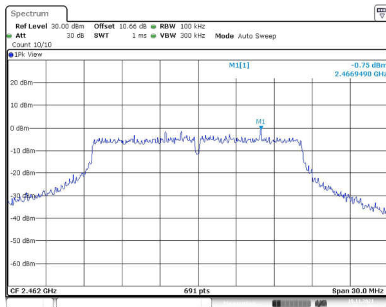
Fig.80 Conducted Spurious Emission (Center Frequency, 802.11g, CH11)
