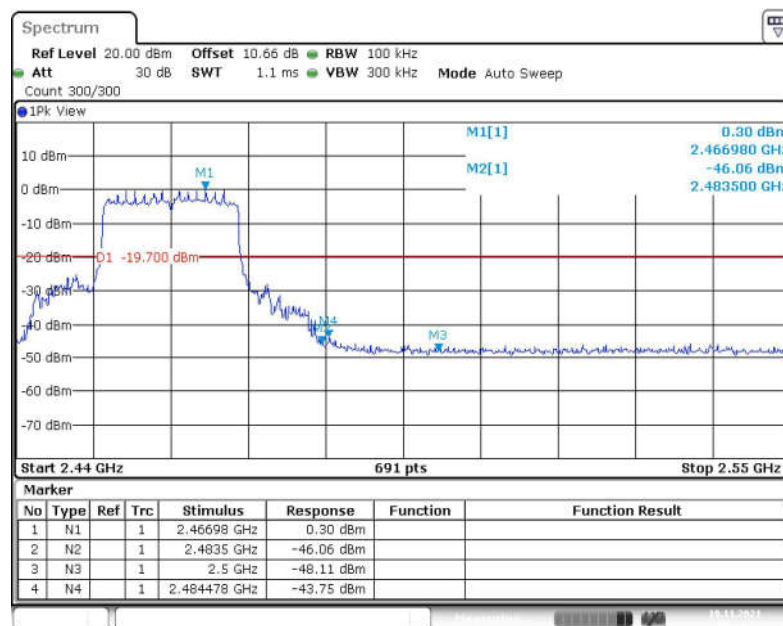
Fig.58 Band Edges (802.11ax-HE20, CH 11)
