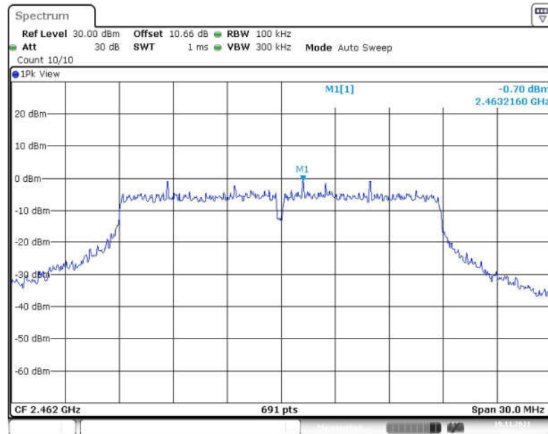
Fig.89 Conducted Spurious Emission (Center Frequency, 802.11n-HT20, CH11)
