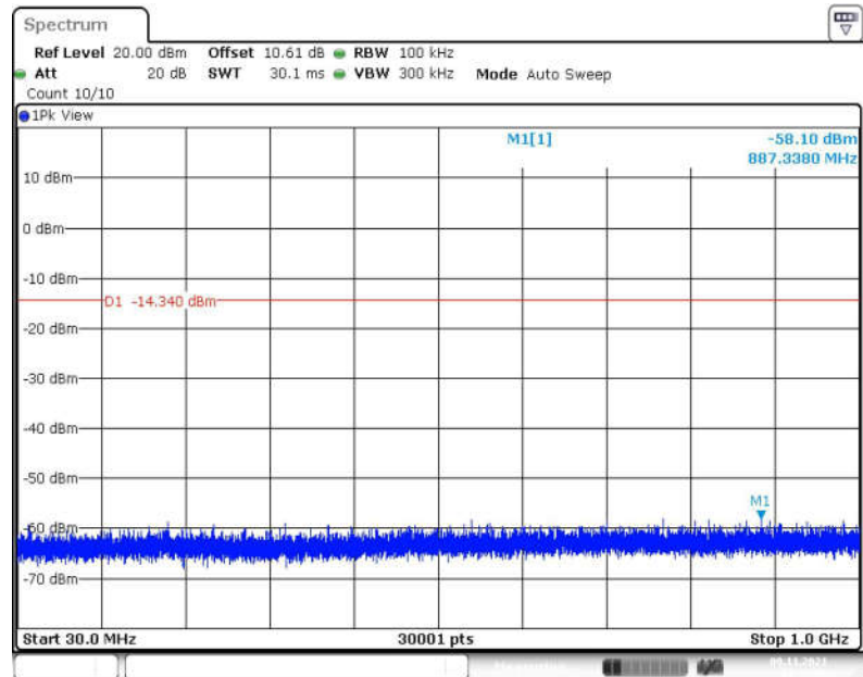
Fig.93 Conducted Spurious Emission (30MHz -1GHz, 802.11-VHT20, CH1)
