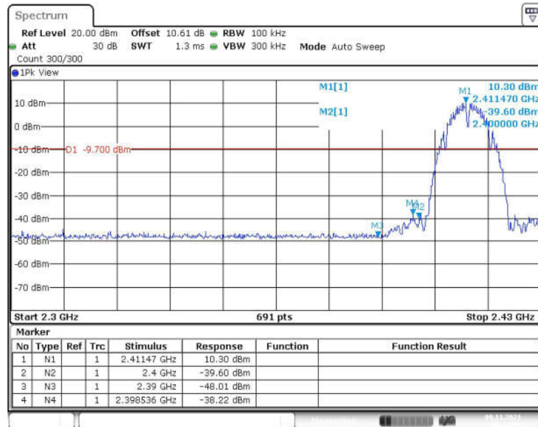
Fig.49 Band Edges (802.11b, CH 1)
