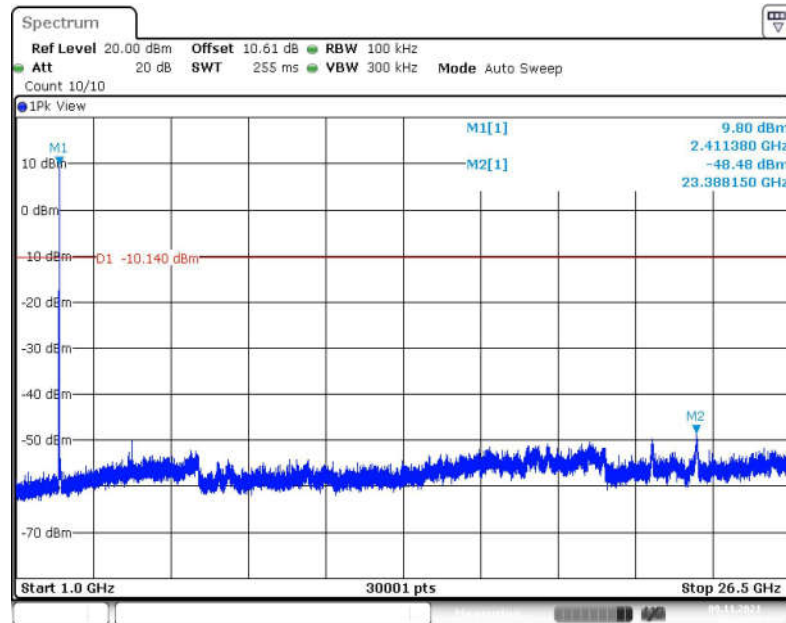
Fig.67 Conducted Spurious Emission (1GHz-26.5GHz, 802.11b, CH1)
