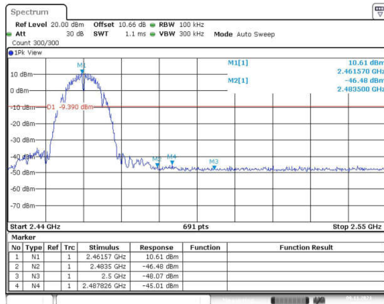
Fig.50 Band Edges (802.11b, CH 11)
