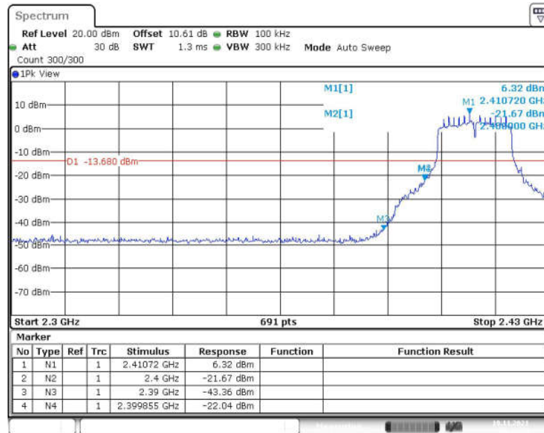
Fig.53 Band Edges (802.11n-HT20, CH 1)
