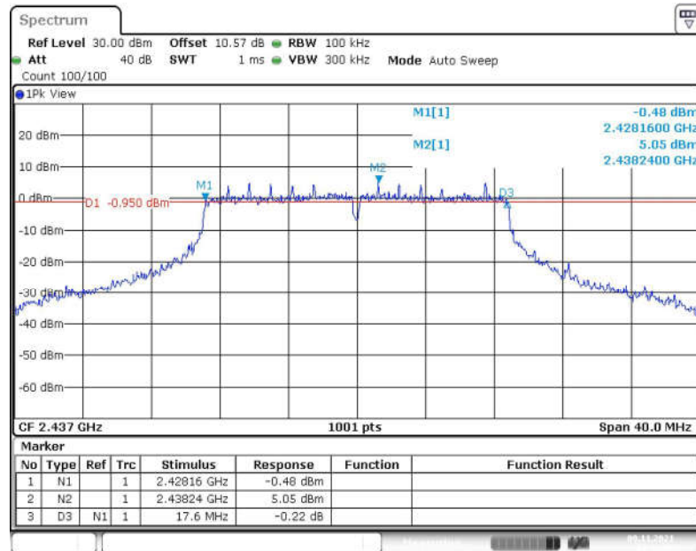
Fig.35 6dB Bandwidth (802.11-VHT20, CH 6)
