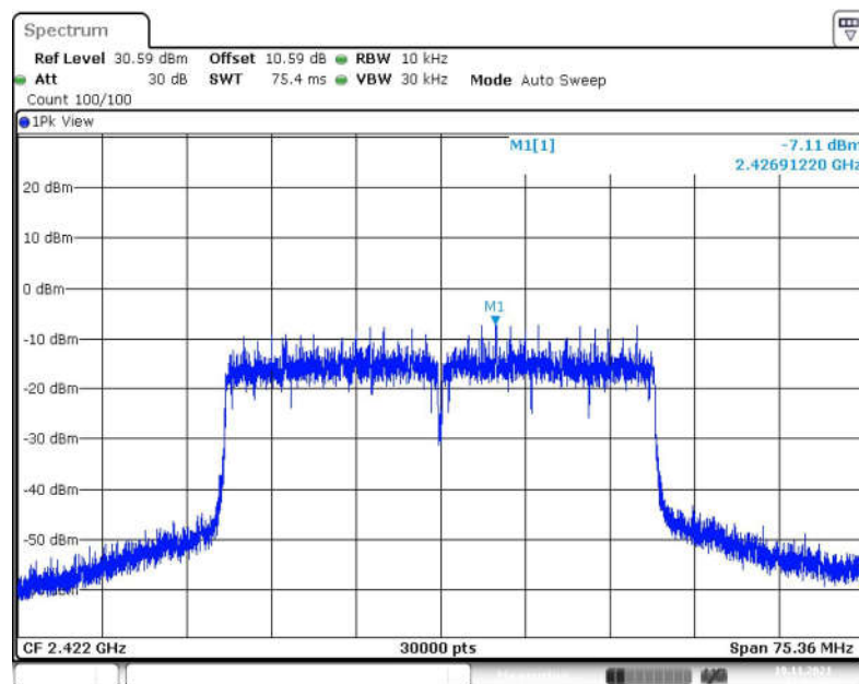
Fig.22 Power Spectral Density (802.11ax-HE40, CH 3)
