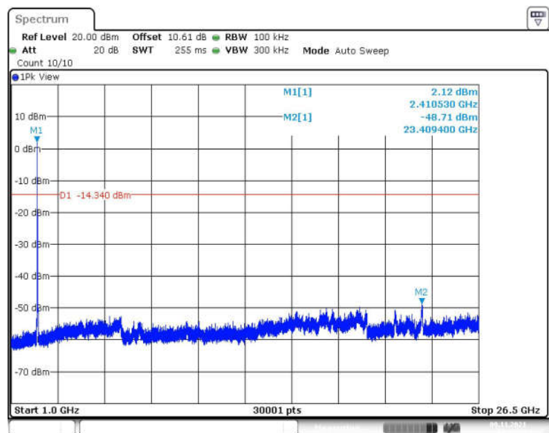
Fig.94 Conducted Spurious Emission (1GHz-26.5GHz, 802.11-VHT20, CH1)
