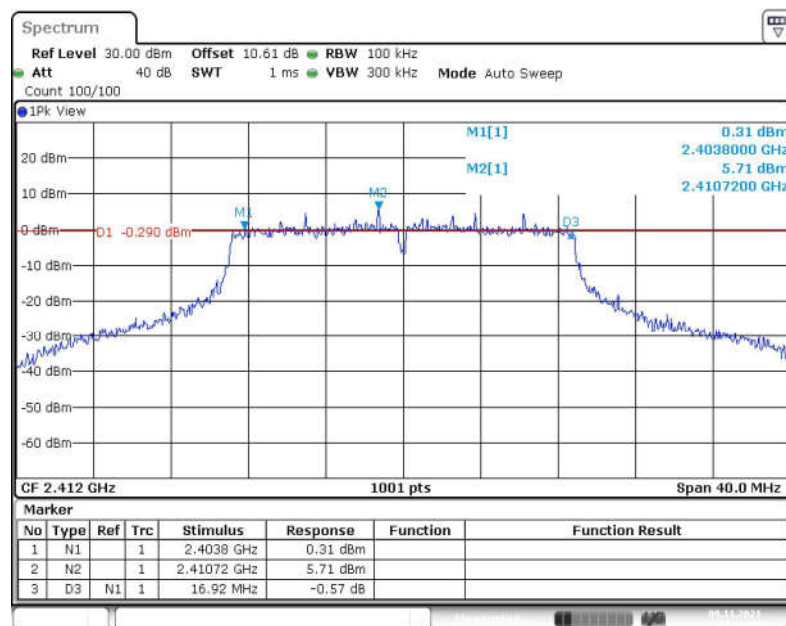
Fig.34 6dB Bandwidth (802.11-VHT20, CH 1)
