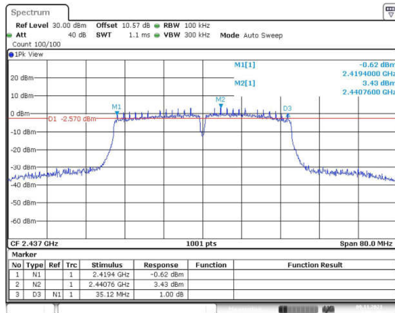
Fig.44 6dB Bandwidth (802.11-VHT40, CH 6)
