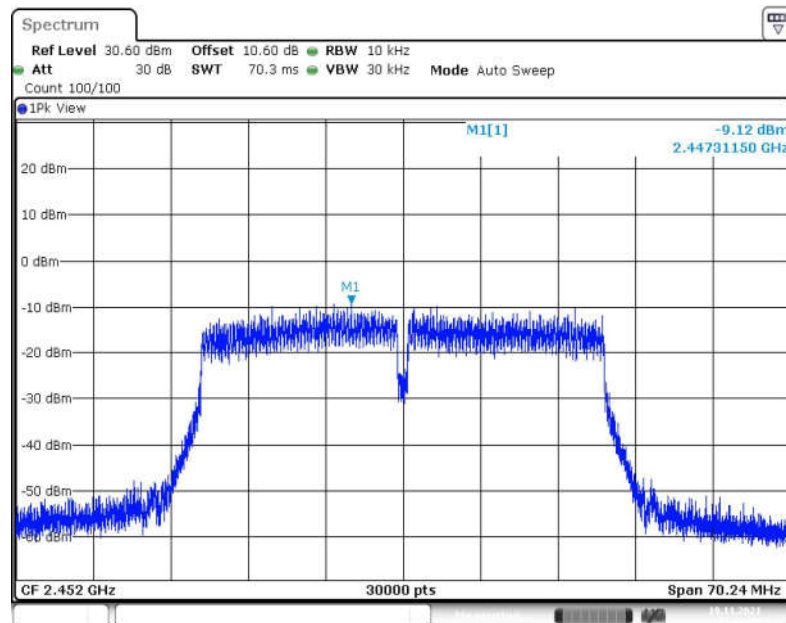
Fig.18 Power Spectral Density (802.11n-HT40, CH 9)
