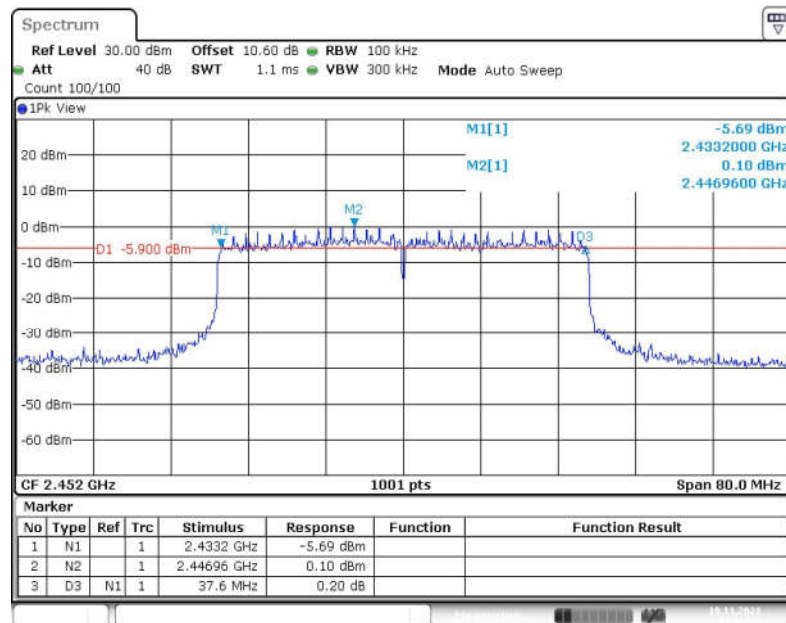
Fig.48 6dB Bandwidth (802.11ax-HE40, CH 9)
