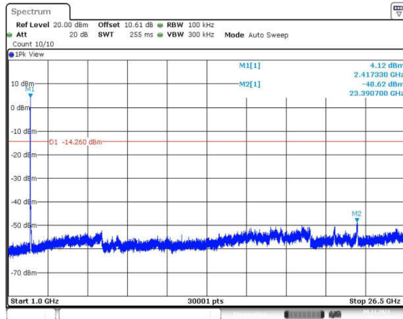
Fig.85 Conducted Spurious Emission (1GHz-26.5GHz, 802.11n-HT20, CH1)
