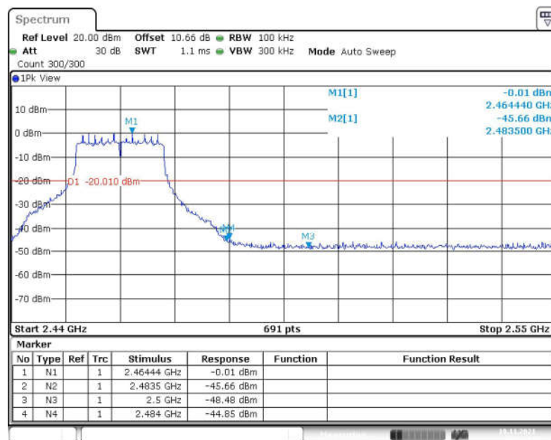
Fig.54 Band Edges (802.11n-HT20, CH 11)
