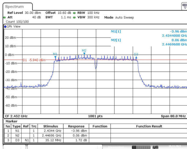
Fig.42 6dB Bandwidth (802.11n-HT40, CH 9)
