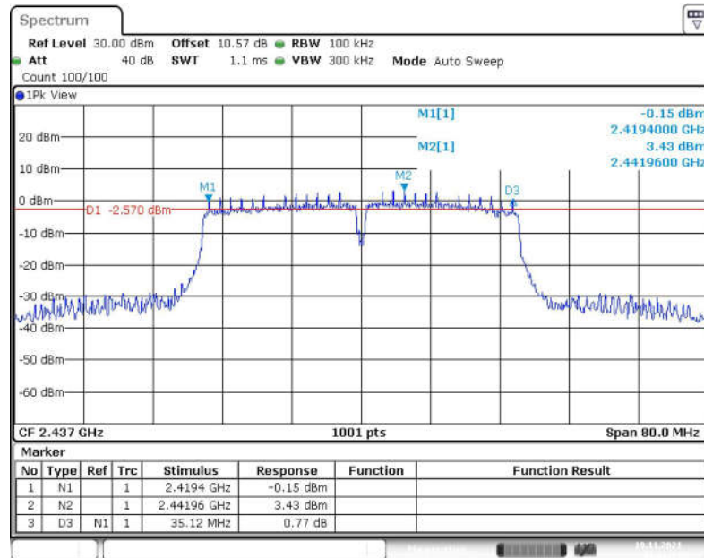
Fig.41 6dB Bandwidth (802.11n-HT40, CH 6)
