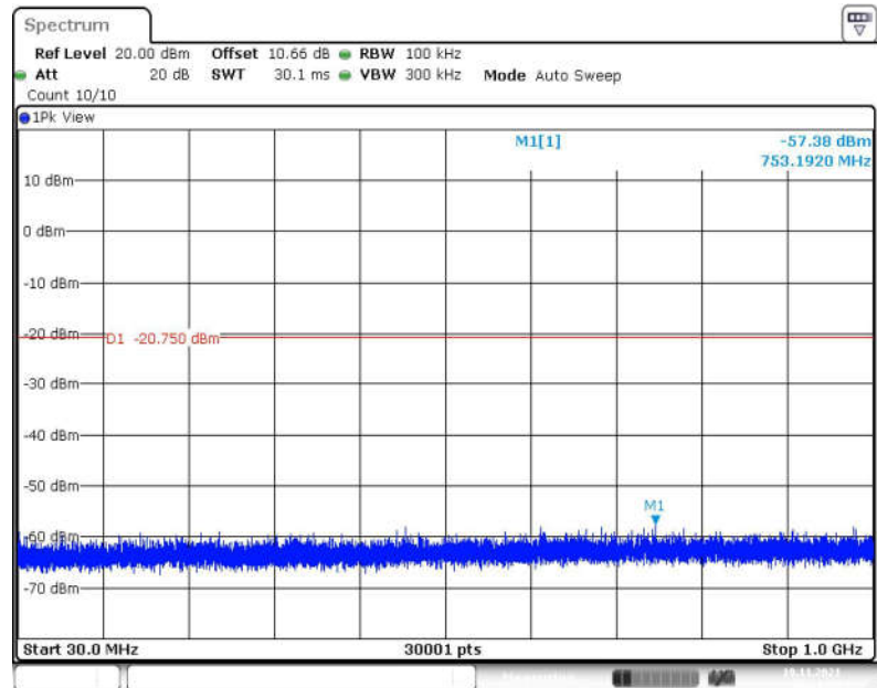
Fig.81 Conducted Spurious Emission (30MHz -1GHz, 802.11g, CH11)
