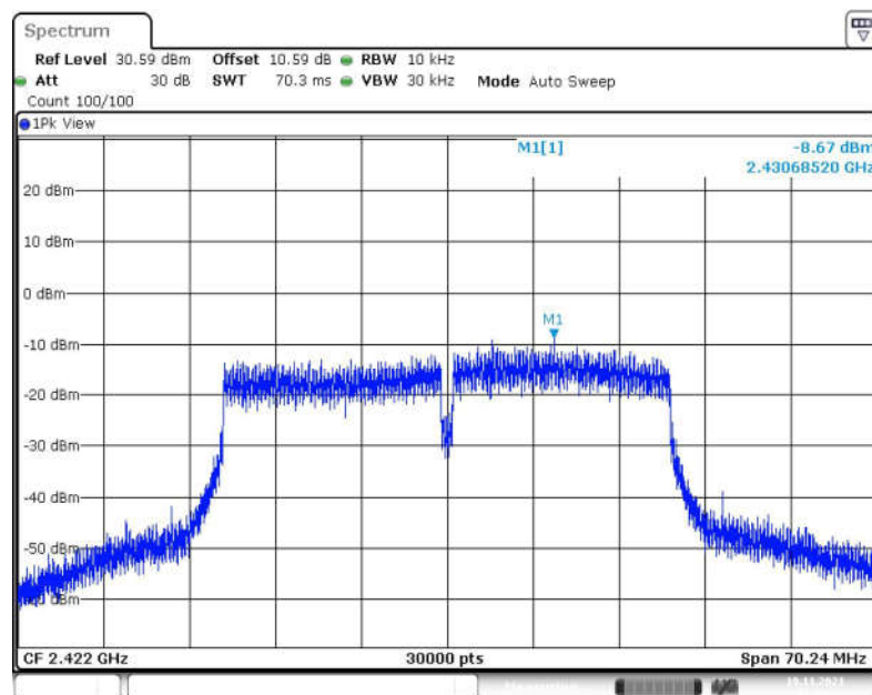
Fig.16 Power Spectral Density (802.11n-HT40, CH 3)
