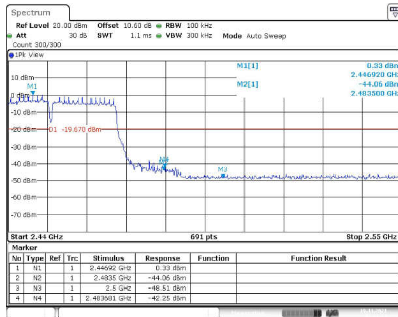
Fig.60 Band Edges (802.11n-HT40, CH 9)
