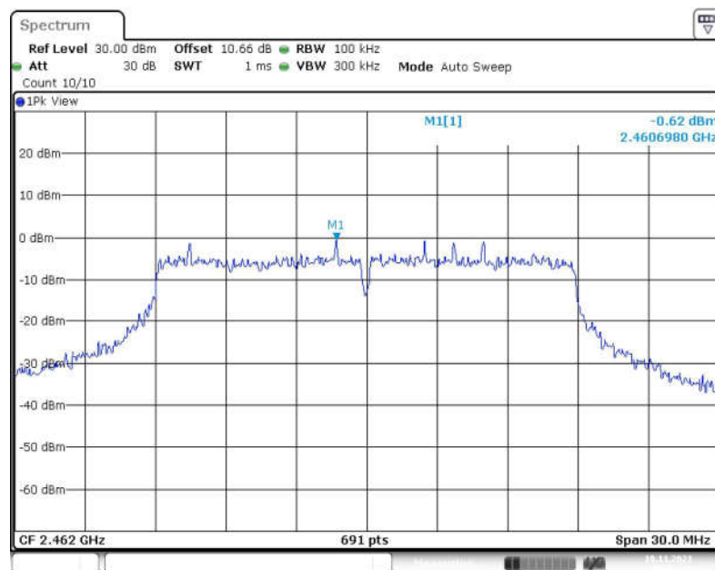
Fig.98 Conducted Spurious Emission (Center Frequency, 802.11-VHT20, CH11)
