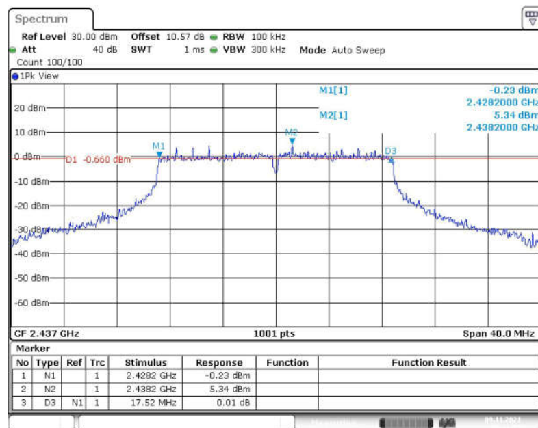
Fig.32 6dB Bandwidth (802.11n-HT20, CH 6)
