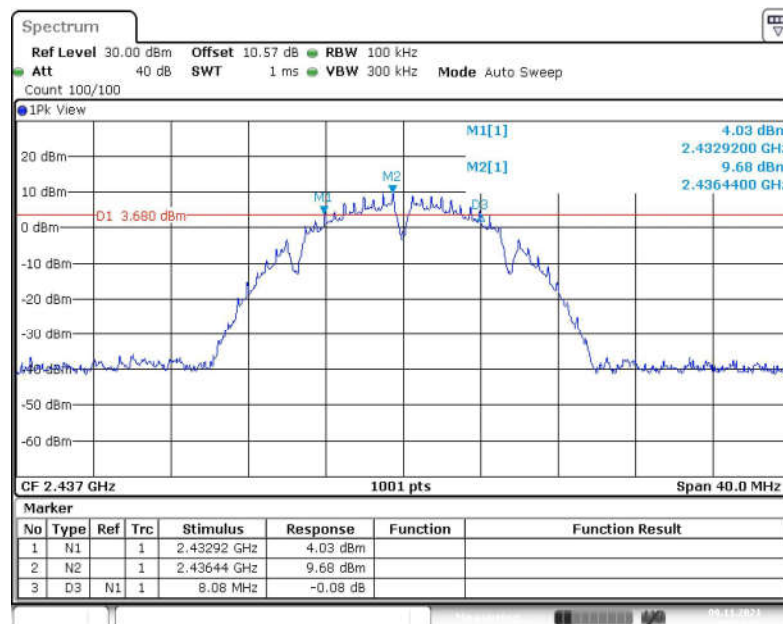
Fig.26 6dB Bandwidth (802.11b, CH 6)
