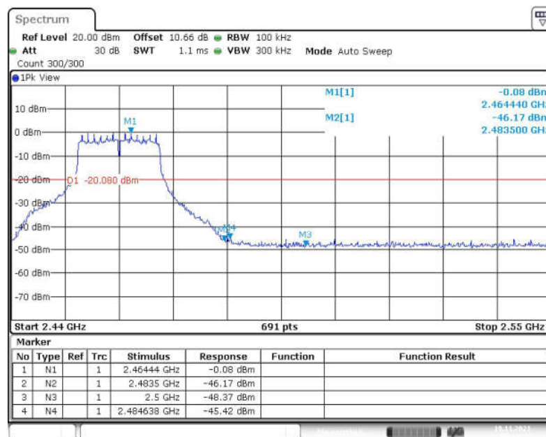
Fig.52 Band Edges (802.11g, CH 11)
