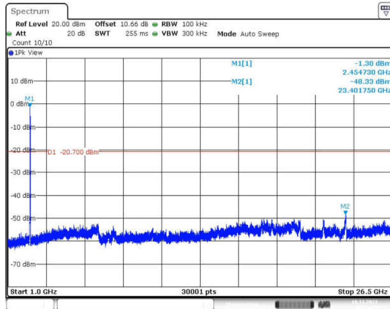
Fig.91 Conducted Spurious Emission (1GHz-26.5GHz, 802.11n-HT20, CH11)
