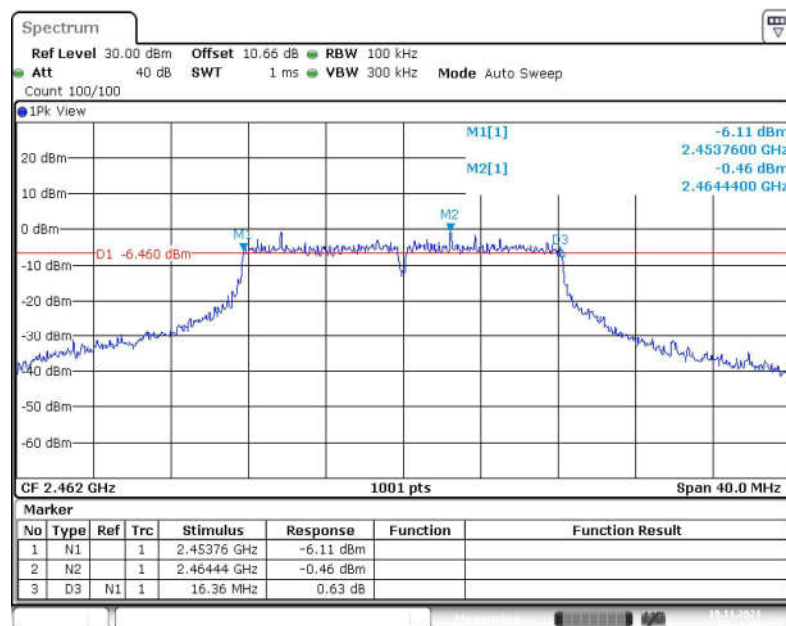
Fig.30 6dB Bandwidth (802.11g, CH 11)
