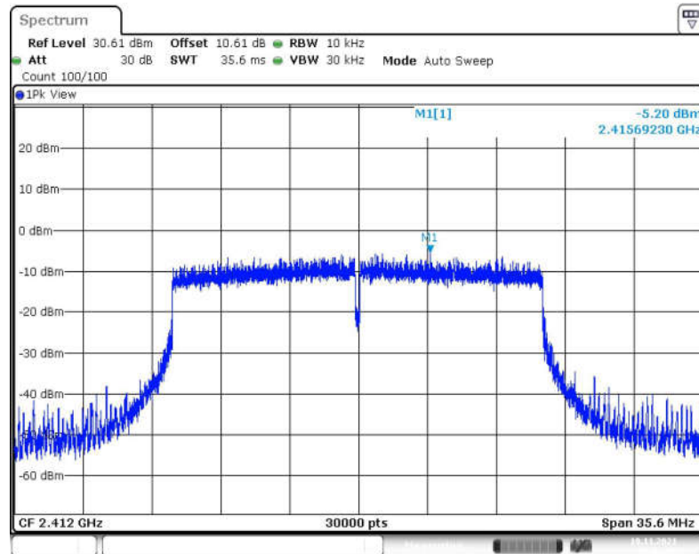
Fig.13 Power Spectral Density (802.11ax-HE20, CH 1)
