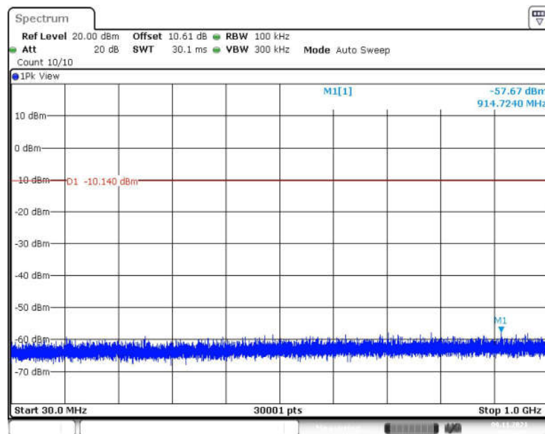
Fig.66 Conducted Spurious Emission (30MHz -1GHz, 802.11b, CH1)
