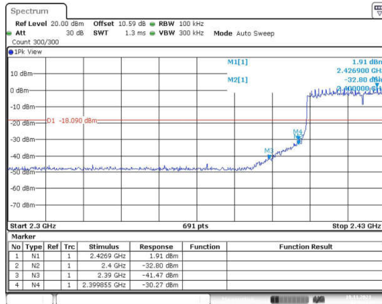
Fig.63 Band Edges (802.11ax-HE40, CH 3)
