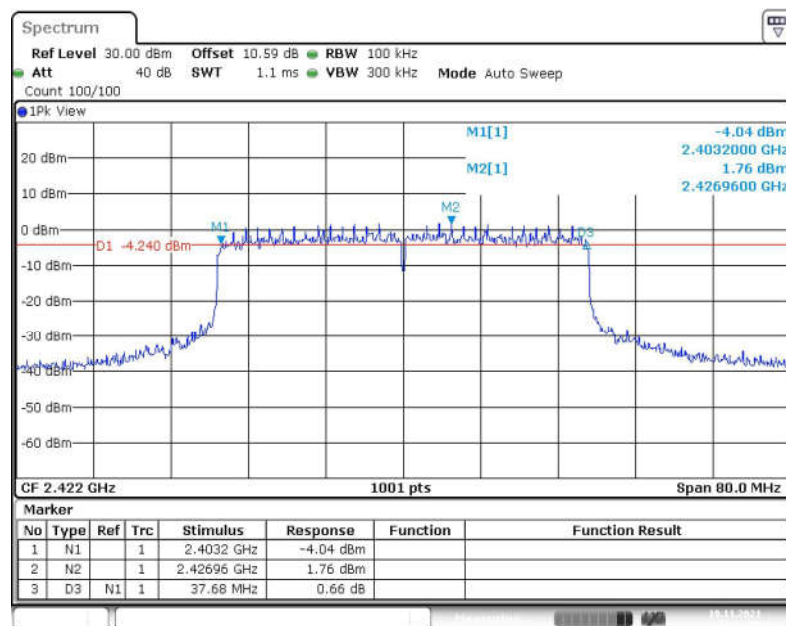
Fig.46 6dB Bandwidth (802.11ax-HE40, CH 3)
