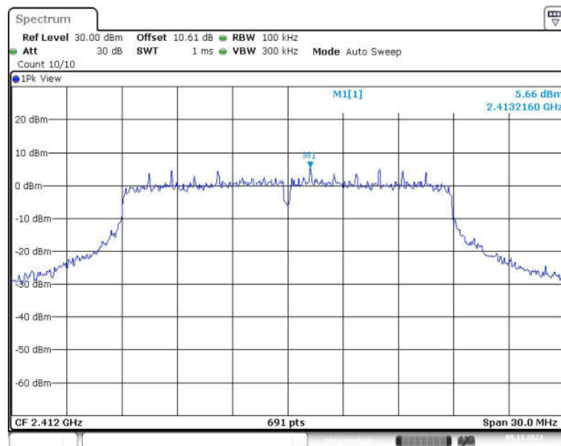
Fig.92 Conducted Spurious Emission (Center Frequency, 802.11-VHT20, CH1)
