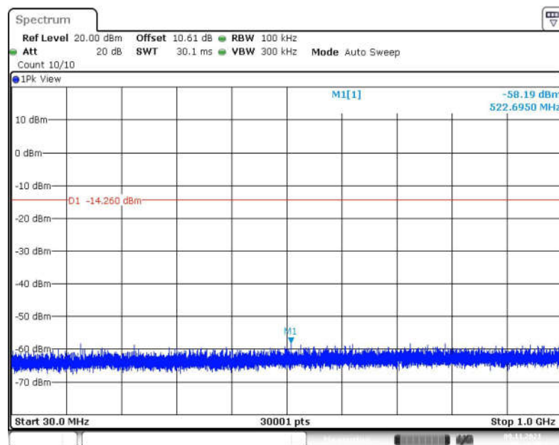
Fig.84 Conducted Spurious Emission (30MHz -1GHz, 802.11n-HT20, CH1)
