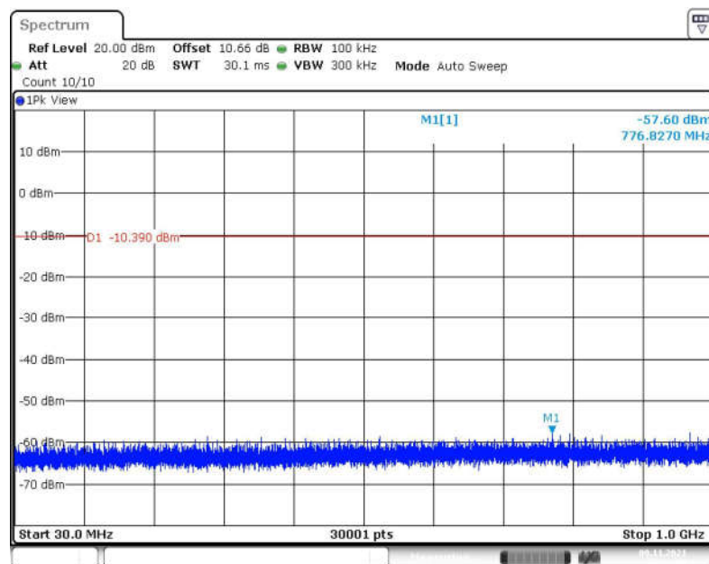
Fig.72 Conducted Spurious Emission (30MHz -1GHz, 802.11b, CH11)
