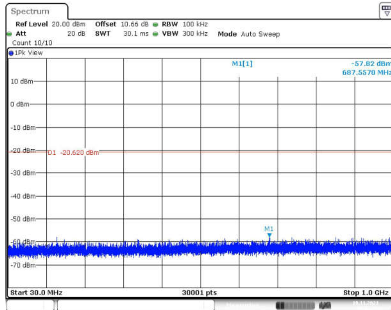
Fig.99 Conducted Spurious Emission (30MHz -1GHz, 802.11-VHT20, CH11)
