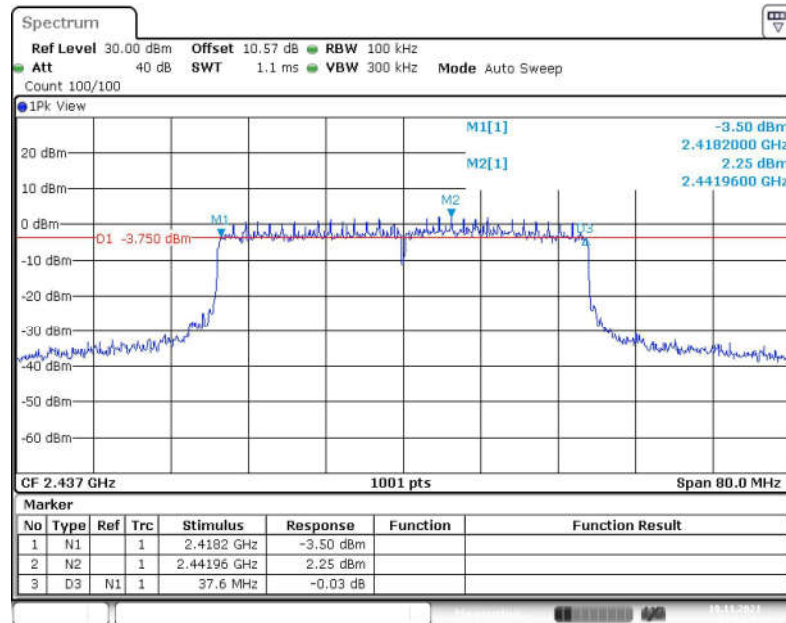
Fig.47 6dB Bandwidth (802.11ax-HE40, CH 6)
