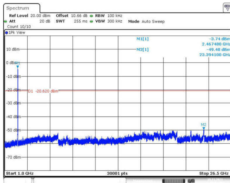
Fig.100 Conducted Spurious Emission (1GHz-26.5GHz, 802.11-VHT20, CH11)
