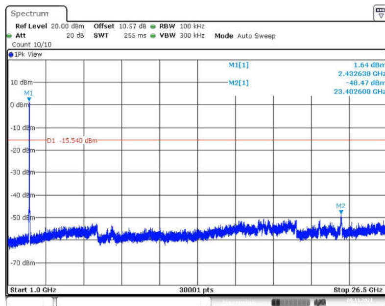
Fig.88 Conducted Spurious Emission (1GHz-26.5GHz, 802.11n-HT20, CH6)
