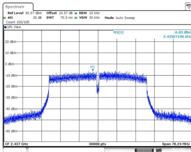
Fig.20 Power Spectral Density (802.11-VHT40, CH 6)
