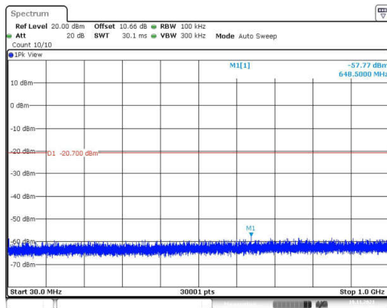
Fig.90 Conducted Spurious Emission (30MHz -1GHz, 802.11n-HT20, CH11)
