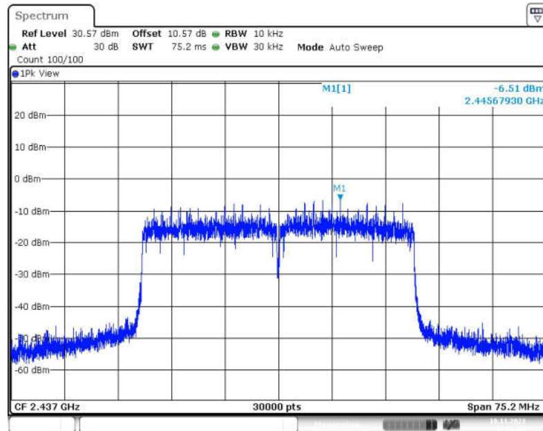
Fig.23 Power Spectral Density (802.11ax-HE40, CH 6)
