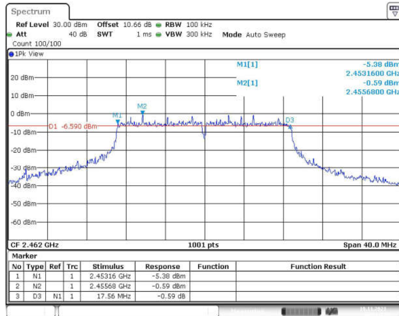
Fig.33 6dB Bandwidth (802.11n-HT20, CH 11)
