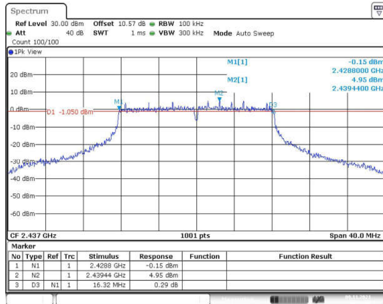
Fig.29 6dB Bandwidth (802.11g, CH 6)
