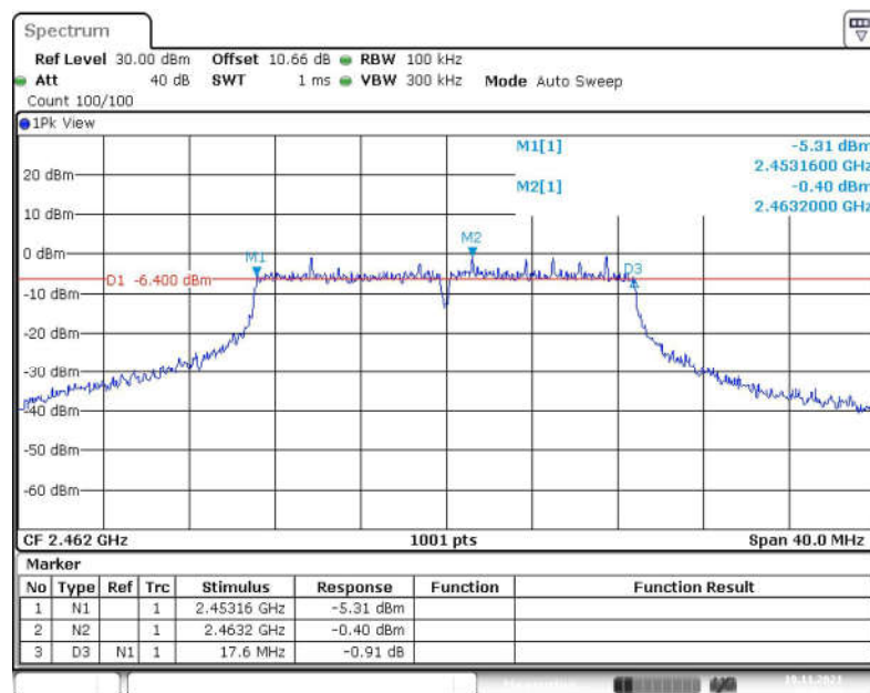
Fig.36 6dB Bandwidth (802.11-VHT20, CH 11)
