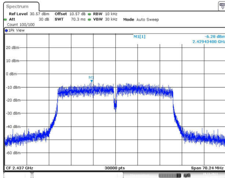
Fig.17 Power Spectral Density (802.11n-HT40, CH 6)
