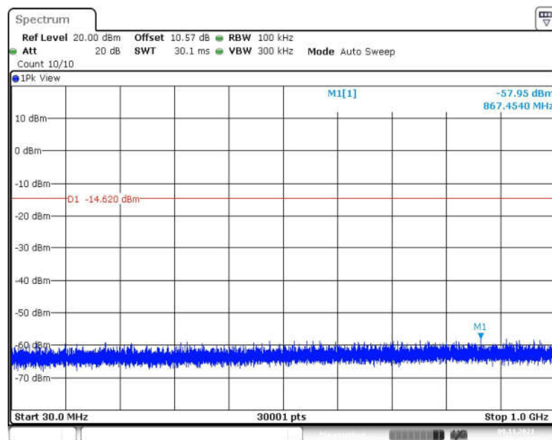
Fig.96 Conducted Spurious Emission (30MHz -1GHz, 802.11-VHT20, CH6)
