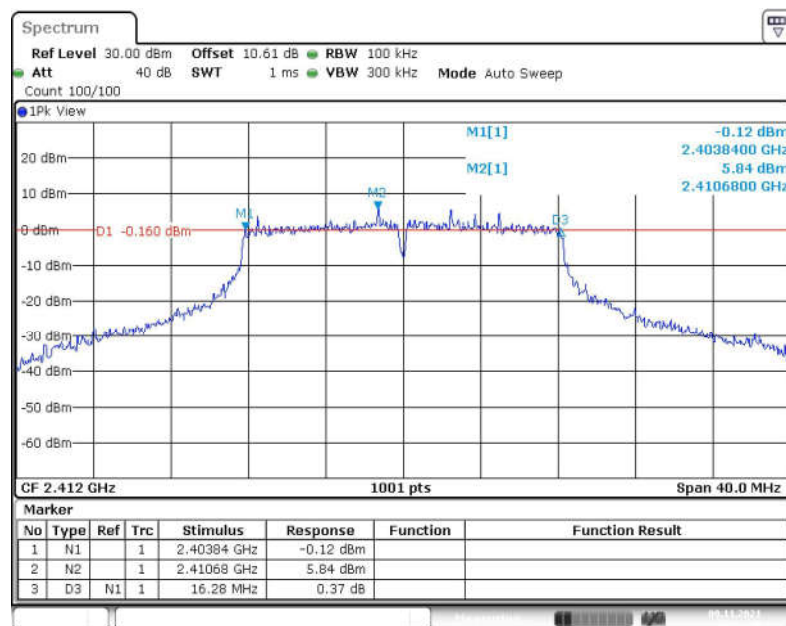
Fig.28 6dB Bandwidth (802.11g, CH 1)
