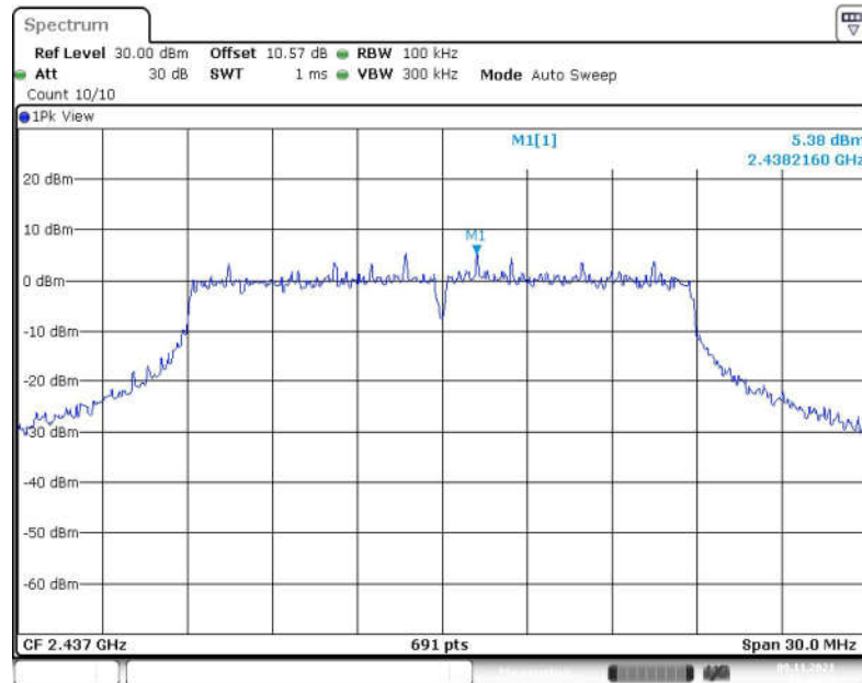
Fig.95 Conducted Spurious Emission (Center Frequency, 802.11-VHT20, CH6)
