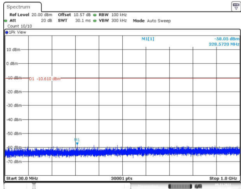
Fig.69 Conducted Spurious Emission (30MHz -1GHz, 802.11b, CH6)
