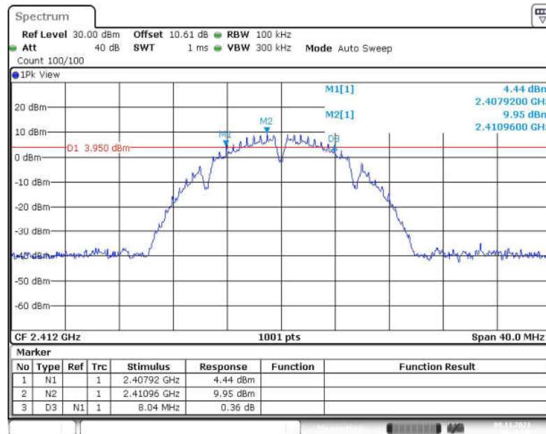
Fig.25 6dB Bandwidth (802.11b, CH 1)
