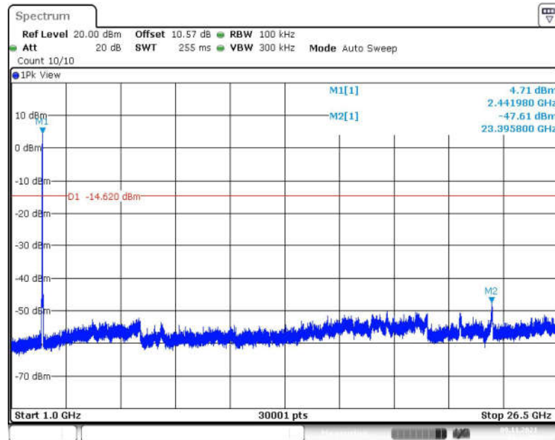
Fig.97 Conducted Spurious Emission (1GHz-26.5GHz, 802.11-VHT20, CH6)
