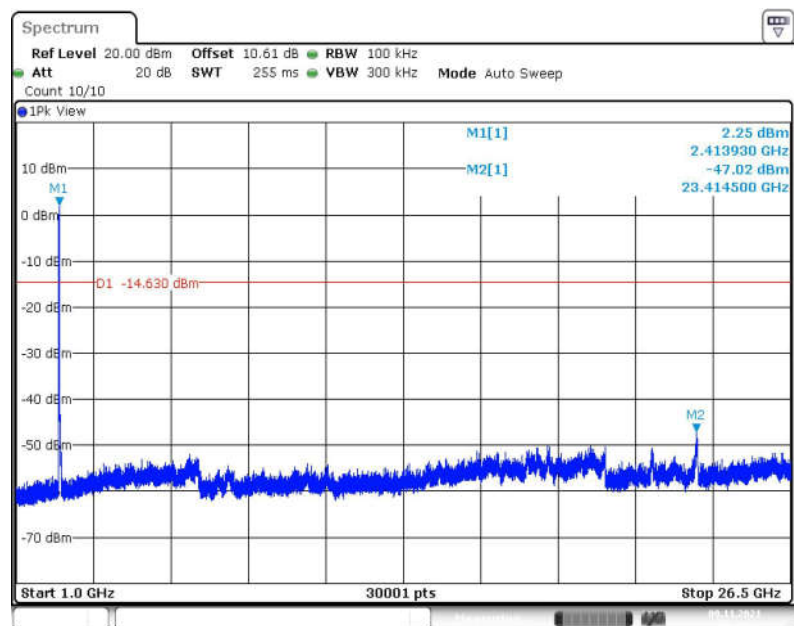
Fig.76 Conducted Spurious Emission (1GHz-26.5GHz, 802.11g, CH1)
