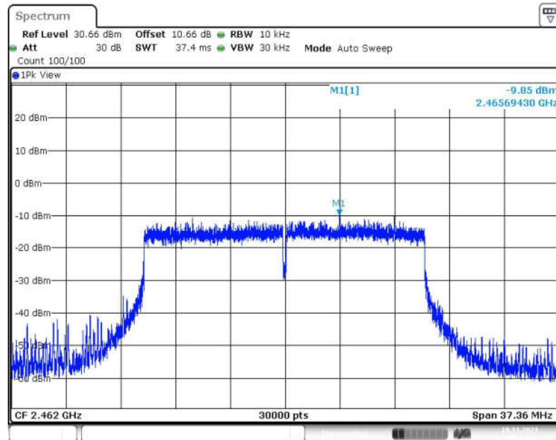
Fig.15 Power Spectral Density (802.11ax-HE20, CH 11)
