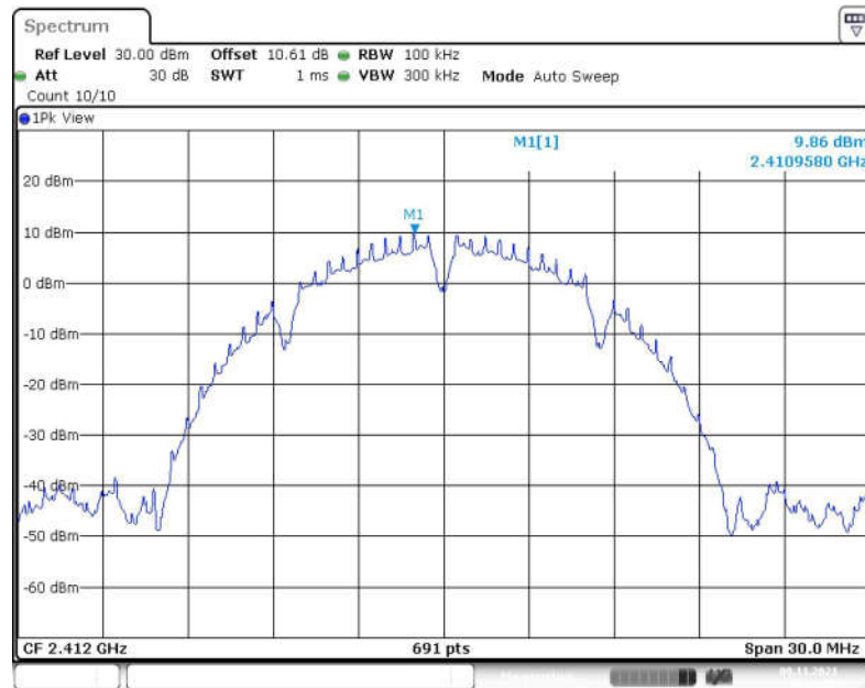
Fig.65 Conducted Spurious Emission (Center Frequency, 802.11b, CH1)
