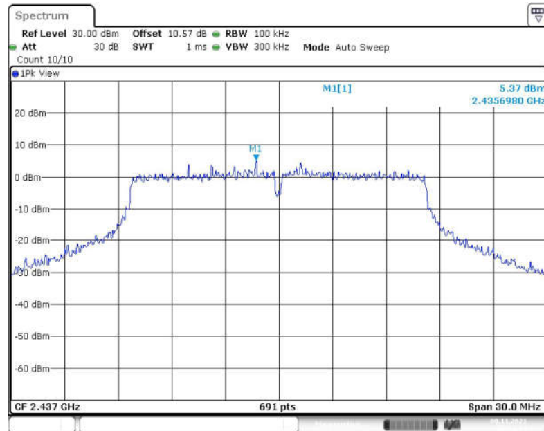
Fig.77 Conducted Spurious Emission (Center Frequency, 802.11g, CH6)
