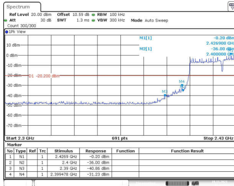
Fig.59 Band Edges (802.11n-HT40, CH 3)
