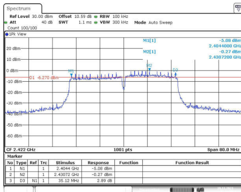
Fig.40 6dB Bandwidth (802.11n-HT40, CH 3)
