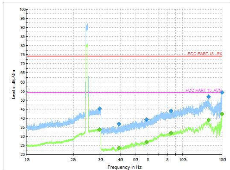
Fig.154 Radiated Spurious Emission (802.11-VHT20, CH11, 1 GHz-18 GHz)
