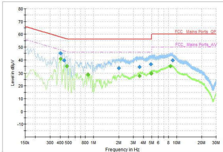
Fig.214 AC Power line Conducted Emission (Idle)
