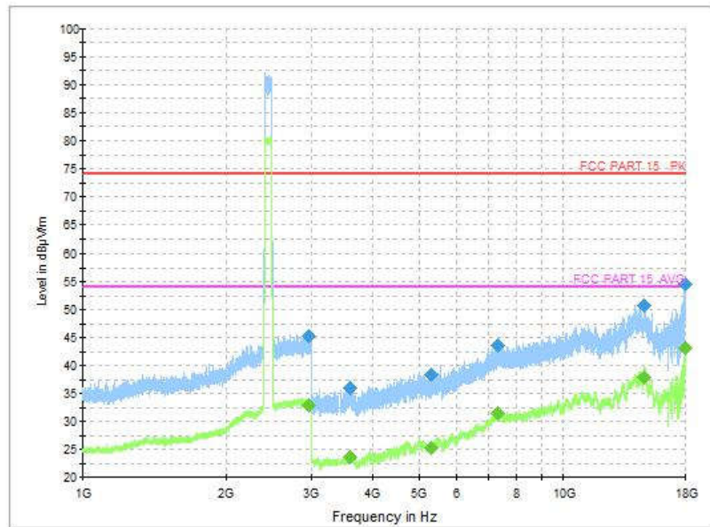
Fig.148 Radiated Spurious Emission (802.11n-HT20, CH6, 1 GHz-18 GHz)
