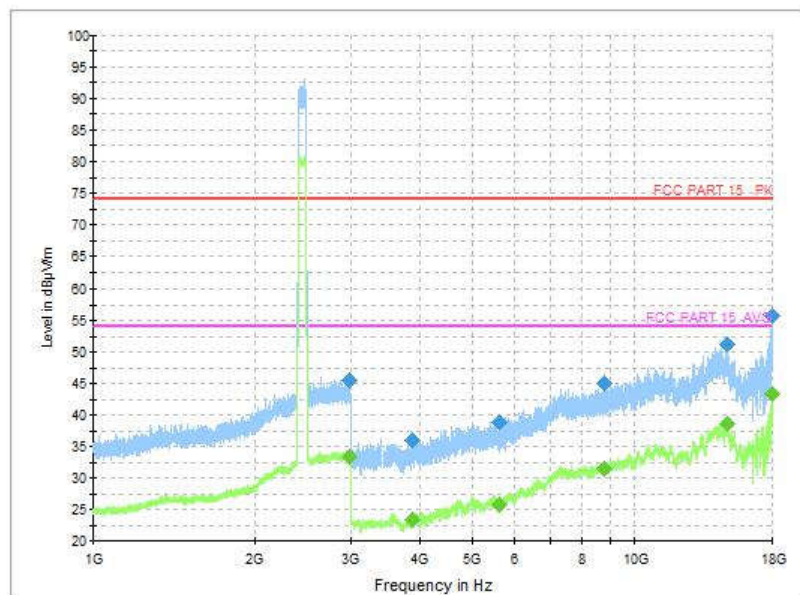
Fig.174 Radiated Spurious Emission (802.11ax-HE40, CH9, 1 GHz-18 GHz)
