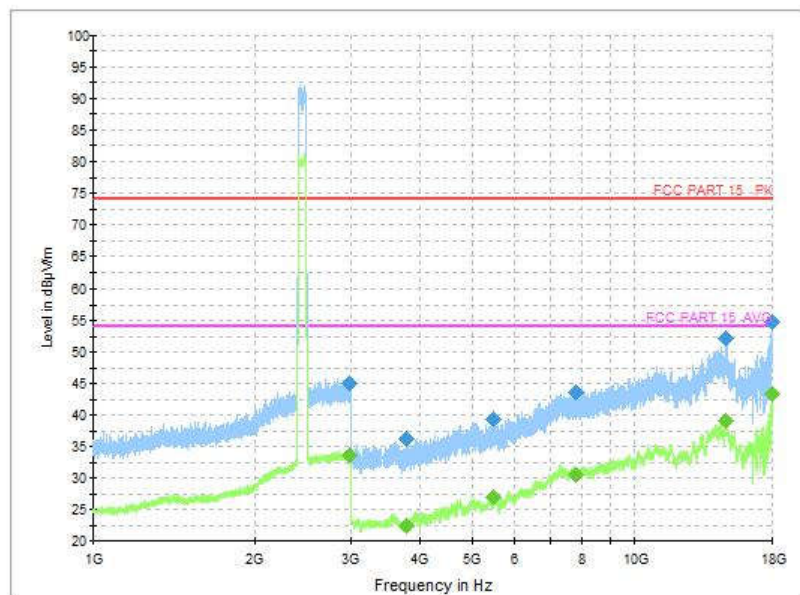
Fig.158 Radiated Spurious Emission (802.11ax-HE20, CH6, 1 GHz-18 GHz)
