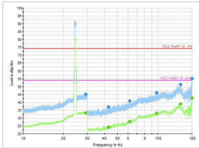
Fig.153 Radiated Spurious Emission (802.11-VHT20, CH6, 1 GHz-18 GHz)
