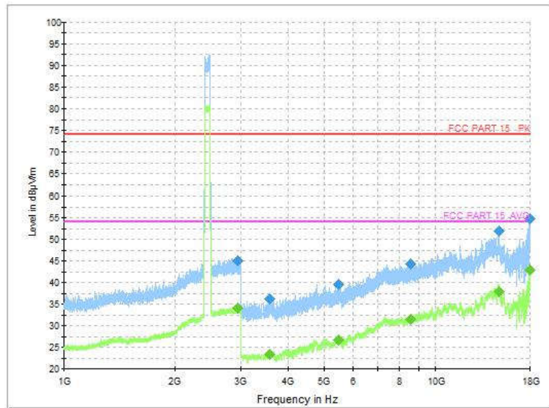
Fig.163 Radiated Spurious Emission (802.11n-HT40, CH6, 1 GHz-18 GHz)
