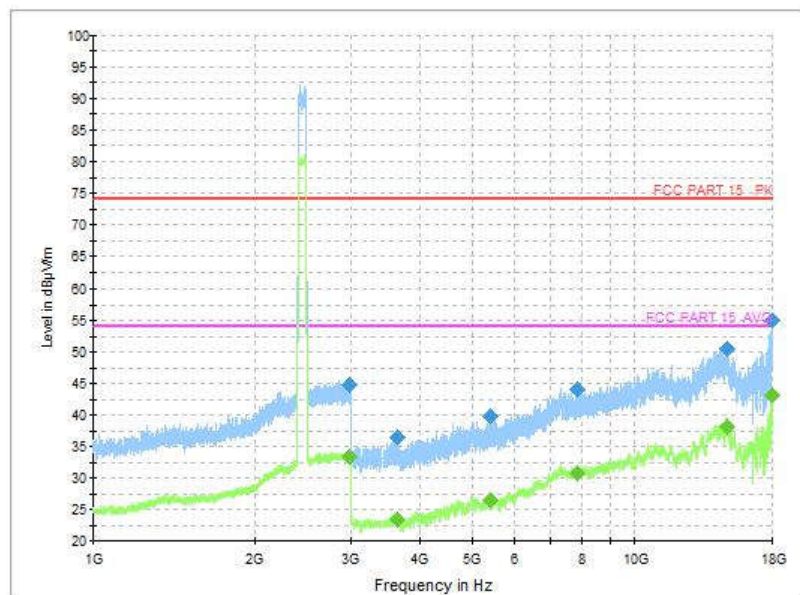
Fig.164 Radiated Spurious Emission (802.11n-HT40, CH9, 1 GHz-18 GHz)
