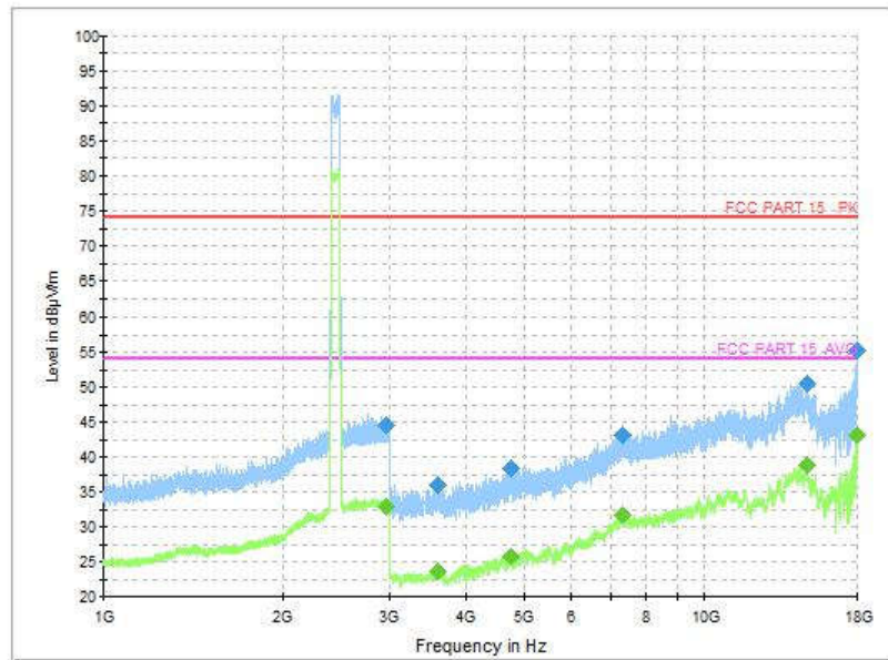
Fig.173 Radiated Spurious Emission (802.11ax-HE40, CH6, 1 GHz-18 GHz)
