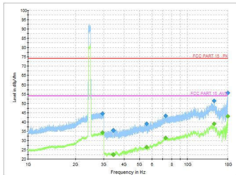
Fig.138 Radiated Spurious Emission (802.11b, CH6, 1 GHz-18GHz)
