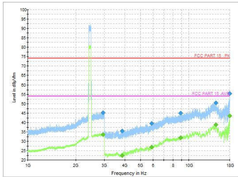
Fig.147 Radiated Spurious Emission (802.11n-HT20, CH1, 1 GHz-18 GHz)
