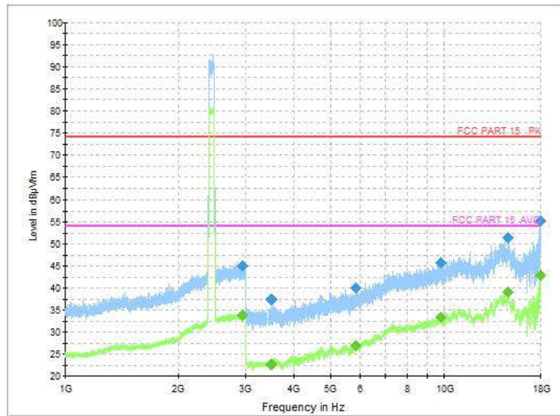
Fig.157 Radiated Spurious Emission (802.11ax-HE20, CH1, 1 GHz-18 GHz)
