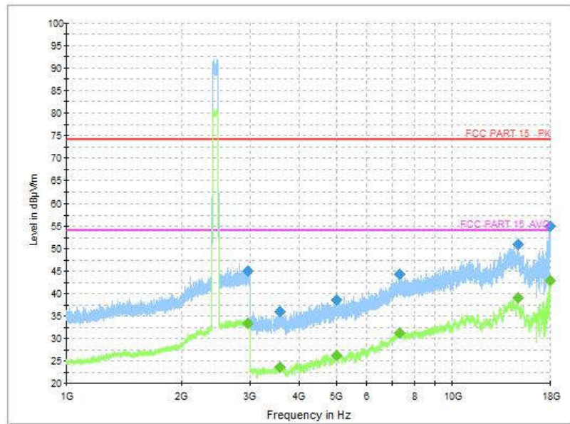
Fig.167 Radiated Spurious Emission (802.11-VHT40, CH3, 1 GHz-18 GHz)
