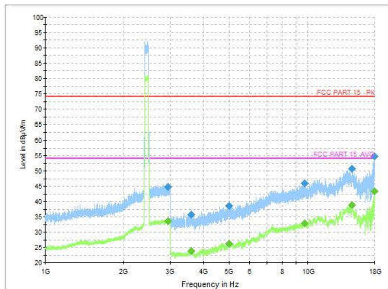
Fig.168 Radiated Spurious Emission (802.11-VHT40, CH6, 1 GHz-18 GHz)
