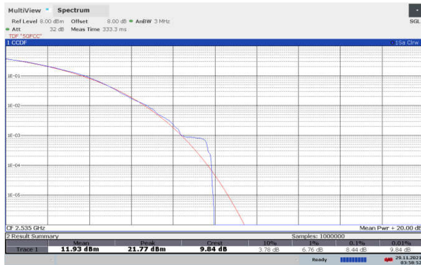
n7, CP-64QAM (PAPR)
