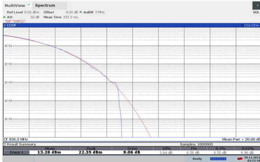
n5, DFT-s-pi/2 BPSK (PAPR)
