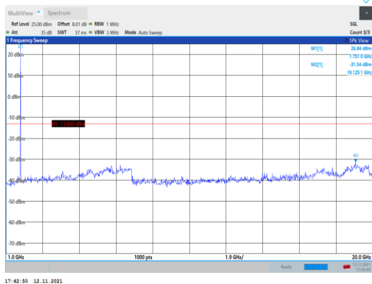
Band66-1.4MHz-QPSK-132322-1RB#0- Range2:1000~20000MHz
