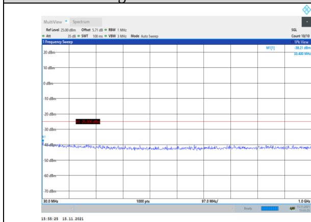
Band38-15MHz-16QAM-38175-1RB#0- Range1:30~1000MHz
