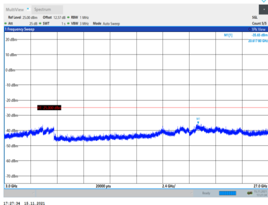
Band41-15MHz-QPSK-40115-1RB#0- Range3:3000~27000MHz
