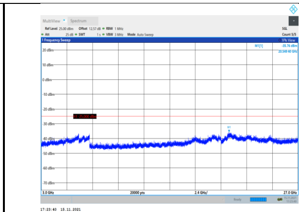
Band41-10MHz-16QAM-40090-1RB#0- Range3:3000~27000MHz
