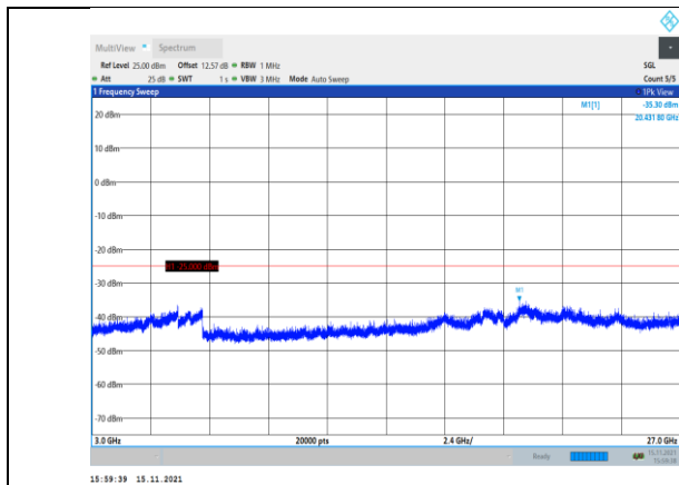
Band38-20MHz-QPSK-38150-1RB#0- Range3:3000~27000MHz
