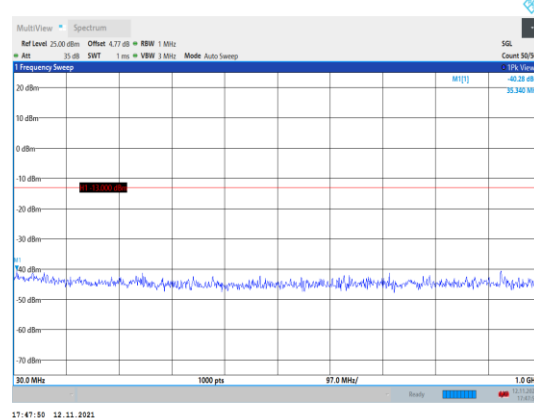
Band66-3MHz-16QAM-131987-1RB#0- Range1:30~1000MHz
