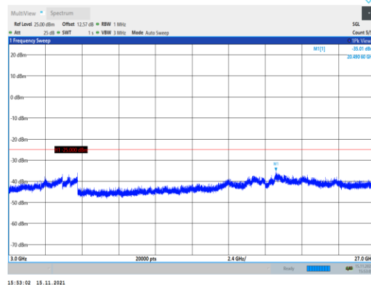
Band38-15MHz-16QAM-37825-1RB#0- Range3:3000~27000MHz
