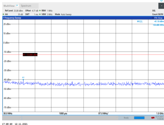
Band66-3MHz-16QAM-132322-1RB#0- Range1:30~1000MHz
