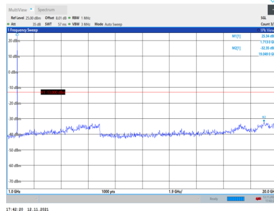
Band66-1.4MHz-16QAM-131979-1RB#0- Range2:1000~20000MHz
