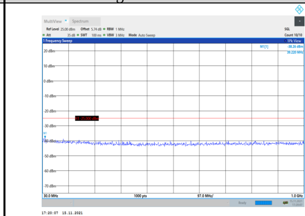
Band41-5MHz-16QAM-40590-1RB#0- Range1:30~1000MHz
