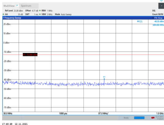
Band66-3MHz-16QAM-132657-1RB#0- Range1:30~1000MHz
