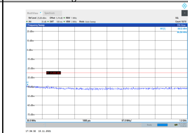
Band41-20MHz-QPSK-41140-1RB#0- Range1:30~1000MHz
