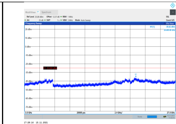
Band41-15MHz-16QAM-40115-1RB#0- Range3:3000~27000MHz
