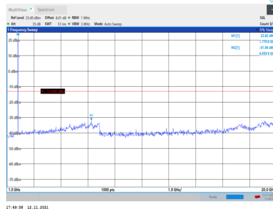
Band66-3MHz-16QAM-132657-1RB#0- Range2:1000~20000MHz
