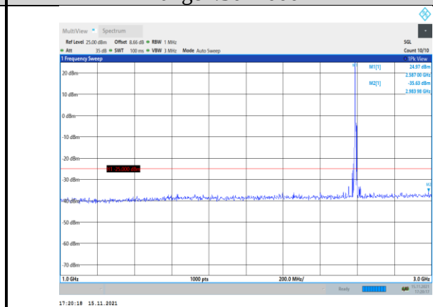
Band41-5MHz-16QAM-40590-1RB#0- Range2:1000~3000MHz
