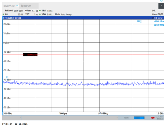
Band66-1.4MHz-16QAM-132665-1RB#0- Range1:30~1000MHz
