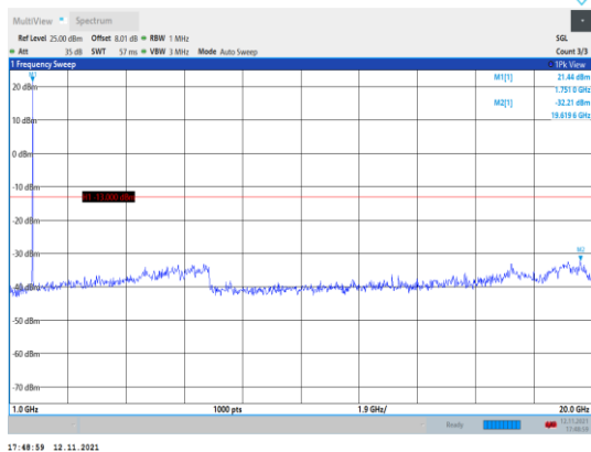
Band66-3MHz-16QAM-132322-1RB#0- Range2:1000~20000MHz
