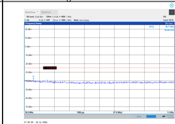
Band41-20MHz-16QAM-40590-1RB#0- Range1:30~1000MHz
