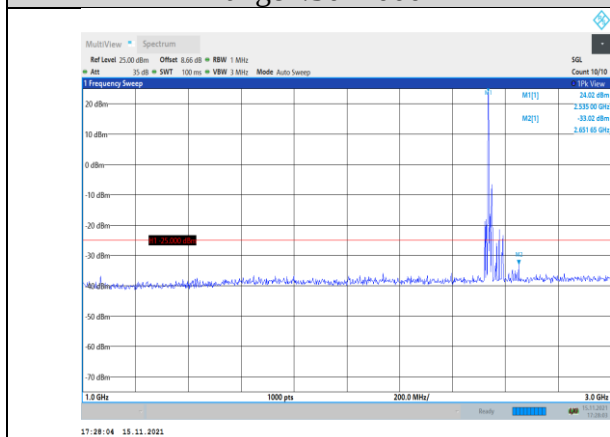
Band41-15MHz-16QAM-40115-1RB#0- Range2:1000~3000MHz
