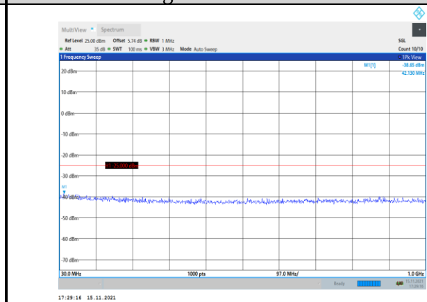
Band41-15MHz-16QAM-40590-1RB#0- Range1:30~1000MHz
