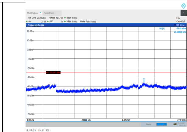
Band38-20MHz-16QAM-37850-1RB#0- Range3:3000~27000MHz
