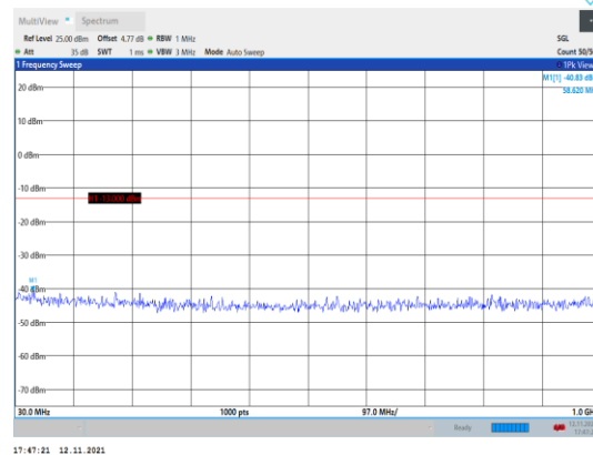
Band66-3MHz-QPSK-131987-1RB#0- Range1:30~1000MHz
