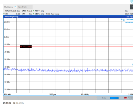
Band66-5MHz-16QAM-131997-1RB#0- Range1:30~1000MHz
