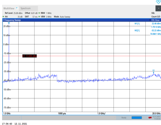
Band66-5MHz-QPSK-132322-1RB#0- Range2:1000~20000MHz
