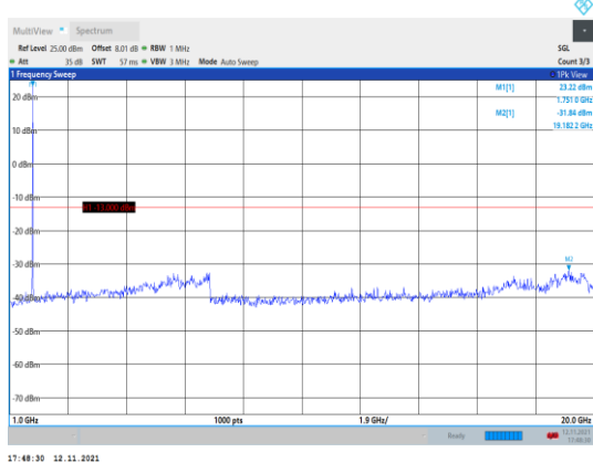
Band66-3MHz-QPSK-132322-1RB#0- Range2:1000~20000MHz
