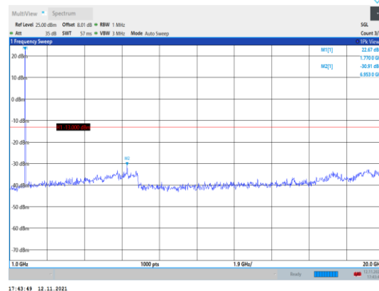
Band66-1.4MHz-QPSK-132665-1RB#0- Range2:1000~20000MHz
