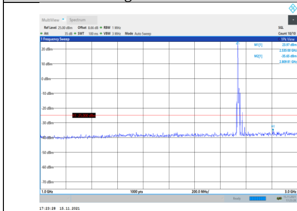
Band41-10MHz-16QAM-40090-1RB#0- Range2:1000~3000MHz
