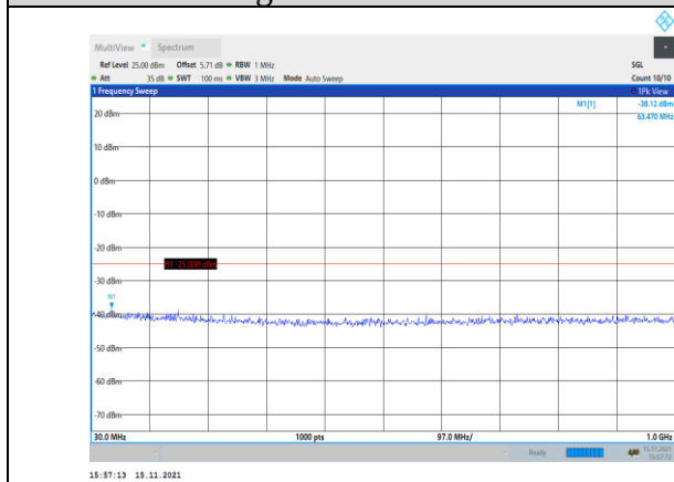
Band38-20MHz-16QAM-37850-1RB#0- Range1:30~1000MHz
