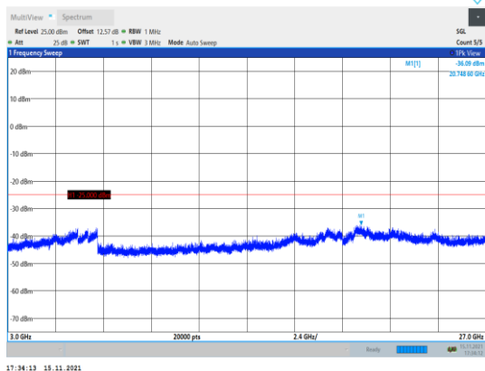
Band41-20MHz-16QAM-40590-1RB#0- Range3:3000~27000MHz
