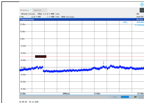
Band38-15MHz-16QAM-38000-1RB#0- Range3:3000~27000MHz
