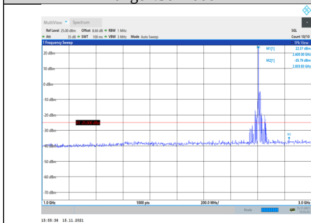
Band38-15MHz-16QAM-38175-1RB#0- Range2:1000~3000MHz
