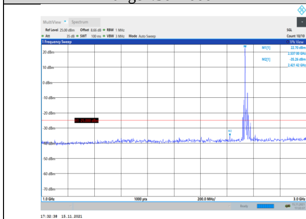
Band41-20MHz-16QAM-40140-1RB#0- Range2:1000~3000MHz
