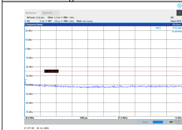
Band41-15MHz-16QAM-40115-1RB#0- Range1:30~1000MHz
