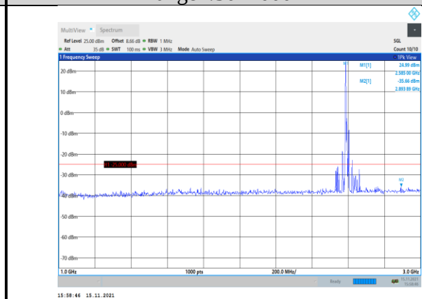
Band38-20MHz-16QAM-38000-1RB#0- Range2:1000~3000MHz
