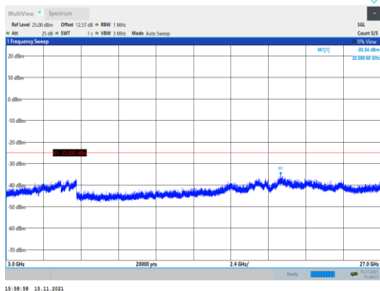
Band38-20MHz-16QAM-38000-1RB#0- Range3:3000~27000MHz
