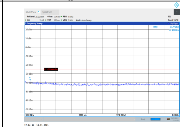
Band41-10MHz-16QAM-40590-1RB#0- Range1:30~1000MHz
