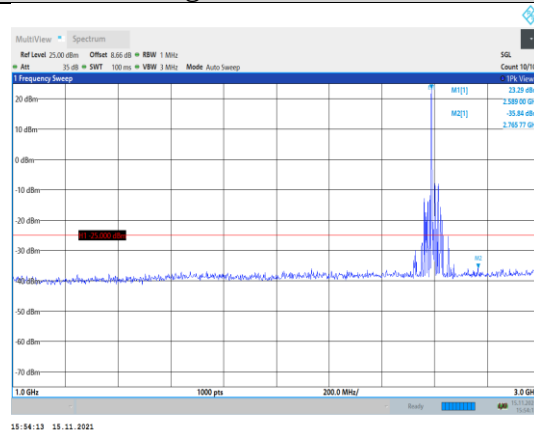
Band38-15MHz-16QAM-38000-1RB#0- Range2:1000~3000MHz
