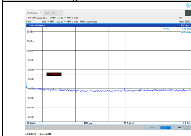
Band41-10MHz-16QAM-40090-1RB#0- Range1:30~1000MHz
