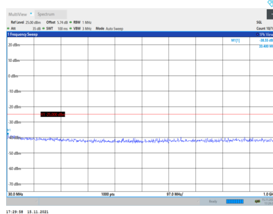
Band41-15MHz-QPSK-41165-1RB#0- Range1:30~1000MHz
