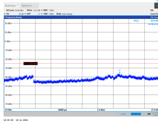
Band38-20MHz-16QAM-38150-1RB#0- Range3:3000~27000MHz
