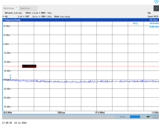
Band41-15MHz-QPSK-40590-1RB#0- Range1:30~1000MHz
