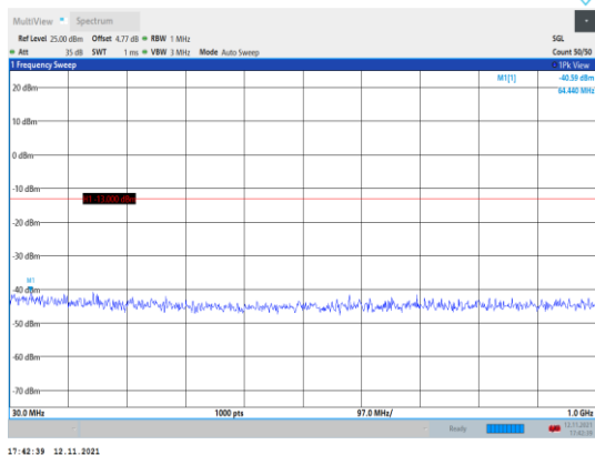
Band66-1.4MHz-QPSK-132322-1RB#0- Range1:30~1000MHz
