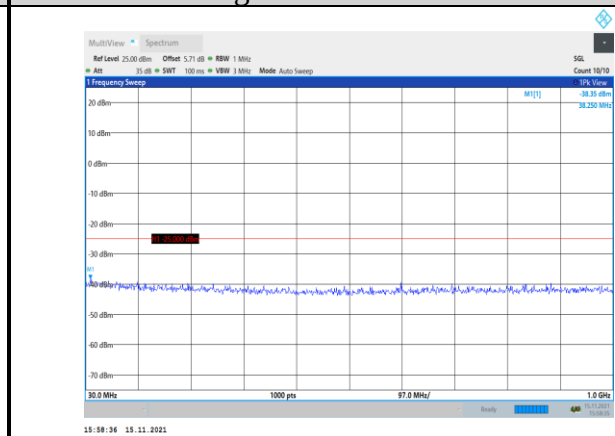
Band38-20MHz-16QAM-38000-1RB#0- Range1:30~1000MHz
