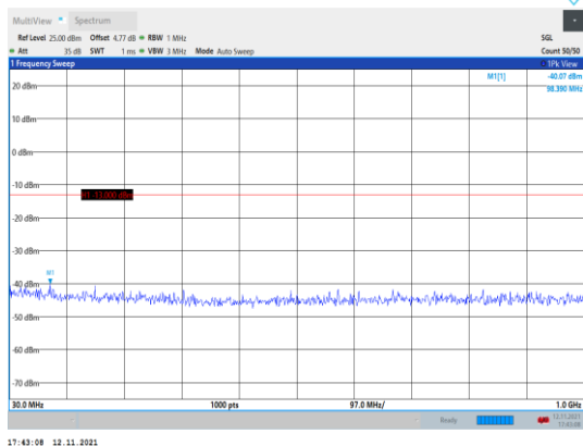
Band66-1.4MHz-16QAM-132322-1RB#0- Range1:30~1000MHz
