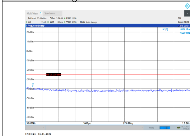
Band41-5MHz-QPSK-40590-1RB#0- Range1:30~1000MHz
