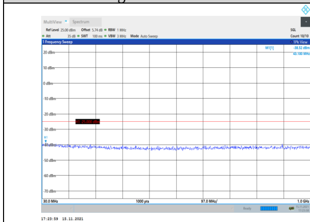
Band41-10MHz-QPSK-40590-1RB#0- Range1:30~1000MHz
