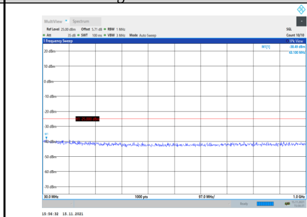
Band38-20MHz-QPSK-37850-1RB#0- Range1:30~1000MHz
