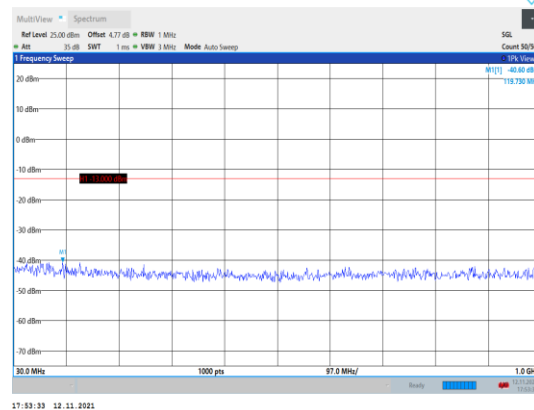
Band66-5MHz-QPSK-131997-1RB#0- Range1:30~1000MHz
