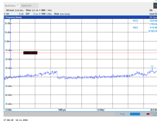
Band66-1.4MHz-16QAM-132665-1RB#0- Range2:1000~20000MHz
