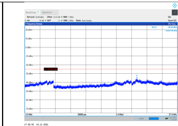
Band41-20MHz-16QAM-40140-1RB#0- Range3:3000~27000MHz
