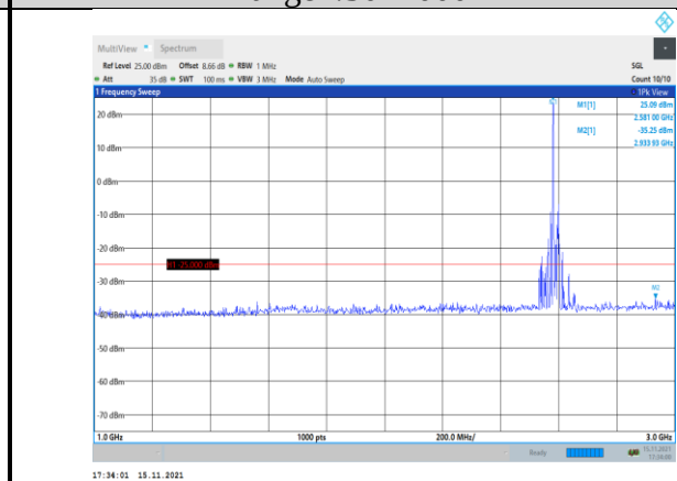
Band41-20MHz-16QAM-40590-1RB#0- Range2:1000~3000MHz
