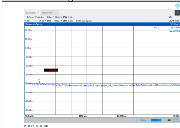
Band41-20MHz-16QAM-40140-1RB#0- Range1:30~1000MHz
