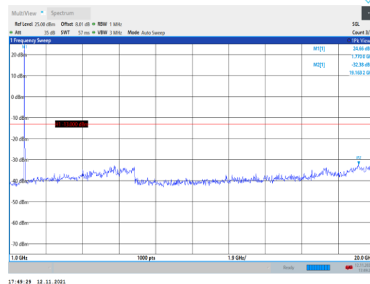
Band66-3MHz-QPSK-132657-1RB#0- Range2:1000~20000MHz
