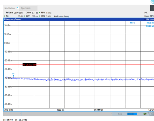
Band38-15MHz-16QAM-38000-1RB#0- Range1:30~1000MHz
