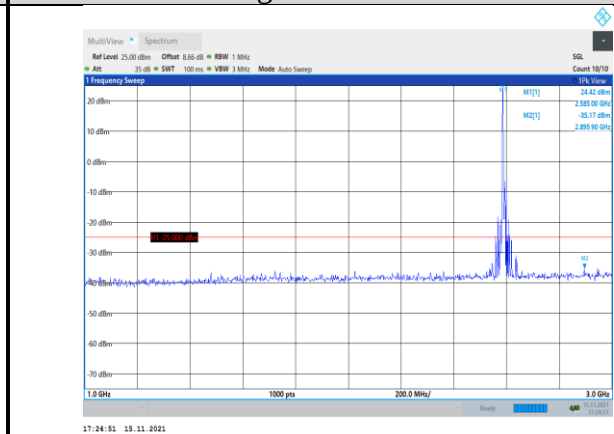
Band41-10MHz-16QAM-40590-1RB#0- Range2:1000~3000MHz
