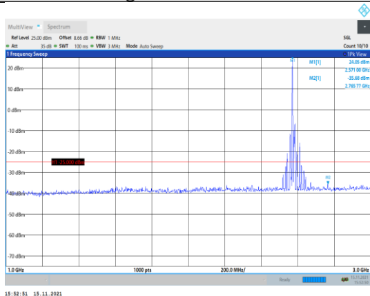
Band38-15MHz-16QAM-37825-1RB#0- Range2:1000~3000MHz
