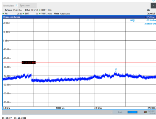
Band38-15MHz-QPSK-38175-1RB#0- Range3:3000~27000MHz
