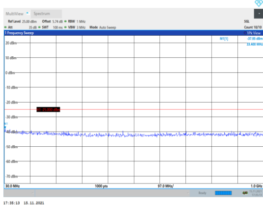
Band41-20MHz-16QAM-41140-1RB#0- Range1:30~1000MHz
