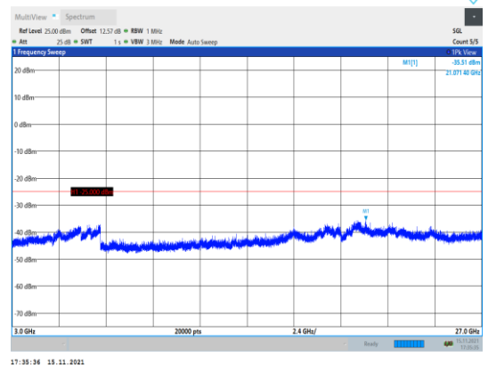
Band41-20MHz-16QAM-41140-1RB#0- Range3:3000~27000MHz
