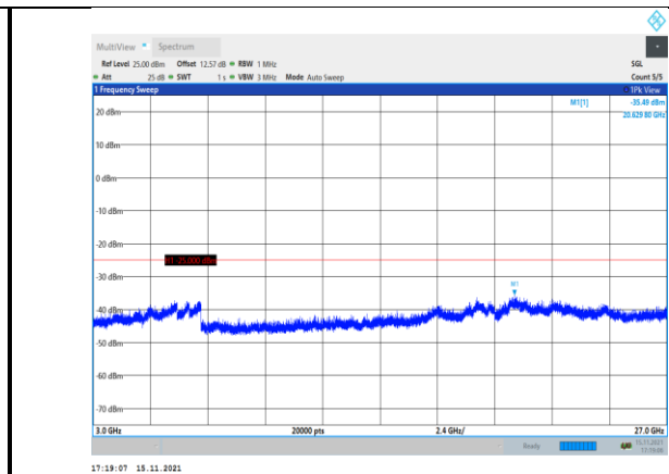
Band41-5MHz-16QAM-40065-1RB#0- Range3:3000~27000MHz
