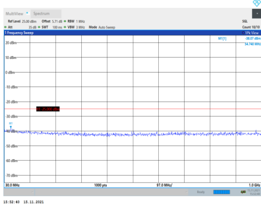
Band38-15MHz-16QAM-37825-1RB#0- Range1:30~1000MHz
