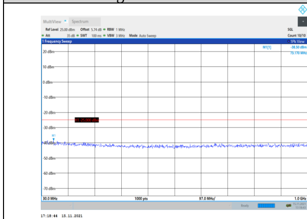
Band41-5MHz-16QAM-40065-1RB#0- Range1:30~1000MHz
