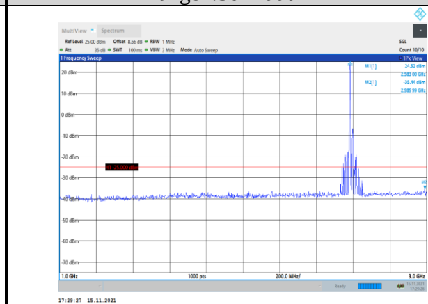
Band41-15MHz-16QAM-40590-1RB#0- Range2:1000~3000MHz
