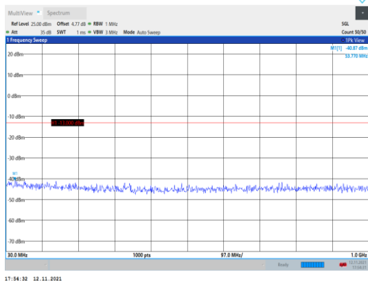
Band66-5MHz-QPSK-132322-1RB#0- Range1:30~1000MHz
