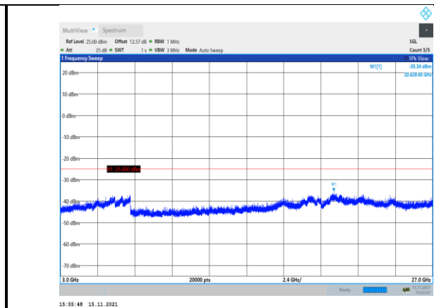
Band38-15MHz-16QAM-38175-1RB#0- Range3:3000~27000MHz
