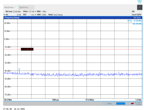
Band66-1.4MHz-QPSK-131979-1RB#0- Range1:30~1000MHz
