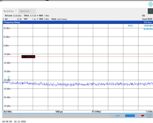
Band66-15MHz-QPSK-132597-1RB#0- Range1:30~1000MHz
