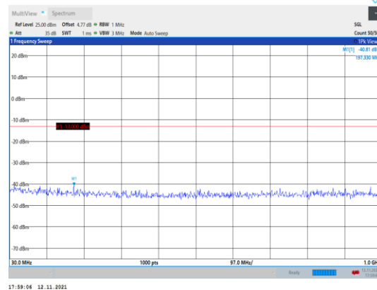
Band66-10MHz-QPSK-132022-1RB#0- Range1:30~1000MHz
