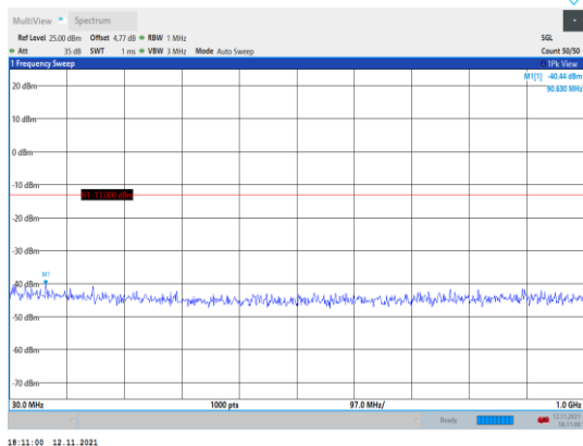
Band66-20MHz-QPSK-132322-1RB#0- Range1:30~1000MHz
