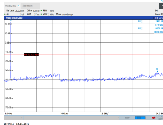
Band66-15MHz-16QAM-132597-1RB#0- Range2:1000~20000MHz
