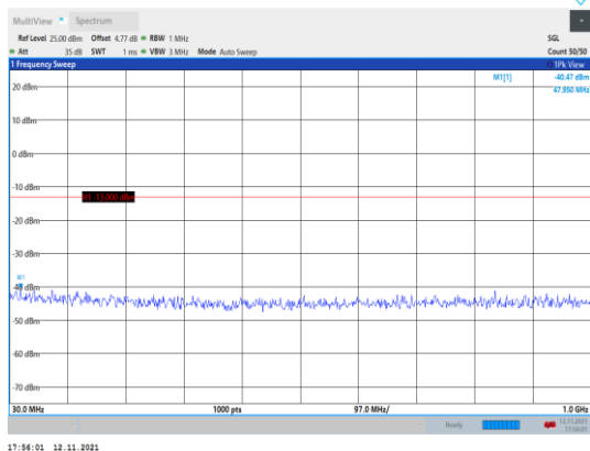
Band66-5MHz-16QAM-132647-1RB#0- Range1:30~1000MHz
