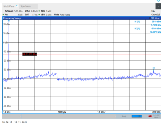
Band66-15MHz-16QAM-132322-1RB#0- Range2:1000~20000MHz
