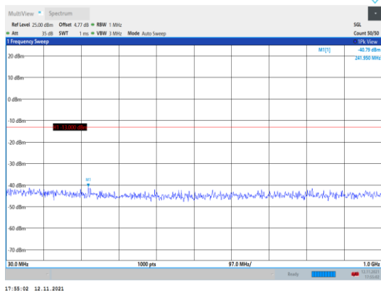
Band66-5MHz-16QAM-132322-1RB#0- Range1:30~1000MHz
