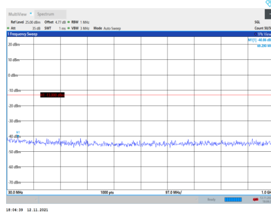
Band66-15MHz-QPSK-132047-1RB#0- Range1:30~1000MHz
