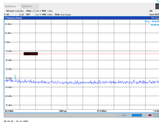
Band66-20MHz-16QAM-132072-1RB#0- Range1:30~1000MHz
