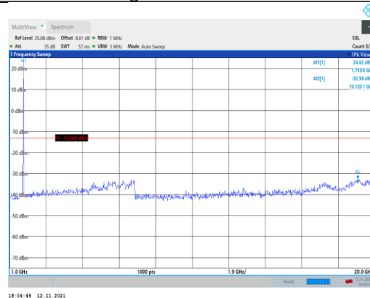
Band66-15MHz-QPSK-132047-1RB#0- Range2:1000~20000MHz
