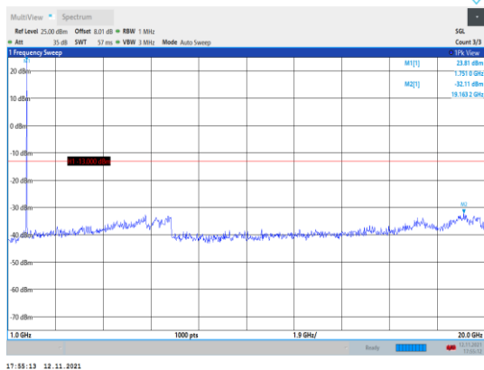
Band66-5MHz-16QAM-132322-1RB#0- Range2:1000~20000MHz
