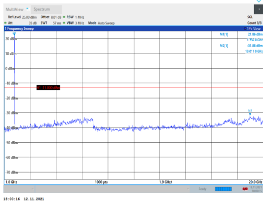
Band66-10MHz-QPSK-132322-1RB#0- Range2:1000~20000MHz
