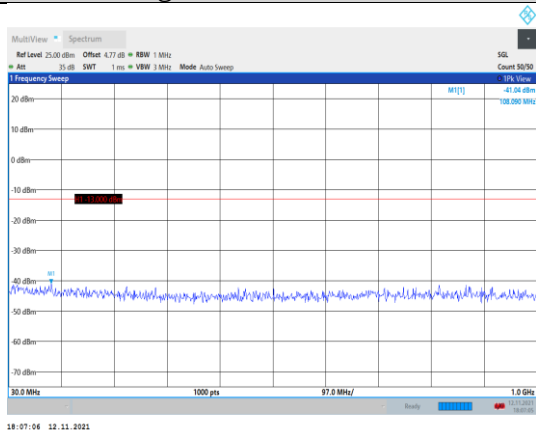
Band66-15MHz-16QAM-132597-1RB#0- Range1:30~1000MHz
