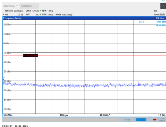
Band66-15MHz-16QAM-132322-1RB#0- Range1:30~1000MHz
