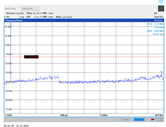
Band66-20MHz-16QAM-132572-1RB#0- Range2:1000~20000MHz
