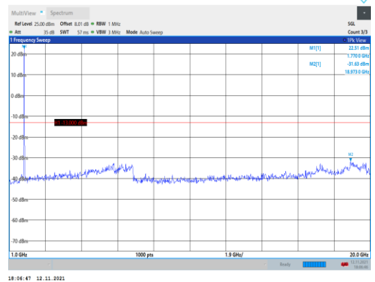
Band66-15MHz-QPSK-132597-1RB#0- Range2:1000~20000MHz
