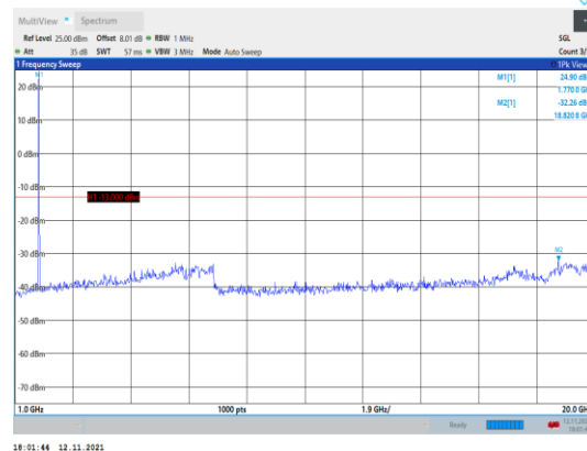
Band66-10MHz-16QAM-132622-1RB#0- Range2:1000~20000MHz
