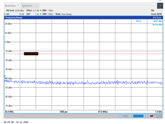
Band66-15MHz-16QAM-132047-1RB#0- Range1:30~1000MHz
