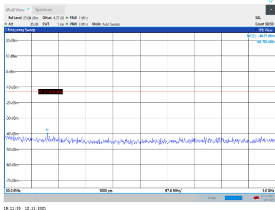
Band66-20MHz-16QAM-132322-1RB#0- Range1:30~1000MHz
