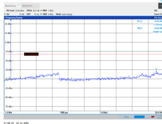
Band66-5MHz-16QAM-132647-1RB#0- Range2:1000~20000MHz
