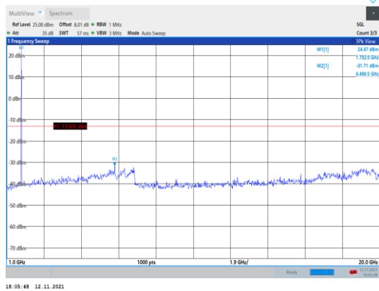
Band66-15MHz-QPSK-132322-1RB#0- Range2:1000~20000MHz
