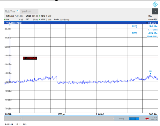
Band66-15MHz-16QAM-132047-1RB#0- Range2:1000~20000MHz
