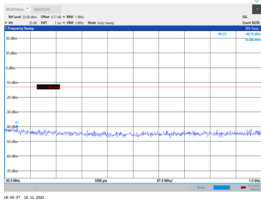
Band66-15MHz-QPSK-132322-1RB#0- Range1:30~1000MHz
