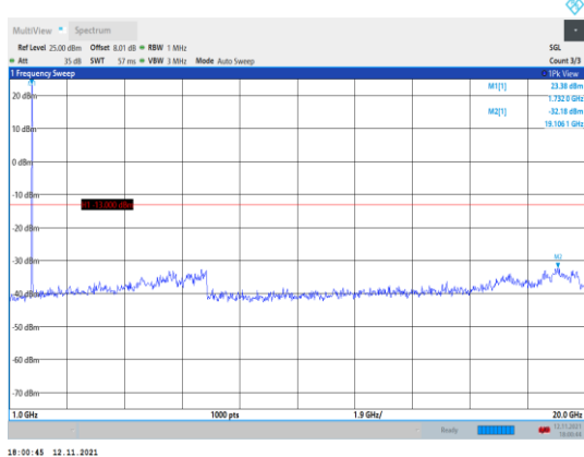
Band66-10MHz-16QAM-132322-1RB#0- Range2:1000~20000MHz
