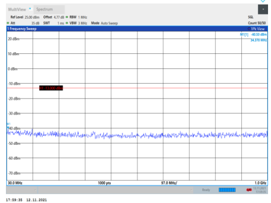
Band66-10MHz-16QAM-132022-1RB#0- Range1:30~1000MHz
