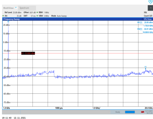
Band66-20MHz-16QAM-132322-1RB#0- Range2:1000~20000MHz
