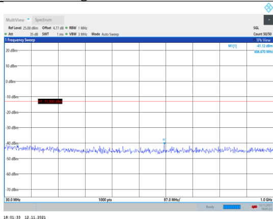
Band66-10MHz-16QAM-132622-1RB#0- Range1:30~1000MHz
