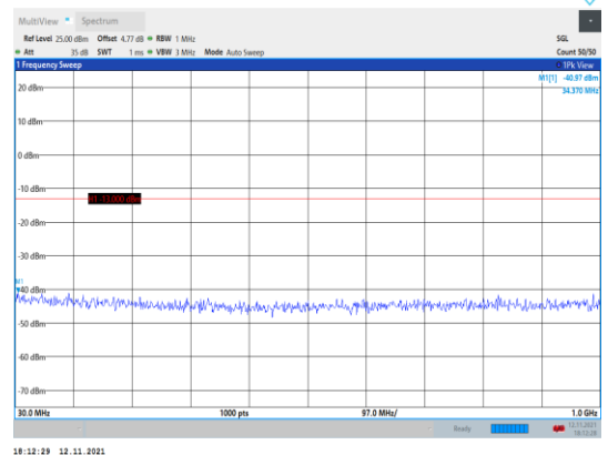
Band66-20MHz-16QAM-132572-1RB#0- Range1:30~1000MHz
