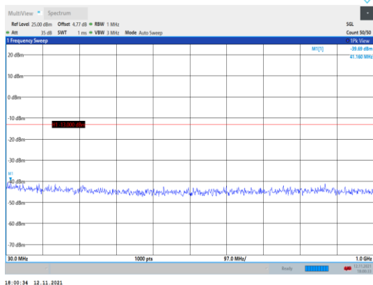
Band66-10MHz-16QAM-132322-1RB#0- Range1:30~1000MHz
