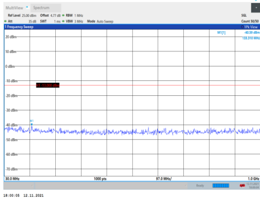
Band66-10MHz-QPSK-132322-1RB#0- Range1:30~1000MHz
