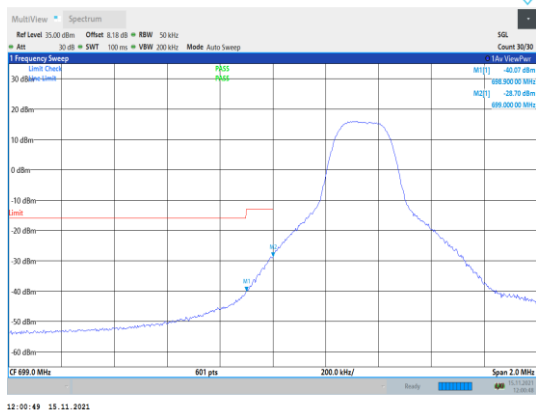
Band12-5MHz-16QAM-23035-1RB#0
