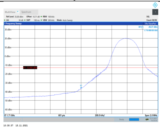
Band4-10MHz-16QAM-20000-1RB#0
