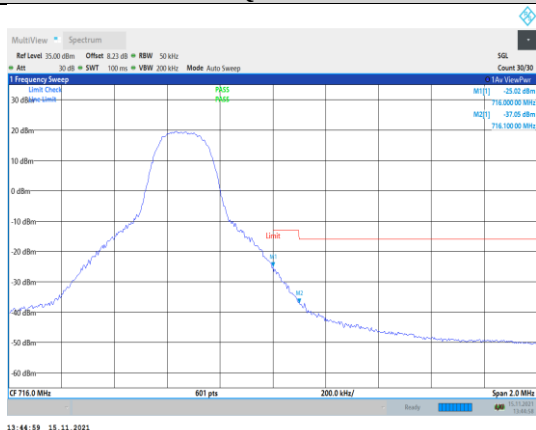
Band17-5MHz-QPSK-23825-1RB#24
