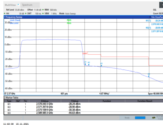
Band7-20MHz-16QAM-21350-100RB#0
