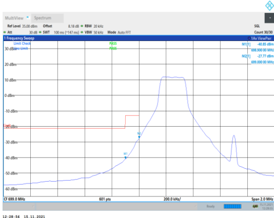
Band12-1.4MHz-16QAM-23017-1RB#0
