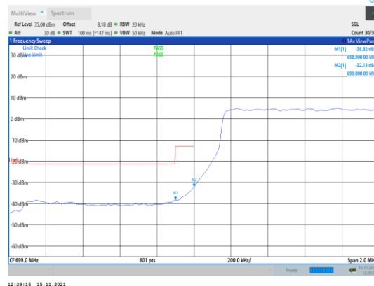
Band12-1.4MHz-QPSK-23017-6RB#0
