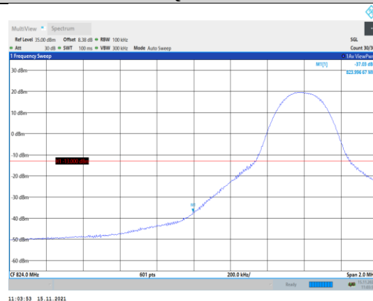
Band5-10MHz-16QAM-20450-1RB#0
