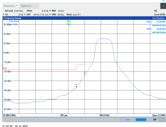
Band12-3MHz-QPSK-23025-1RB#0
