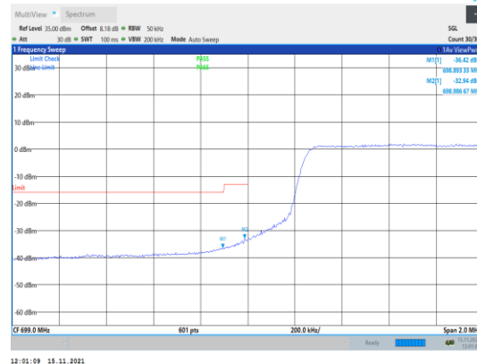
Band12-5MHz-QPSK-23035-25RB#0
