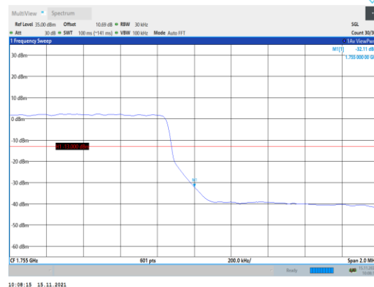
Band4-3MHz-16QAM-20385-15RB#0
