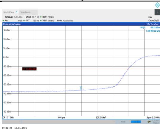
Band4-15MHz-16QAM-20025-75RB#0
