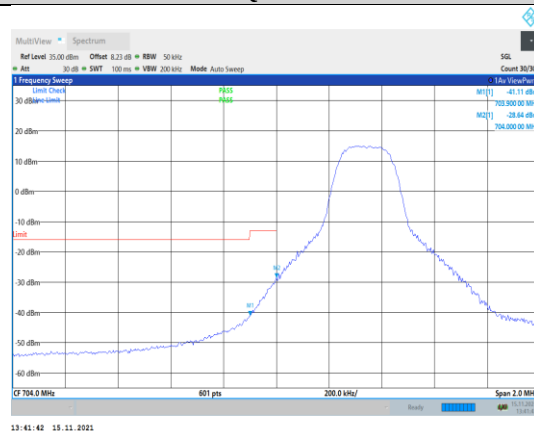
Band17-5MHz-16QAM-23755-1RB#0
