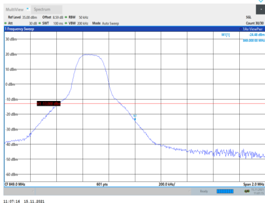
Band5-5MHz-QPSK-20625-1RB#24
