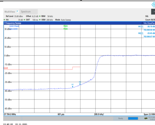
Band17-5MHz-16QAM-23755-25RB#0
