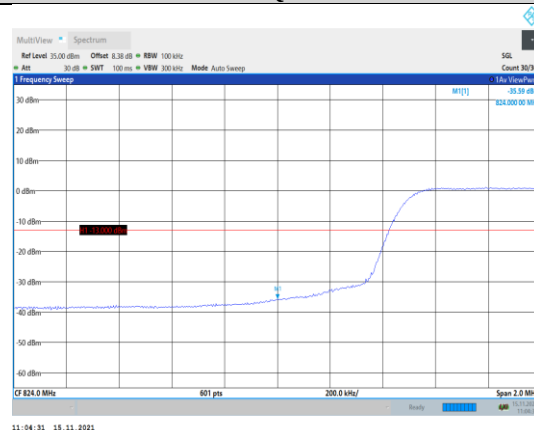
Band5-10MHz-16QAM-20450-50RB#0
