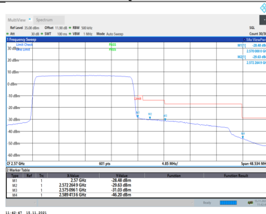
Band7-20MHz-QPSK-21350-100RB#0
