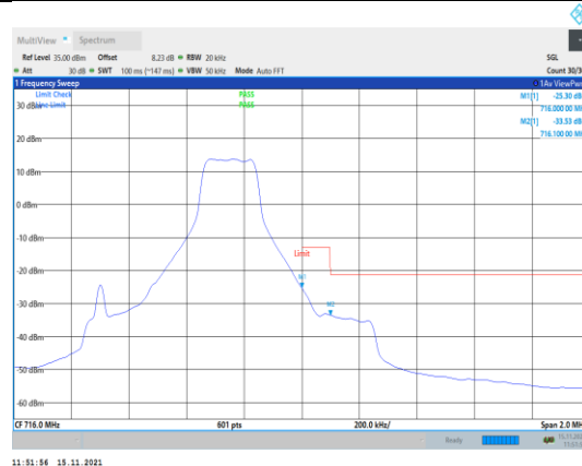
Band12-1.4MHz-16QAM-23173-1RB#5
