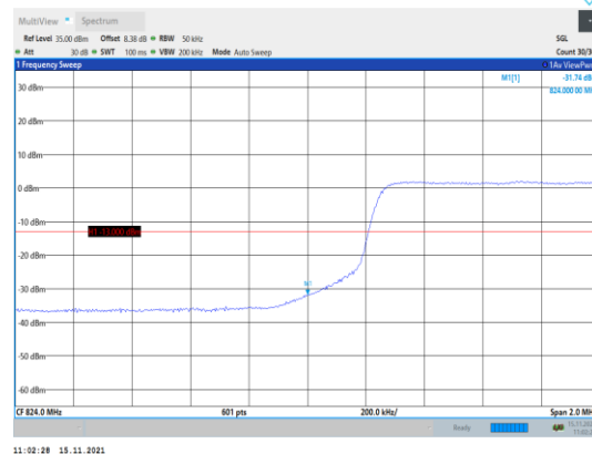
Band5-5MHz-16QAM-20425-25RB#0
