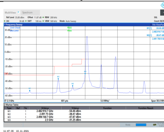
Band7-10MHz-QPSK-20800-1RB#0
