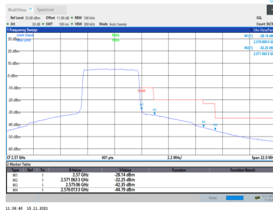
Band7-5MHz-16QAM-21425-25RB#0
