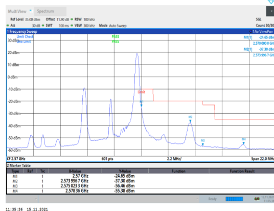
Band7-5MHz-QPSK-21425-1RB#24
