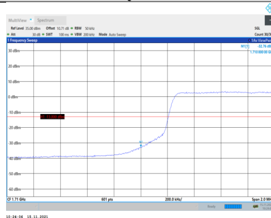
Band4-5MHz-QPSK-19975-25RB#0
