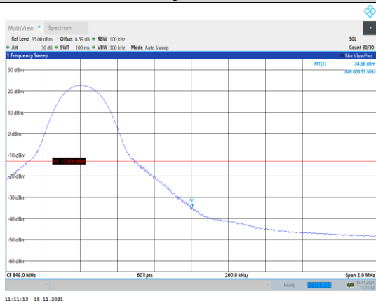
Band5-10MHz-QPSK-20600-1RB#49
