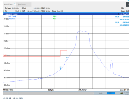
Band12-1.4MHz-QPSK-23017-1RB#0
