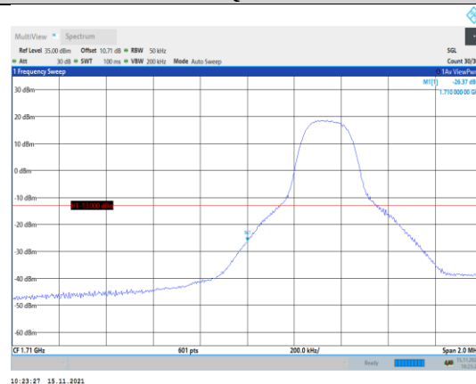
Band4-5MHz-QPSK-19975-1RB#0
