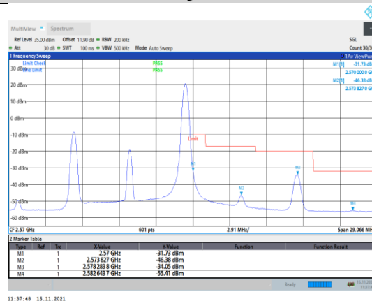
Band7-10MHz-16QAM-21400-1RB#49
