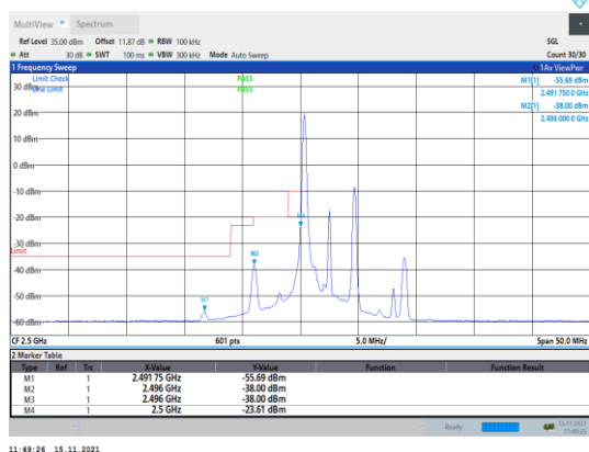
Band7-5MHz-QPSK-20775-1RB#0
