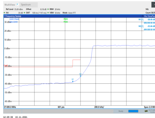
Band12-1.4MHz-16QAM-23017-6RB#0
