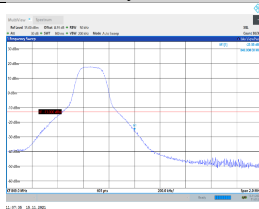
Band5-5MHz-16QAM-20625-1RB#24
