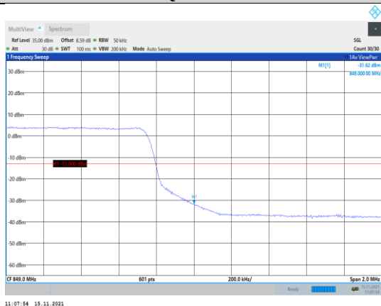
Band5-5MHz-QPSK-20625-25RB#0
