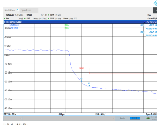
Band12-1.4MHz-16QAM-23173-6RB#0
