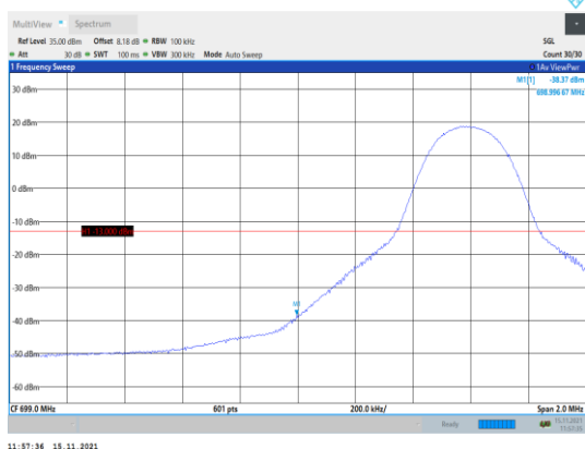
Band12-10MHz-16QAM-23060-1RB#0
