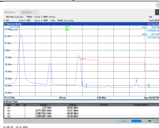
Band7-20MHz-QPSK-21350-1RB#0
