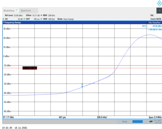
Band4-15MHz-QPSK-20025-1RB#0
