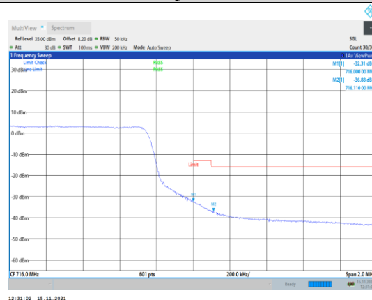
Band12-5MHz-QPSK-23155-25RB#0
