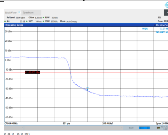
Band5-5MHz-16QAM-20625-25RB#0
