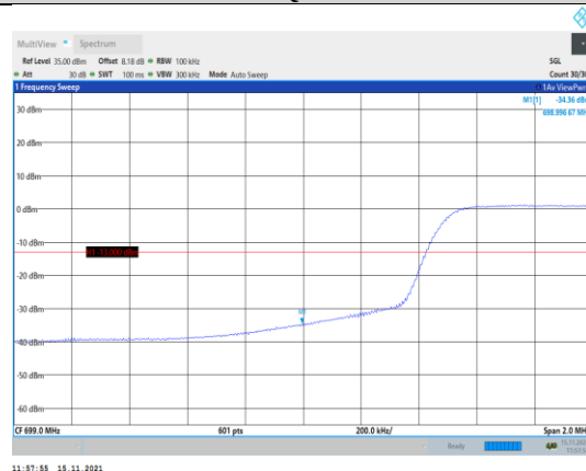
Band12-10MHz-QPSK-23060-50RB#0
