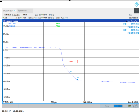
Band12-3MHz-16QAM-23165-15RB#0
