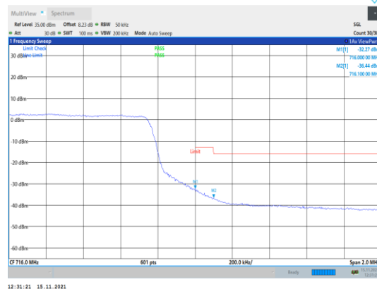
Band12-5MHz-16QAM-23155-25RB#0
