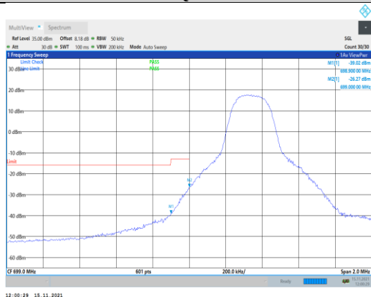
Band12-5MHz-QPSK-23035-1RB#0
