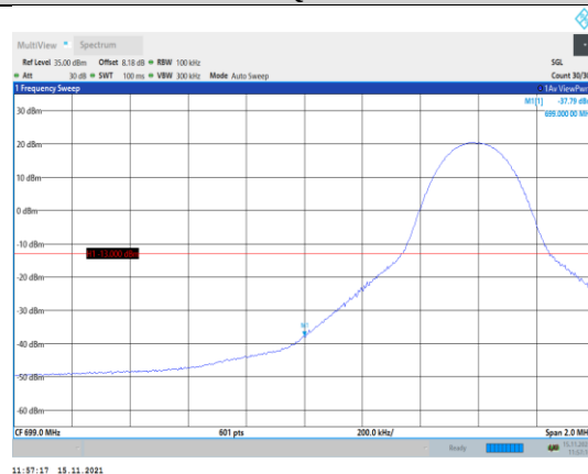
Band12-10MHz-QPSK-23060-1RB#0
