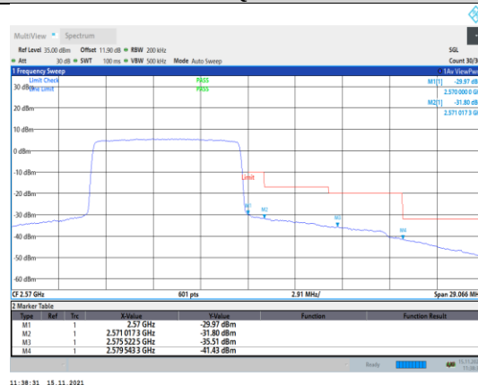
Band7-10MHz-16QAM-21400-50RB#0
