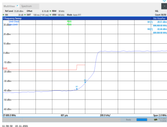
Band12-3MHz-QPSK-23025-15RB#0
