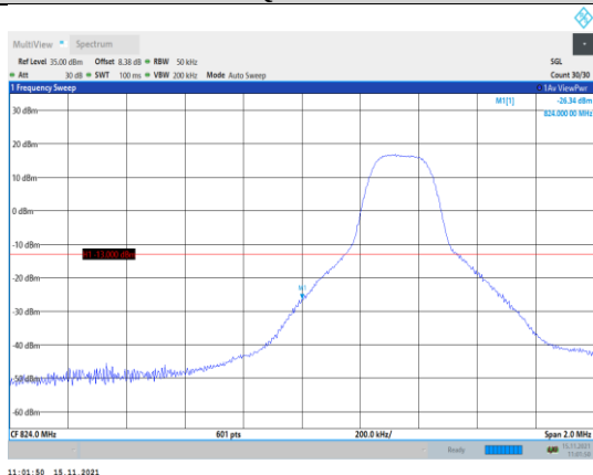
Band5-5MHz-16QAM-20425-1RB#0
