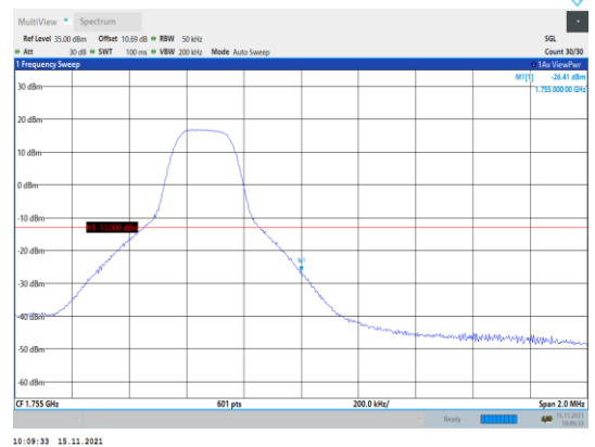
Band4-5MHz-16QAM-20375-1RB#24
