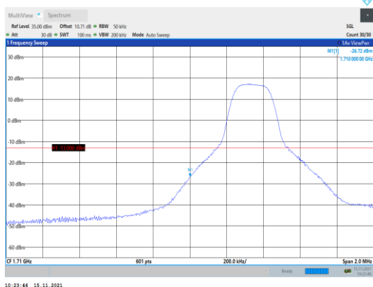
Band4-5MHz-16QAM-19975-1RB#0
