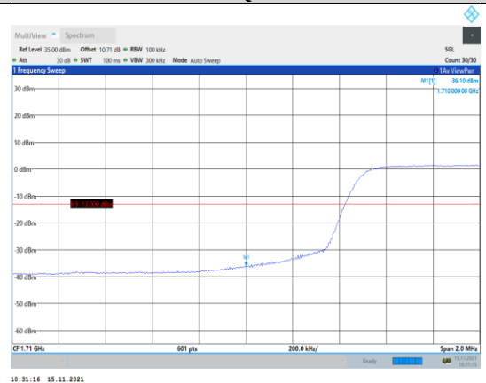
Band4-10MHz-16QAM-20000-50RB#0
