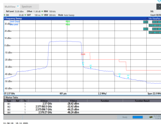
Band7-5MHz-QPSK-21425-25RB#0
