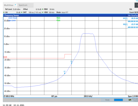
Band12-3MHz-16QAM-23025-1RB#0
