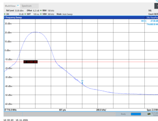
Band12-10MHz-16QAM-23130-1RB#49
