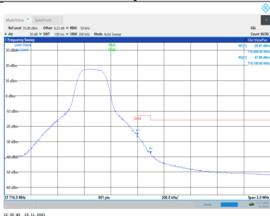
Band12-5MHz-16QAM-23155-1RB#24
