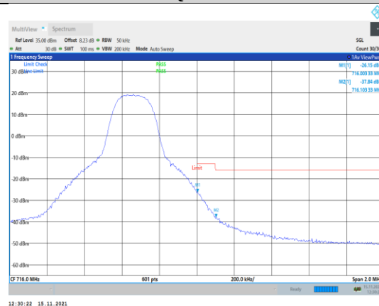
Band12-5MHz-QPSK-23155-1RB#24
