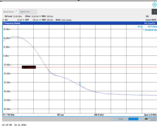
Band4-15MHz-16QAM-20325-1RB#74
