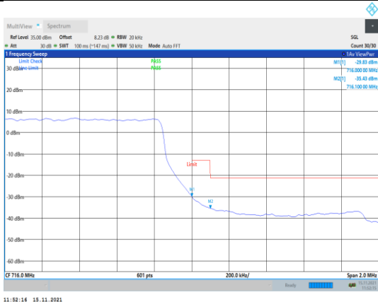
Band12-1.4MHz-QPSK-23173-6RB#0
