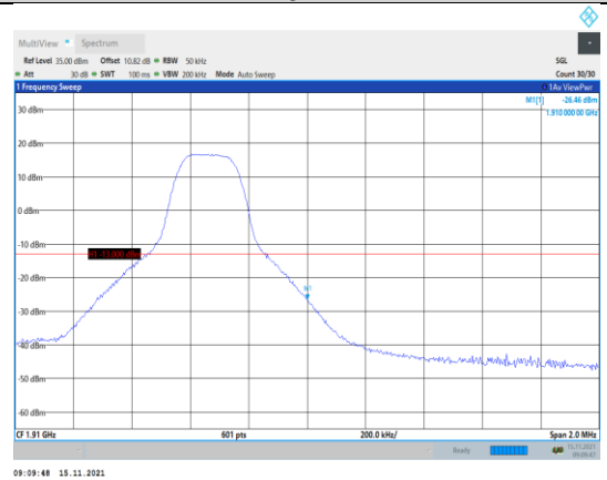
Band2-5MHz-16QAM-19175-1RB#24
