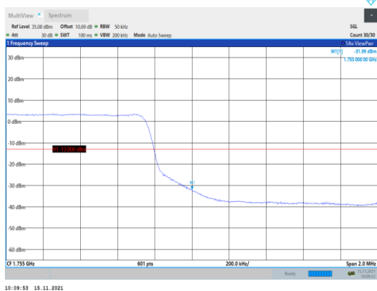
Band4-5MHz-QPSK-20375-25RB#0
