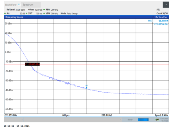
Band4-20MHz-16QAM-20300-1RB#99
