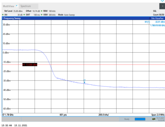
Band66-10MHz-QPSK-132622-50RB#0
