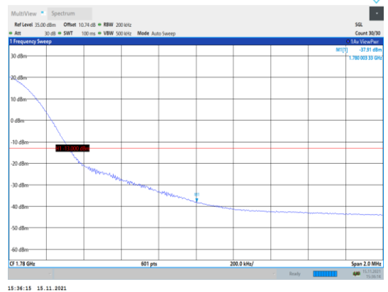
Band66-20MHz-16QAM-132572-1RB#99
