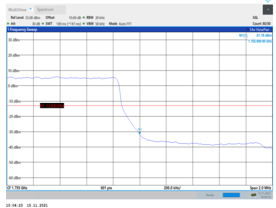
Band4-1.4MHz-QPSK-20393-6RB#0
