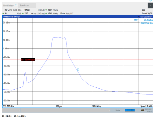
Band4-1.4MHz-16QAM-20393-1RB#5
