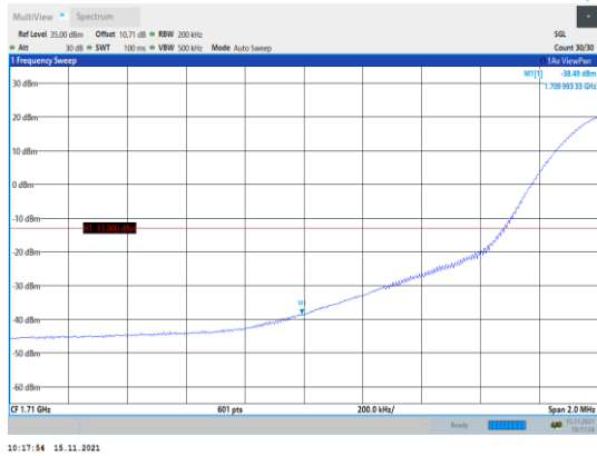
Band4-20MHz-16QAM-20050-1RB#0
