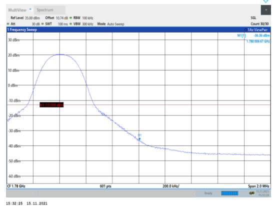
Band66-10MHz-16QAM-132622-1RB#49
