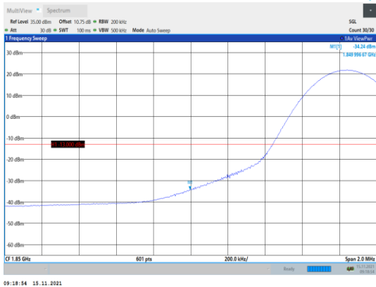
Band2-15MHz-QPSK-18675-1RB#0
