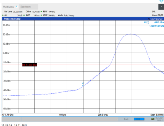
Band66-10MHz-16QAM-132022-1RB#0
