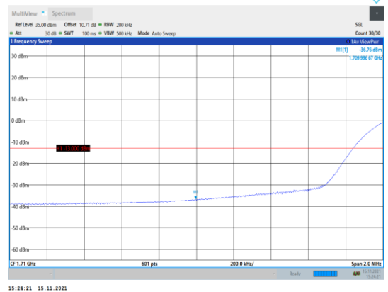
Band66-20MHz-QPSK-132072-100RB#0
