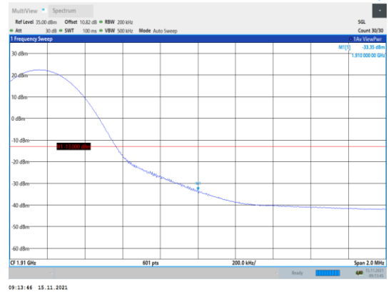
Band2-15MHz-QPSK-19125-1RB#74
