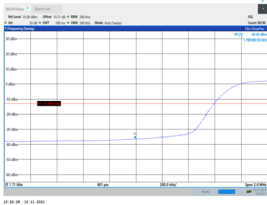
Band4-15MHz-16QAM-20025-75RB#0
