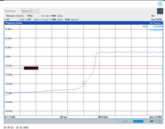
Band4-1.4MHz-16QAM-19957-6RB#0
