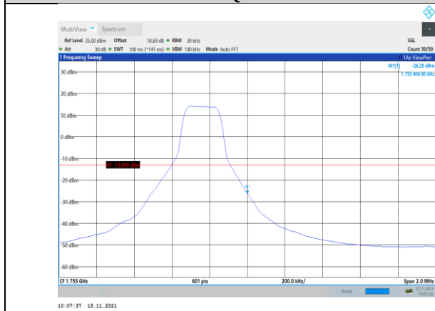
Band4-3MHz-16QAM-20385-1RB#14
