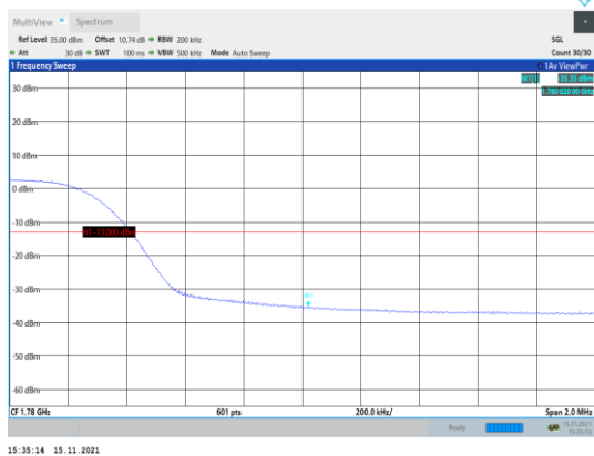
Band66-15MHz-16QAM-132597-75RB#0
