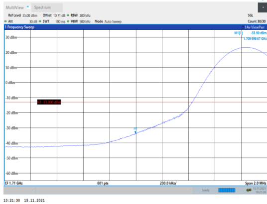
Band4-15MHz-QPSK-20025-1RB#0
