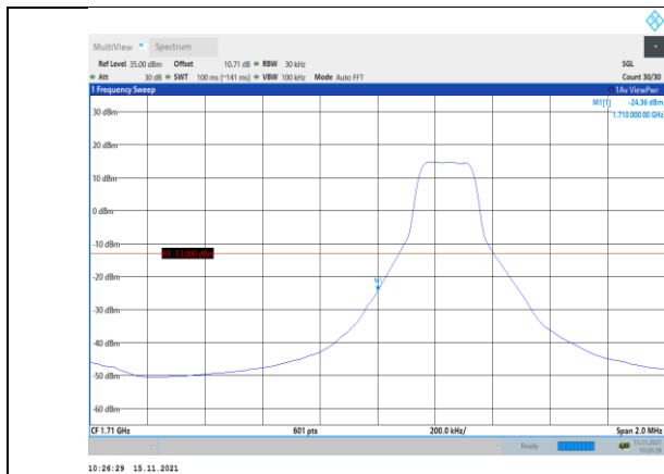
Band4-3MHz-16QAM-19965-1RB#0
