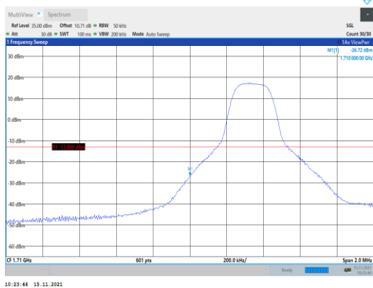
Band4-5MHz-16QAM-19975-1RB#0
