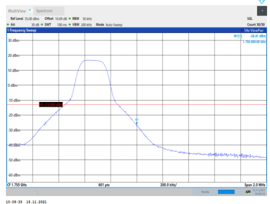
Band4-5MHz-16QAM-20375-1RB#24
