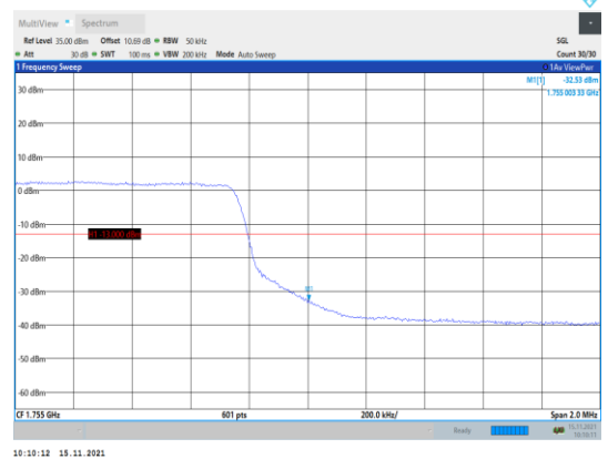
Band4-5MHz-16QAM-20375-25RB#0
