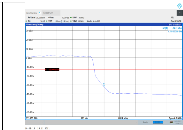
Band4-3MHz-16QAM-20385-15RB#0
