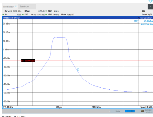
Band2-3MHz-16QAM-19185-1RB#14
