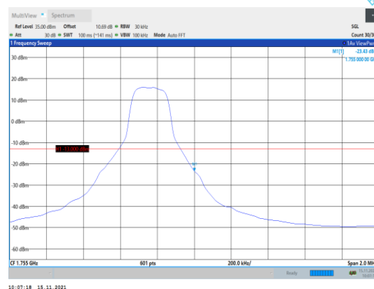
Band4-3MHz-QPSK-20385-1RB#14
