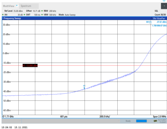
Band66-20MHz-16QAM-132072-1RB#0
