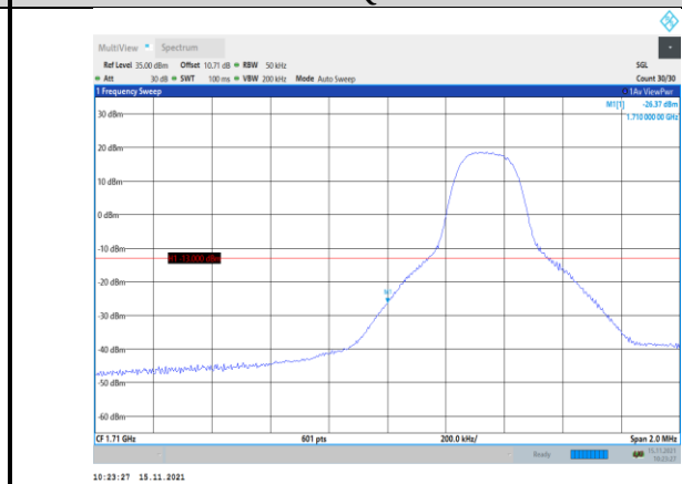
Band4-5MHz-QPSK-19975-1RB#0
