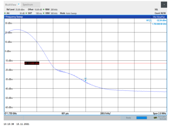
Band4-15MHz-QPSK-20325-1RB#74
