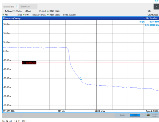
Band4-1.4MHz-16QAM-20393-6RB#0
