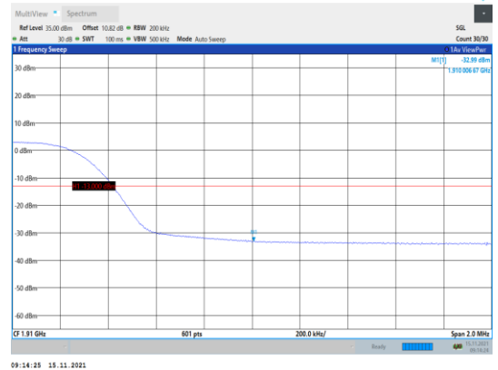
Band2-15MHz-QPSK-19125-75RB#0
