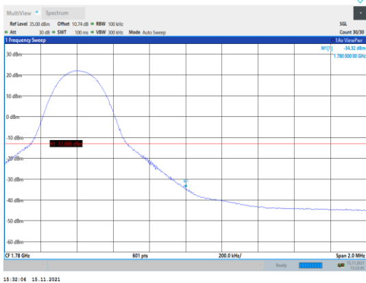
Band66-10MHz-QPSK-132622-1RB#49
