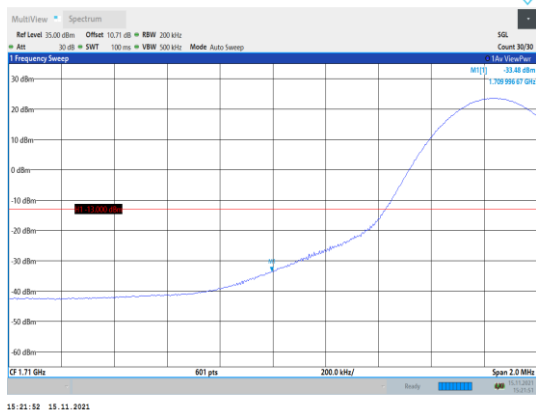
Band66-15MHz-QPSK-132047-1RB#0
