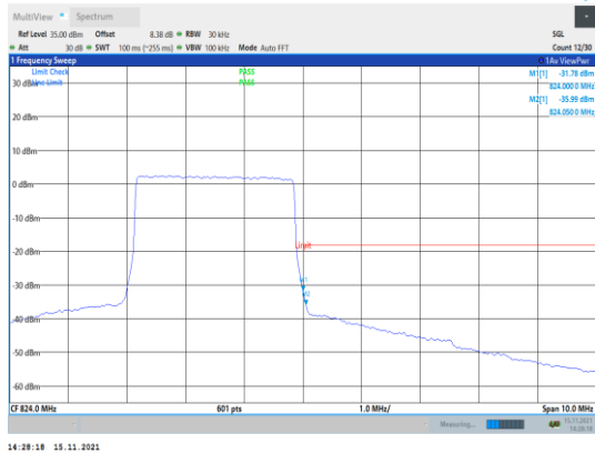
Band26-3MHz-16QAM-26775-15RB#0
