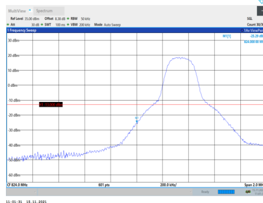
Band5-5MHz-QPSK-20425-1RB#0
