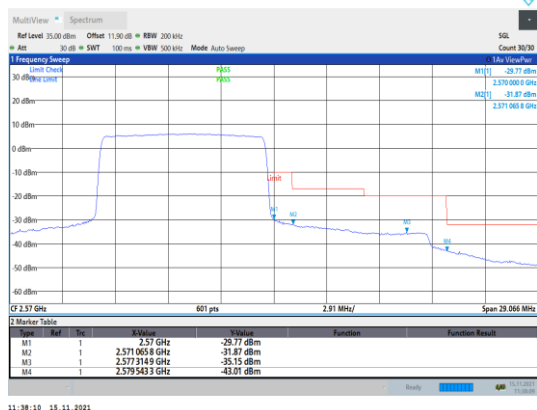
Band7-10MHz-QPSK-21400-50RB#0
