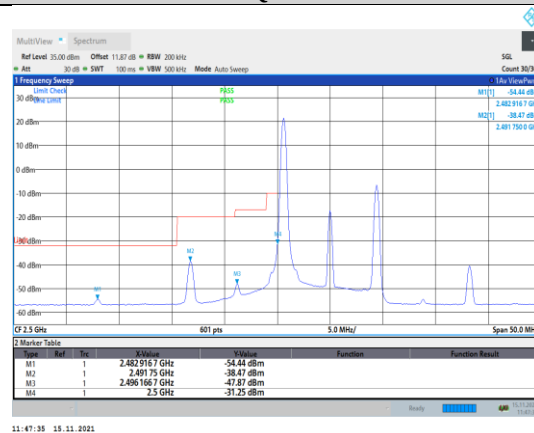
Band7-10MHz-QPSK-20800-1RB#0
