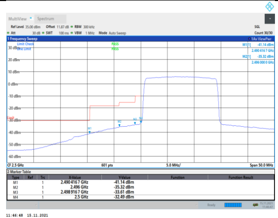
Band7-15MHz-16QAM-20825-75RB#0
