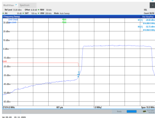
Band26-5MHz-16QAM-26715-25RB#0
