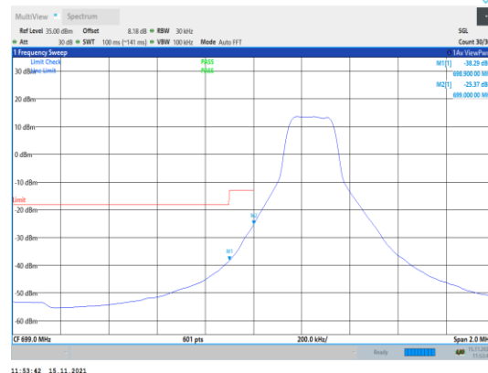
Band12-3MHz-16QAM-23025-1RB#0
