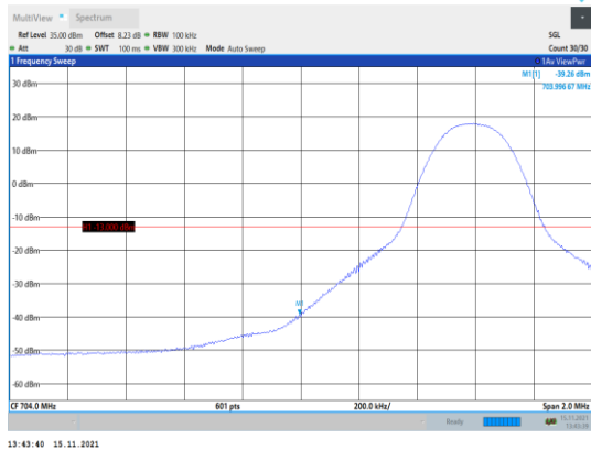
Band17-10MHz-16QAM-23780-1RB#0
