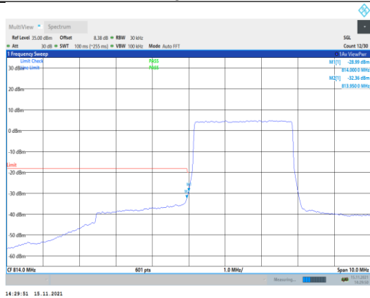
Band26-3MHz-QPSK-26705-15RB#0
