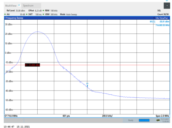
Band17-10MHz-QPSK-23800-1RB#49
