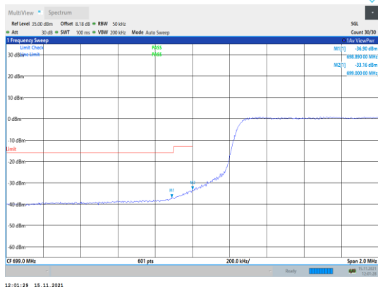
Band12-5MHz-16QAM-23035-25RB#0
