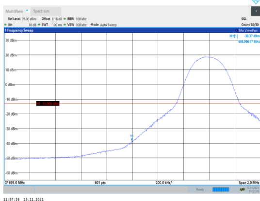
Band12-10MHz-16QAM-23060-1RB#0
