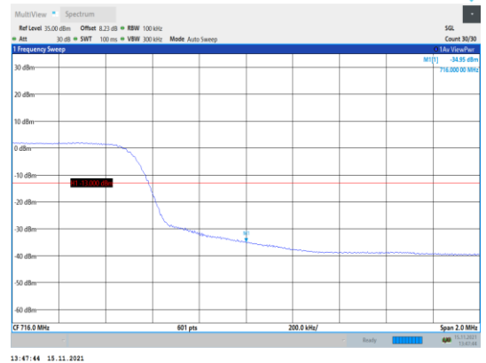
Band17-10MHz-16QAM-23800-50RB#0
