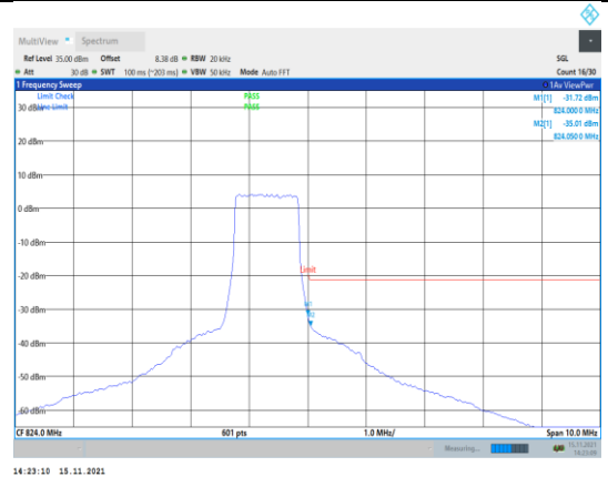
Band26-1.4MHz-16QAM-26783-6RB#0
