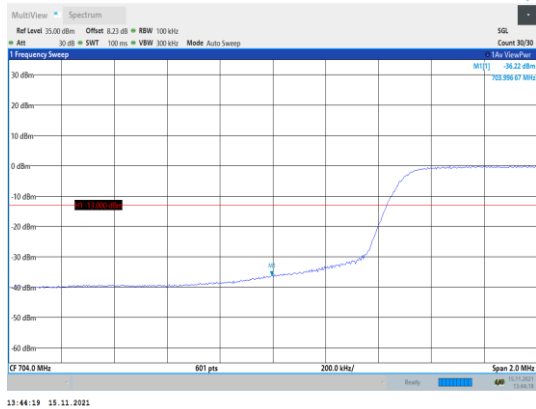
Band17-10MHz-16QAM-23780-50RB#0
