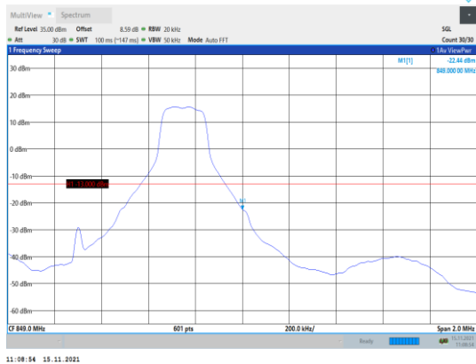
Band5-1.4MHz-QPSK-20643-1RB#5
