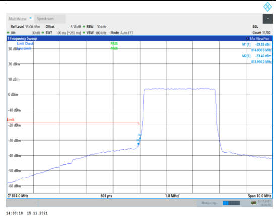
Band26-3MHz-16QAM-26705-15RB#0
