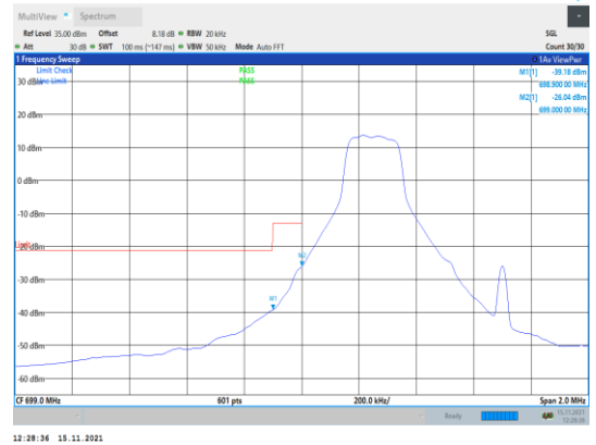
Band12-1.4MHz-QPSK-23017-1RB#0
