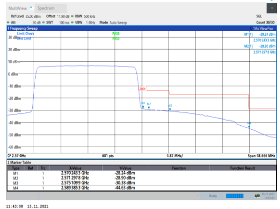
Band7-20MHz-16QAM-21350-100RB#0
