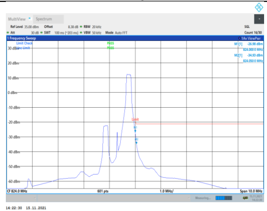
Band26-1.4MHz-16QAM-26783-1RB#5
