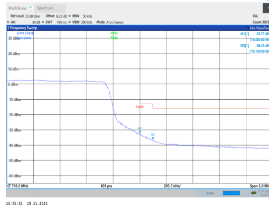
Band12-5MHz-16QAM-23155-25RB#0
