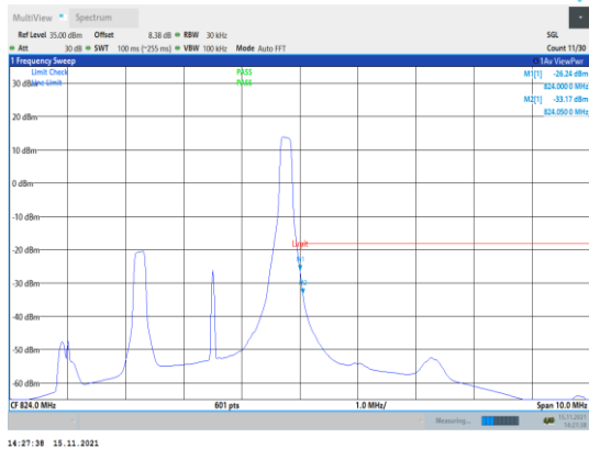
Band26-3MHz-16QAM-26775-1RB#14
