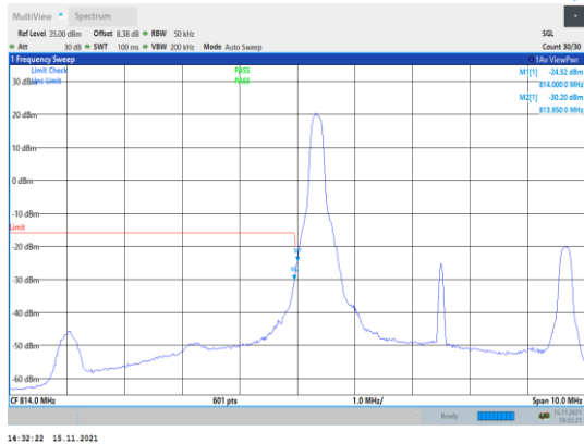
Band26-5MHz-QPSK-26715-1RB#0
