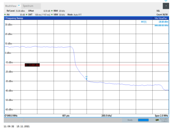
Band5-1.4MHz-QPSK-20643-6RB#0
