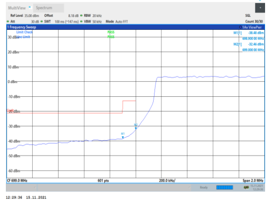
Band12-1.4MHz-16QAM-23017-6RB#0
