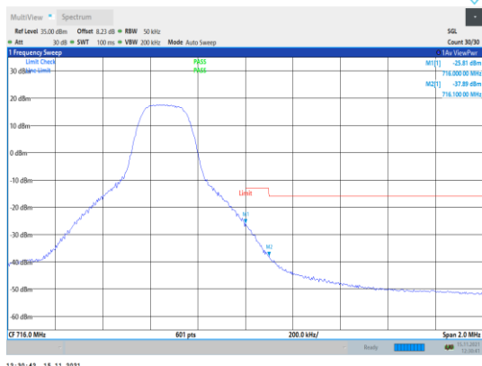
Band12-5MHz-16QAM-23155-1RB#24
