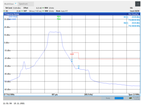
Band12-1.4MHz-16QAM-23173-1RB#5
