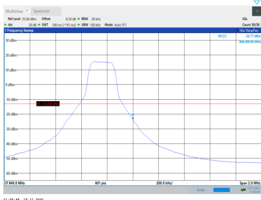
Band5-3MHz-16QAM-20635-1RB#14
