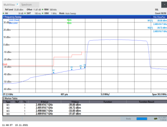
Band7-20MHz-16QAM-20850-100RB#0
