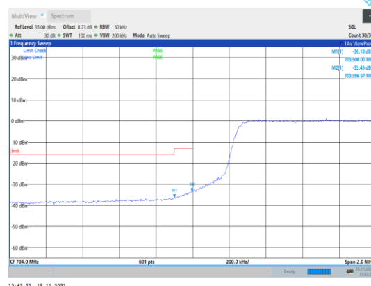
Band17-5MHz-16QAM-23755-25RB#0
