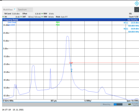
Band26-3MHz-QPSK-26775-1RB#14
