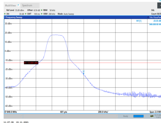
Band5-5MHz-16QAM-20625-1RB#24
