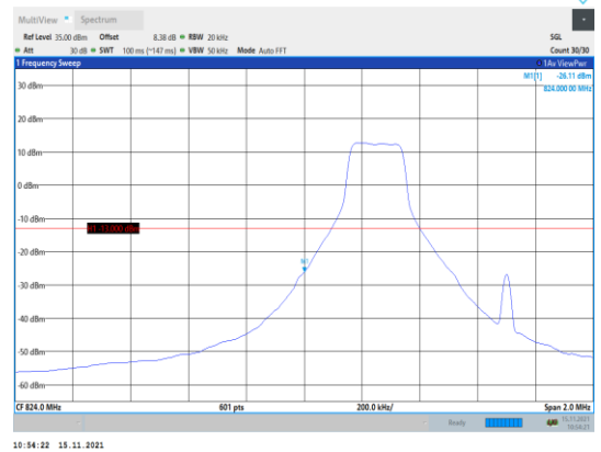
Band5-1.4MHz-16QAM-20407-1RB#0
