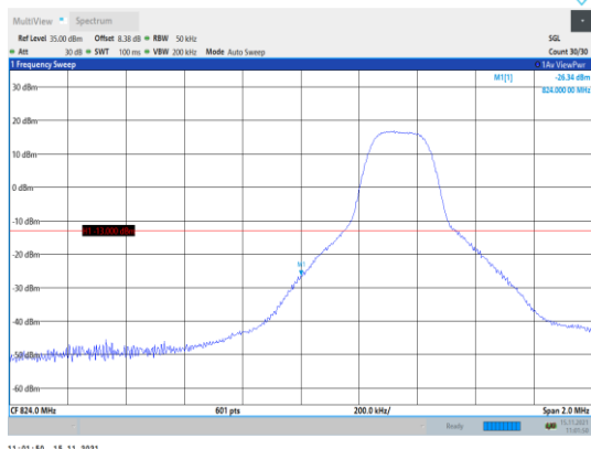
Band5-5MHz-16QAM-20425-1RB#0
