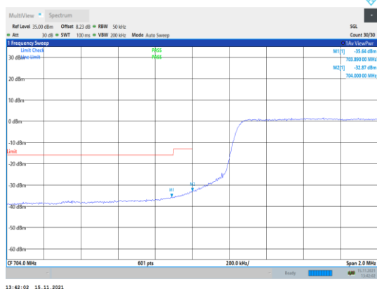
Band17-5MHz-QPSK-23755-25RB#0
