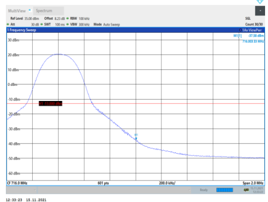
Band12-10MHz-16QAM-23130-1RB#49
