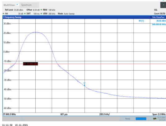
Band5-10MHz-16QAM-20600-1RB#49
