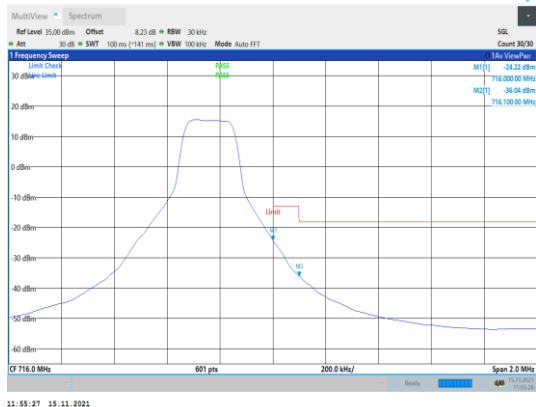
Band12-3MHz-16QAM-23165-1RB#14
