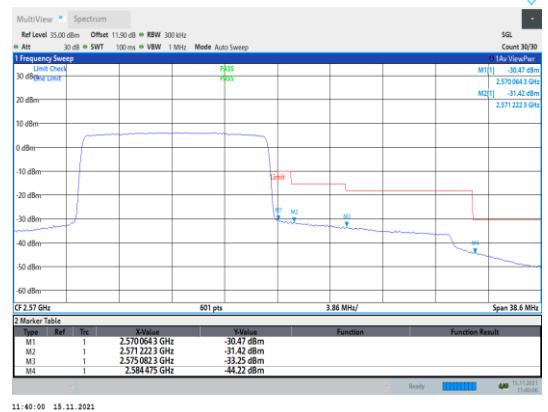
Band7-15MHz-QPSK-21375-75RB#0
