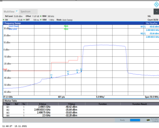
Band7-15MHz-QPSK-20825-75RB#0
