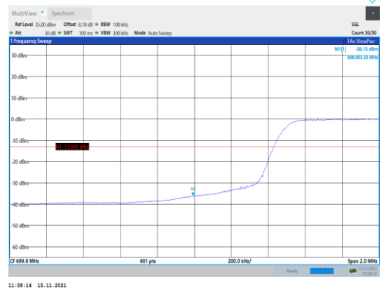
Band12-10MHz-16QAM-23060-50RB#0
