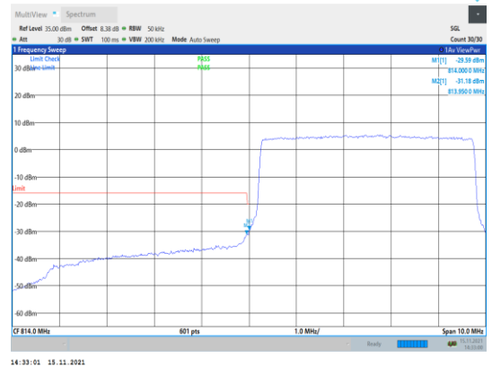
Band26-5MHz-QPSK-26715-25RB#0
