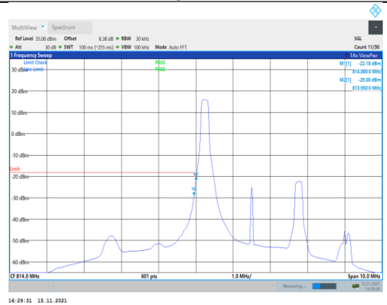
Band26-3MHz-16QAM-26705-1RB#0
