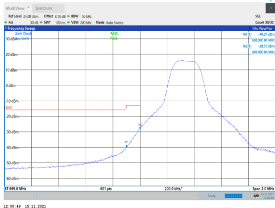
Band12-5MHz-16QAM-23035-1RB#0
