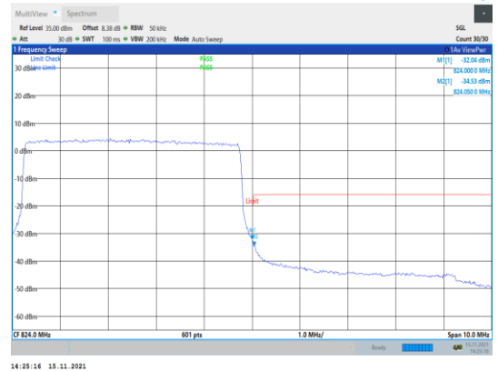
Band26-5MHz-QPSK-26765-25RB#0
