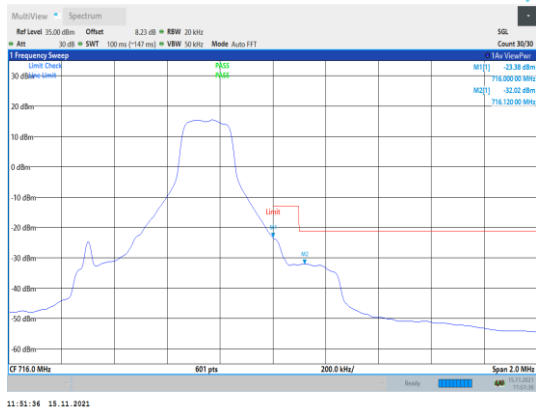
Band12-1.4MHz-QPSK-23173-1RB#5
