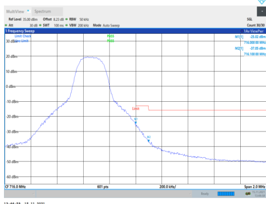
Band17-5MHz-QPSK-23825-1RB#24
