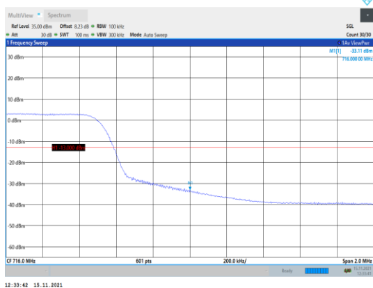
Band12-10MHz-QPSK-23130-50RB#0
