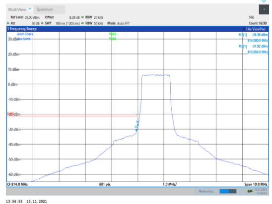
Band26-1.4MHz-16QAM-26697-6RB#0
