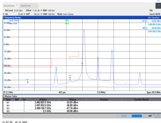
Band7-10MHz-16QAM-20800-1RB#0
