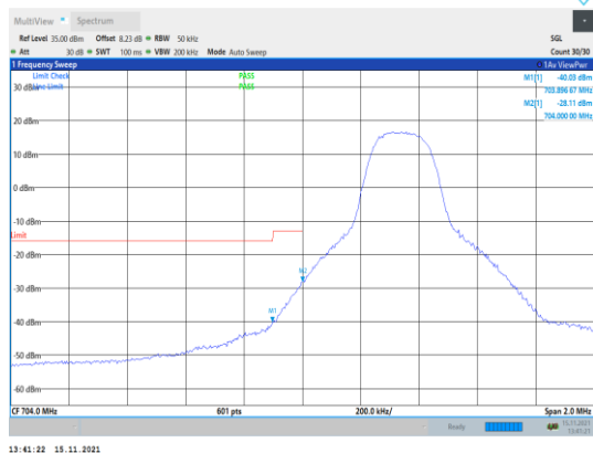
Band17-5MHz-QPSK-23755-1RB#0
