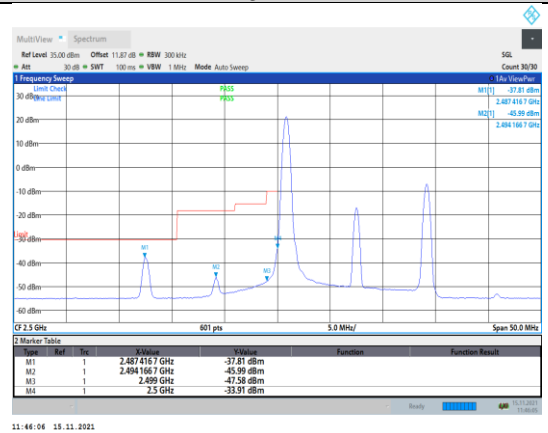
Band7-15MHz-16QAM-20825-1RB#0
