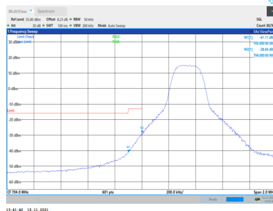
Band17-5MHz-16QAM-23755-1RB#0
