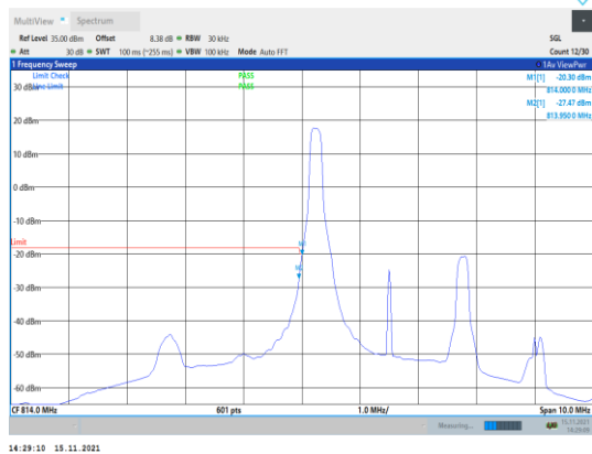
Band26-3MHz-QPSK-26705-1RB#0
