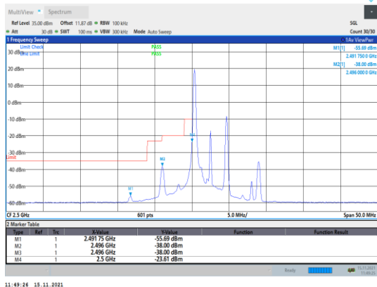
Band7-5MHz-QPSK-20775-1RB#0
