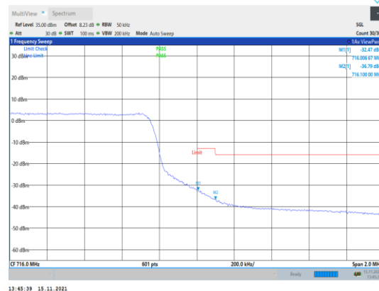
Band17-5MHz-QPSK-23825-25RB#0
