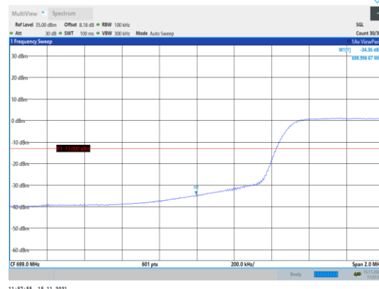
Band12-10MHz-QPSK-23060-50RB#0
