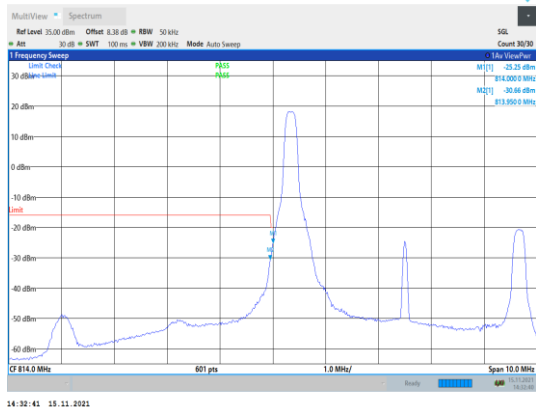
Band26-5MHz-16QAM-26715-1RB#0
