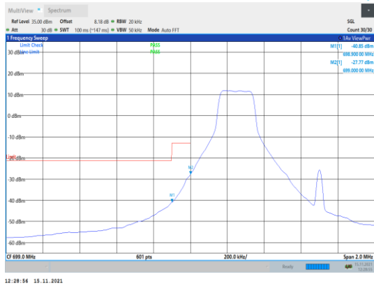
Band12-1.4MHz-16QAM-23017-1RB#0
