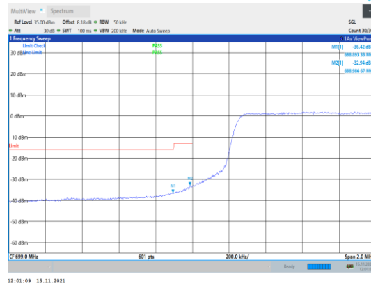
Band12-5MHz-QPSK-23035-25RB#0
