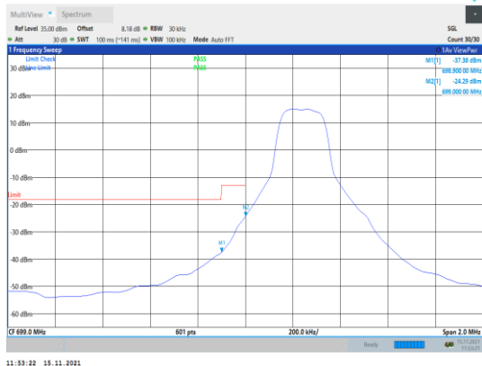
Band12-3MHz-QPSK-23025-1RB#0
