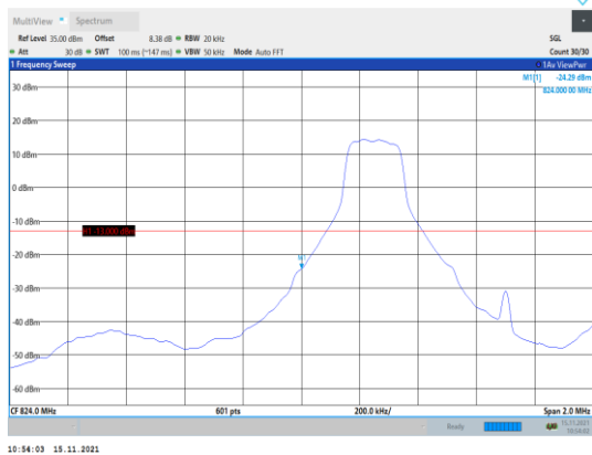
Band5-1.4MHz-QPSK-20407-1RB#0
