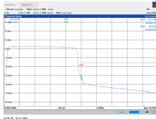
Band26-5MHz-16QAM-26765-25RB#0
