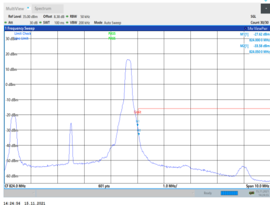
Band26-5MHz-16QAM-26765-1RB#24
