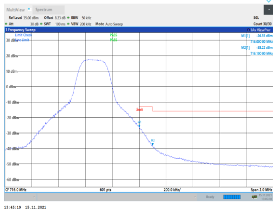
Band17-5MHz-16QAM-23825-1RB#24
