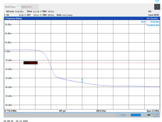
Band12-10MHz-16QAM-23130-50RB#0
