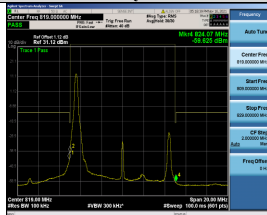
Band26-10MHz-QPSK-26740_Left-1RB#0
