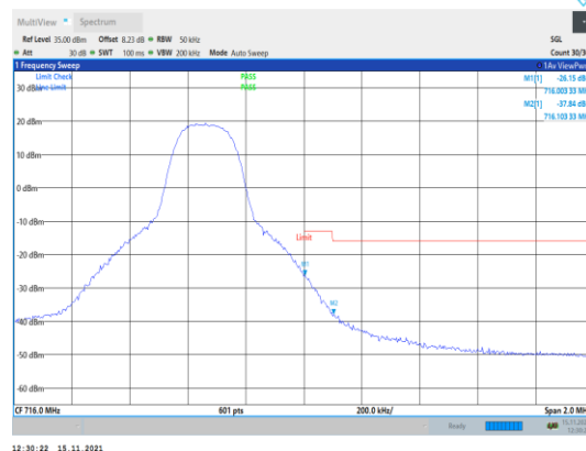
Band12-5MHz-QPSK-23155-1RB#24
