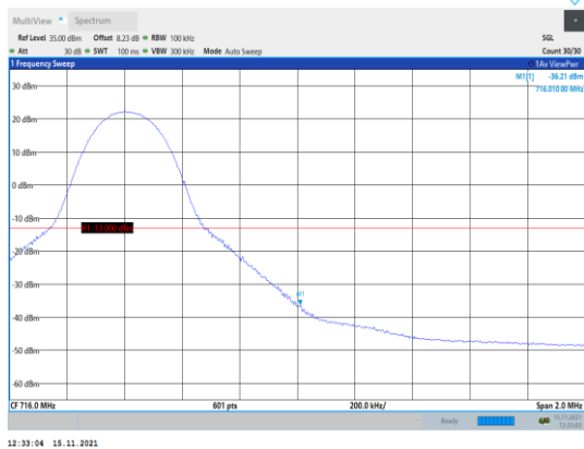
Band12-10MHz-QPSK-23130-1RB#49
