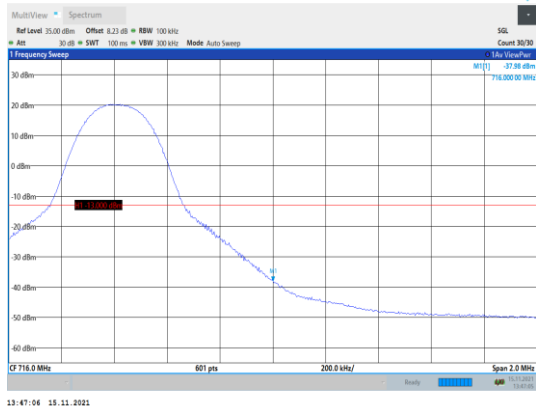
Band17-10MHz-16QAM-23800-1RB#49
