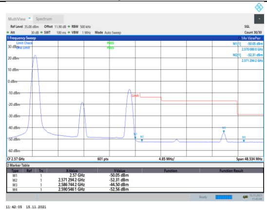
Band7-20MHz-QPSK-21350-1RB#0
