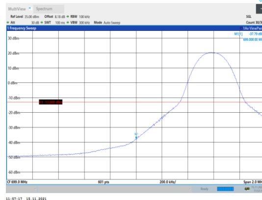
Band12-10MHz-QPSK-23060-1RB#0
