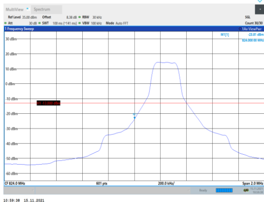
Band5-3MHz-16QAM-20415-1RB#0
