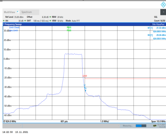
Band26-1.4MHz-QPSK-26783-6RB#0
