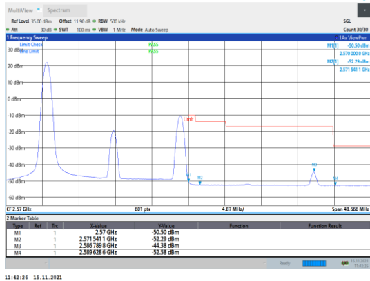
Band7-20MHz-16QAM-21350-1RB#0
