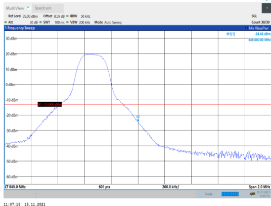
Band5-5MHz-QPSK-20625-1RB#24
