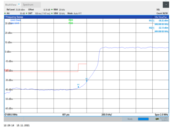
Band12-1.4MHz-QPSK-23017-6RB#0
