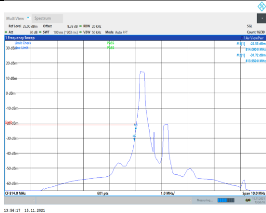
Band26-1.4MHz-16QAM-26697-1RB#0
