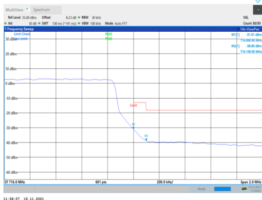
Band12-3MHz-16QAM-23165-15RB#0
