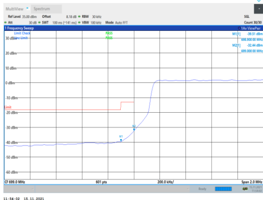
Band12-3MHz-QPSK-23025-15RB#0
