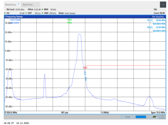
Band26-5MHz-QPSK-26765-1RB#24
