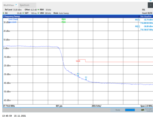
Band17-5MHz-16QAM-23825-25RB#0
