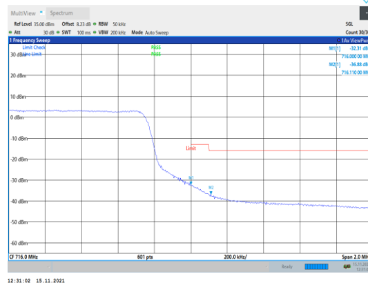
Band12-5MHz-QPSK-23155-25RB#0
