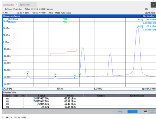
Band7-20MHz-16QAM-20850-1RB#99
