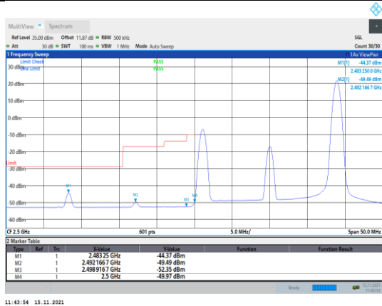
Band7-20MHz-QPSK-20850-1RB#99
