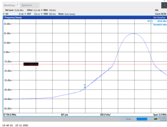
Band17-10MHz-QPSK-23780-1RB#0
