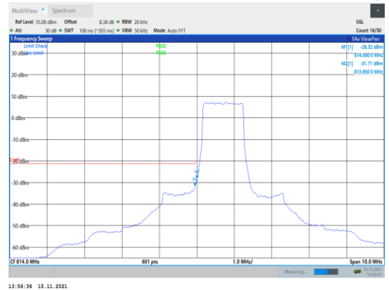
Band26-1.4MHz-QPSK-26697-6RB#0
