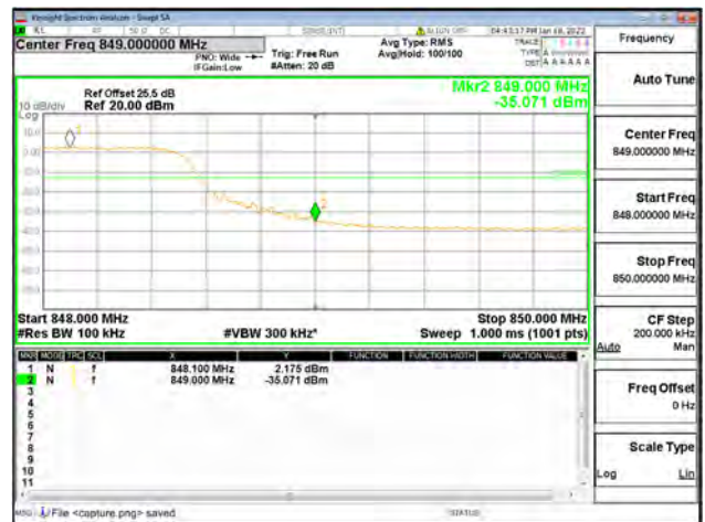
Band5 / 10MHz / High CH / QPSK / FULL RB
