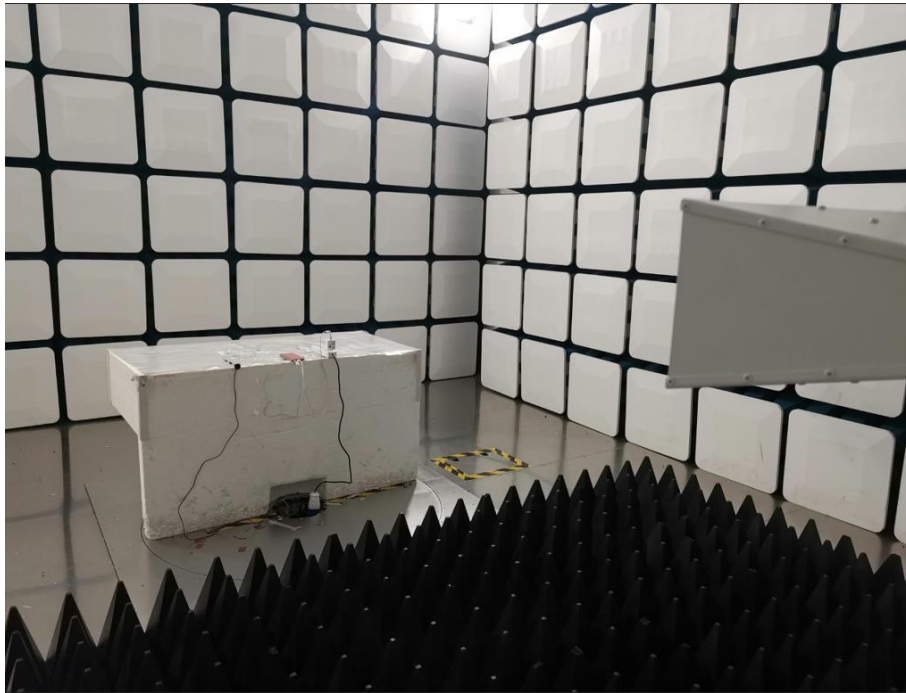
Above 1GHz-RF
