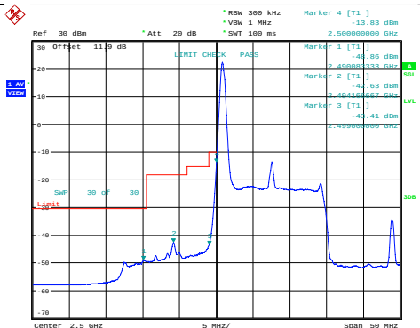
Band7-15MHz-QPSK-20825-1RB#0
