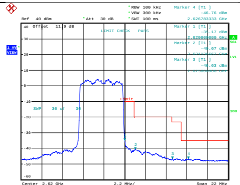
Band38-5MHz-QPSK-38225-25RB#0
