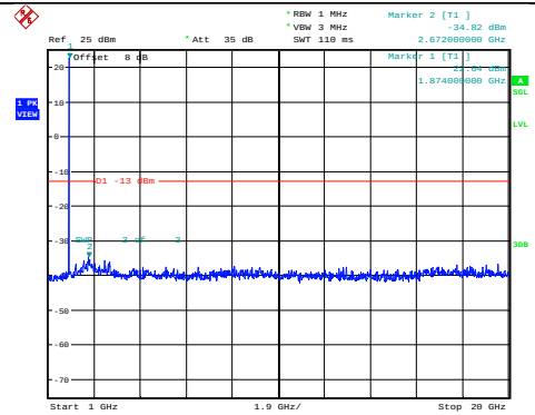
Band2-5MHz-64QAM-18900-1RB#0- Range2:1000~20000MHz
