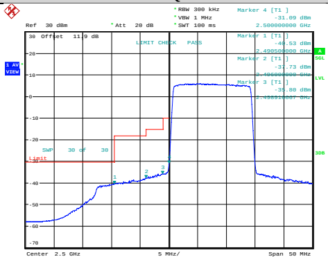
Band7-15MHz-QPSK-20825-1RB#0
