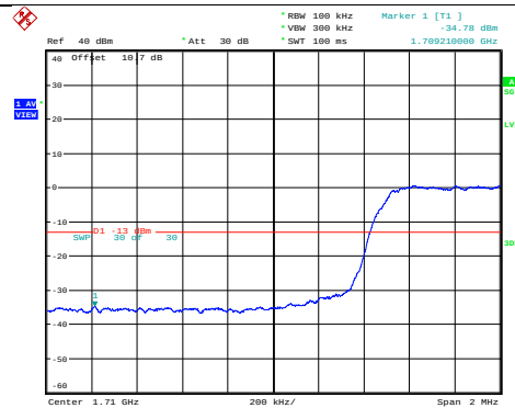
Band66-10MHz-64QAM-132022-50RB#0
