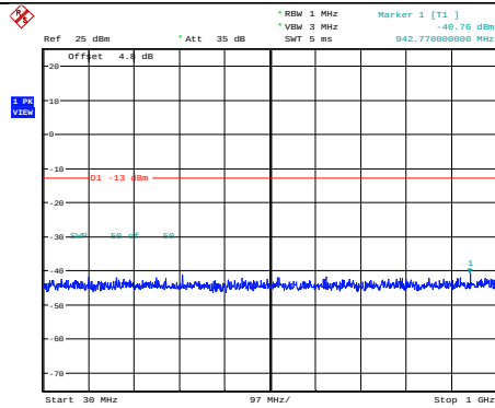
Band2-5MHz-64QAM-18625-1RB#0- Range1:30~1000MHz
