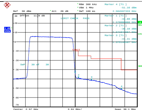
Band7-15MHz-QPSK-21375-75RB#0
