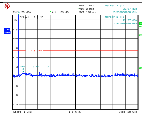
Band2-3MHz-16QAM-18900-1RB#0- Range2:1000~20000MHz
