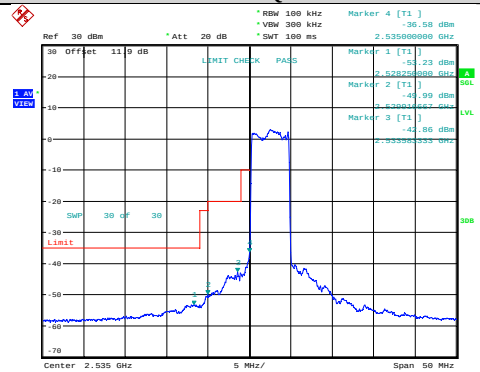
Band41-5MHz-16QAM-40065-1RB#0
