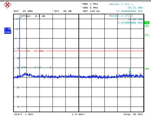
Band2-5MHz-16QAM-18900-1RB#0-Range2:1000~20000MHz
