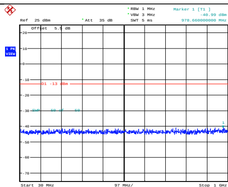
Band2-3MHz-16QAM-18615-1RB#0- Range1:30~1000MHz
