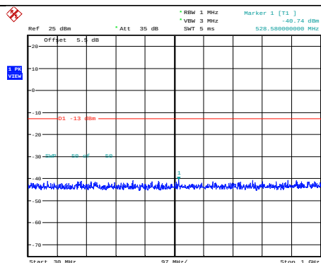
Band2-3MHz-QPSK-18615-1RB#0-Range1:30~1000MHz
