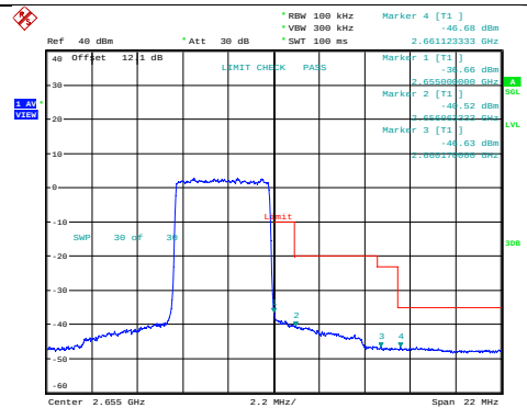
Band41-5MHz-QPSK-41215-25RB#0
