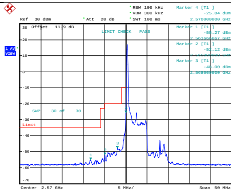
Band38-5MHz-QPSK-37775-1RB#0
