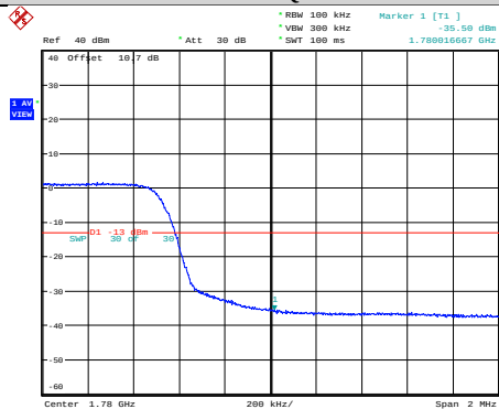
Band66-10MHz-16QAM-132622-1RB#49
