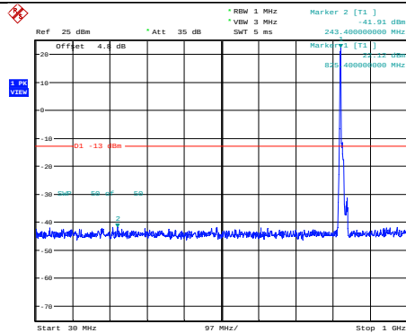
Band5-10MHz-64QAM-20450-1RB#0- Range1:30~1000MHz
