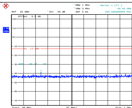
Band4-1.4MHz-QPSK-19957-1RB#0- Range1:30~1000MHz
