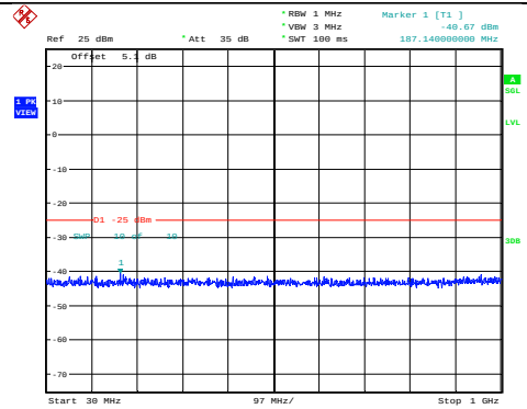
Band7-5MHz-64QAM-21100-1RB#0- Range1:30~1000MHz
