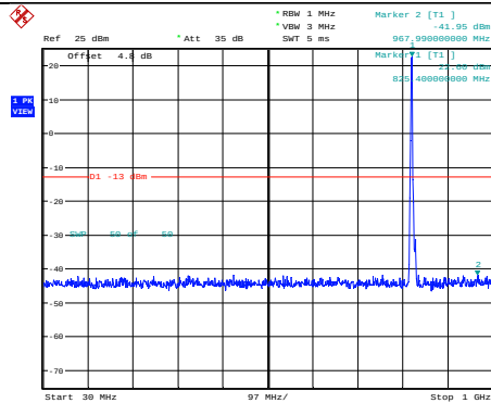
Band5-5MHz-64QAM-20425-1RB#0- Range1:30~1000MHz
