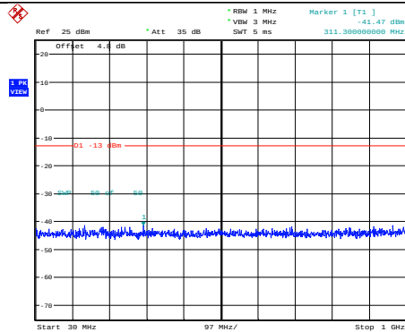
Band4-5MHz-64QAM-19975-1RB#0- Range1:30~1000MHz
