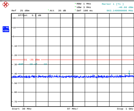
Band7-5MHz-64QAM-20775-1RB#0- Range1:30~1000MHz
