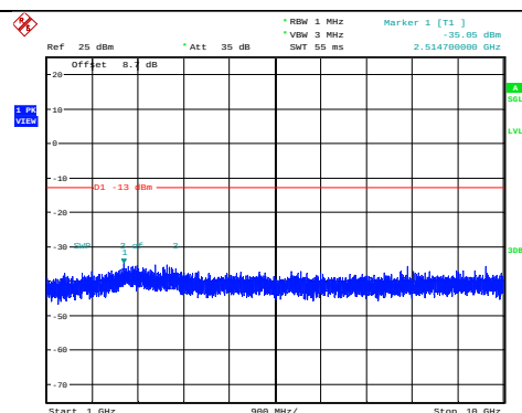
Band12-3MHz-QPSK-23095-1RB#0- Range2:1000~10000MHz
