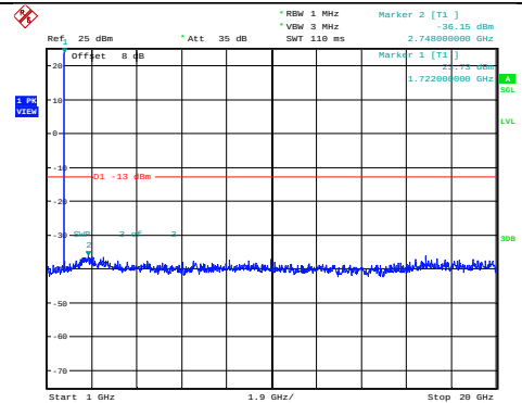
Band4-3MHz-64QAM-20175-1RB#0- Range2:1000~20000MHz
