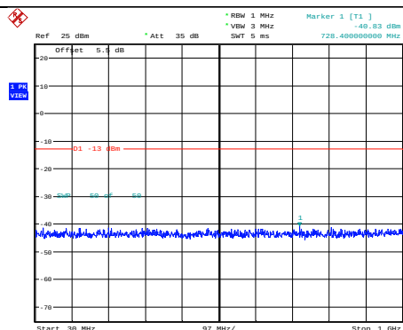
Band4-15MHz-16QAM-20025-1RB#0- Range1:30~1000MHz
