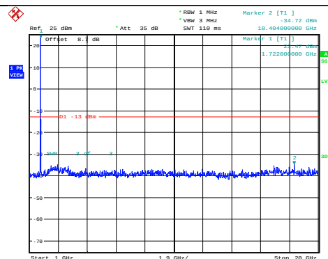
Band4-15MHz-16QAM-20175-1RB#0- Range2:1000~20000MHz
