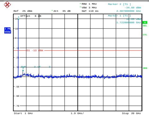
Band4-1.4MHz-64QAM-20175-1RB#0-Range2:1000~20000MHz
