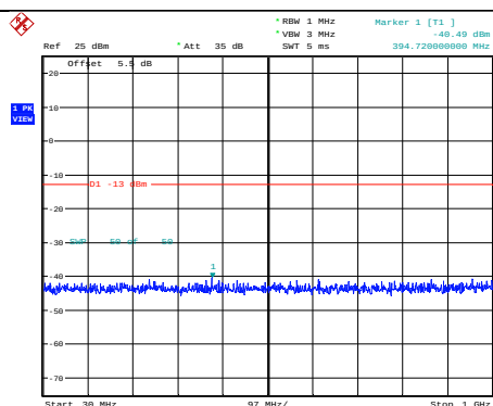
Band4-5MHz-QPSK-19975-1RB#0- Range1:30~1000MHz
