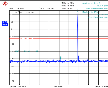
Band12-1.4MHz-64QAM-23017-1RB#0- Range1:30~1000MHz
