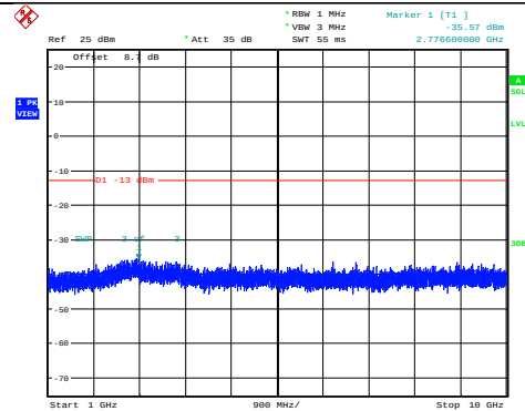
Band12-1.4MHz-64QAM-23095-1RB#0- Range2:1000~10000MHz
