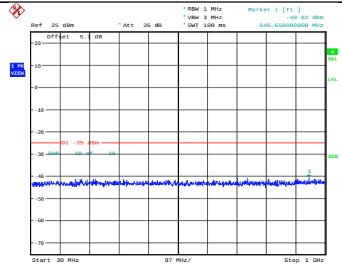
Band7-20MHz-64QAM-20850-1RB#0- Range1:30~1000MHz
