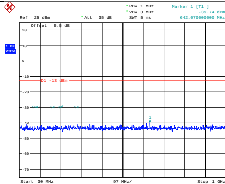
Band4-3MHz-16QAM-19965-1RB#0-Range1:30~1000MHz
