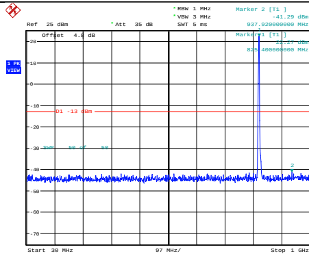
Band5-3MHz-64QAM-20415-1RB#0-Range1:30~1000MHz
