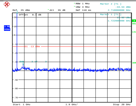
Band4-3MHz-16QAM-20175-1RB#0-Range2:1000~20000MHz
