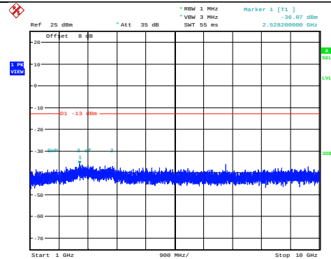
Band5-5MHz-64QAM-20525-1RB#0- Range2:1000~10000MHz
