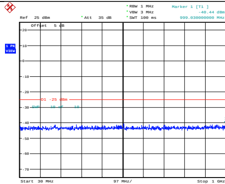
Band41-10MHz-QPSK-40640-1RB#0- Range1:30~1000MHz
