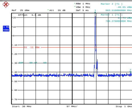
Band12-10MHz-QPSK-23060-1RB#0-Range1:30~1000MHz
