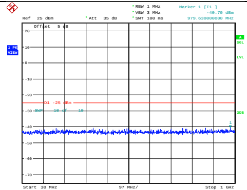
Band38-15MHz-16QAM-37825-1RB#0- Range1:30~1000MHz
