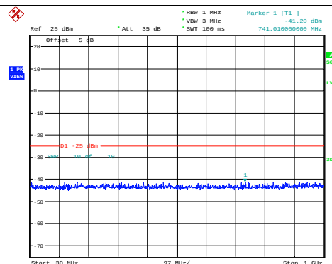
Band41-15MHz-QPSK-40640-1RB#0- Range1:30~1000MHz
