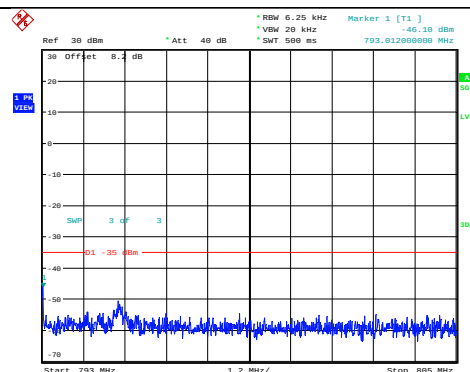
Band13-10MHz-64QAM-23230-1RB#0-Range4:793~805MHz
