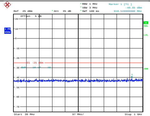
Band41-15MHz-16QAM-41165-1RB#0- Range1:30~1000MHz
