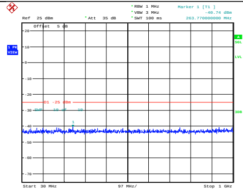
Band38-5MHz-16QAM-37775-1RB#0-Range1:30~1000MHz
