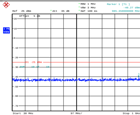
Band41-20MHz-16QAM-40140-1RB#0-Range1:30~1000MHz
