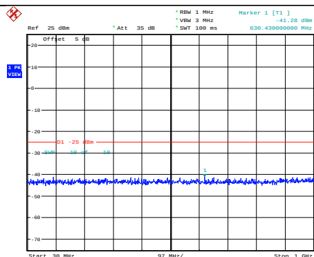
Band38-10MHz-16QAM-37800-1RB#0- Range1:30~1000MHz
