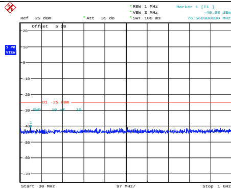
Band38-5MHz-QPSK-38225-1RB#0-Range1:30~1000MHz
