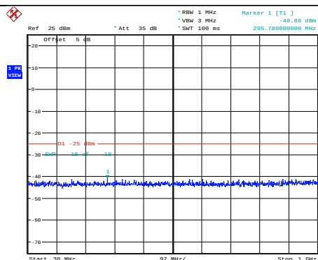
Band41-15MHz-QPSK-41165-1RB#0-Range1:30~1000MHz
