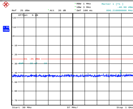
Band38-5MHz-QPSK-37775-1RB#0- Range1:30~1000MHz
