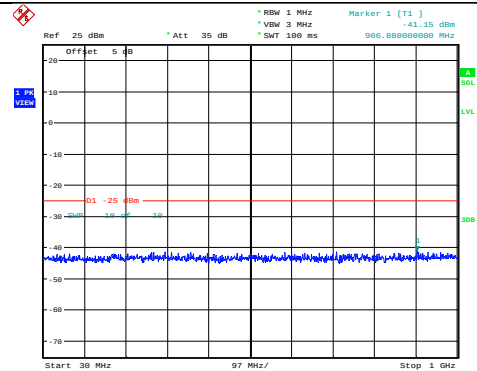
Band38-5MHz-QPSK-38000-1RB#0- Range1:30~1000MHz
