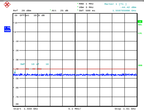
Band13-5MHz-QPSK-23230-1RB#0-Range5:1559~1610MHz
