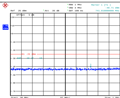
Band41-15MHz-64QAM-41165-1RB#0-Range1:30~1000MHz
