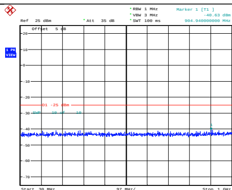
Band41-15MHz-QPSK-40115-1RB#0- Range1:30~1000MHz
