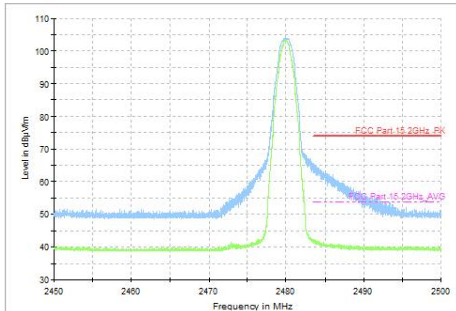
Fig.28 Radiated Band Edges (CH39, 2.45GHz~2.50GHz), LE 1M
