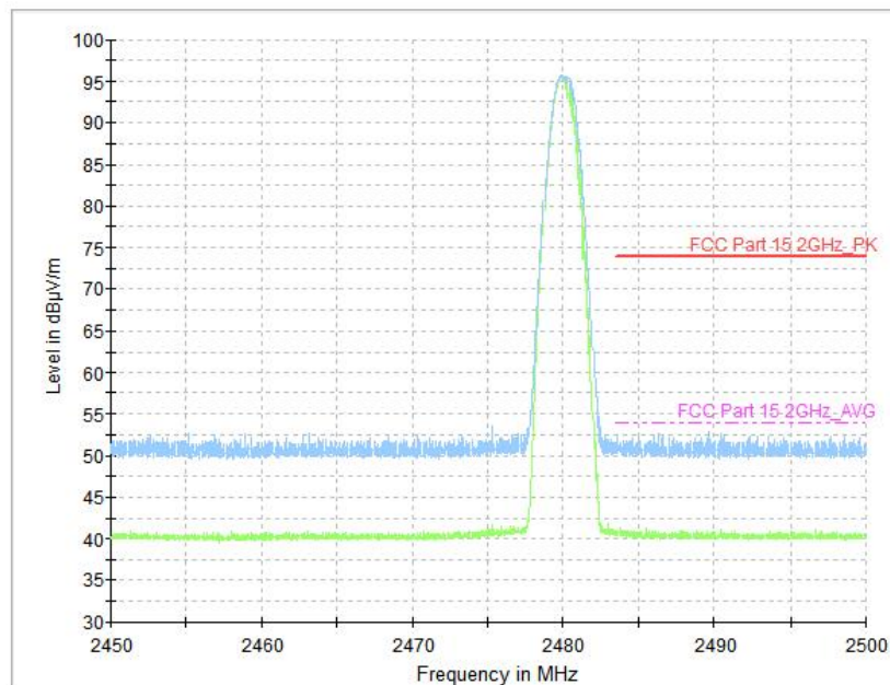
Fig.33 Radiated Band Edges (CH39, 2.45GHz~2.50GHz), LE 2M
