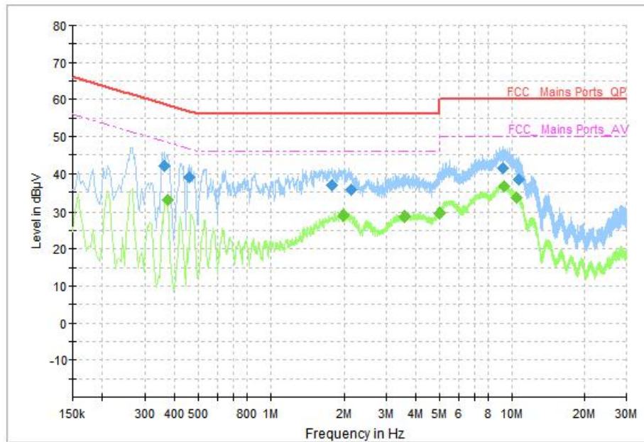
Fig.38 AC Power line Conducted Emission (Idle), LE 1M
