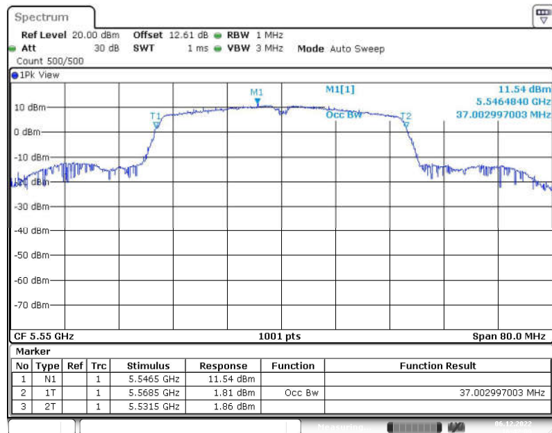
Fig. 50 99% Occupied Bandwidth (802.11n-HT40, 5550MHz)
