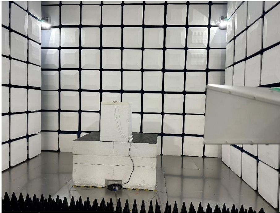
Above 1GHz-BT
