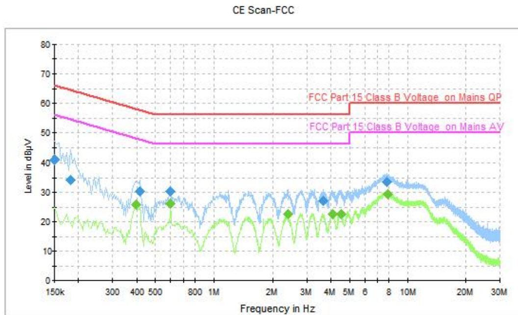
Figure A-6 Conducted Emission (Idle)
