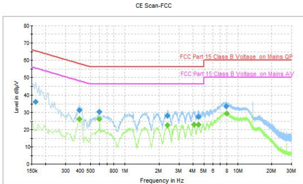
Figure A-5 Conducted Emission (Traffic)
