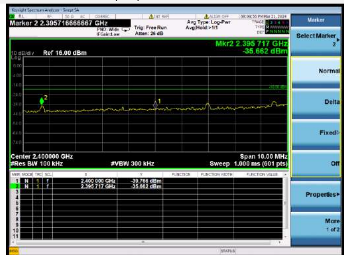
802.11ax-40 MHz(SU) CHANNEL 4, BAND EDGE
