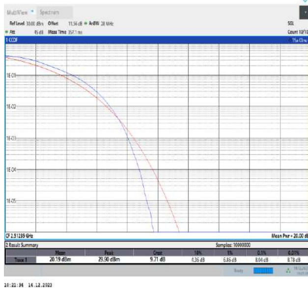
41-41-15MHz-20MHz-QPSK-QPSK-39728-39899-75RB#0-100RB#0-PASS
