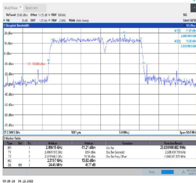
41-41-15MHz-10MHz-QPSK-QPSK-39725-39845-75RB#0-50RB#0-PASS
