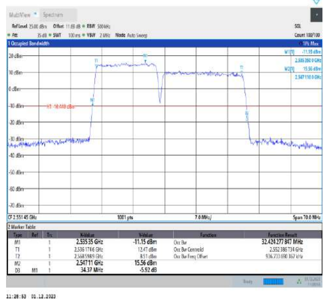
7-7-15MHz-20MHz-QPSK-QPSK-21179-21350-75RB#0-100RB#0-PASS
