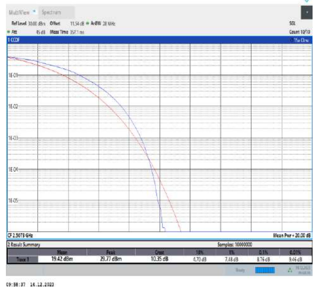
41-41-10MHz-15MHz-16QAM-16QAM-39703-39823-50RB#0-75RB#0-PASS
