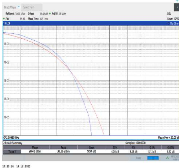
41-41-20MHz-5MHz-QPSK-QPSK-40595-40712-100RB#0-25RB#0-PASS
