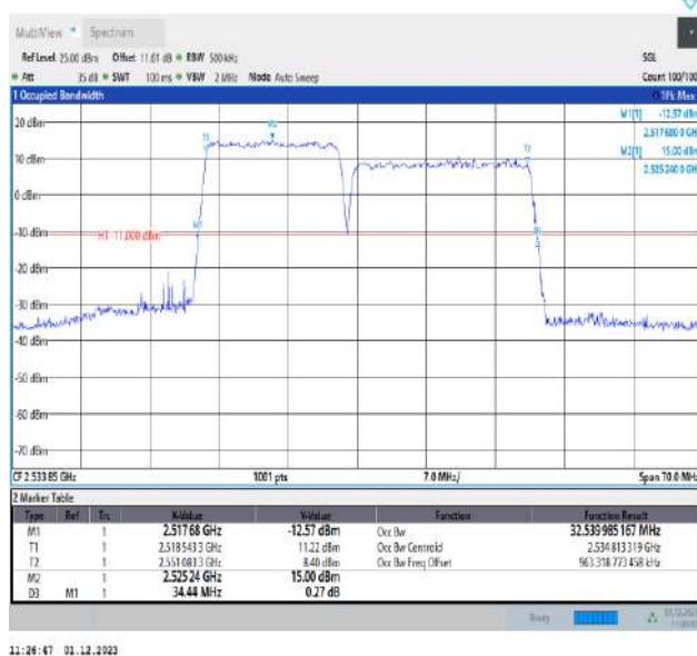
7-7-15MHz-20MHz-QPSK-QPSK-21003-21174-75RB#0-100RB#0-PASS
