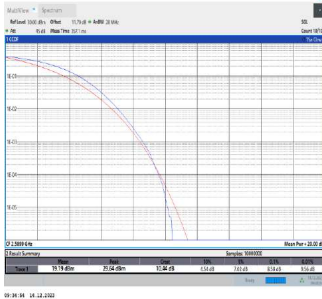
38-38-20MHz-20MHz-QPSK-QPSK-37850-38048-100RB#0-100RB#0-PASS
