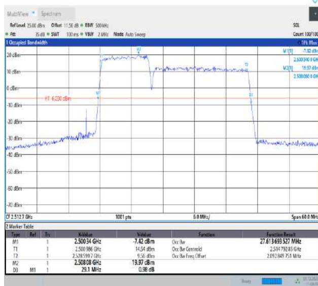
7-7-10MHz-20MHz-16QAM-16QAM-20805-20949-50RB#0-100RB#0-PASS
