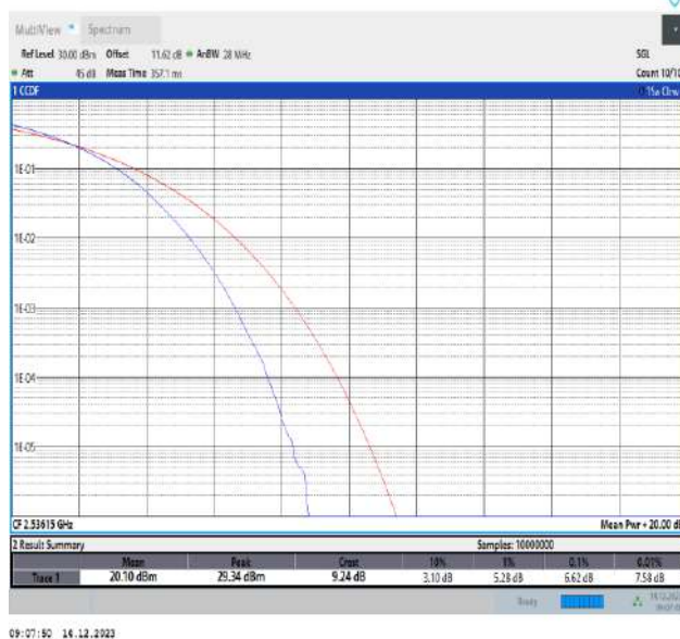
7-7-20MHz-15MHz-64QAM-64QAM-21026-21197-100RB#0-75RB#0-PASS
