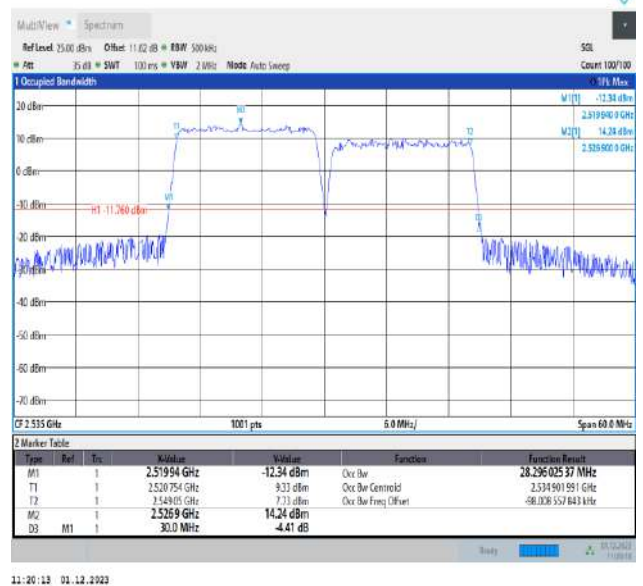
7-7-15MHz-15MHz-16QAM-16QAM-21025-21175-75RB#0-75RB#0-PASS
