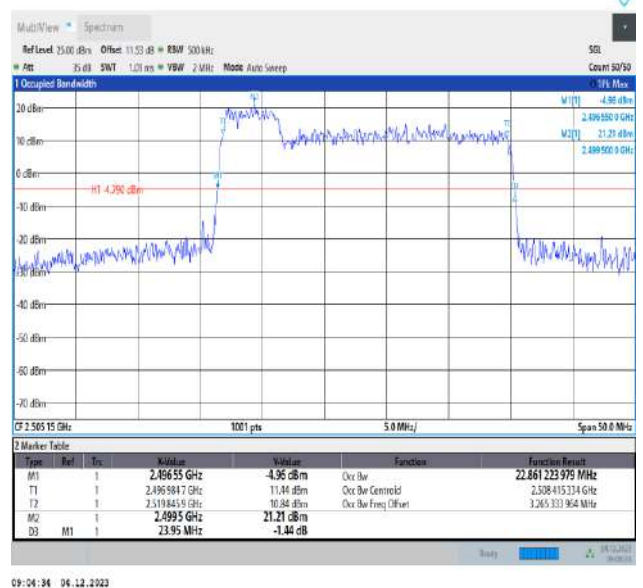
41-41-5MHz-20MHz-QPSK-QPSK-39683-39800-25RB#0-100RB#0-PASS
