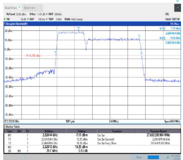
7-7-10MHz-20MHz-16QAM-16QAM-21006-21150-50RB#0-100RB#0-PASS
