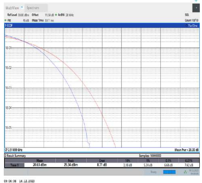
7-7-20MHz-15MHz-64QAM-64QAM-20850-21021-100RB#0-75RB#0-PASS
