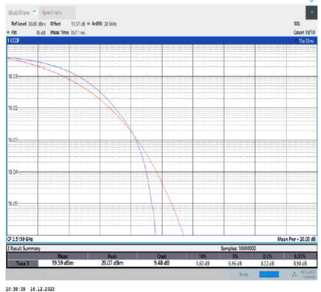
41-41-20MHz-20MHz-QPSK-QPSK-39750-39948-100RB#0-100RB#0-PASS
