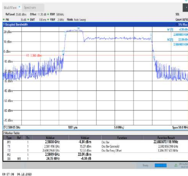
41-41-5MHz-20MHz-QPSK-QPSK-40528-40645-25RB#0-100RB#0-PASS
