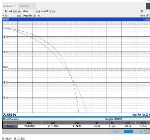
41-41-5MHz-20MHz-16QAM-16QAM-39683-39800-25RB#0-100RB#0-PASS
