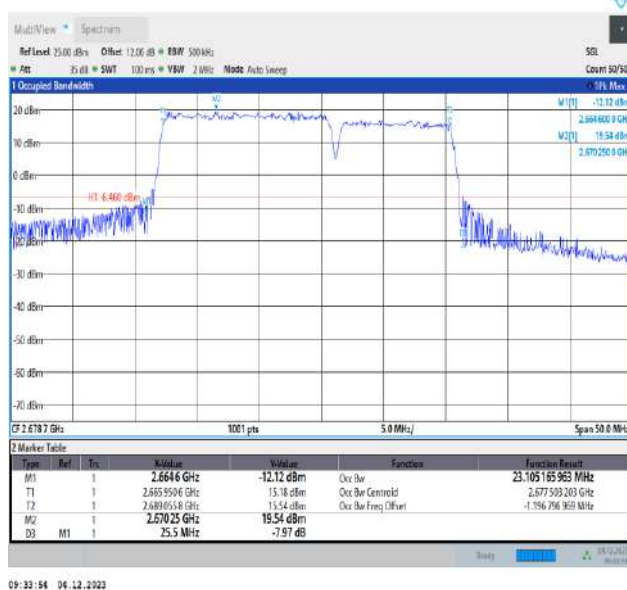
41-41-15MHz-10MHz-QPSK-QPSK-41417-41537-75RB#0-50RB#0-PASS
