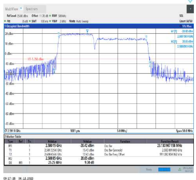
41-41-10MHz-15MHz-QPSK-QPSK-40549-40669-50RB#0-75RB#0-PASS
