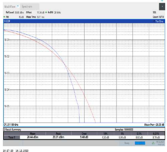
41-41-20MHz-5MHz-QPSK-QPSK-39750-39867-100RB#0-25RB#0-PASS
