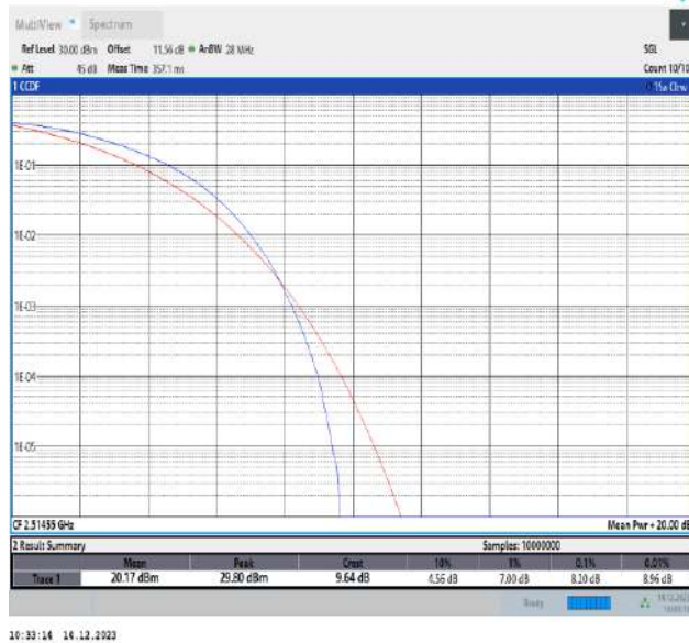
41-41-20MHz-15MHz-QPSK-QPSK-39750-39921-100RB#0-75RB#0-PASS
