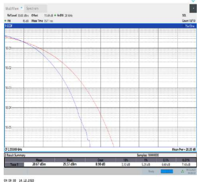
7-7-20MHz-15MHz-64QAM-64QAM-21201-21372-100RB#0-75RB#0-PASS
