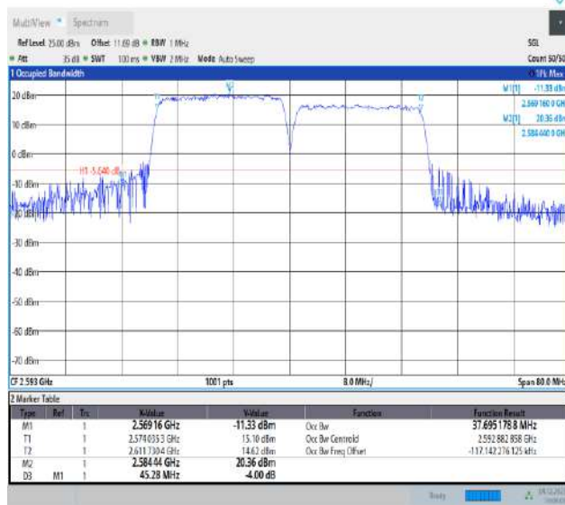
41-41-20MHz-20MHz-QPSK-QPSK-40521-40719-100RB#0-100RB#0-PASS
