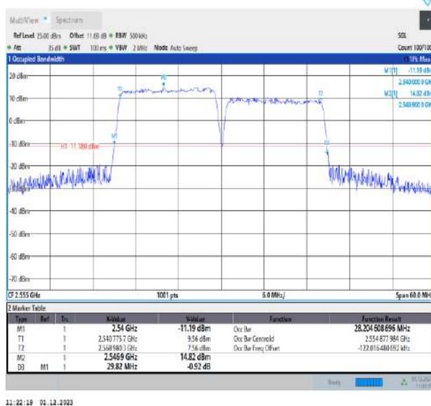
7-7-15MHz-15MHz-16QAM-16QAM-21225-21375-75RB#0-75RB#0-PASS
