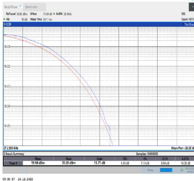
38-38-15MHz-15MHz-QPSK-QPSK-37925-38075-75RB#0-75RB#0-PASS
