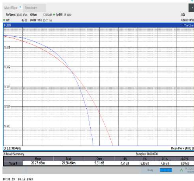
41-41-20MHz-15MHz-QPSK-QPSK-41341-41512-100RB#0-75RB#0-PASS
