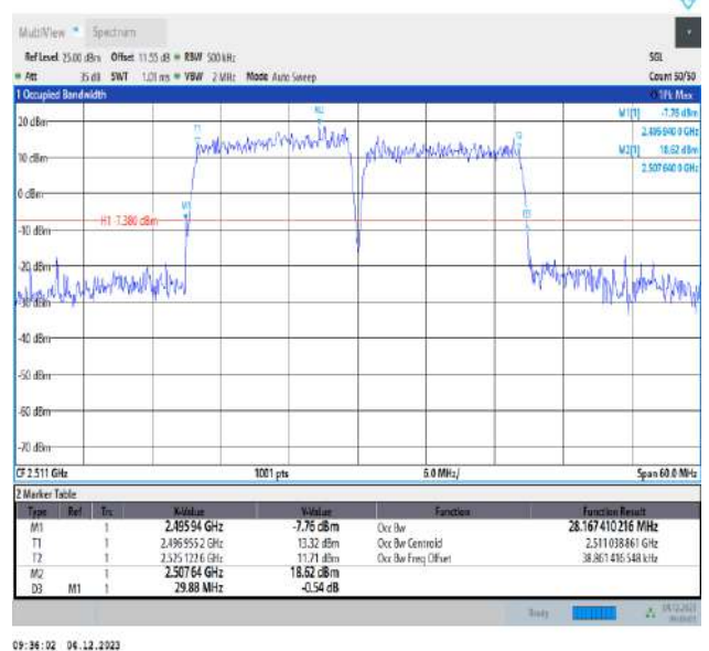
41-41-15MHz-15MHz-QPSK-QPSK-39725-39875-75RB#0-75RB#0-PASS
