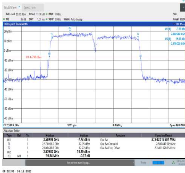
38-38-20MHz-20MHz-QPSK-QPSK-37850-38048-100RB#0-100RB#0-PASS
