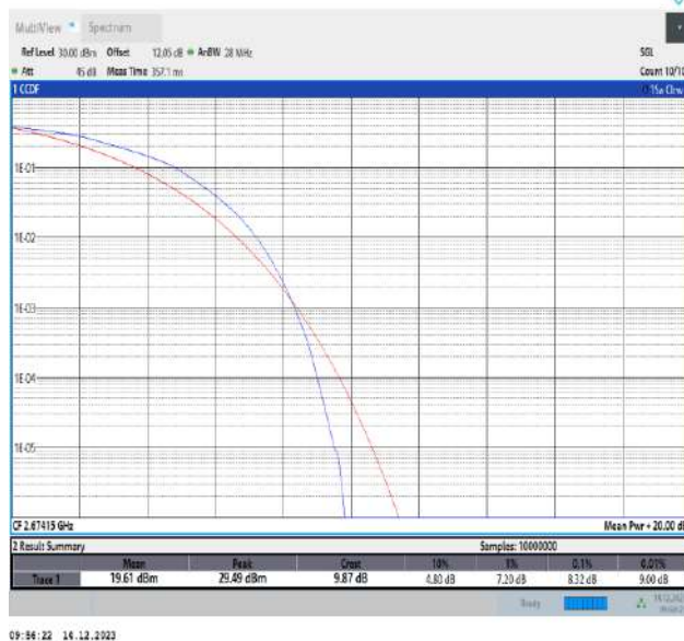
41-41-5MHz-20MHz-16QAM-16QAM-41373-41490-25RB#0-100RB#0-PASS
