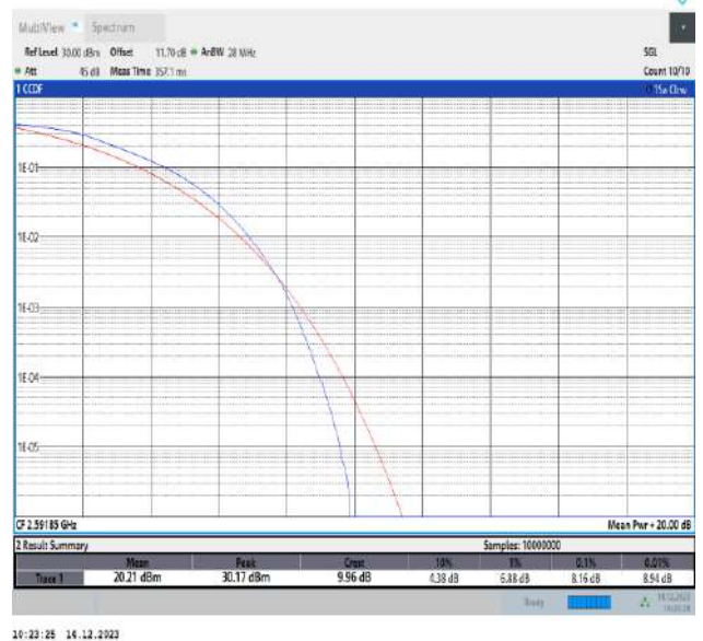
41-41-15MHz-20MHz-QPSK-QPSK-40523-40694-75RB#0-100RB#0-PASS
