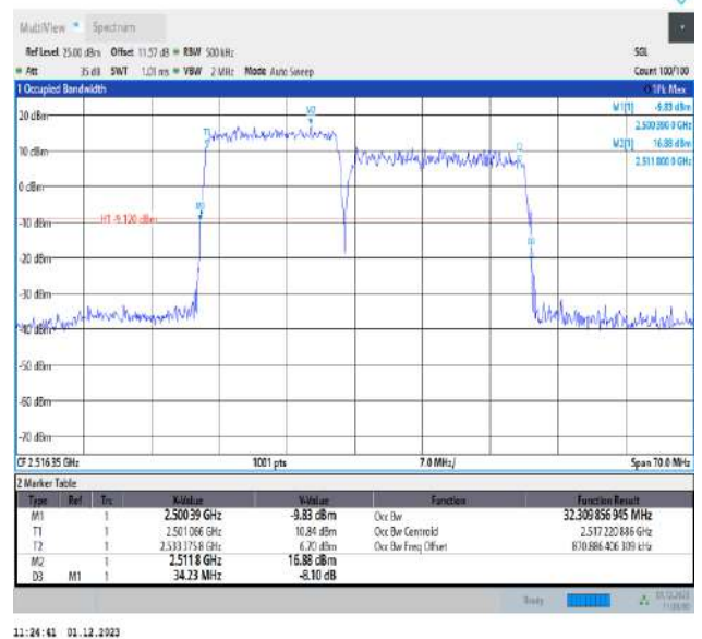
7-7-15MHz-20MHz-QPSK-QPSK-20828-20999-75RB#0-100RB#0-PASS
