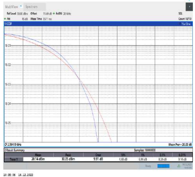
41-41-20MHz-15MHz-QPSK-QPSK-40546-40717-100RB#0-75RB#0-PASS
