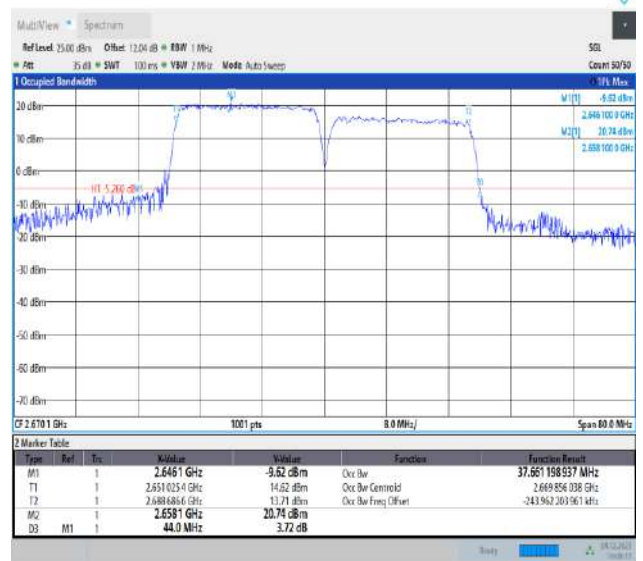
41-41-20MHz-20MHz-QPSK-QPSK-41292-41490-100RB#0-100RB#0-PASS
