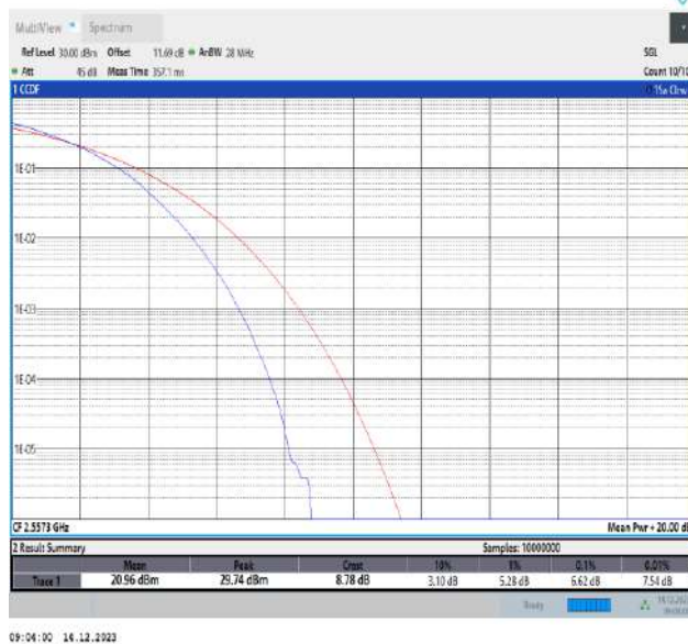
7-7-20MHz-10MHz-64QAM-64QAM-21251-21395-100RB#0-50RB#0-PASS
