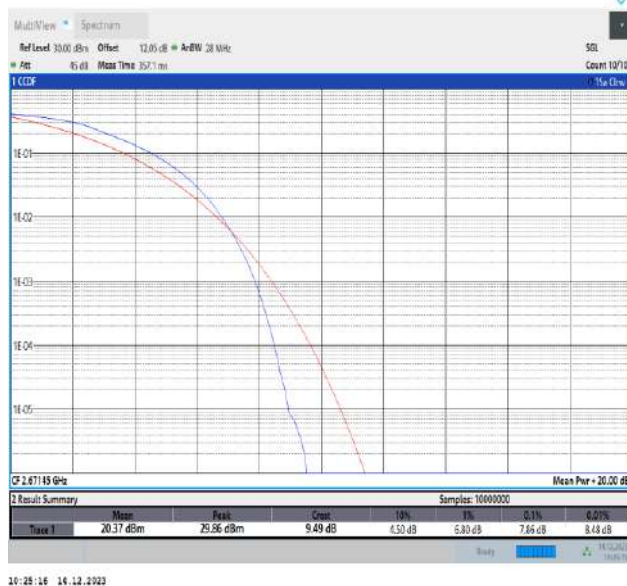
41-41-15MHz-20MHz-QPSK-QPSK-41319-41490-75RB#0-100RB#0-PASS
