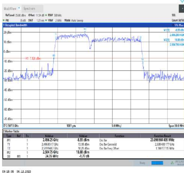
41-41-10MHz-15MHz-QPSK-QPSK-39703-39823-50RB#0-75RB#0-PASS
