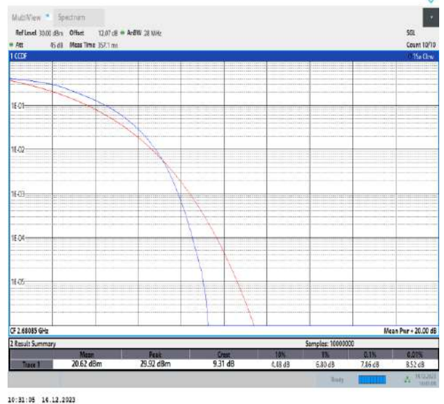
41-41-20MHz-5MHz-QPSK-QPSK-41440-41557-100RB#0-25RB#0-PASS
