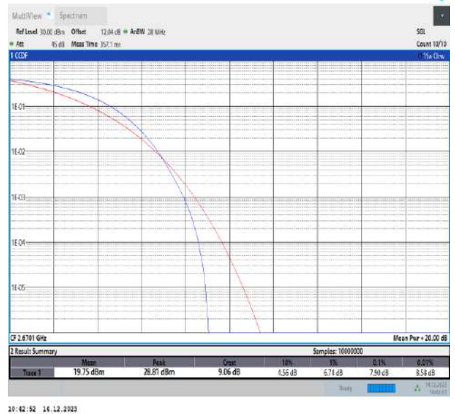
41-41-20MHz-20MHz-QPSK-QPSK-41292-41490-100RB#0-100RB#0-PASS
