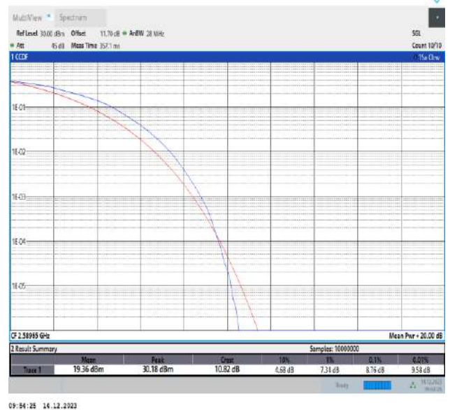
41-41-5MHz-20MHz-16QAM-16QAM-40528-40645-25RB#0-100RB#0-PASS
