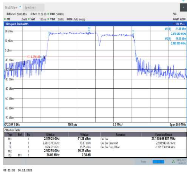
41-41-15MHz-10MHz-QPSK-QPSK-40571-40691-75RB#0-50RB#0-PASS
