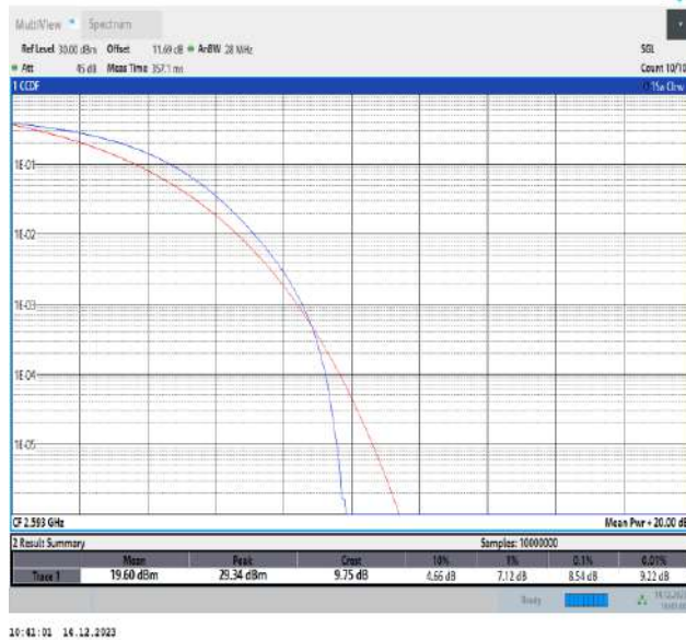
41-41-20MHz-20MHz-QPSK-QPSK-40521-40719-100RB#0-100RB#0-PASS
