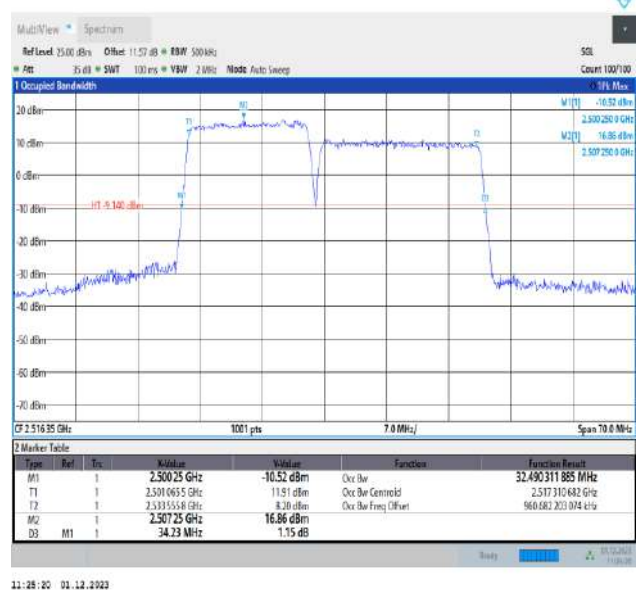
7-7-15MHz-20MHz-16QAM-16QAM-20828-20999-75RB#0-100RB#0-PASS
