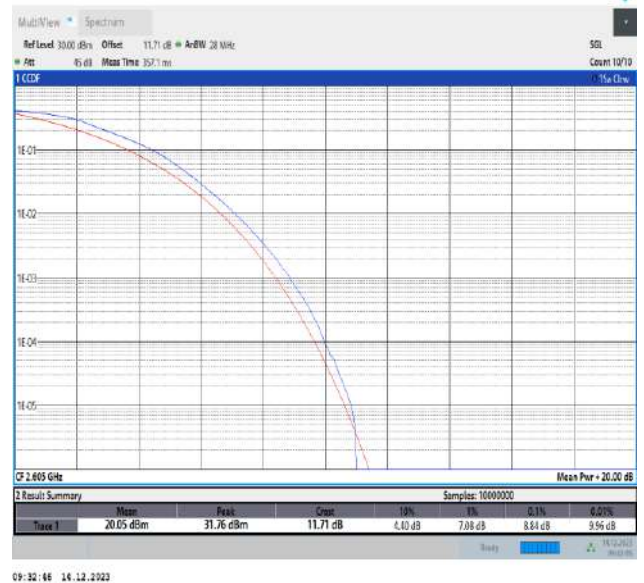
38-38-15MHz-15MHz-QPSK-QPSK-38025-38175-75RB#0-75RB#0-PASS
