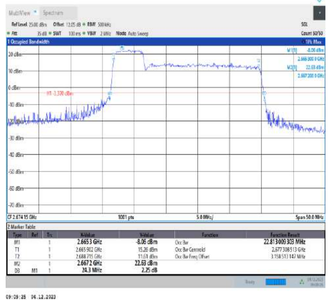
41-41-5MHz-20MHz-QPSK-QPSK-41373-41490-25RB#0-100RB#0-PASS
