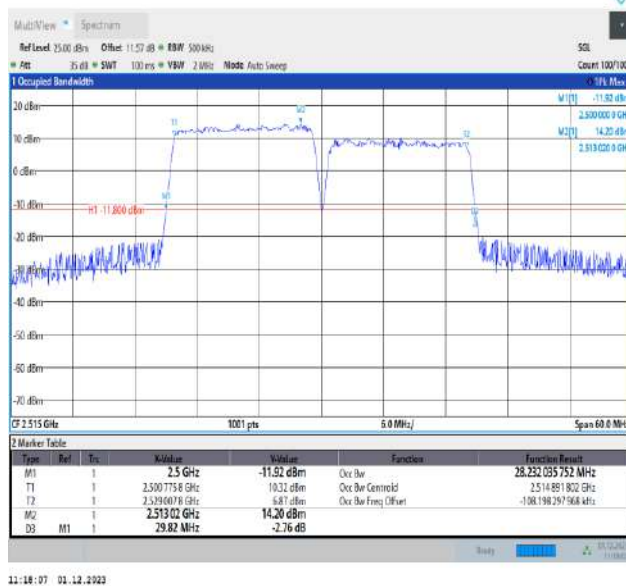
7-7-15MHz-15MHz-16QAM-16QAM-20825-20975-75RB#0-75RB#0-PASS
