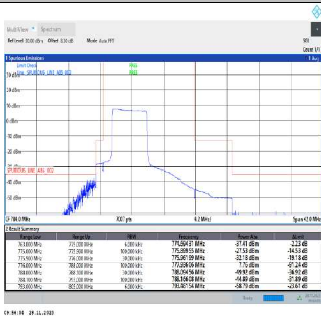
Band13_5MHz_QPSK_23205_25RB#0
