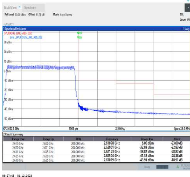
Band38_10MHz_16QAM_38200_50RB#0
