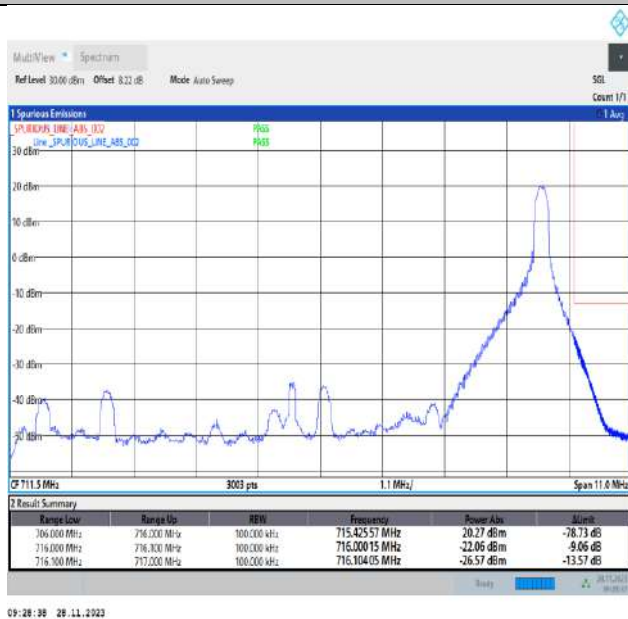
Band12_10MHz_64QAM_23130_1RB#49
