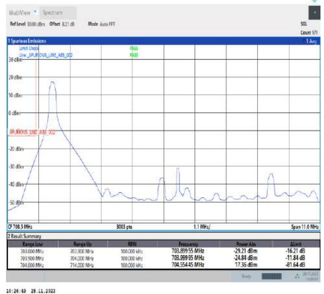
Band17_10MHz_64QAM_23780_1RB#0
