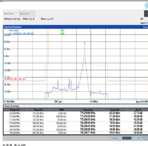
Band13_10MHz_QPSK_23230_1RB#49
