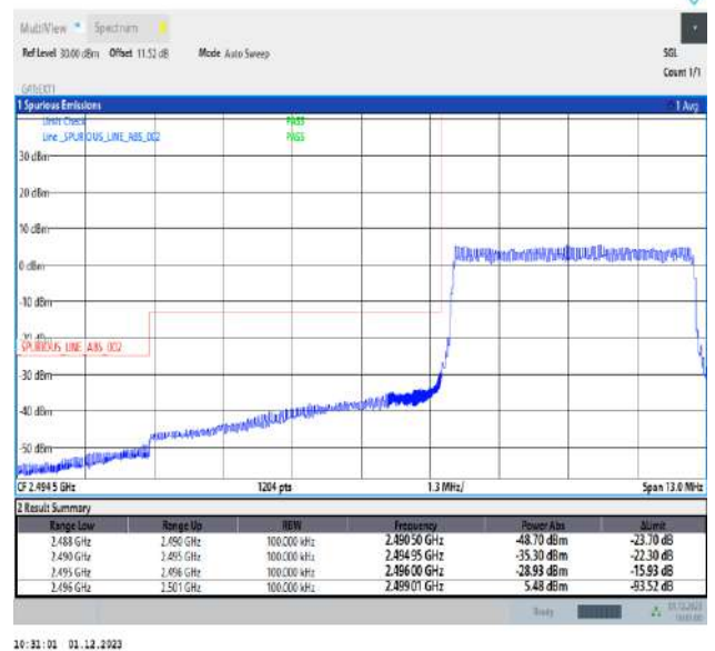
Band41_5MHz_64QAM_39675_25RB#0
