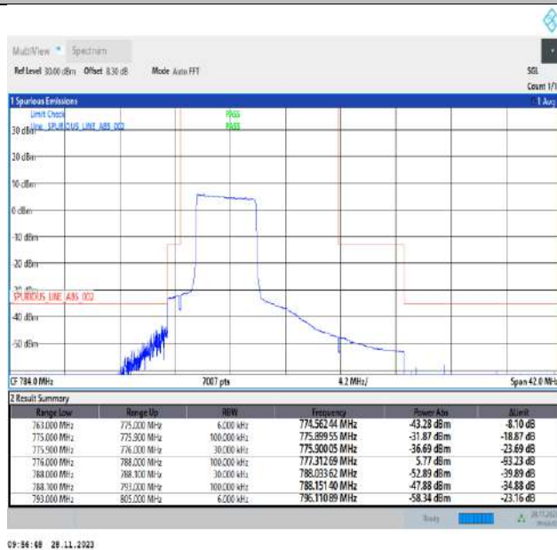
Band13_5MHz_64QAM_23205_25RB#0
