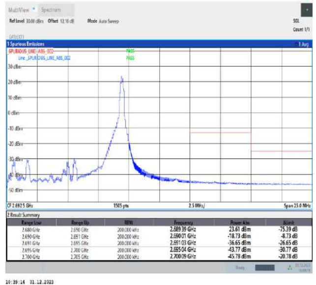
Band41_10MHz_QPSK_41540_1RB#49
