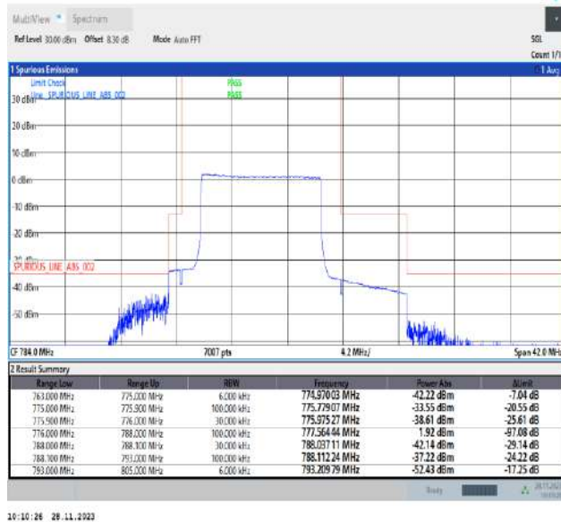
Band13_10MHz_64QAM_23230_50RB#0
