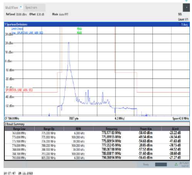
Band13_10MHz_16QAM_23230_1RB#0
