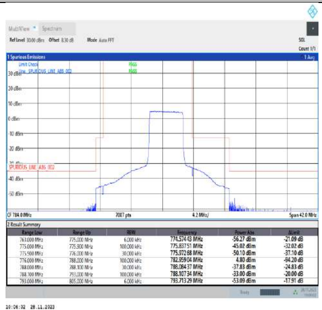
Band13_5MHz_16QAM_23255_25RB#0
