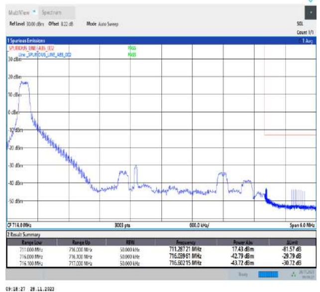
Band12_5MHz_16QAM_23155_1RB#0
