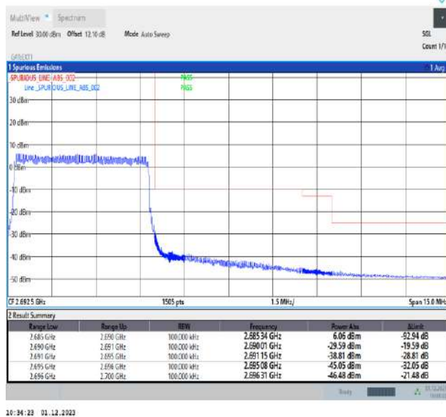
Band41_5MHz_64QAM_41565_25RB#0
