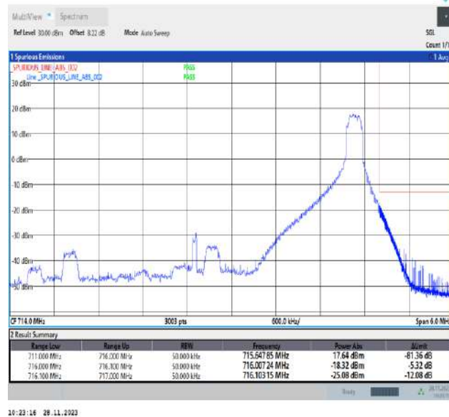
Band17_5MHz_64QAM_23825_1RB#24
