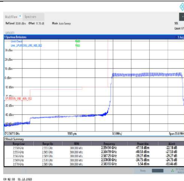
Band38_15MHz_16QAM_37825_75RB#0
