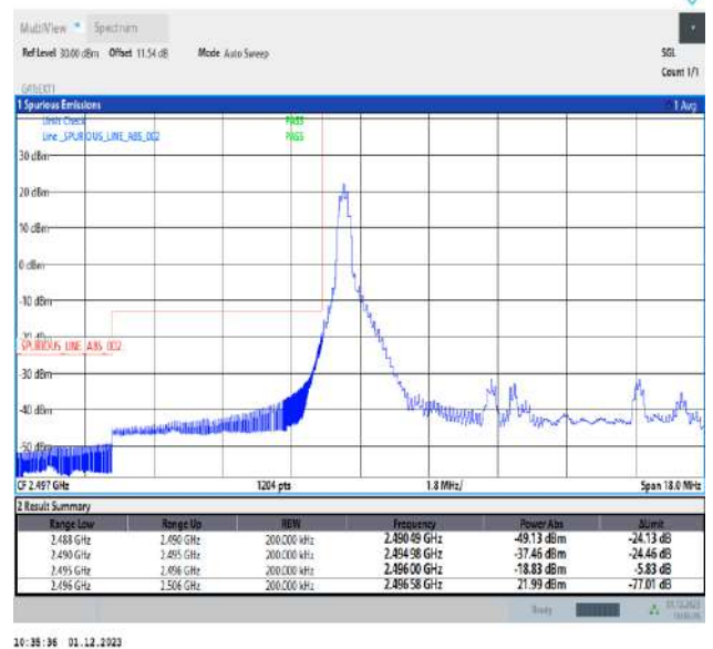
Band41_10MHz_64QAM_39700_1RB#0
