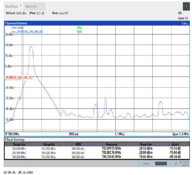
Band17_10MHz_16QAM_23780_1RB#0
