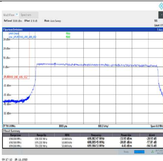
Band12_5MHz_QPSK_23035_25RB#0
