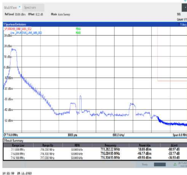
Band17_5MHz_16QAM_23825_1RB#0
