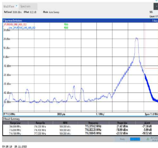
Band12_10MHz_16QAM_23130_1RB#49
