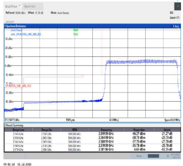
Band38_20MHz_16QAM_37850_100RB#0
