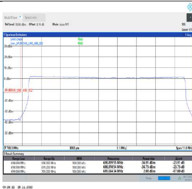
Band12_10MHz_16QAM_23060_50RB#0
