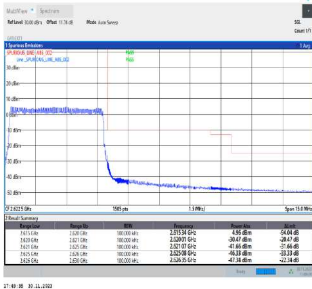
Band38_5MHz_64QAM_38225_25RB#0
