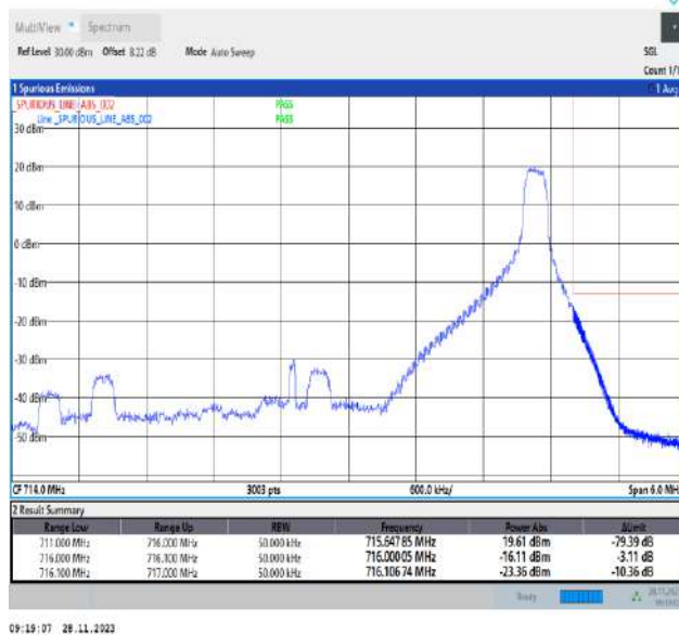
Band12_5MHz_QPSK_23155_1RB#24
