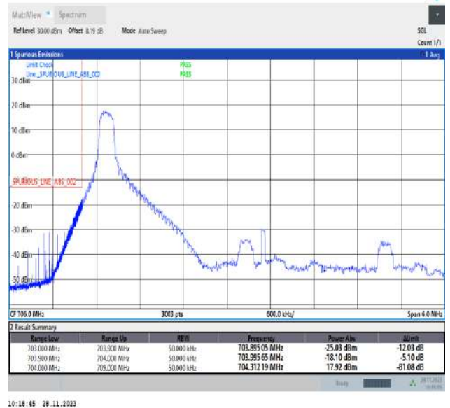
Band17_5MHz_QPSK_23755_1RB#0
