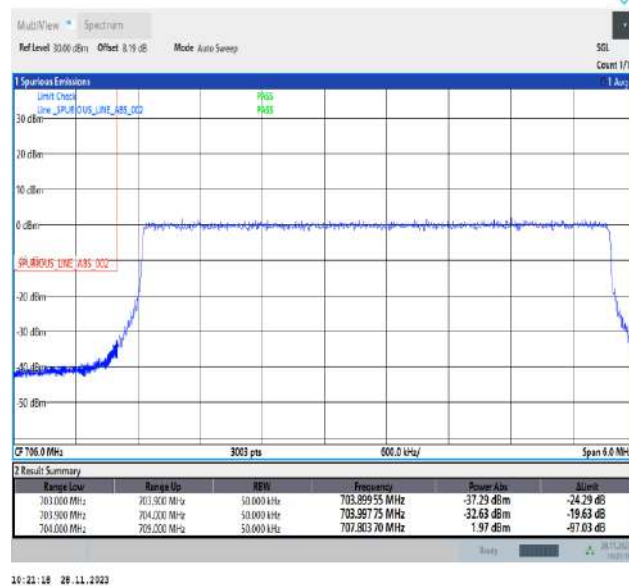
Band17_5MHz_64QAM_23755_25RB#0
