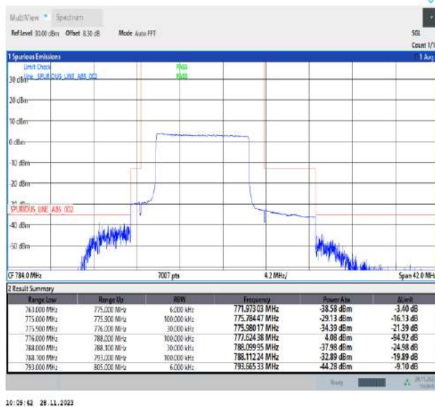
Band13_10MHz_QPSK_23230_50RB#0
