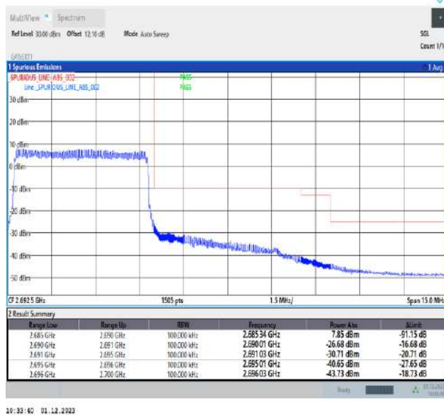
Band41_5MHz_QPSK_41565_25RB#0
