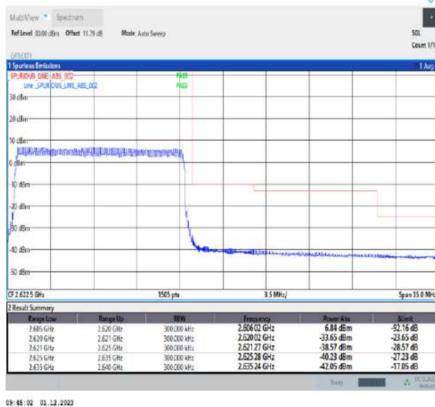
Band38_15MHz_QPSK_38175_75RB#0
