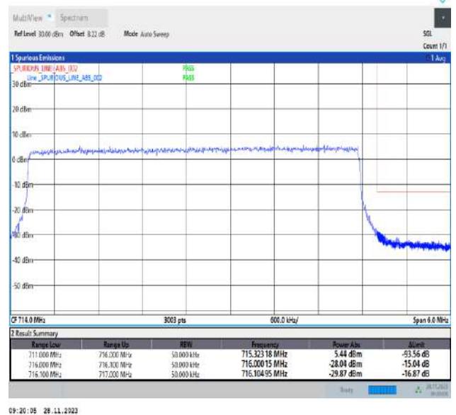
Band12_5MHz_QPSK_23155_25RB#0
