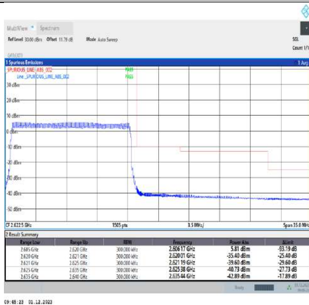
Band38_15MHz_16QAM_38175_75RB#0
