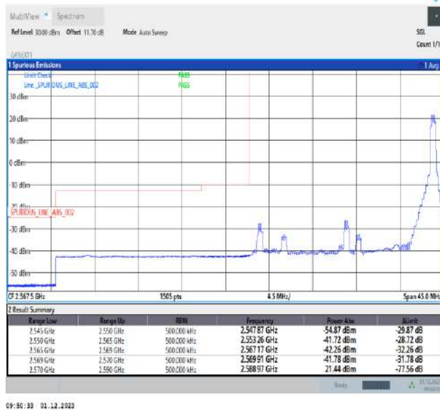
Band38_20MHz_64QAM_37850_1RB#99
