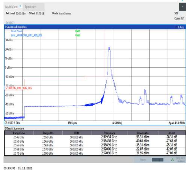
Band38_20MHz_16QAM_37850_1RB#0
