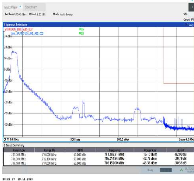
Band17_5MHz_64QAM_23825_1RB#0
