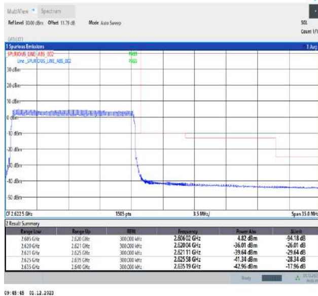
Band38_15MHz_64QAM_38175_75RB#0
