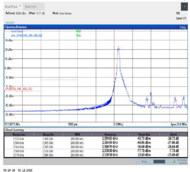
Band38_10MHz_QPSK_37800_1RB#0
