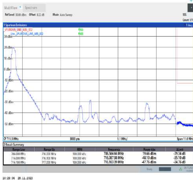
Band17_10MHz_QPSK_23800_1RB#0
