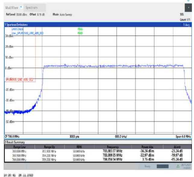
Band17_5MHz_QPSK_23755_25RB#0
