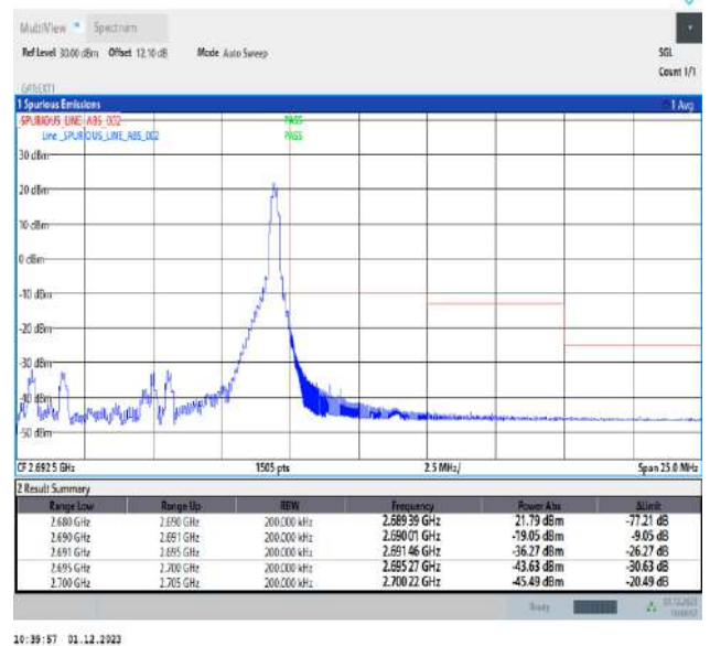
Band41_10MHz_64QAM_41540_1RB#49
