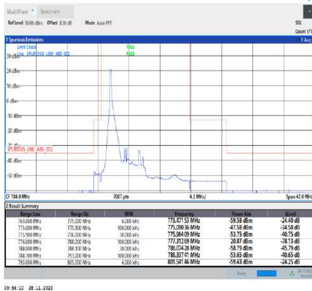
Band13_5MHz_16QAM_23205_1RB#0
