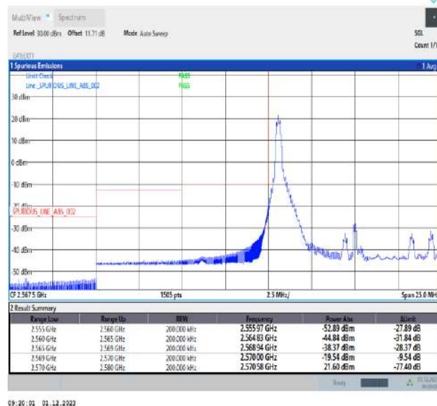
Band38_10MHz_64QAM_37800_1RB#0
