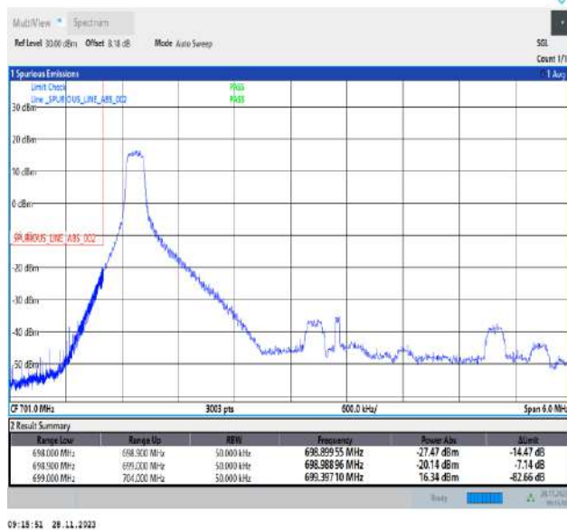
Band12_5MHz_64QAM_23035_1RB#0
