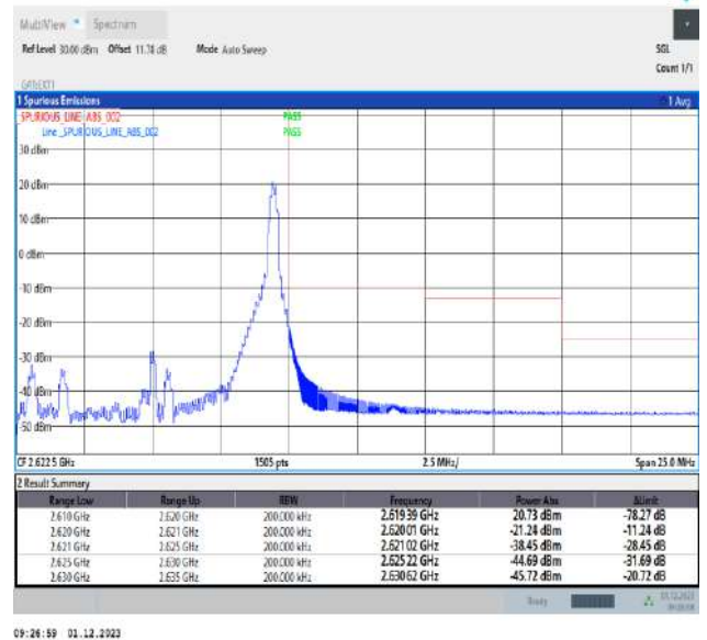
Band38_10MHz_64QAM_38200_1RB#49
