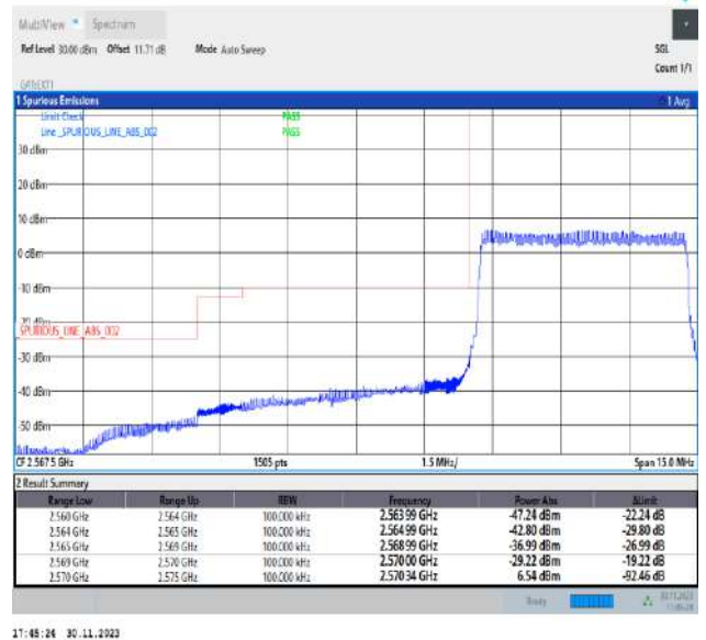
Band38_5MHz_QPSK_37775_25RB#0
