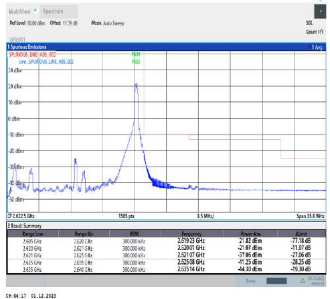
Band38_15MHz_16QAM_38175_1RB#74
