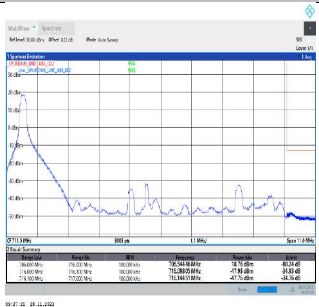
Band12_10MHz_16QAM_23130_1RB#0
