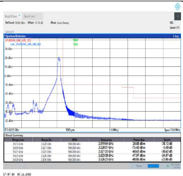
Band38_5MHz_QPSK_38225_1RB#24
