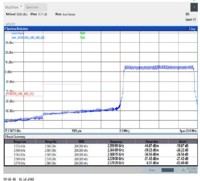
Band38_10MHz_QPSK_37800_50RB#0
