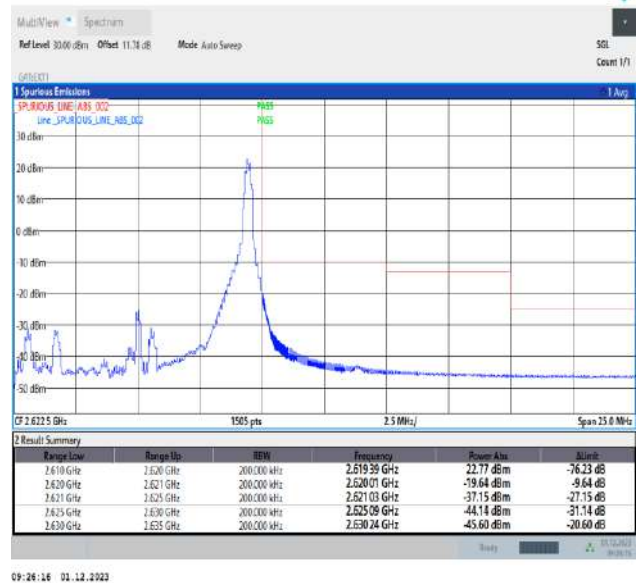
Band38_10MHz_QPSK_38200_1RB#49
