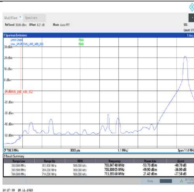
Band17_10MHz_QPSK_23780_1RB#49
