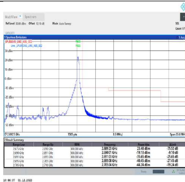
Band41_15MHz_QPSK_41515_1RB#74
