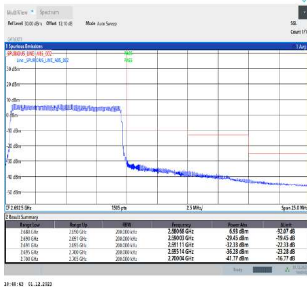
Band41_10MHz_16QAM_41540_50RB#0
