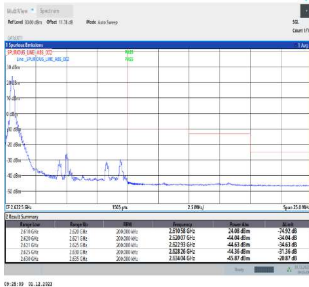
Band38_10MHz_QPSK_38200_1RB#0
