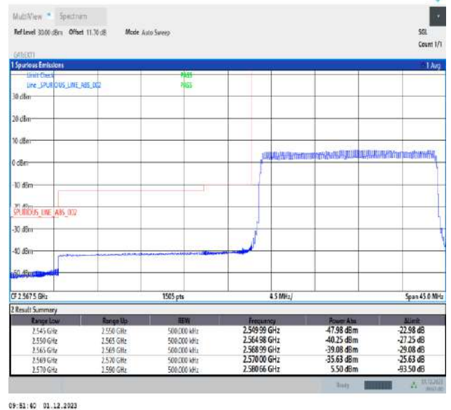
Band38_20MHz_64QAM_37850_100RB#0
