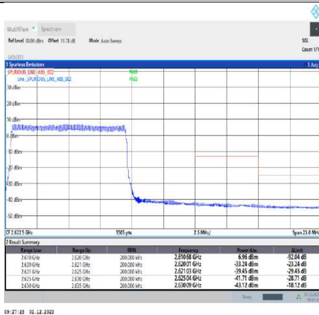
Band38_10MHz_QPSK_38200_50RB#0
