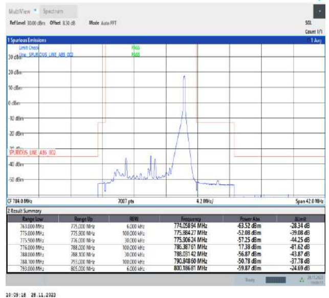
Band13_10MHz_64QAM_23230_1RB#49
