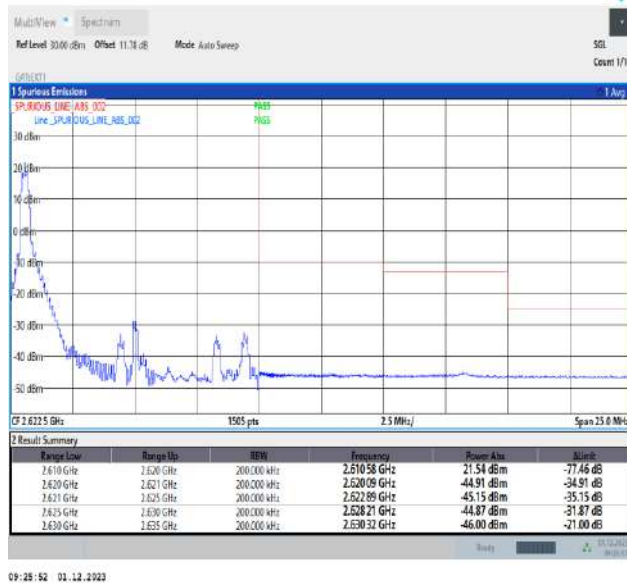
Band38_10MHz_64QAM_38200_1RB#0
