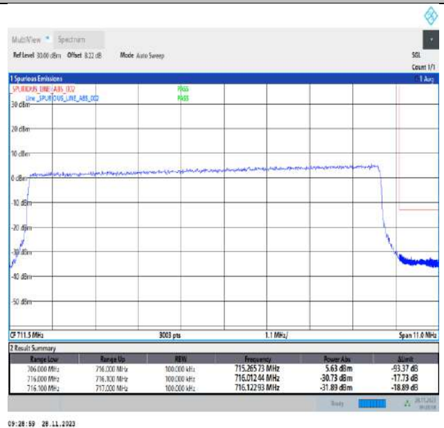
Band12_10MHz_QPSK_23130_50RB#0
