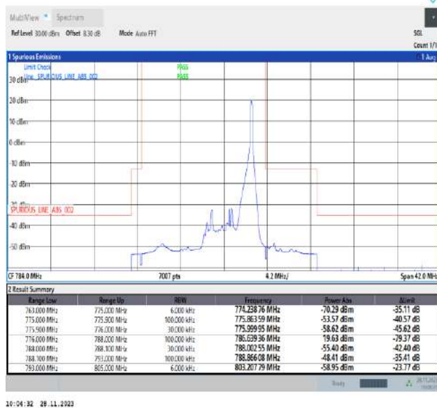
Band13_5MHz_QPSK_23255_1RB#24
