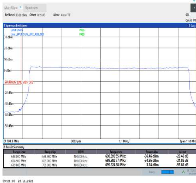
Band12_10MHz_QPSK_23060_50RB#0
