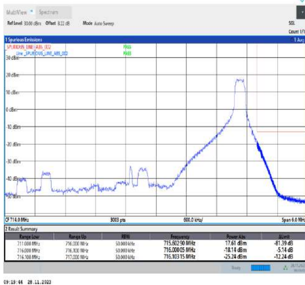
Band12_5MHz_64QAM_23155_1RB#24
