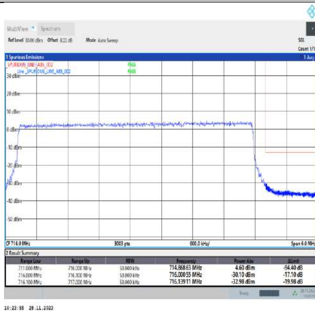
Band17_5MHz_16QAM_23825_25RB#0
