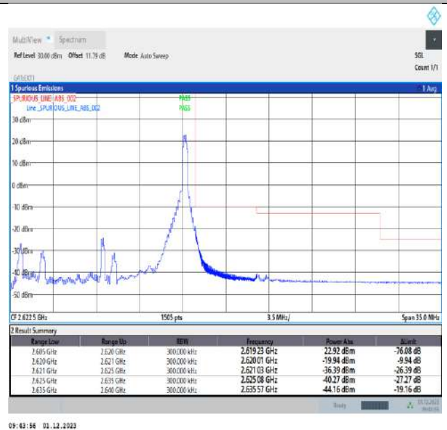
Band38_15MHz_QPSK_38175_1RB#74
