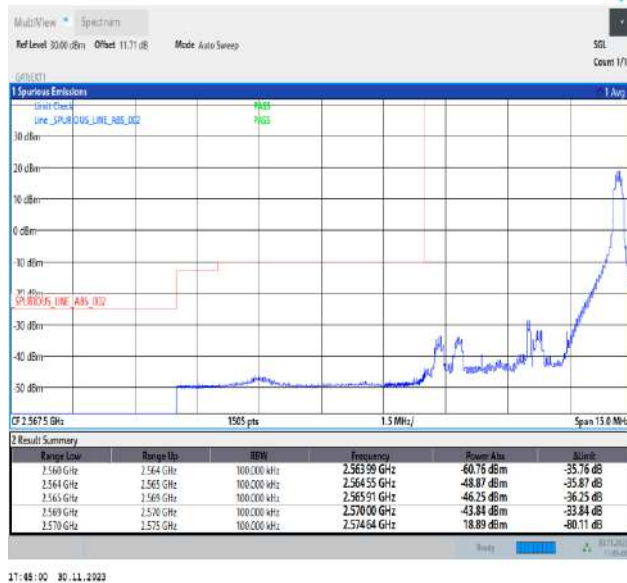
Band38_5MHz_64QAM_37775_1RB#24
