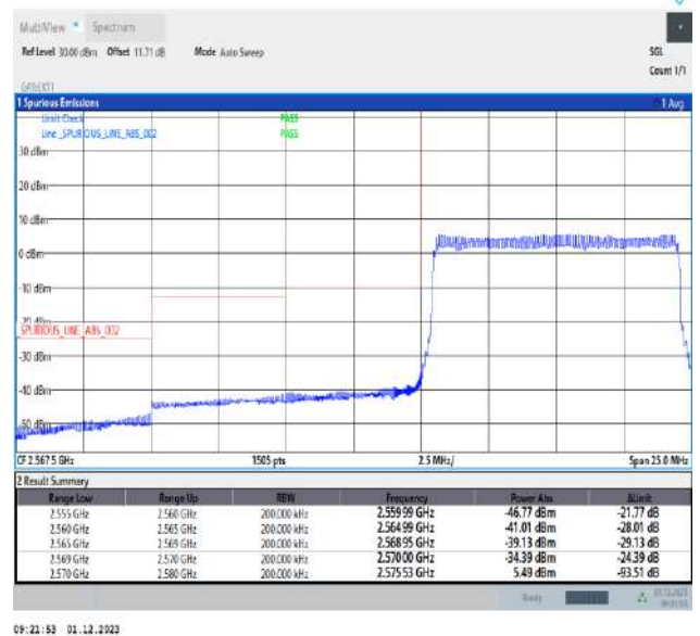
Band38_10MHz_16QAM_37800_50RB#0
