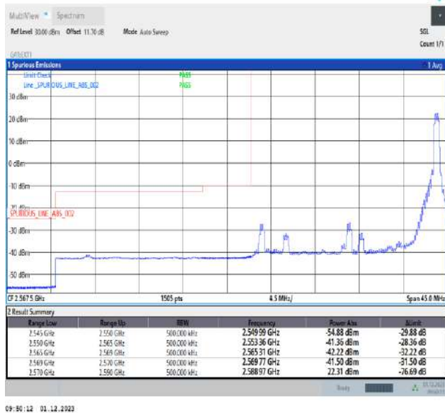
Band38_20MHz_16QAM_37850_1RB#99
