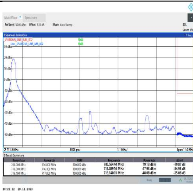
Band17_10MHz_16QAM_23800_1RB#0
