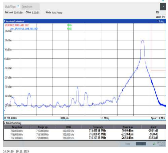
Band17_10MHz_64QAM_23800_1RB#49
