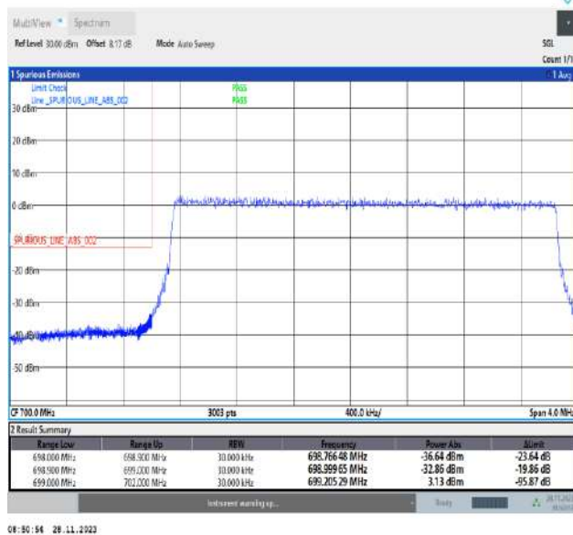
Band12_3MHz_64QAM_23025_15RB#0
