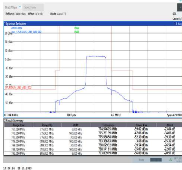
Band13_5MHz_64QAM_23255_25RB#0
