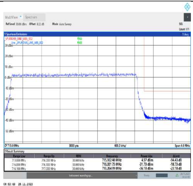
Band12_3MHz_64QAM_23165_15RB#0
