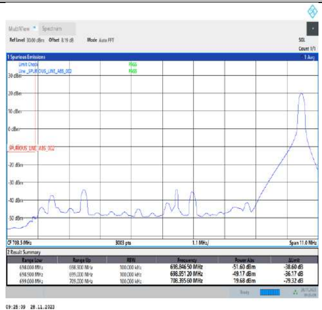
Band12_10MHz_QPSK_23060_1RB#49
