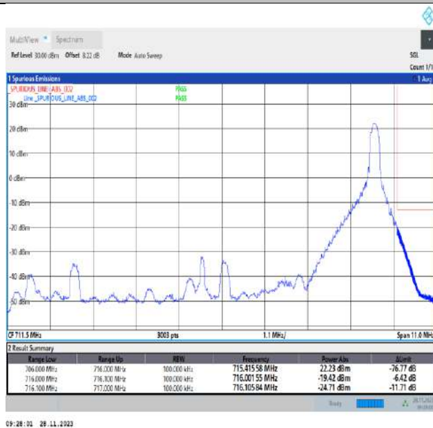
Band12_10MHz_QPSK_23130_1RB#49
