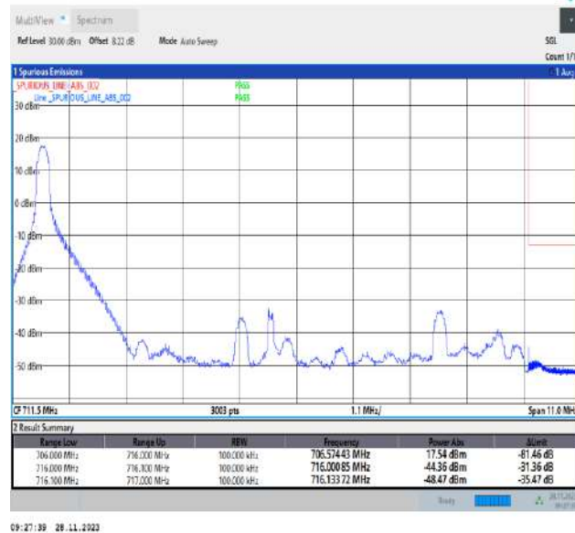
Band12_10MHz_64QAM_23130_1RB#0
