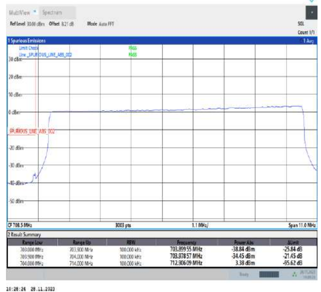
Band17_10MHz_16QAM_23780_50RB#0
