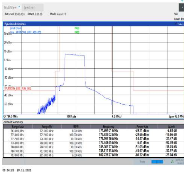
Band13_5MHz_16QAM_23205_25RB#0
