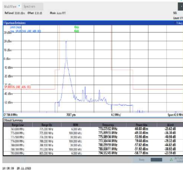
Band13_10MHz_64QAM_23230_1RB#0
