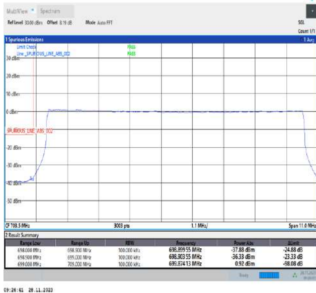
Band12_10MHz_64QAM_23060_50RB#0
