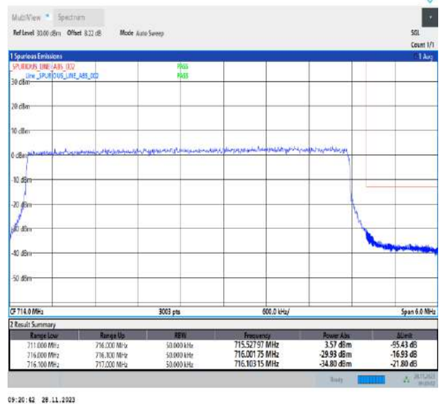
Band12_5MHz_64QAM_23155_25RB#0
