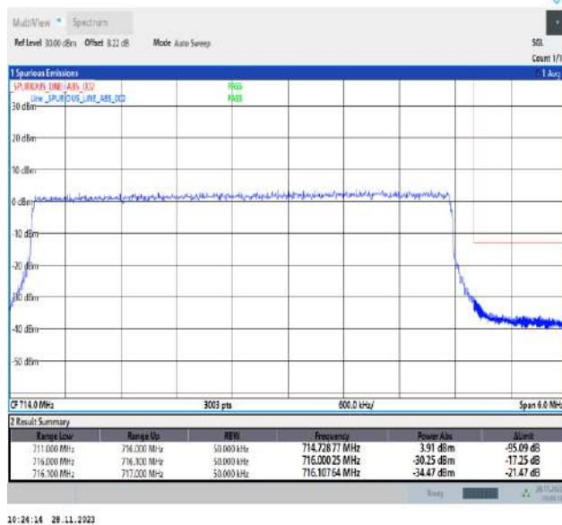
Band17_5MHz_64QAM_23825_25RB#0
