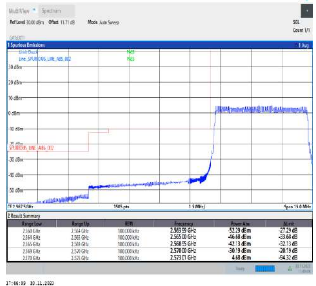
Band38_5MHz_64QAM_37775_25RB#0
