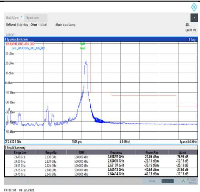
Band38_20MHz_16QAM_38150_1RB#99
