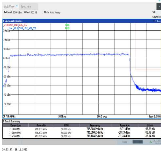
Band17_5MHz_QPSK_23825_25RB#0
