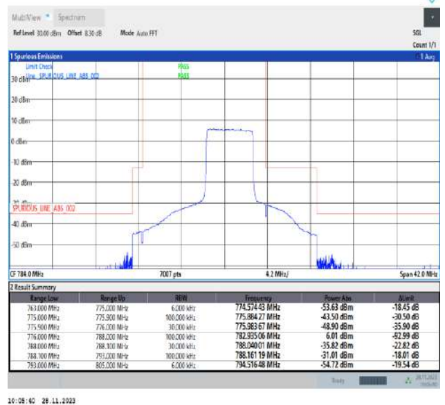
Band13_5MHz_QPSK_23255_25RB#0
