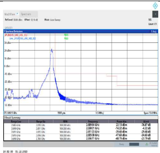
Band41_5MHz_QPSK_41565_1RB#24
