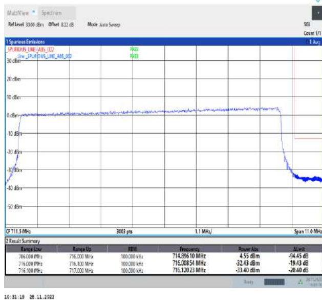
Band17_10MHz_16QAM_23800_50RB#0
