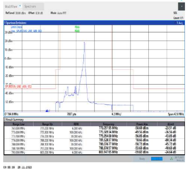
Band13_5MHz_64QAM_23205_1RB#24
