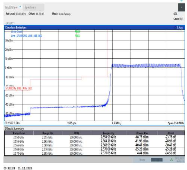
Band38_15MHz_64QAM_37825_75RB#0
