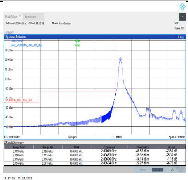
Band41_5MHz_QPSK_39675_1RB#0
