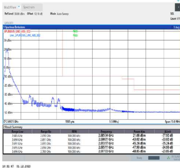
Band41_5MHz_16QAM_41565_1RB#0
