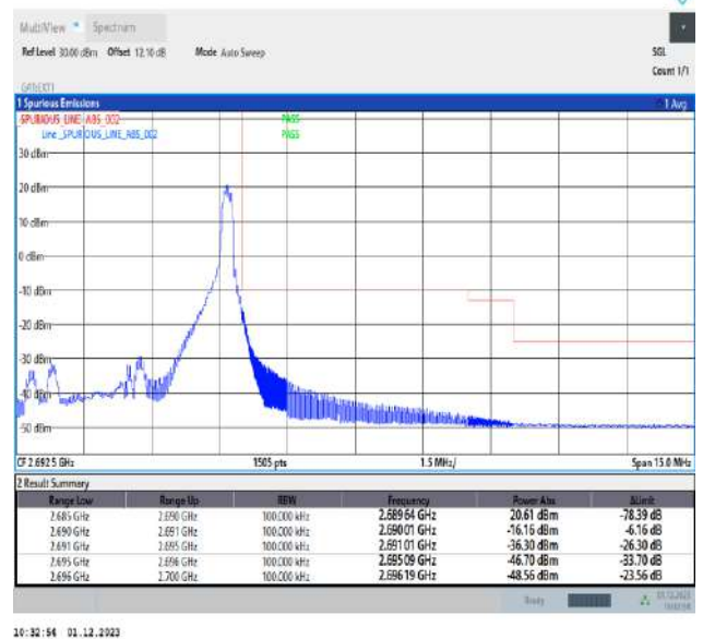
Band41_5MHz_16QAM_41565_1RB#24
