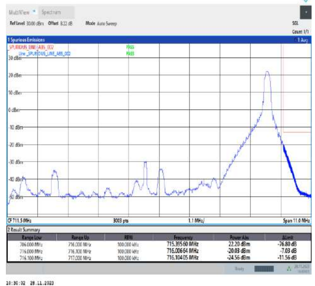
Band17_10MHz_QPSK_23800_1RB#49
