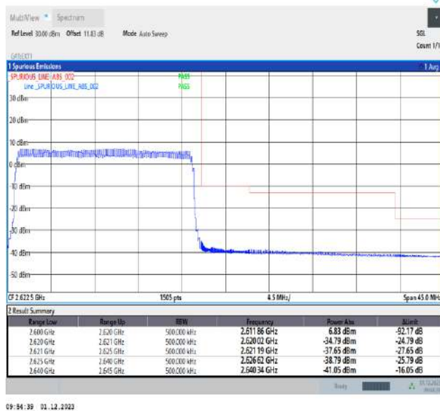
Band38_20MHz_16QAM_38150_100RB#0
