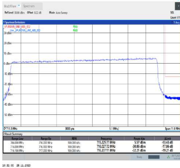
Band17_10MHz_QPSK_23800_50RB#0
