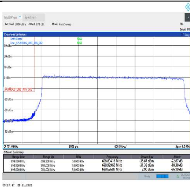
Band12_5MHz_64QAM_23035_25RB#0
