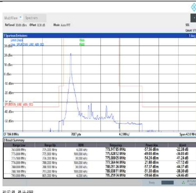
Band13_10MHz_QPSK_23230_1RB#0
