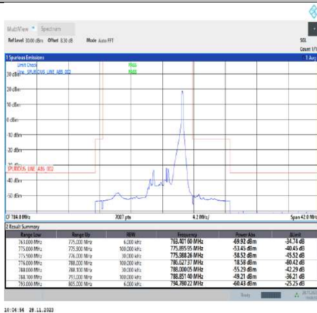
Band13_5MHz_16QAM_23255_1RB#24
