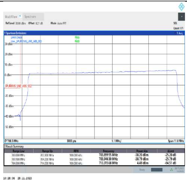
Band17_10MHz_QPSK_23780_50RB#0
