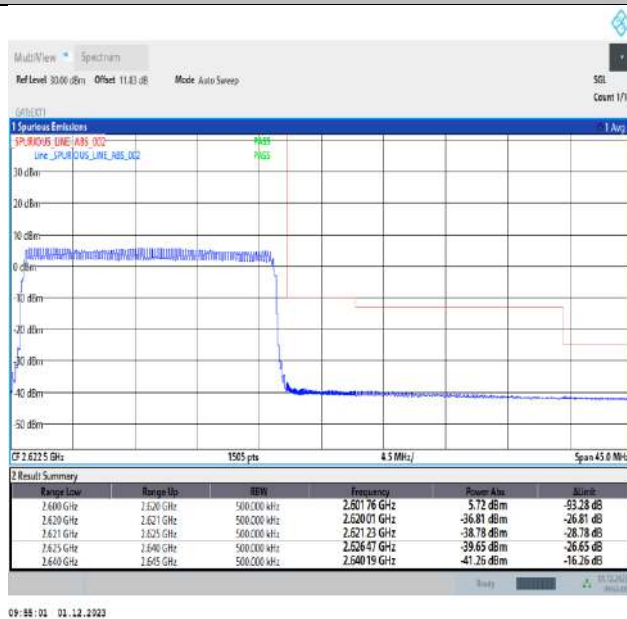
Band38_20MHz_64QAM_38150_100RB#0
