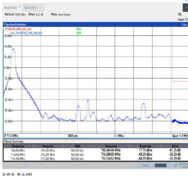
Band17_10MHz_64QAM_23800_1RB#0
