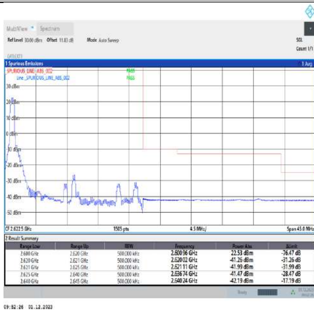
Band38_20MHz_16QAM_38150_1RB#0
