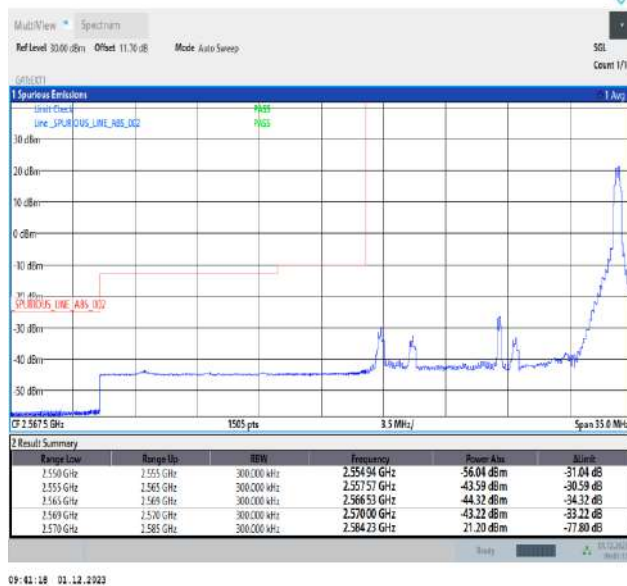
Band38_15MHz_64QAM_37825_1RB#74
