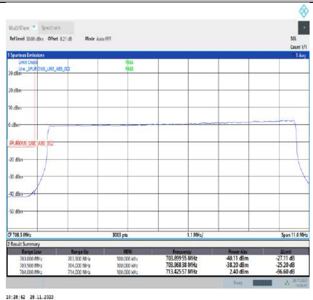
Band17_10MHz_64QAM_23780_50RB#0
