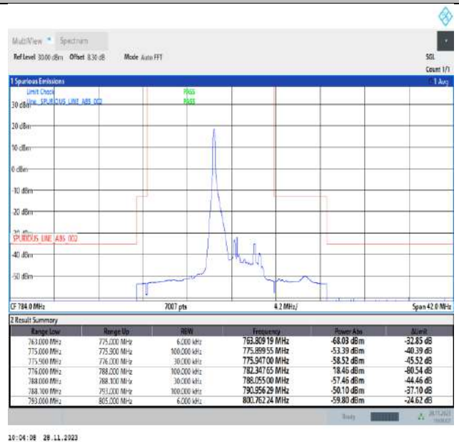
Band13_5MHz_64QAM_23255_1RB#0
