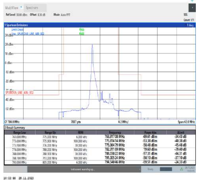
Band13_5MHz_16QAM_23255_1RB#0
