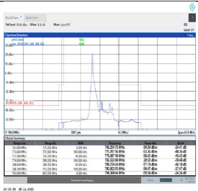
Band13_5MHz_QPSK_23255_1RB#0
