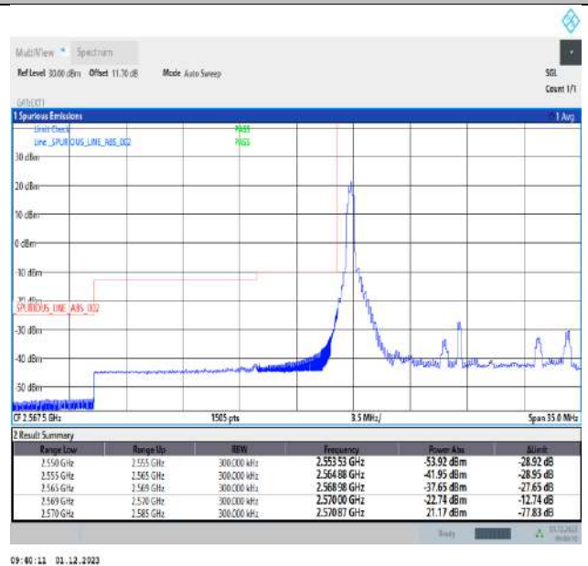
Band38_15MHz_64QAM_37825_1RB#0
