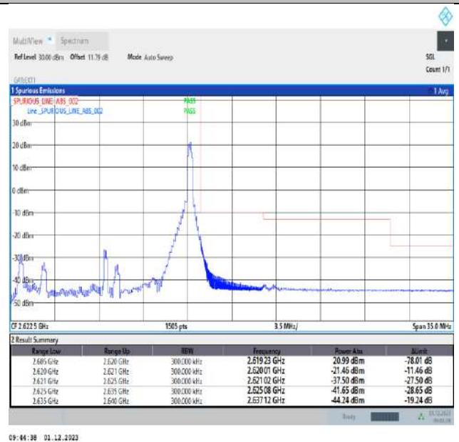
Band38_15MHz_64QAM_38175_1RB#74
