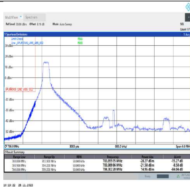
Band17_5MHz_64QAM_23755_1RB#0
