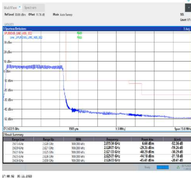
Band38_5MHz_QPSK_38225_25RB#0
