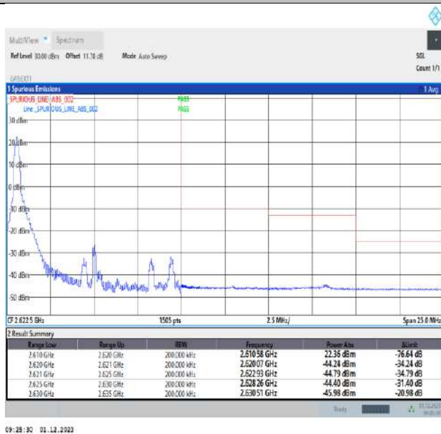
Band38_10MHz_16QAM_38200_1RB#0
