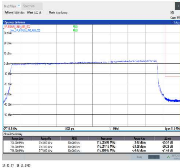
Band17_10MHz_64QAM_23800_50RB#0
