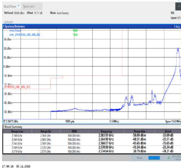
Band38_5MHz_QPSK_37775_1RB#24
