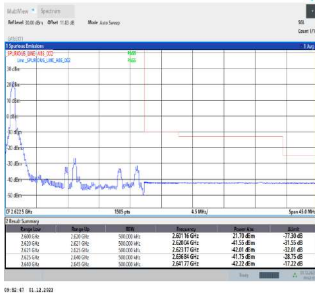
Band38_20MHz_64QAM_38150_1RB#0
