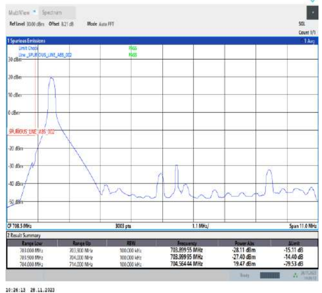
Band17_10MHz_QPSK_23780_1RB#0
