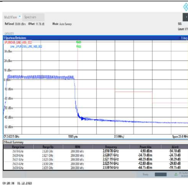
Band38_10MHz_64QAM_38200_50RB#0
