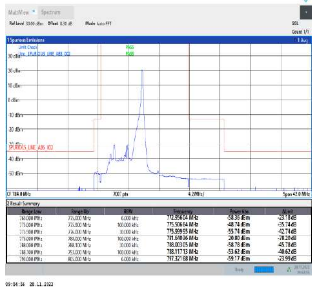
Band13_5MHz_QPSK_23205_1RB#24
