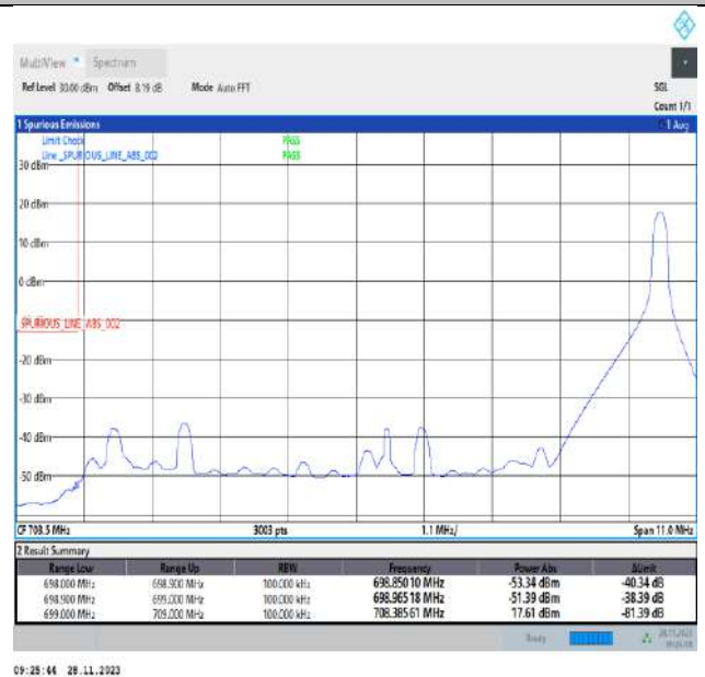
Band12_10MHz_64QAM_23060_1RB#49
