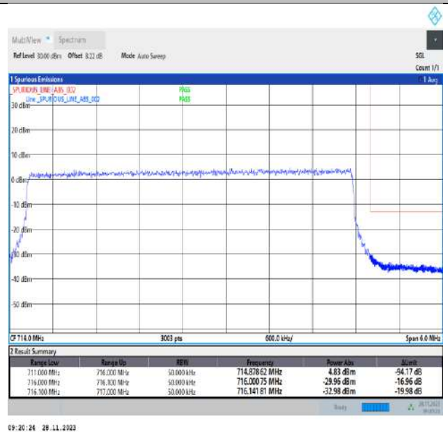
Band12_5MHz_16QAM_23155_25RB#0
