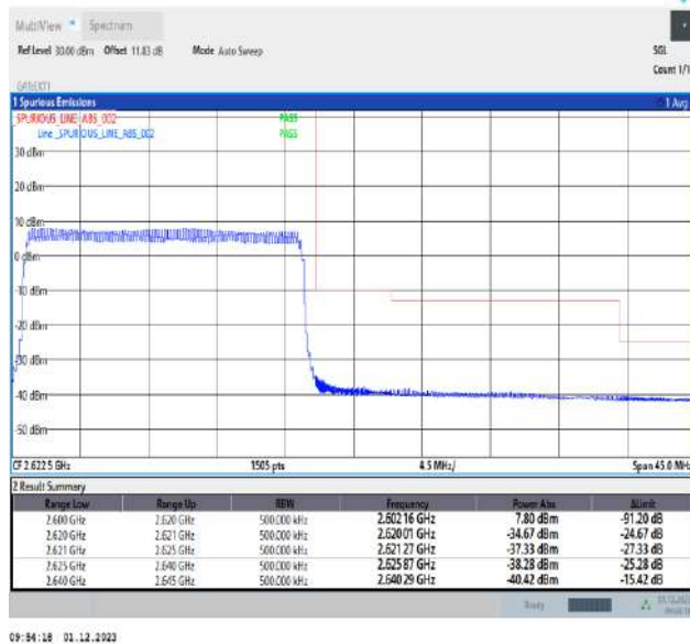
Band38_20MHz_QPSK_38150_100RB#0
