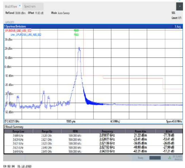
Band38_20MHz_64QAM_38150_1RB#99
