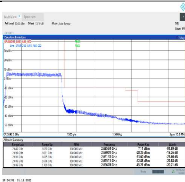
Band41_5MHz_16QAM_41565_25RB#0
