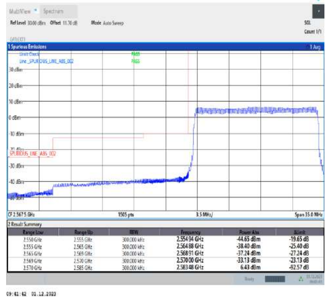
Band38_15MHz_QPSK_37825_75RB#0
