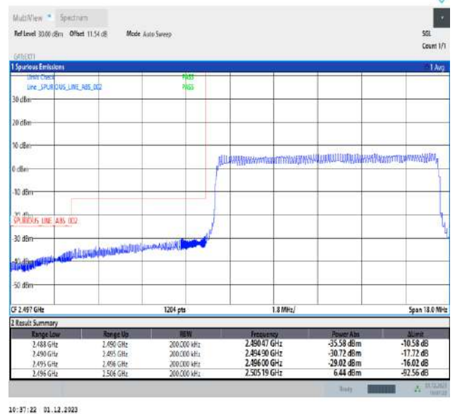
Band41_10MHz_16QAM_39700_50RB#0
