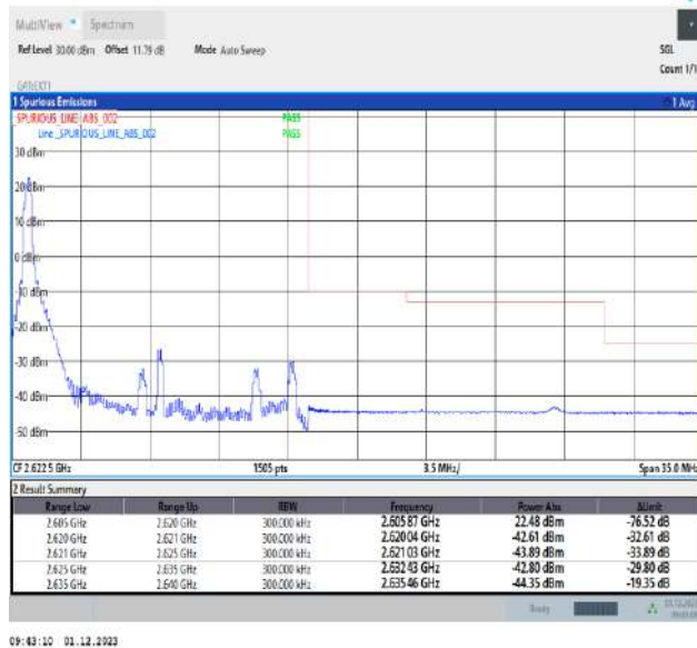
Band38_15MHz_16QAM_38175_1RB#0
