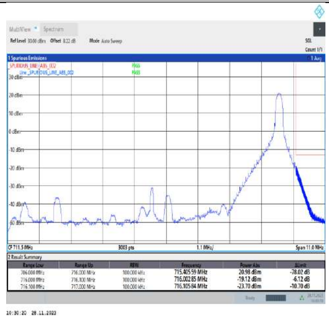
Band17_10MHz_16QAM_23800_1RB#49
