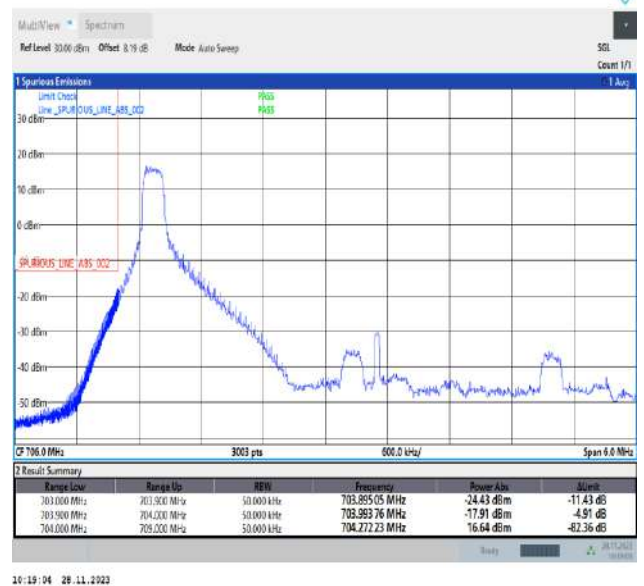
Band17_5MHz_16QAM_23755_1RB#0
