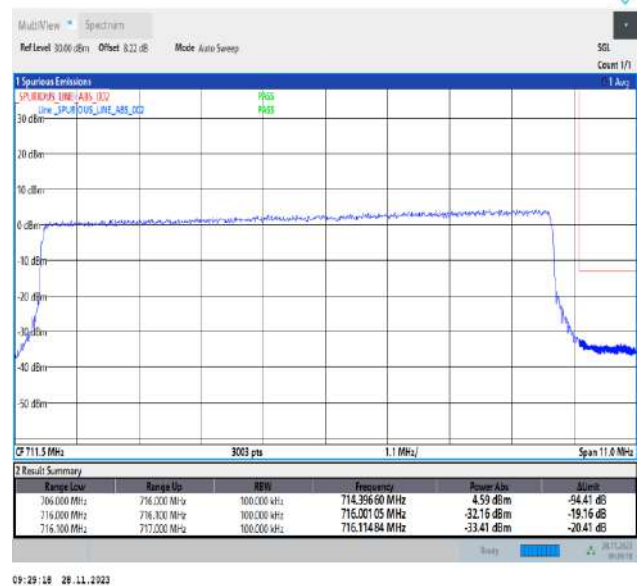
Band12_10MHz_16QAM_23130_50RB#0
