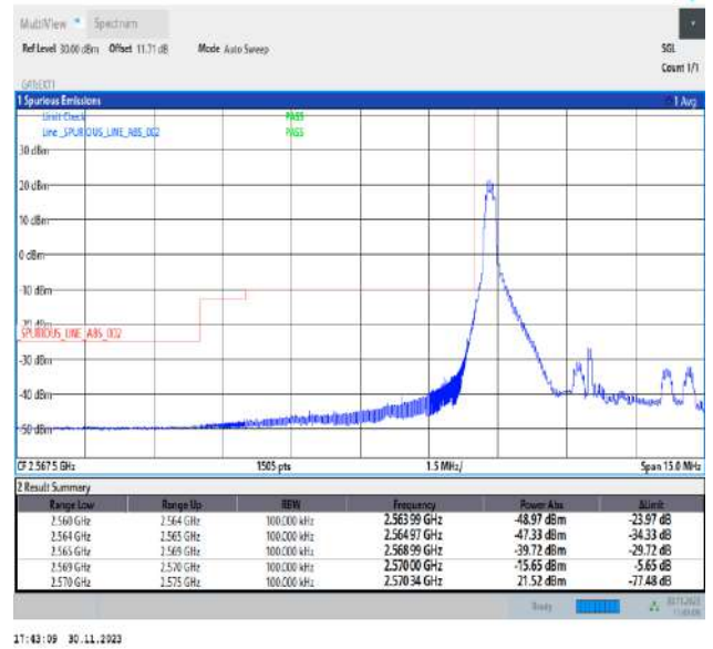
Band38_5MHz_QPSK_37775_1RB#0
