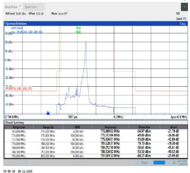
Band13_5MHz_16QAM_23205_1RB#24
