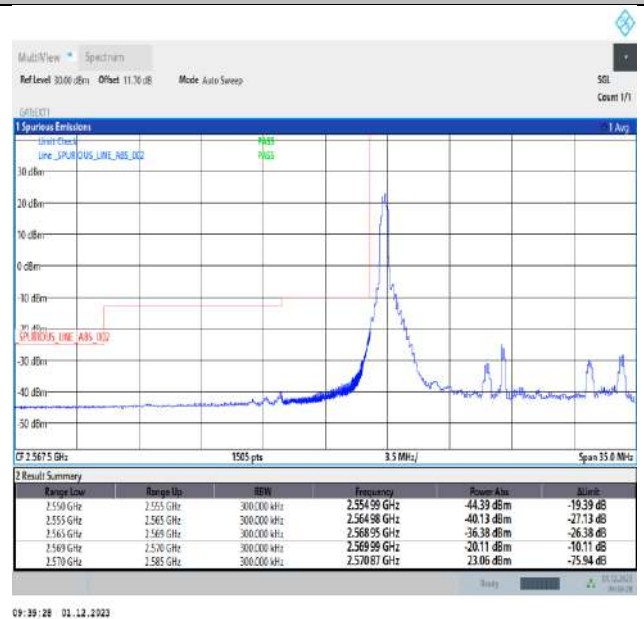
Band38_15MHz_QPSK_37825_1RB#0
