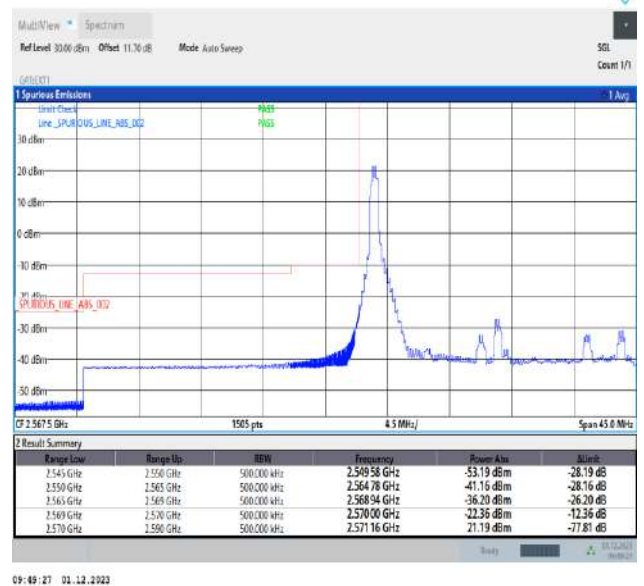
Band38_20MHz_64QAM_37850_1RB#0
