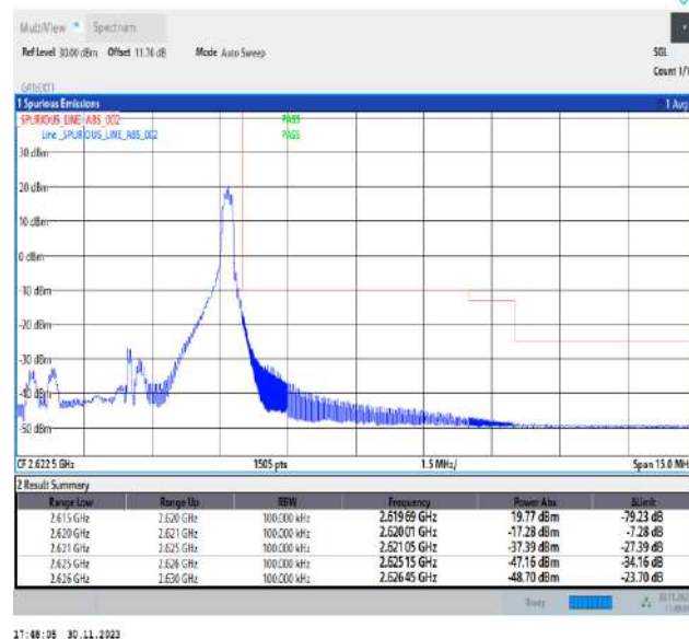
Band38_5MHz_16QAM_38225_1RB#24
