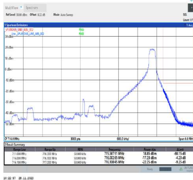
Band17_5MHz_16QAM_23825_1RB#24
