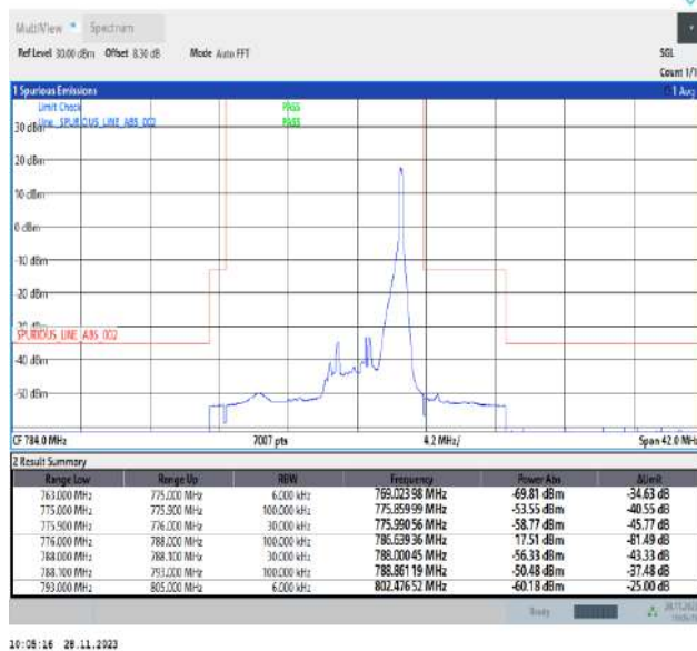
Band13_5MHz_64QAM_23255_1RB#24
