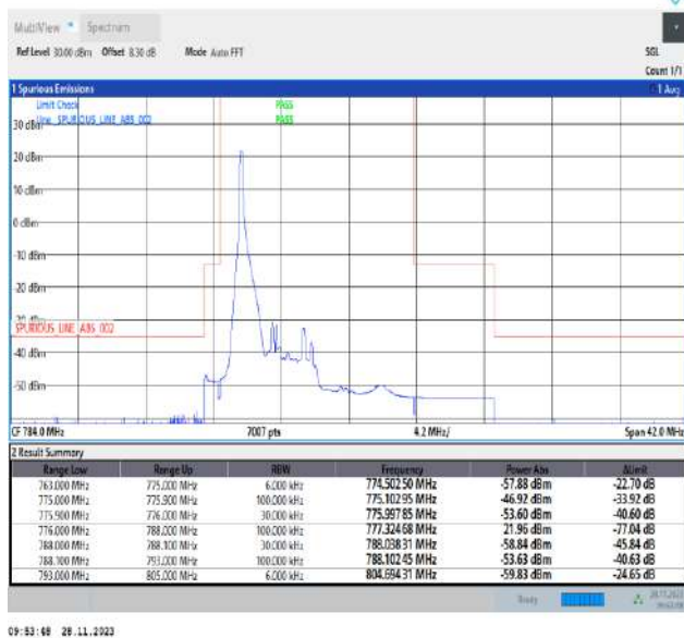
Band13_5MHz_QPSK_23205_1RB#0
