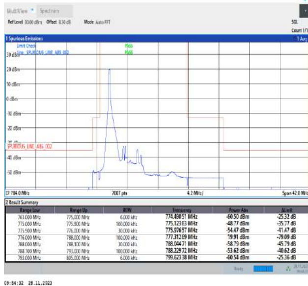
Band13_5MHz_64QAM_23205_1RB#0
