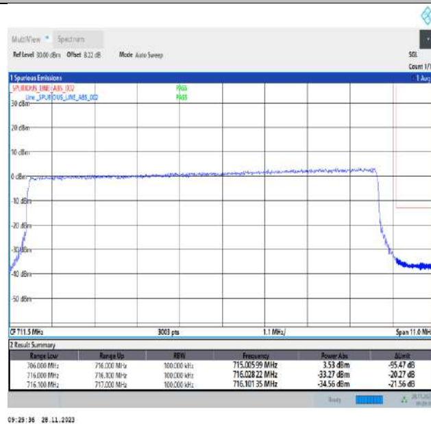
Band12_10MHz_64QAM_23130_50RB#0
