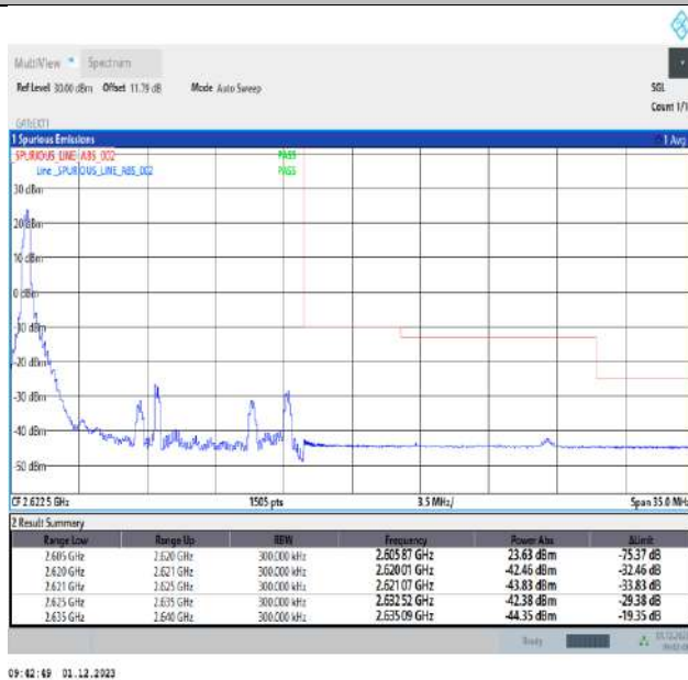
Band38_15MHz_QPSK_38175_1RB#0
