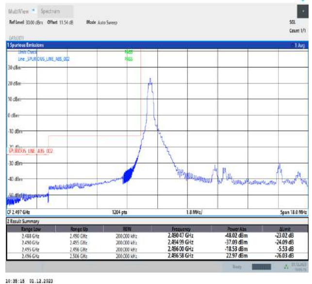
Band41_10MHz_16QAM_39700_1RB#0
