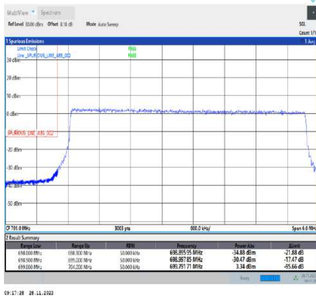
Band12_5MHz_16QAM_23035_25RB#0
