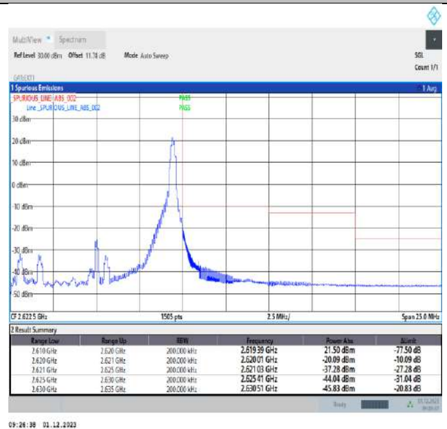
Band38_10MHz_16QAM_38200_1RB#49
