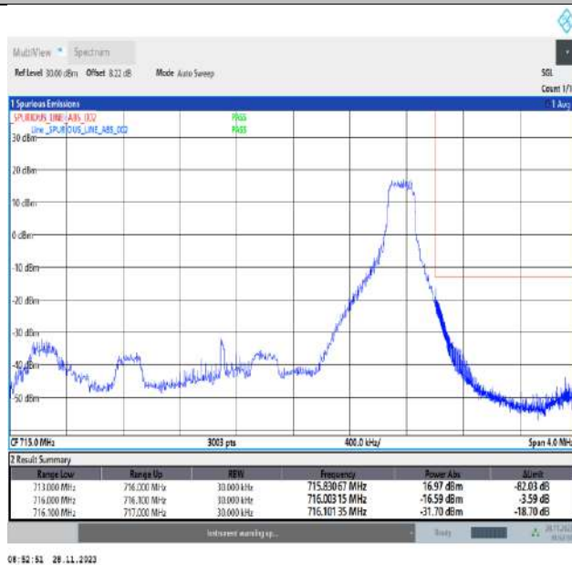
Band12_3MHz_64QAM_23165_1RB#14
