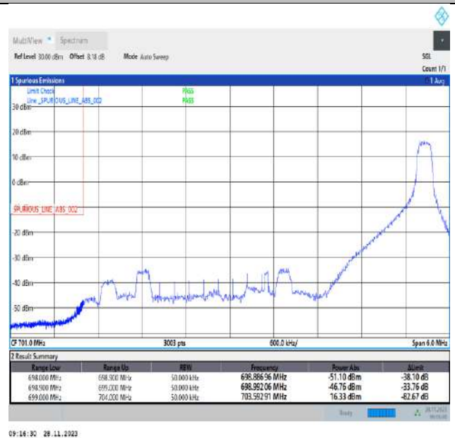
Band12_5MHz_16QAM_23035_1RB#24
