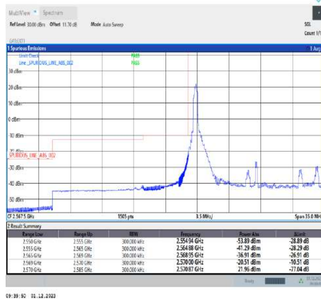
Band38_15MHz_16QAM_37825_1RB#0
