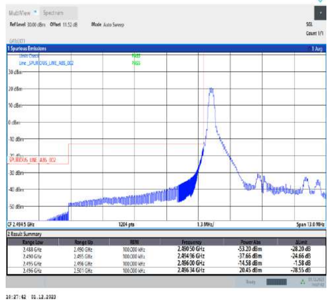
Band41_5MHz_16QAM_39675_1RB#0
