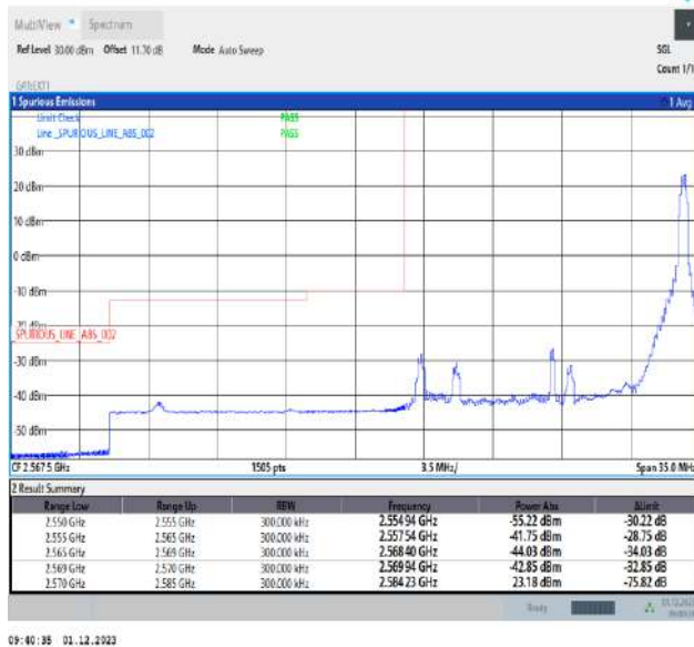
Band38_15MHz_QPSK_37825_1RB#74
