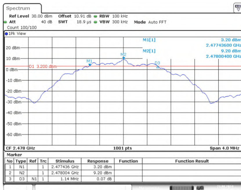
Fig.12 6dB Bandwidth (CH38), LE 2M
