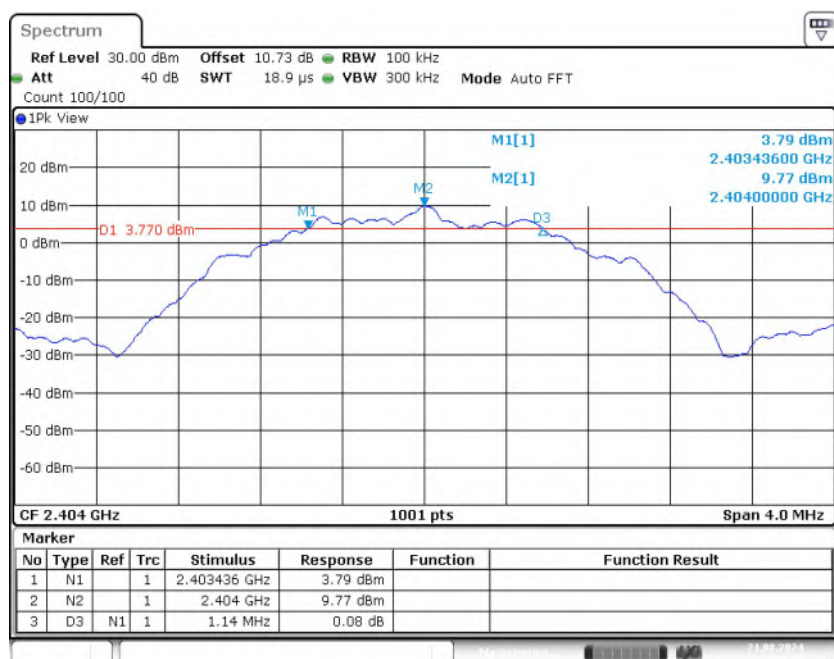
Fig.10 6dB Bandwidth (CH1), LE 2M
