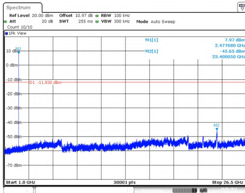
Fig.22 Conducted Spurious Emission (CH38, 1GHz-26.5GHz), LE 2M
