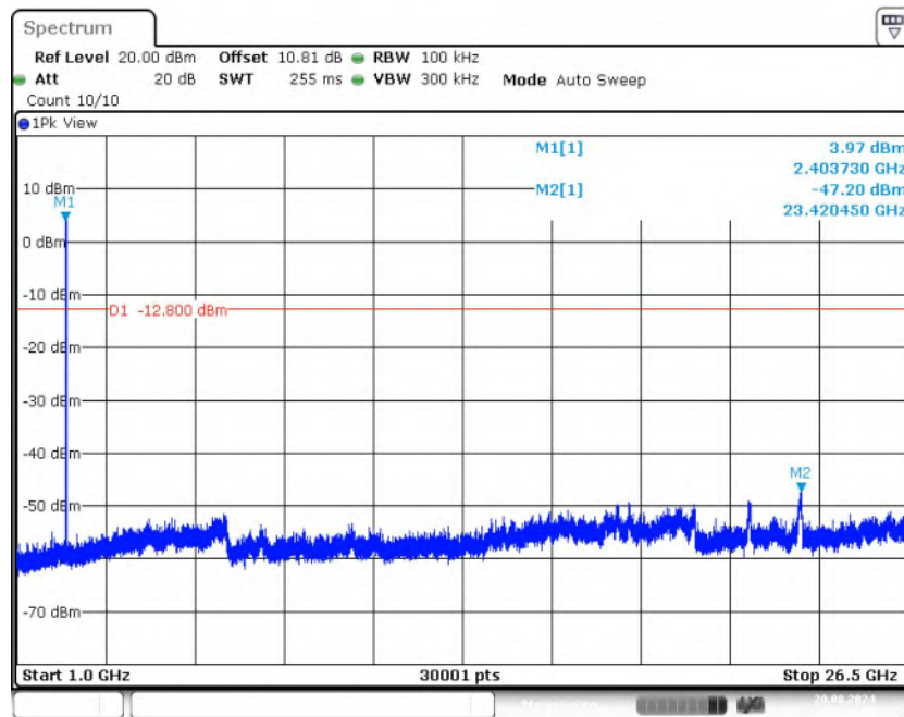
Fig.20 Conducted Spurious Emission (CH1, 1GHz-26.5GHz), LE 2M
