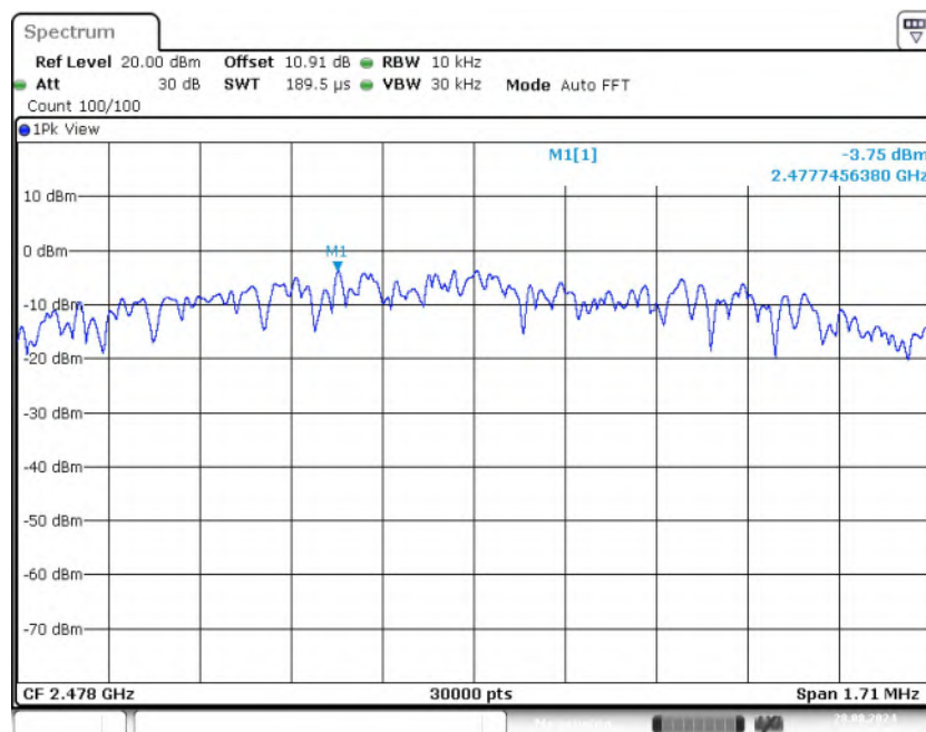
Fig.6 Power Spectral Density (CH38), LE 2M
