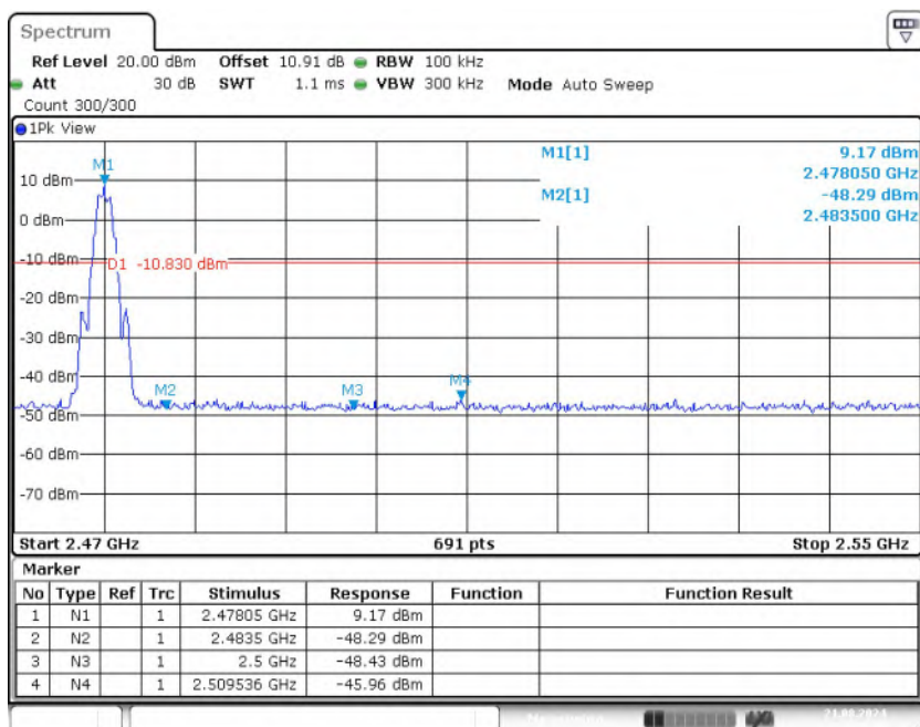
Fig.16 Band Edges (CH38), LE 2M
