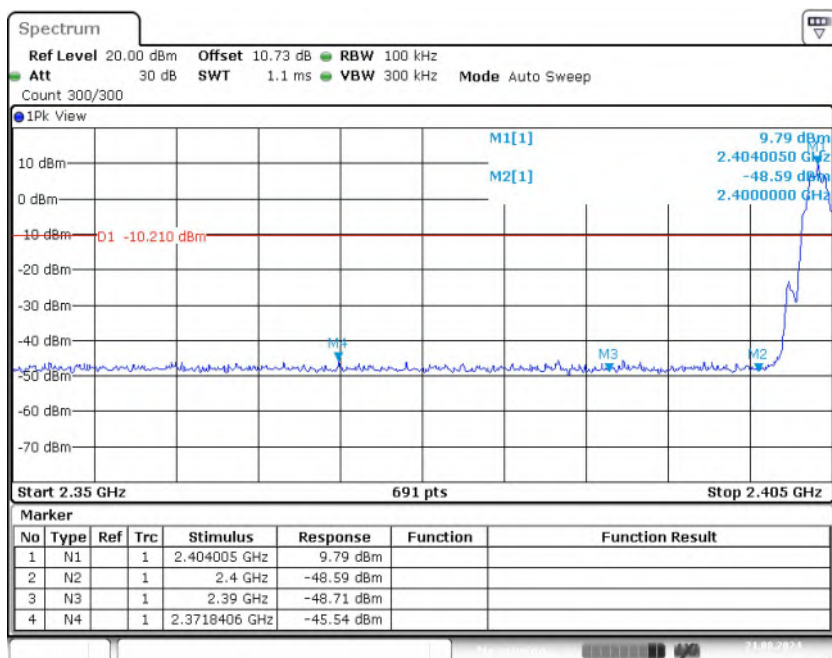
Fig.15 Band Edges (CH1), LE 2M
