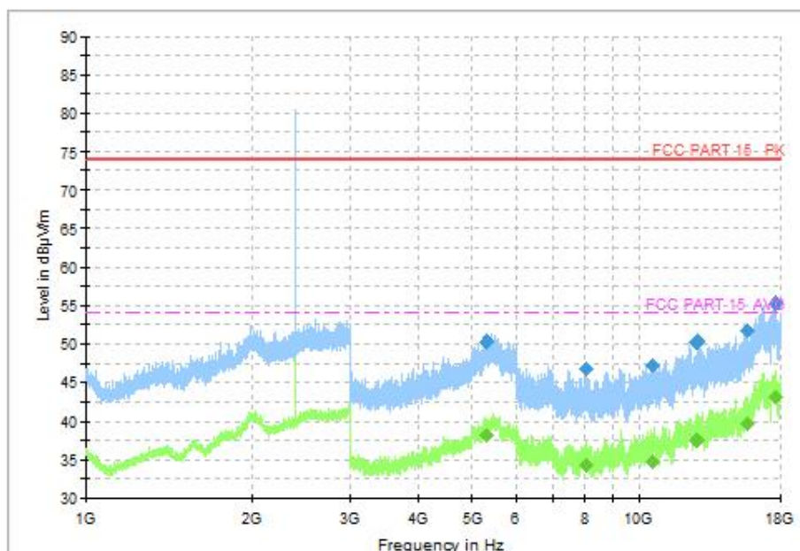
Fig.29 Radiated Spurious Emission (CH1, 1GHz ~18GHz), LE 2M
