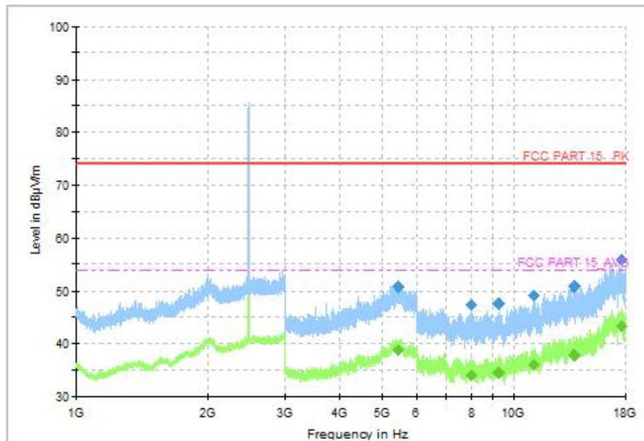
Fig.31 Radiated Spurious Emission (CH38, 1GHz ~18GHz), LE 2M
