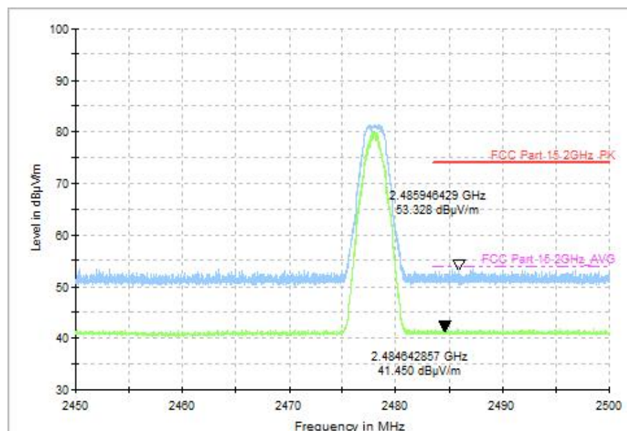
Fig.33 Radiated Band Edges (CH38, 2.45GHz~2.50GHz), LE 2M
