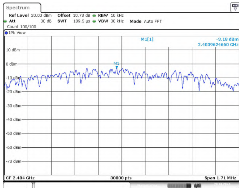
Fig.4 Power Spectral Density (CH1), LE 2M
