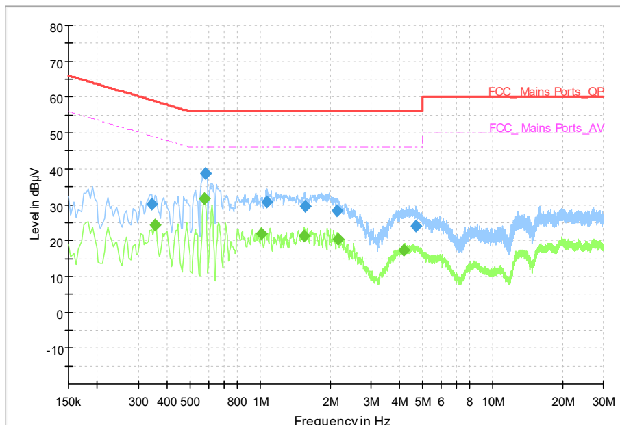
Fig. 78 AC Power line Conducted Emission (Traffic)
