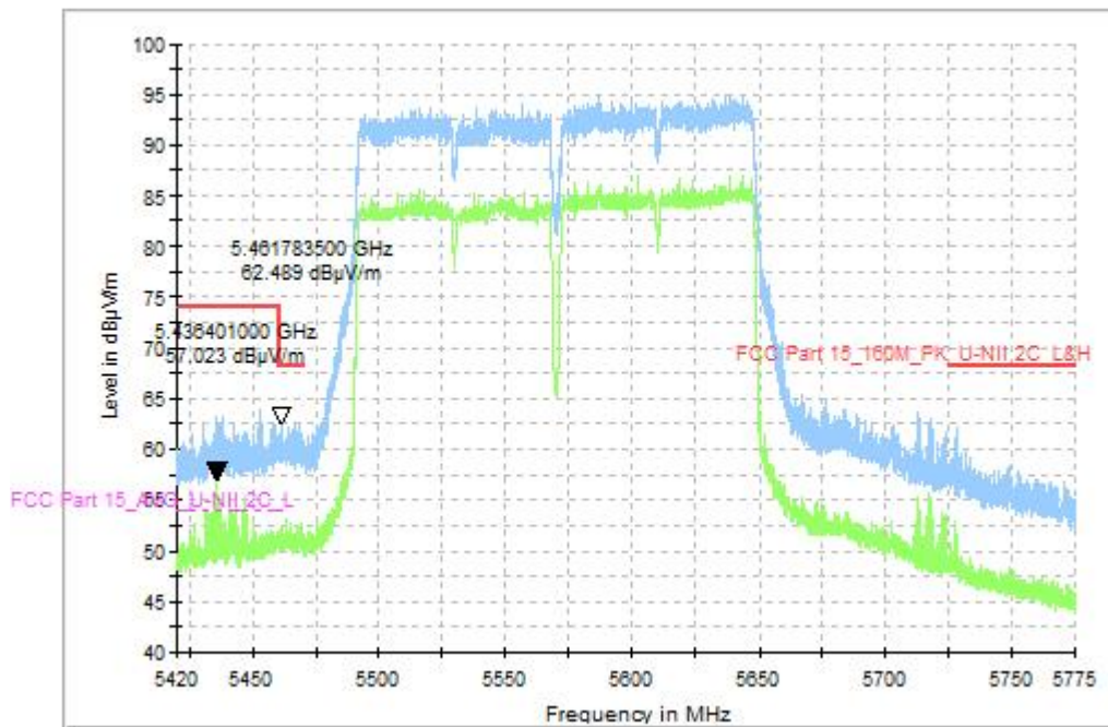
Fig. 45 Band Edges (802.11ac-VHT160, CH114 5570MHz), MIMO
