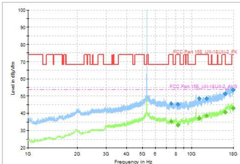
Fig. 51 Transmitter Spurious Emission (802.11n-HT20, CH64 5320MHz, 1GHz-18GHz), MIMO
