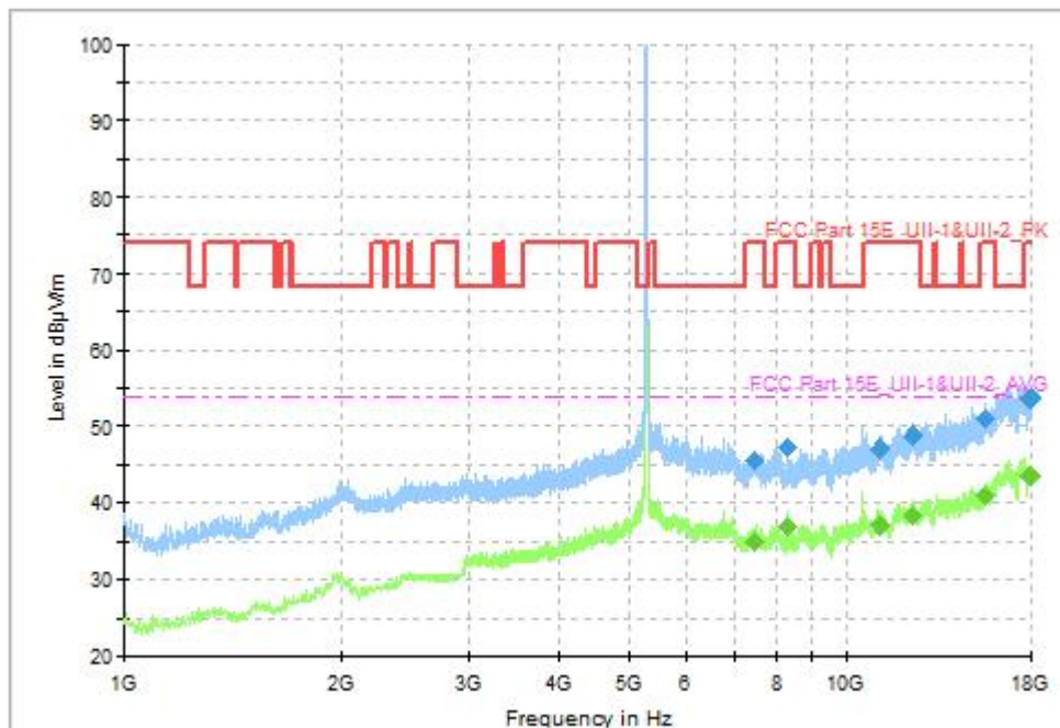
Fig. 50 Transmitter Spurious Emission (802.11n-HT20, CH56 5280MHz, 1GHz-18GHz), MIMO
