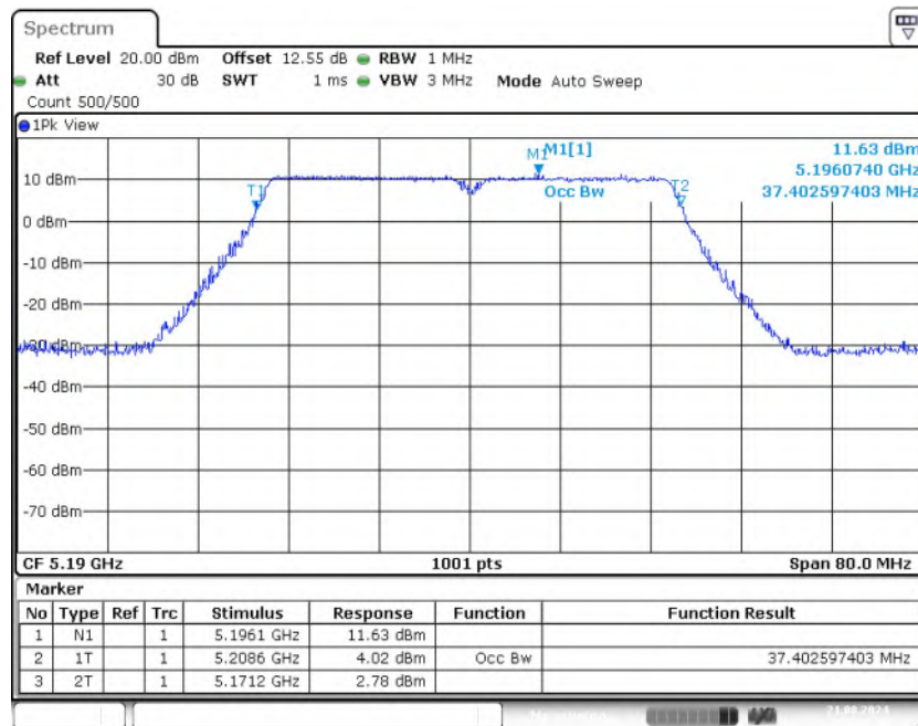
Fig. 17 99% Occupied Bandwidth (802.11ac-VHT40, 5190MHz)
