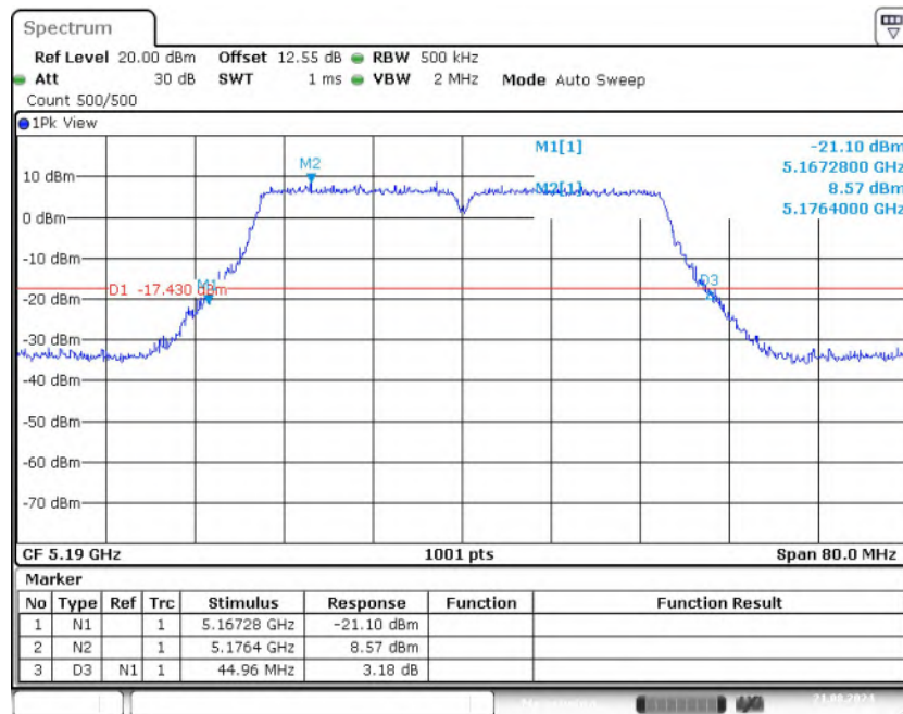
Fig. 3 Occupied 26dB Bandwidth (802.11ac-VHT40, 5190MHz)
