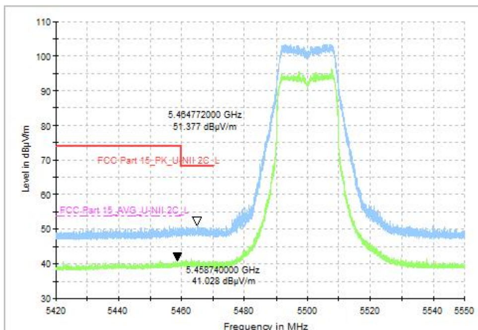
Fig. 29 Band Edges (802.11n-HT20, CH100 5500MHz), MIMO
