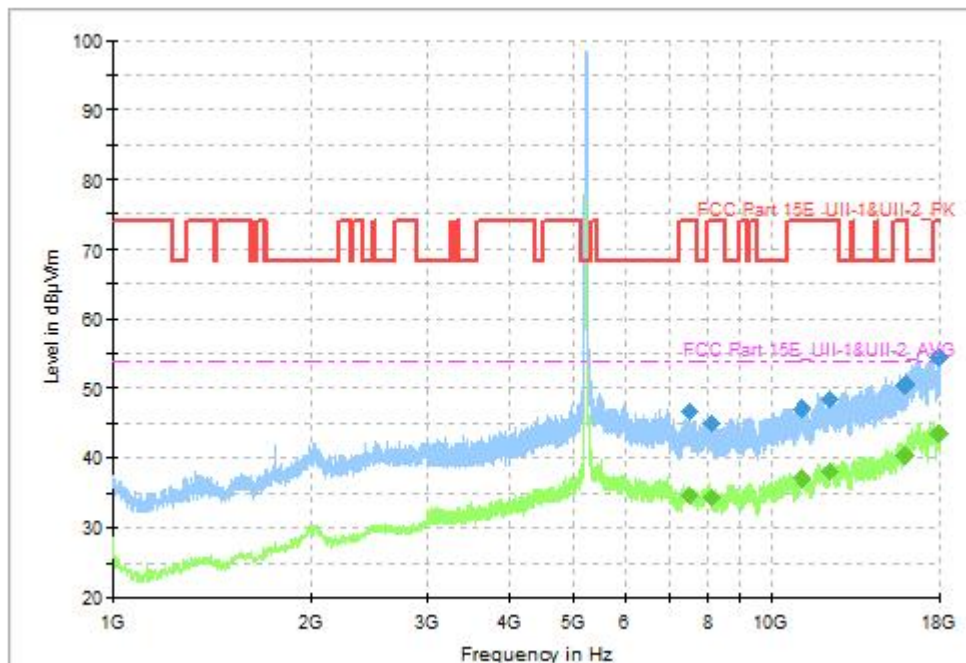
Fig. 59 Transmitter Spurious Emission (802.11ac-VHT40, CH46 5230MHz, 1GHz-18GHz), MIMO
