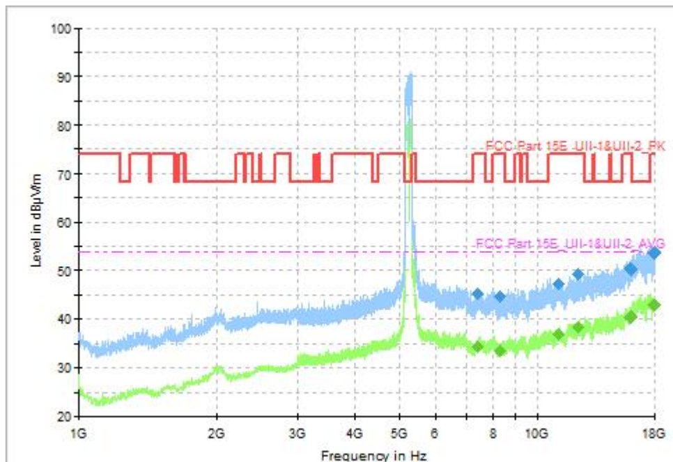
Fig. 72 Transmitter Spurious Emission (802.11ac-VHT160, CH50 5250MHz, 1GHz-18GHz), MIMO
