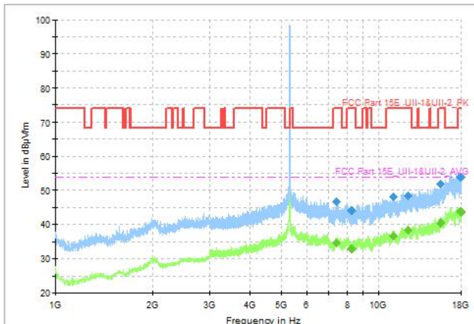
Fig. 61 Transmitter Spurious Emission (802.11ac-VHT40, CH62 5310MHz, 1GHz-18GHz), MIMO
