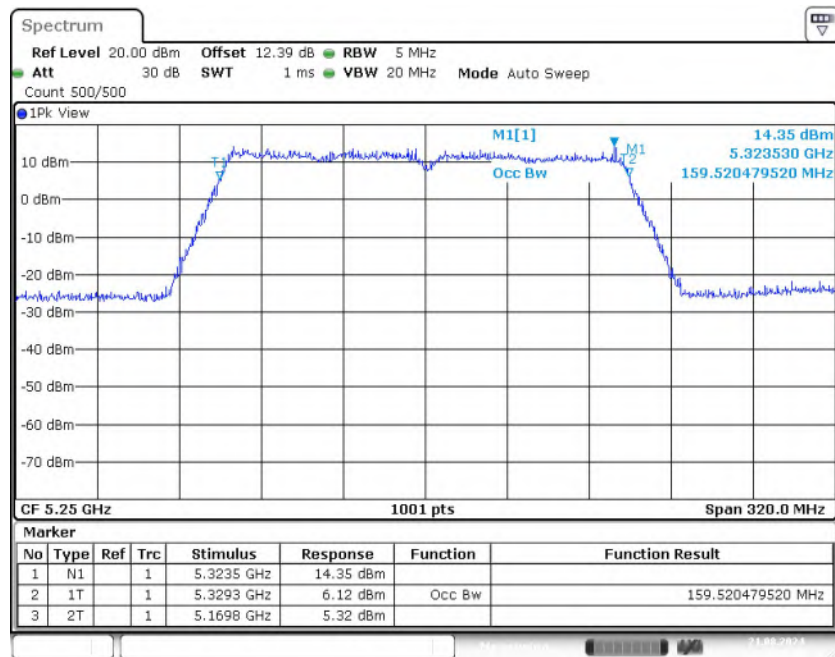
Fig. 21 99% Occupied Bandwidth (802.11ac-VHT160, 5250MHz)
