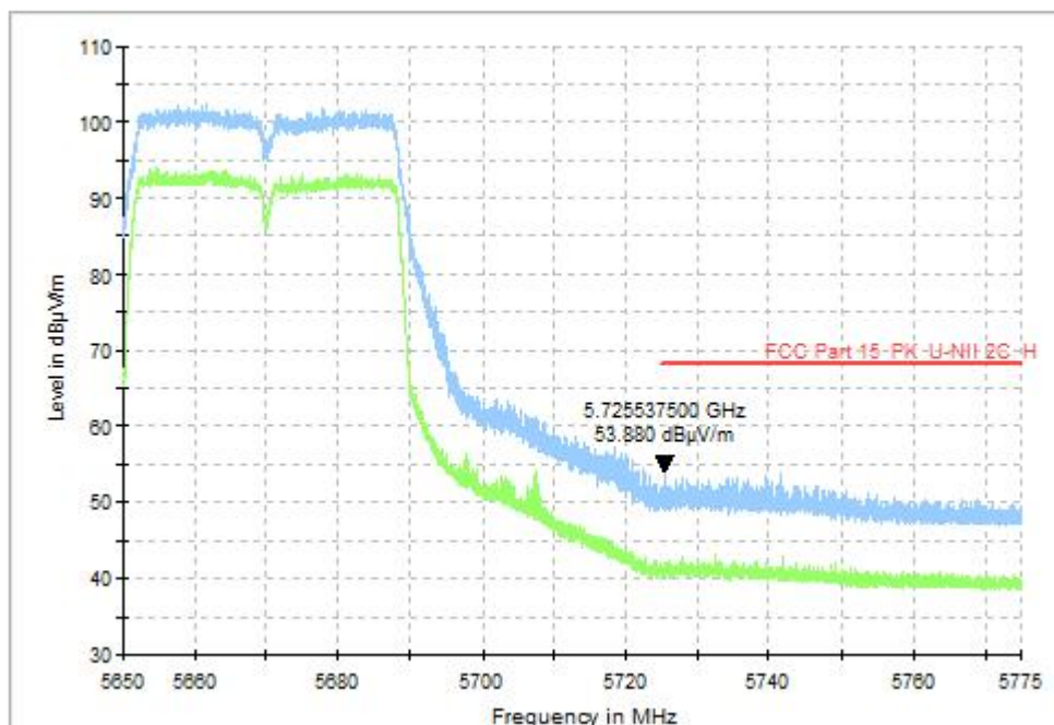
Fig. 36 Band Edges (802.11ac-VHT40, CH134 5670MHz), MIMO
