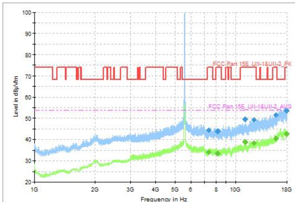
Fig. 63 Transmitter Spurious Emission (802.11ac-VHT40, CH118 5580MHz, 1GHz-18GHz), MIMO
