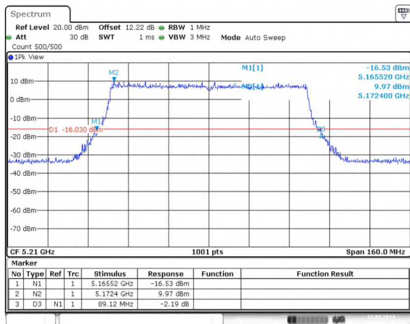
Fig. 5 Occupied 26dB Bandwidth (802.11be-EHT80, 5210MHz)
