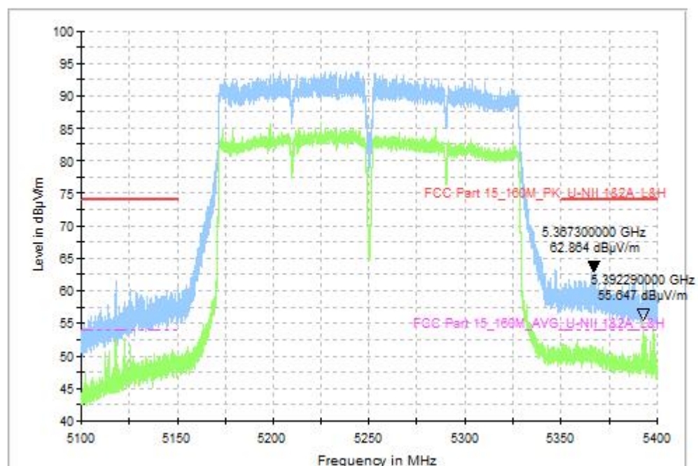
Fig. 44 Band Edges (802.11ac-VHT160, CH50 5250MHz), MIMO
