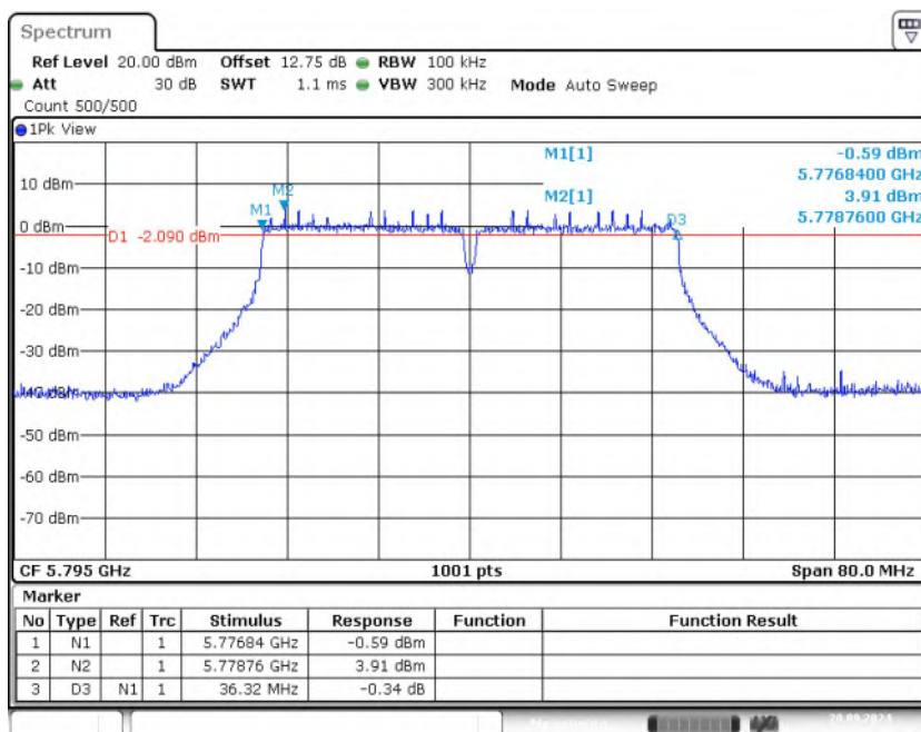
Fig. 13 Occupied 6dB Bandwidth (802.11ac-VHT40, 5795MHz)
