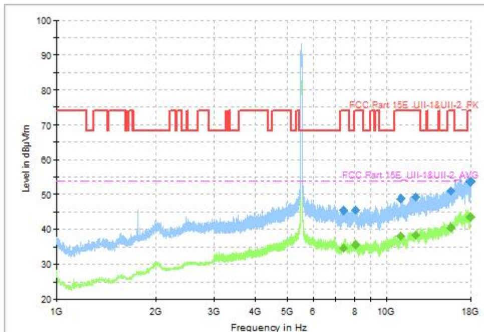
Fig. 69 Transmitter Spurious Emission (802.11be-EHT80, CH106 5530MHz, 1GHz-18GHz), MIMO
