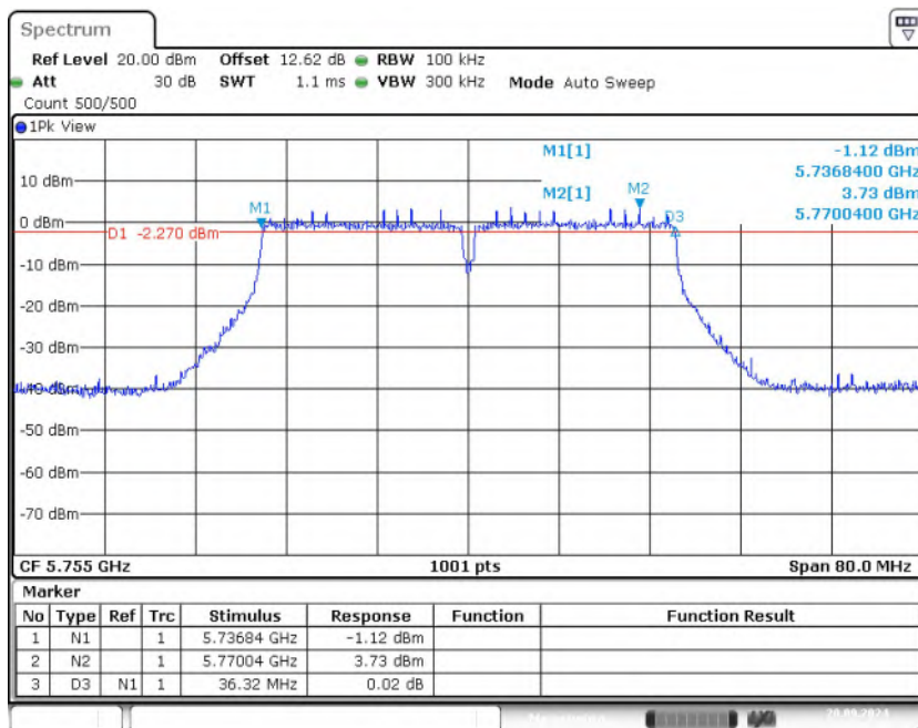
Fig. 12 Occupied 6dB Bandwidth (802.11ac-VHT40, 5755MHz)
