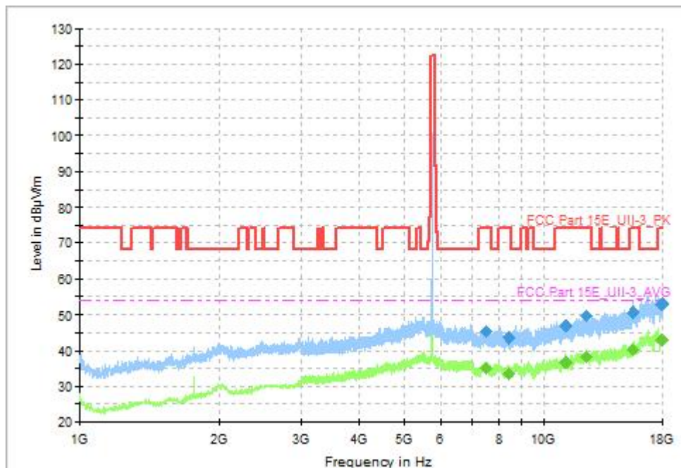
Fig. 55 Transmitter Spurious Emission (802.11n-HT20, CH149 5745MHz, 1GHz-18GHz), MIMO
