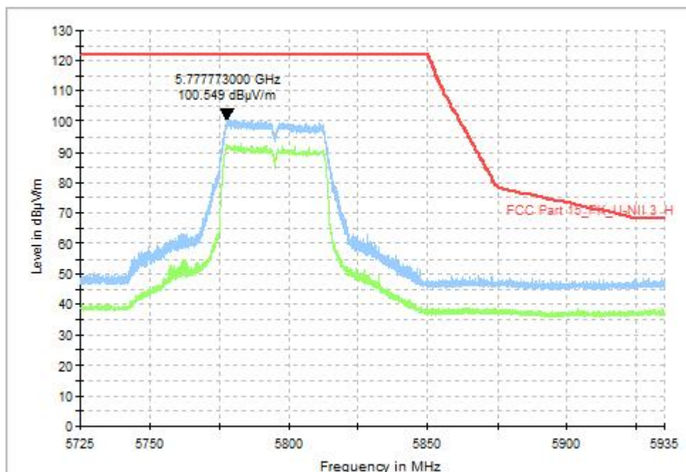
Fig. 38 Band Edges (802.11ac-VHT40, CH159 5795MHz), MIMO
