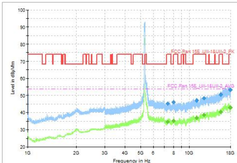
Fig. 68 Transmitter Spurious Emission (802.11be-EHT80, CH58 5290MHz, 1GHz-18GHz), MIMO
