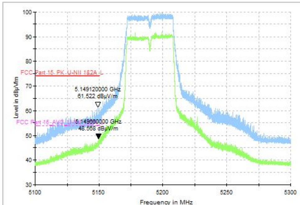
Fig. 33 Band Edges (802.11ac-VHT40, CH38 5190MHz), MIMO
