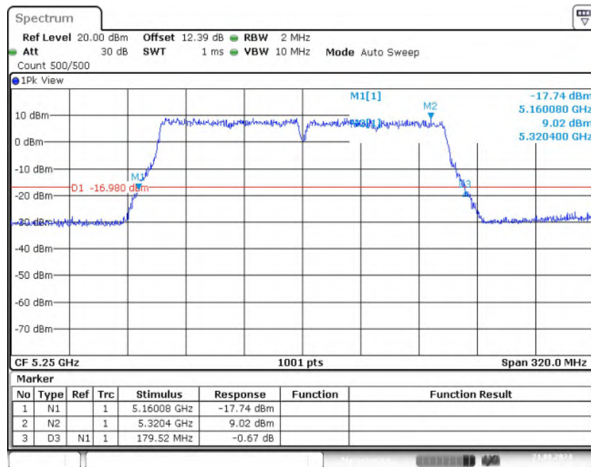
Fig. 7 Occupied 26dB Bandwidth (802.11ac-VHT160, 5250MHz)
