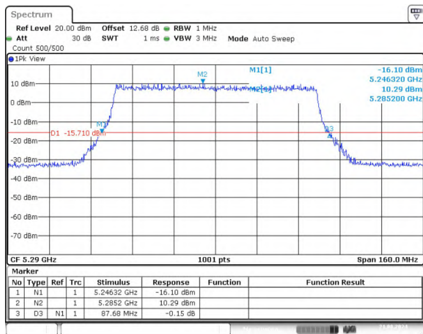
Fig. 6 Occupied 26dB Bandwidth (802.11be-EHT80, 5290MHz)
