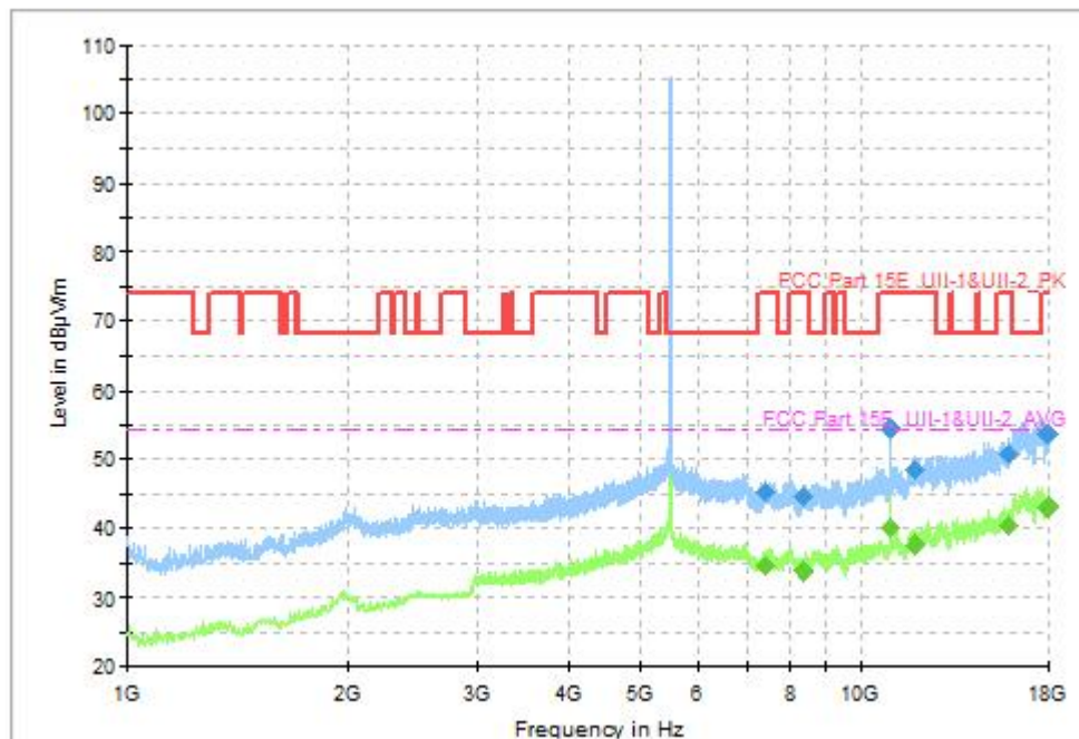
Fig. 52 Transmitter Spurious Emission (802.11n-HT20, CH100 5500MHz, 1GHz-18GHz), MIMO
