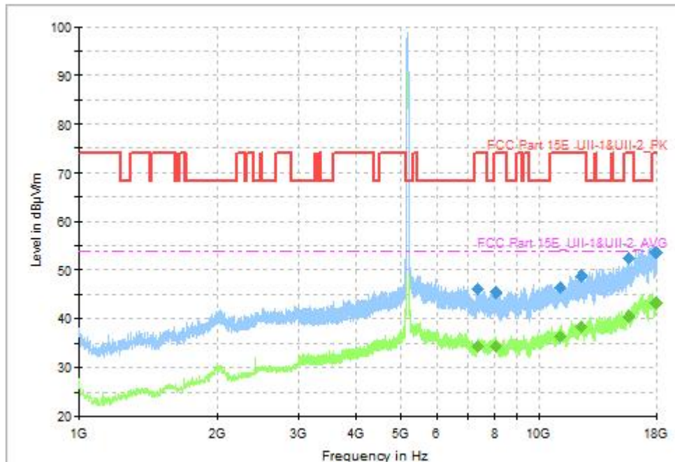
Fig. 58 Transmitter Spurious Emission (802.11ac-VHT40, CH38 5190MHz, 1GHz-18GHz), MIMO
