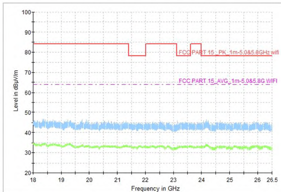
Fig. 75 Transmitter Spurious Emission (All channel, 18GHz~26.5GHz), MIMO
