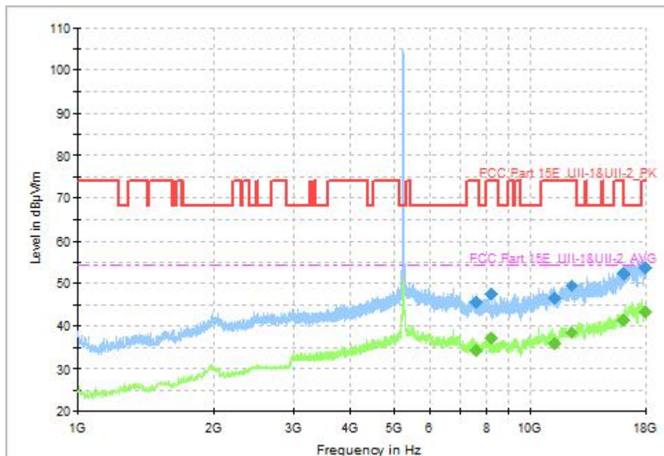
Fig. 48 Transmitter Spurious Emission (802.11n-HT20, CH48 5240MHz, 1GHz-18GHz), MIMO
