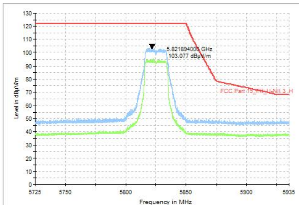
Fig. 32 Band Edges (802.11n-HT20, CH165 5825MHz), MIMO
