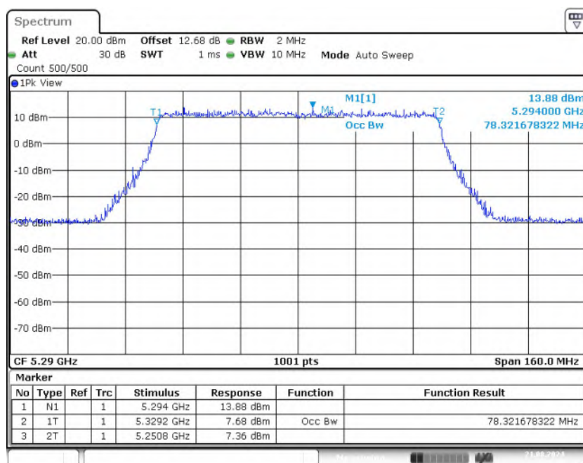
Fig. 20 99% Occupied Bandwidth (802.11be-EHT80, 5290MHz)
