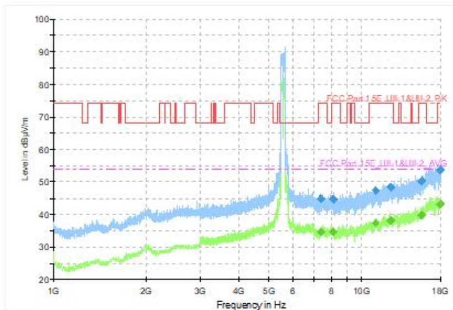
Fig. 73 Transmitter Spurious Emission (802.11ac-VHT160, CH114 5570MHz, 1GHz-18GHz), MIMO
