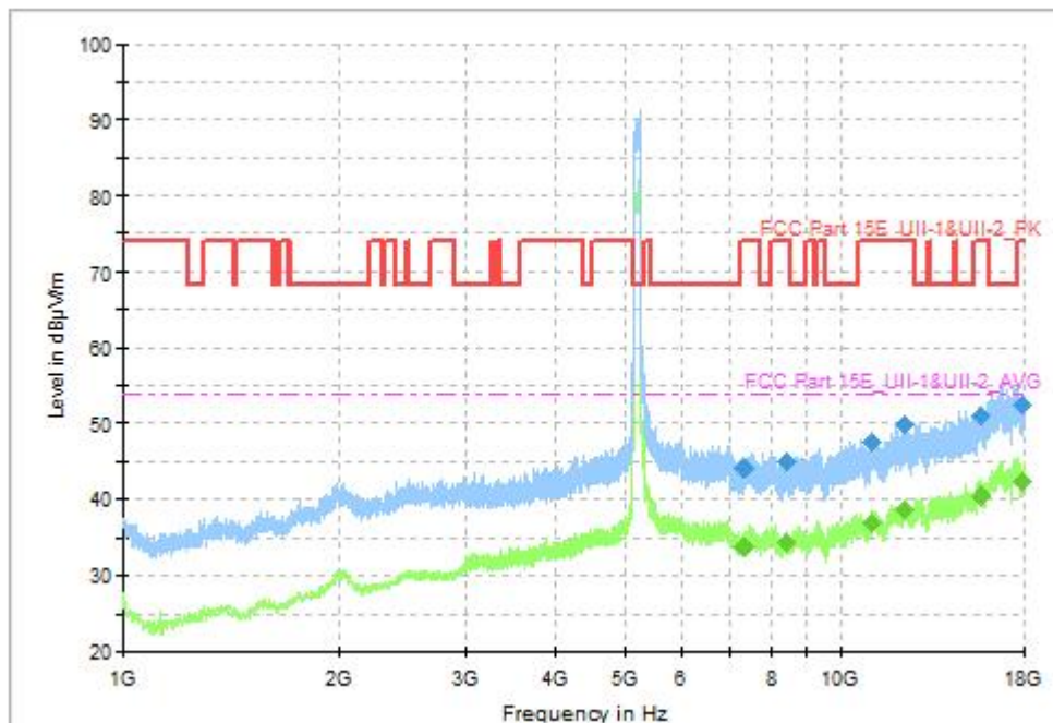
Fig. 67 Transmitter Spurious Emission (802.11be-EHT80, CH42 5210MHz, 1GHz-18GHz), MIMO
