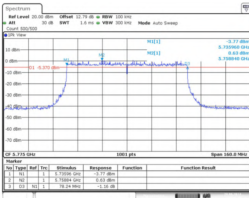
Fig. 14 Occupied 6dB Bandwidth (802.11be-EHT80, 5775MHz)
