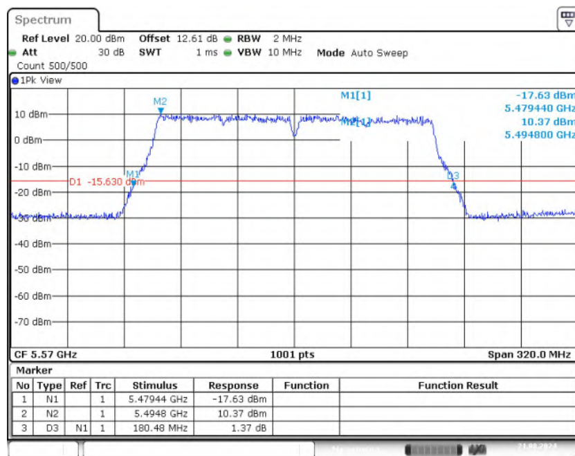
Fig. 8 Occupied 26dB Bandwidth (802.11ac-VHT160, 5570MHz)
