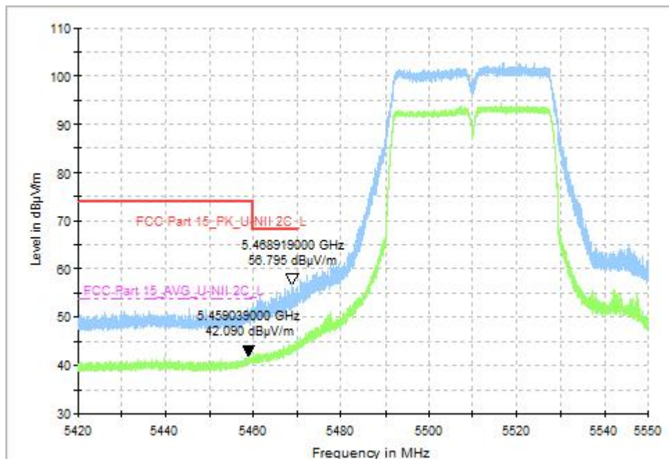
Fig. 35 Band Edges (802.11ac-VHT40, CH102 5510MHz), MIMO
