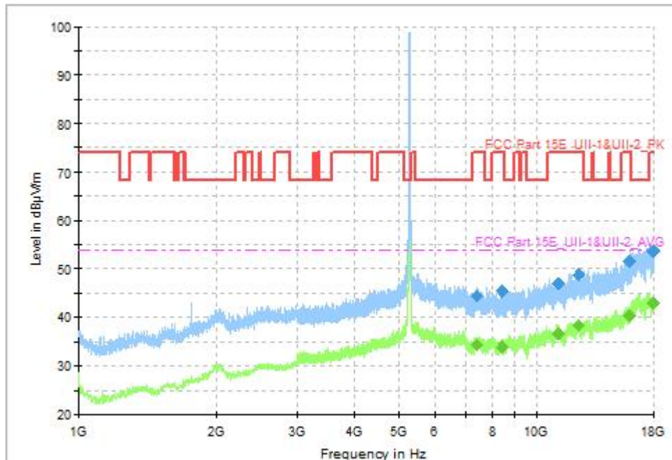
Fig. 60 Transmitter Spurious Emission (802.11ac-VHT40, CH54 5270MHz, 1GHz-18GHz), MIMO
