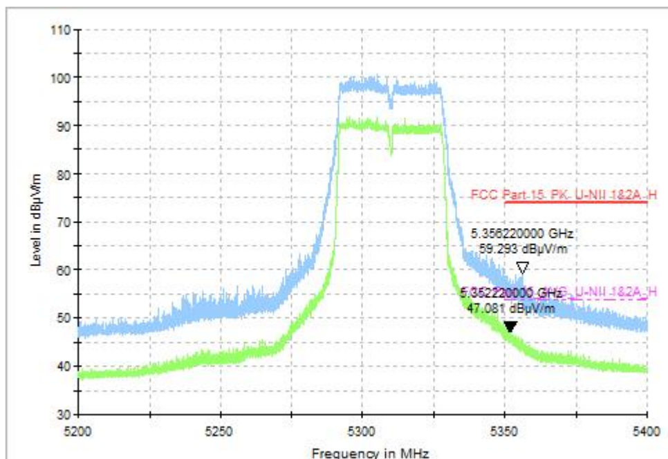
Fig. 34 Band Edges (802.11ac-VHT40, CH62 5310MHz), MIMO
