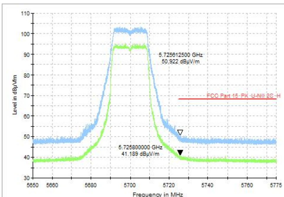
Fig. 30 Band Edges (802.11n-HT20, CH140 5700MHz), MIMO
