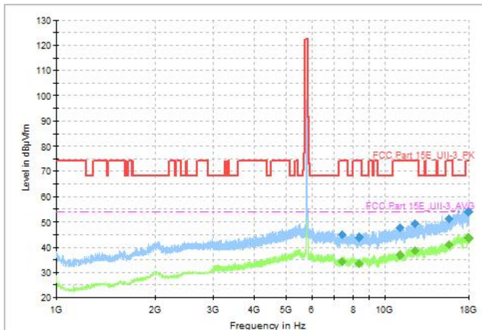
Fig. 66 Transmitter Spurious Emission (802.11ac-VHT40, CH159 5795MHz, 1GHz-18GHz), MIMO
