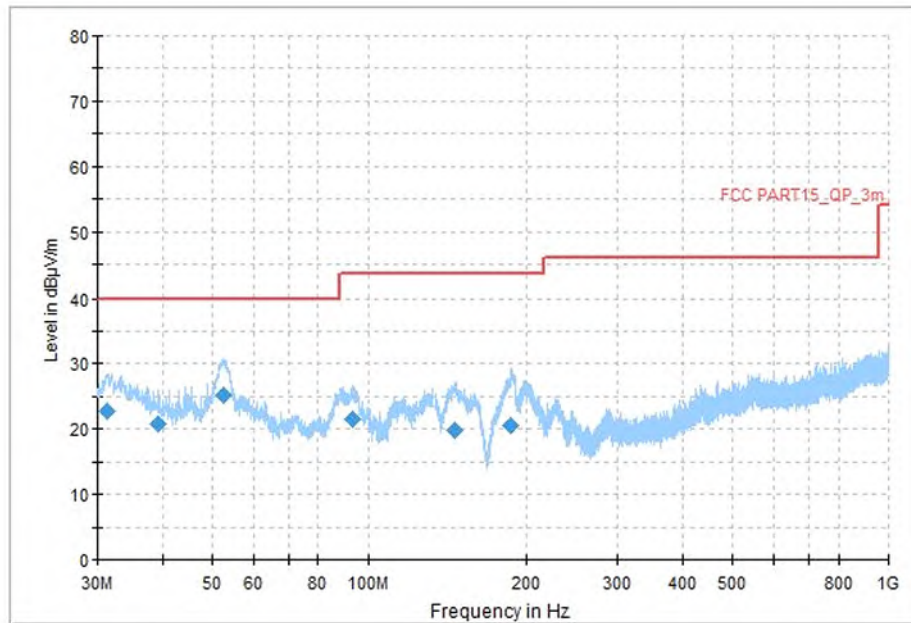
Fig. 74 Transmitter Spurious Emission (All channel, 30MHz~1GHz), MIMO
