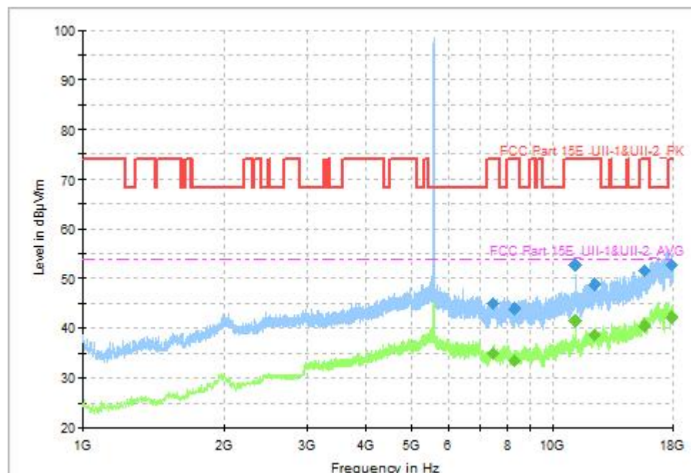
Fig. 53 Transmitter Spurious Emission (802.11n-HT20, CH120 5600MHz, 1GHz-18GHz), MIMO
