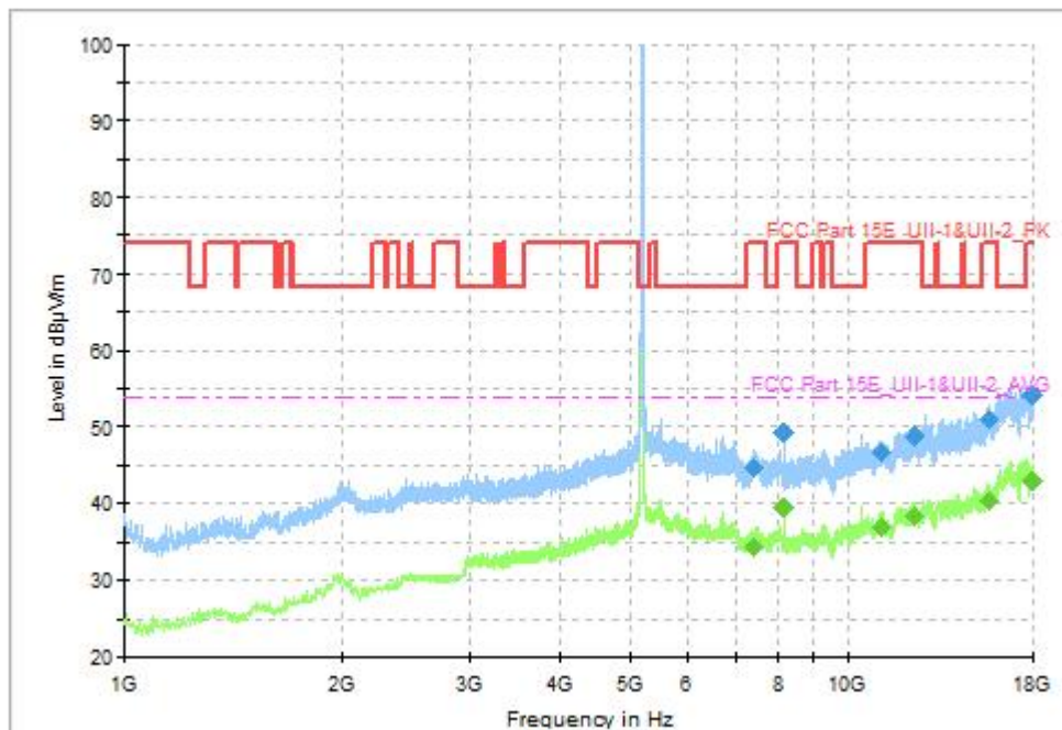
Fig. 47 Transmitter Spurious Emission (802.11n-HT20, CH40 5200MHz, 1GHz-18GHz), MIMO
