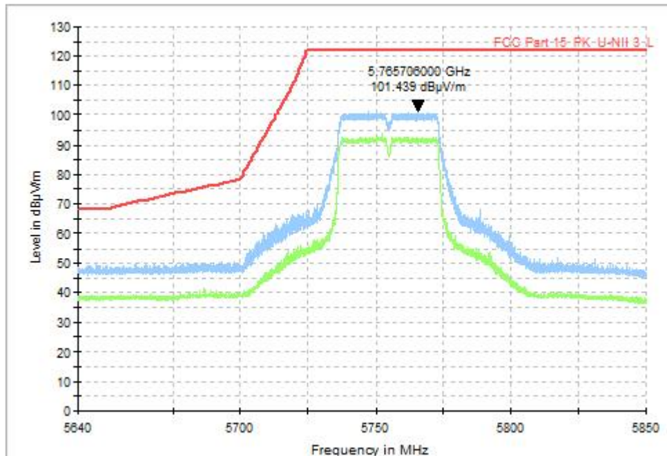
Fig. 37 Band Edges (802.11ac-VHT40, CH151 5755MHz), MIMO
