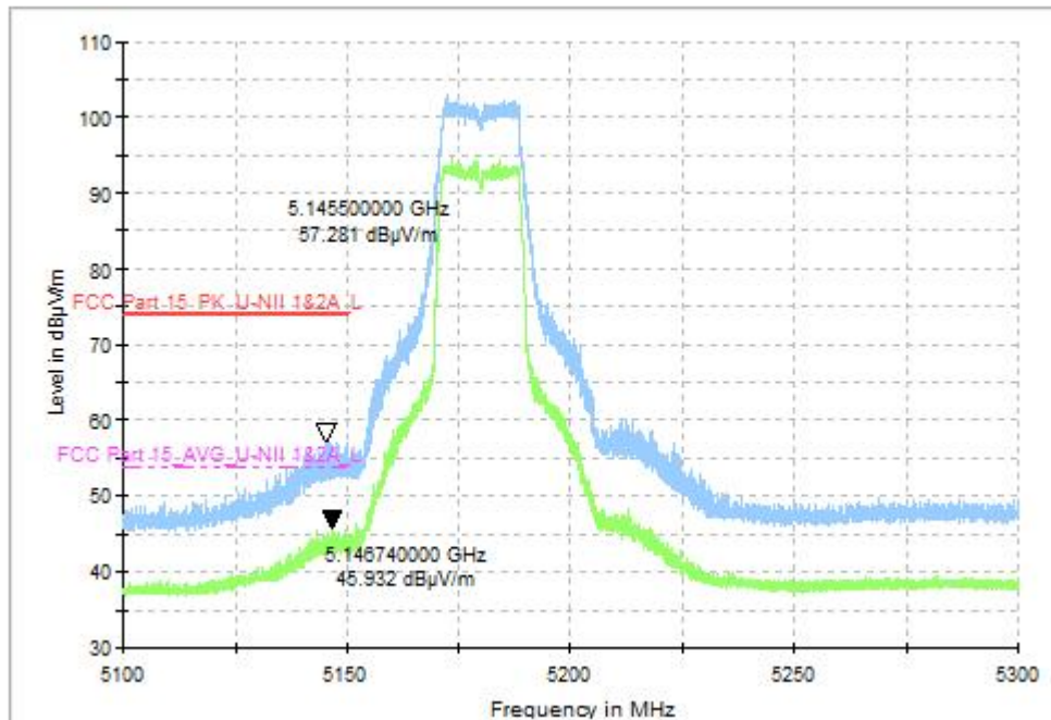
Fig. 27 Band Edges (802.11n-HT20, CH36 5180MHz), MIMO
