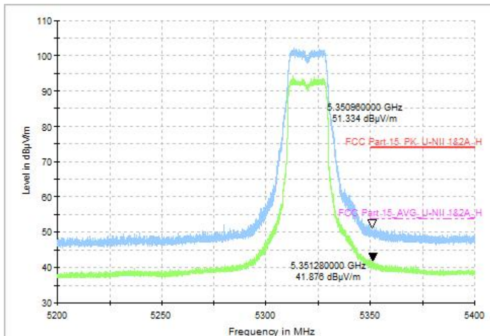
Fig. 28 Band Edges (802.11n-HT20, CH64 5320MHz), MIMO
