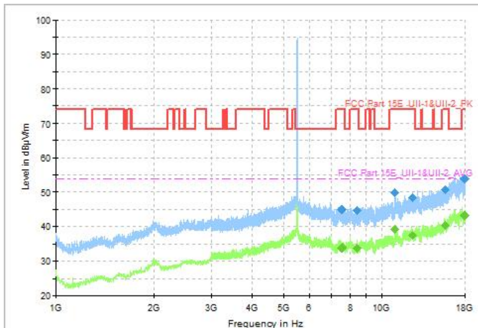
Fig. 62 Transmitter Spurious Emission (802.11ac-VHT40, CH102 5510MHz, 1GHz-18GHz), MIMO
