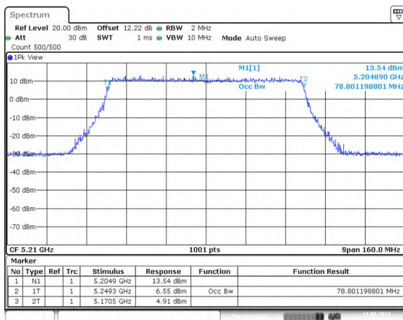
Fig. 19 99% Occupied Bandwidth (802.11be-EHT80, 5210MHz)
