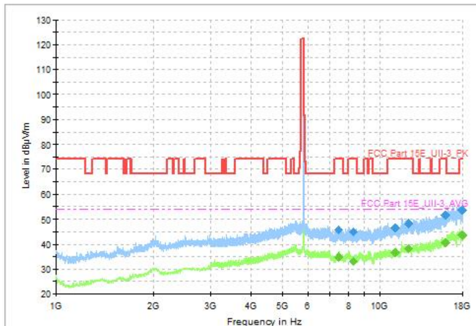
Fig. 57 Transmitter Spurious Emission (802.11n-HT20, CH165 5825MHz, 1GHz-18GHz), MIMO
