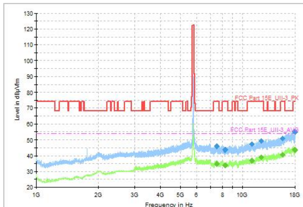
Fig. 71 Transmitter Spurious Emission (802.11be-EHT80, CH155 5775MHz, 1GHz-18GHz), MIMO
