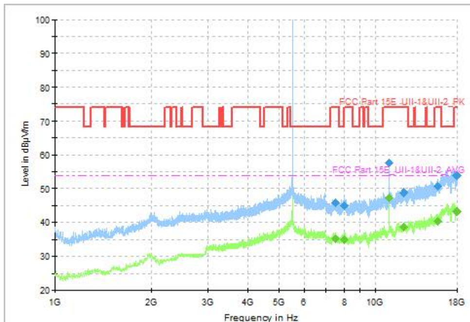
Fig. 49 Transmitter Spurious Emission (802.11n-HT20, CH52 5260MHz, 1GHz-18GHz), MIMO
