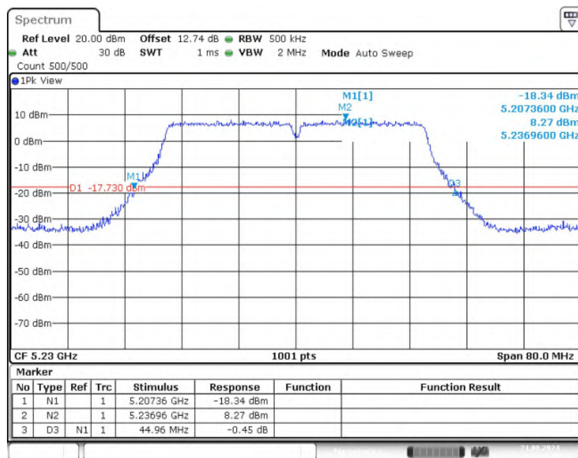
Fig. 4 Occupied 26dB Bandwidth (802.11ac-VHT40, 5230MHz)
