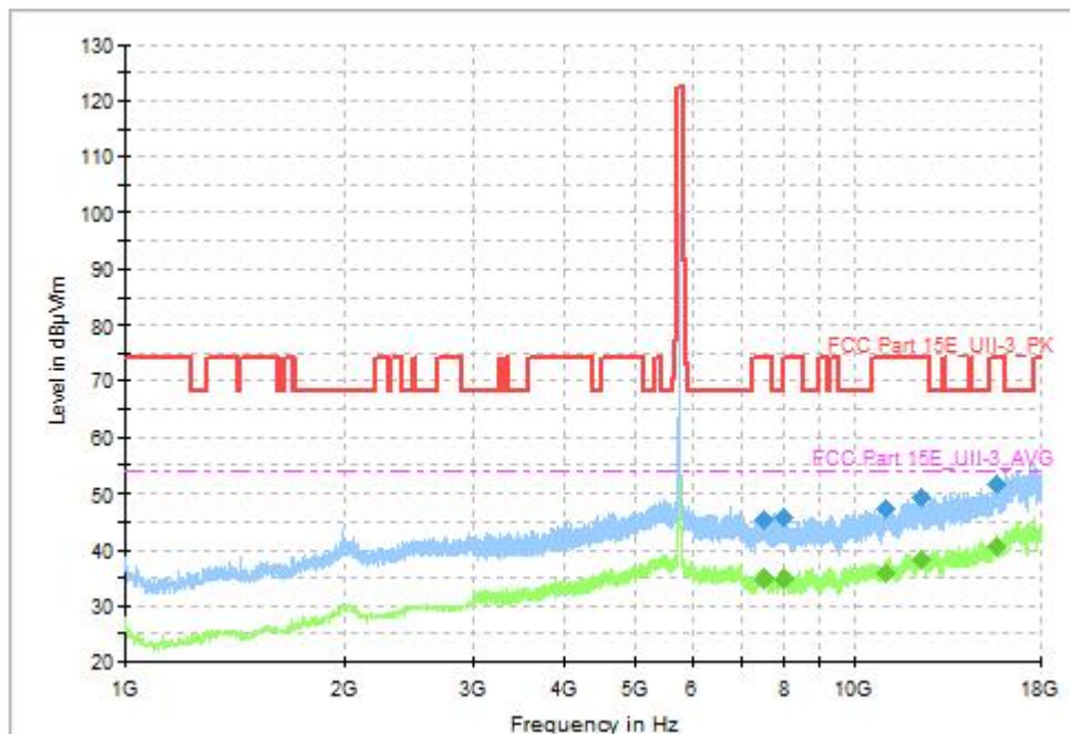
Fig. 65 Transmitter Spurious Emission (802.11ac-VHT40, CH151 5755MHz, 1GHz-18GHz), MIMO
