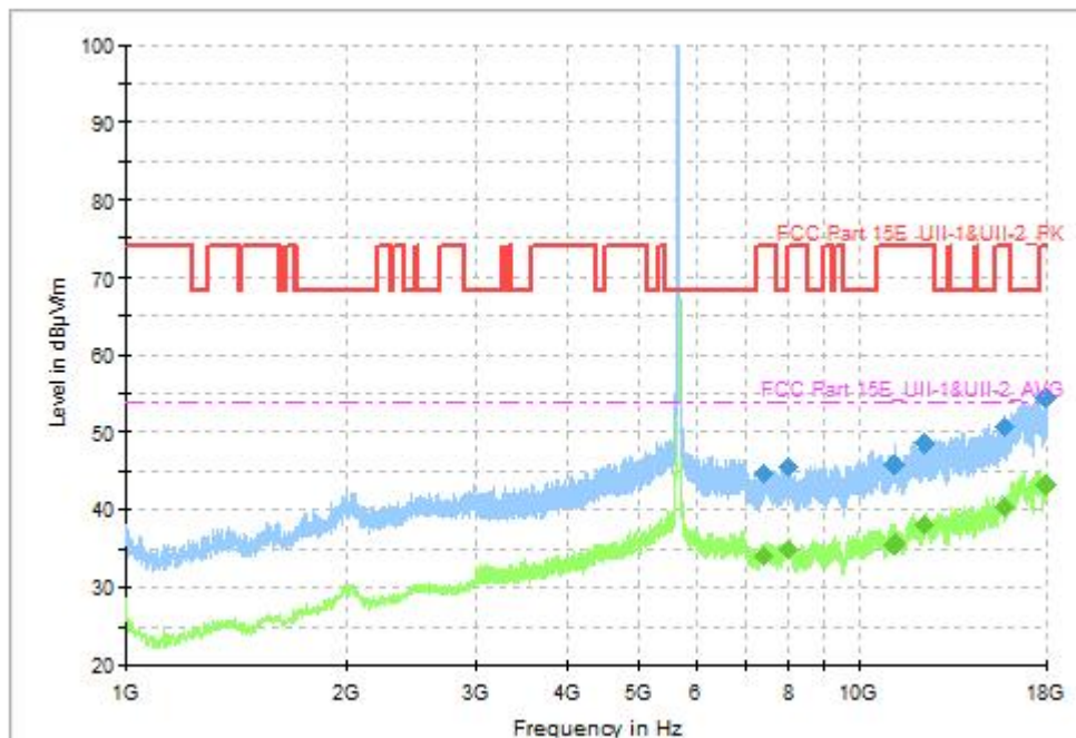
Fig. 64 Transmitter Spurious Emission (802.11ac-VHT40, CH134 5670MHz, 1GHz-18GHz), MIMO
