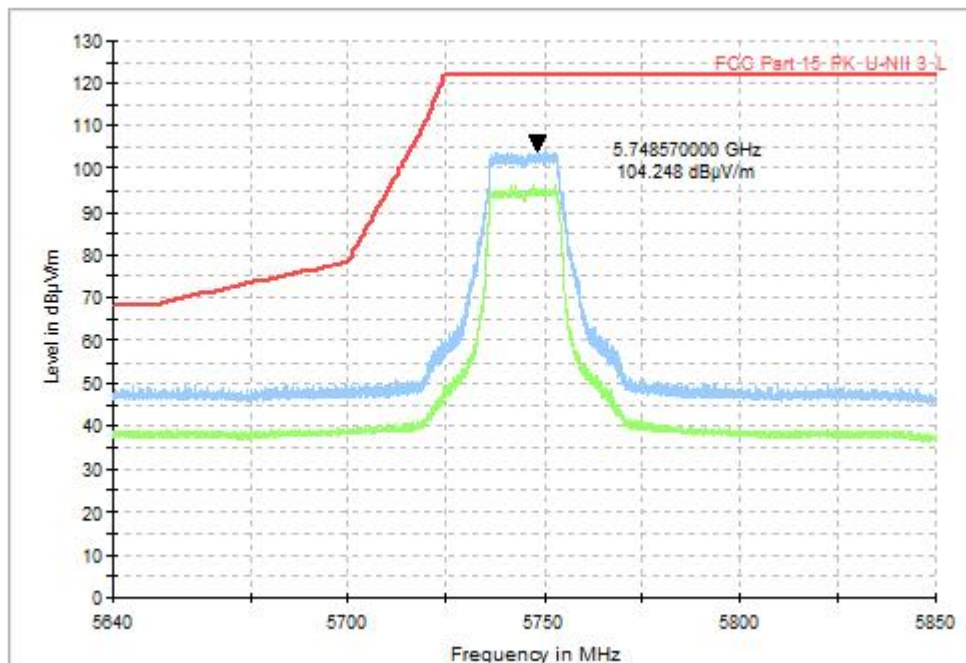
Fig. 31 Band Edges (802.11n-HT20, CH149 5745MHz), MIMO
