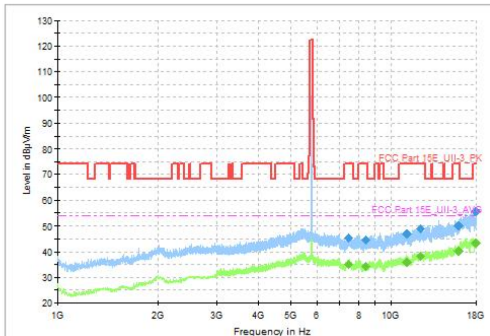
Fig. 56 Transmitter Spurious Emission (802.11n-HT20, CH157 5785MHz, 1GHz-18GHz), MIMO
