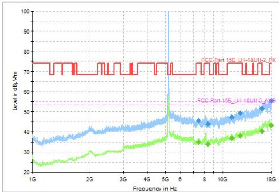
Fig. 46 Transmitter Spurious Emission (802.11n-HT20, CH36 5180MHz, 1GHz-18GHz), MIMO
