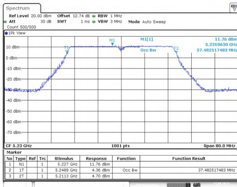
Fig. 18 99% Occupied Bandwidth (802.11ac-VHT40, 5230MHz)
