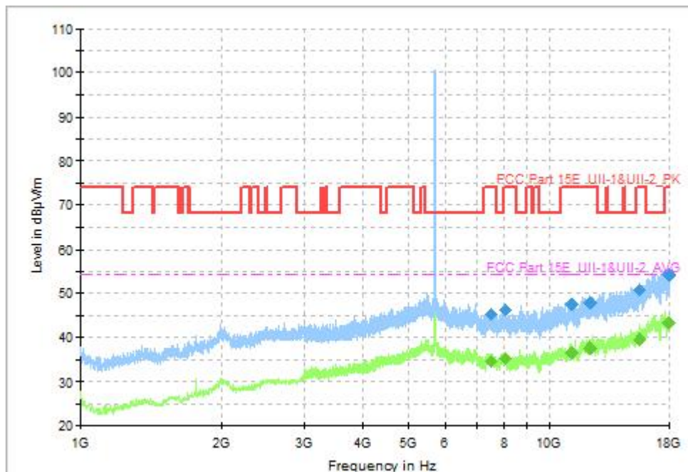
Fig. 54 Transmitter Spurious Emission (802.11n-HT20, CH140 5700MHz, 1GHz-18GHz), MIMO
