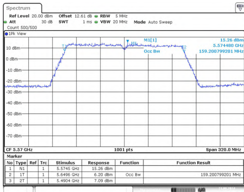
Fig. 22 99% Occupied Bandwidth (802.11ac-VHT160, 5570MHz)
