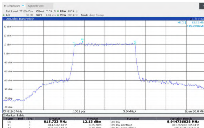
LTE Band 26 , 10MHz Bandwidth,MID,64QAM (99% BW)
