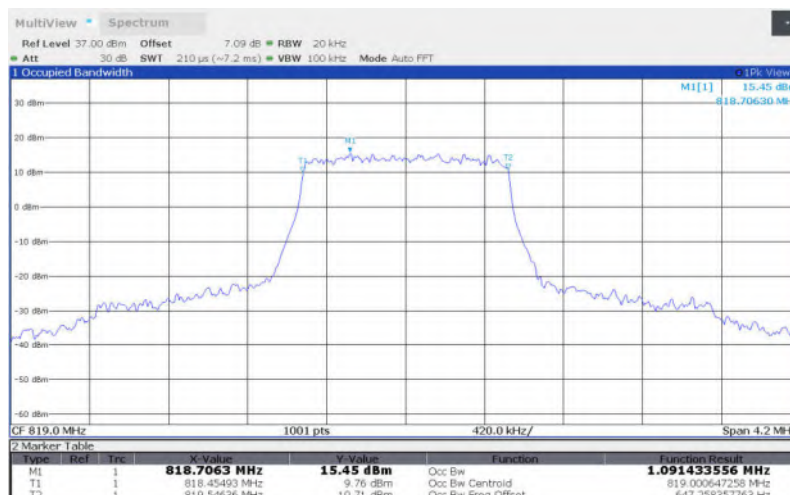
LTE Band 26 , 1.4MHz Bandwidth,MID,QPSK (99% BW)
