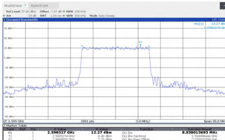
LTE Band 38 , 10MHz Bandwidth,MID,64QAM (99% BW)
