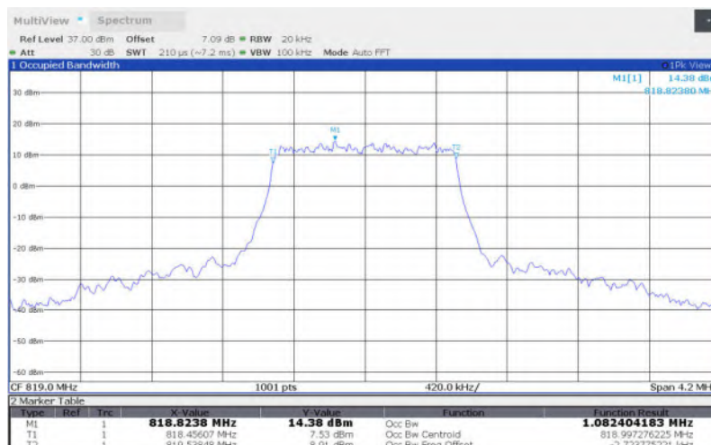
LTE Band 26 , 1.4MHz Bandwidth,MID,64QAM (99% BW)
