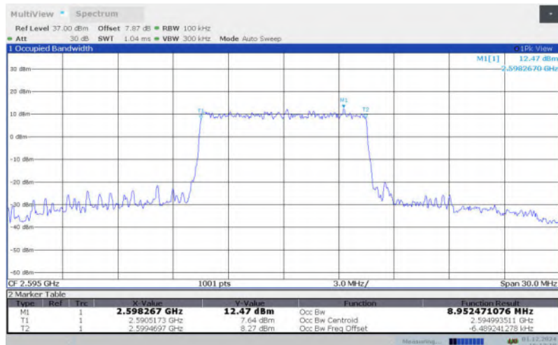
LTE Band 41 , 10MHz Bandwidth,MID,64QAM (99% BW)
