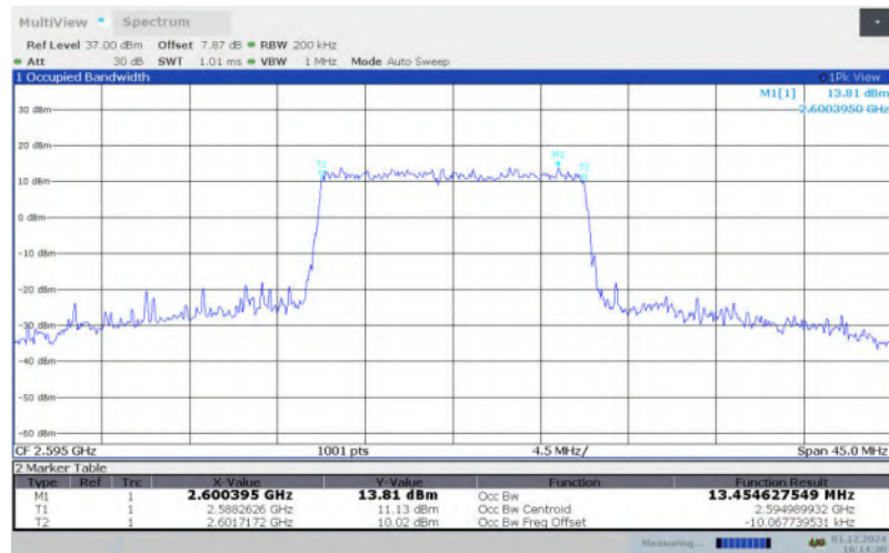
LTE Band 41 , 15MHz Bandwidth,MID,64QAM (99% BW)
