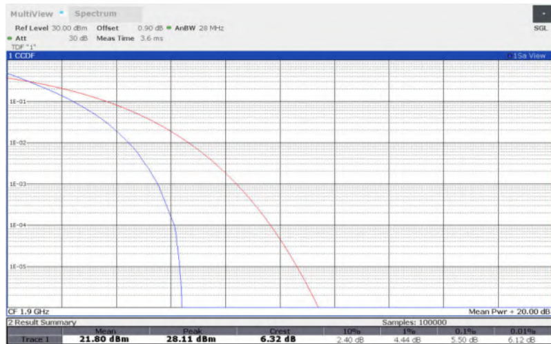
LTE Band 2 , 20MHz Bandwidth,16QAM
