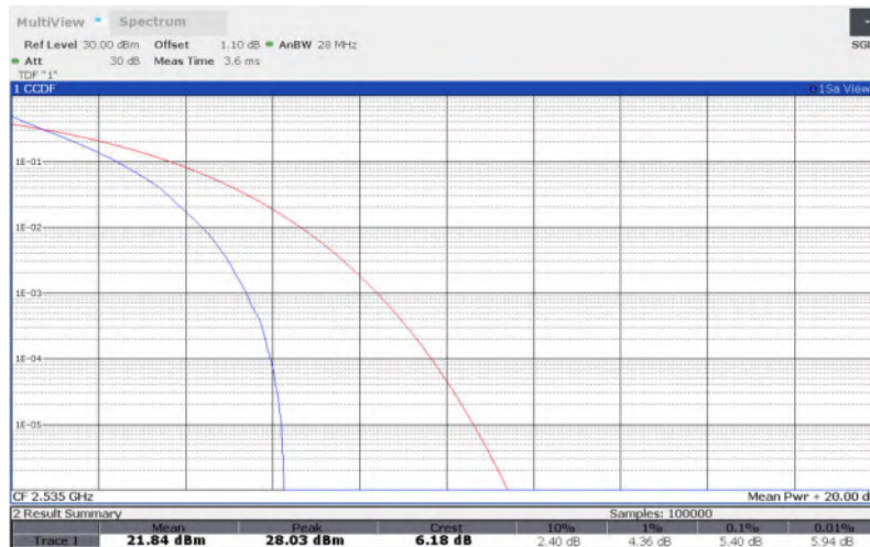
LTE Band 7 , 10MHz Bandwidth,16QAM
