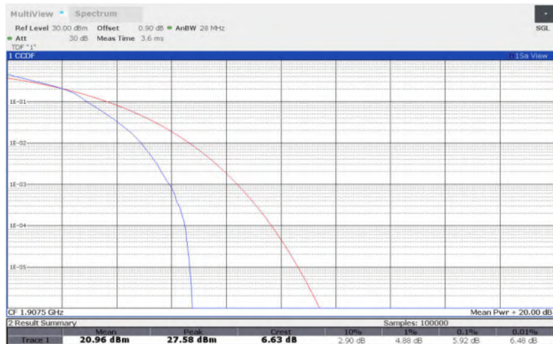
LTE Band 2 , 5MHz Bandwidth,64QAM
