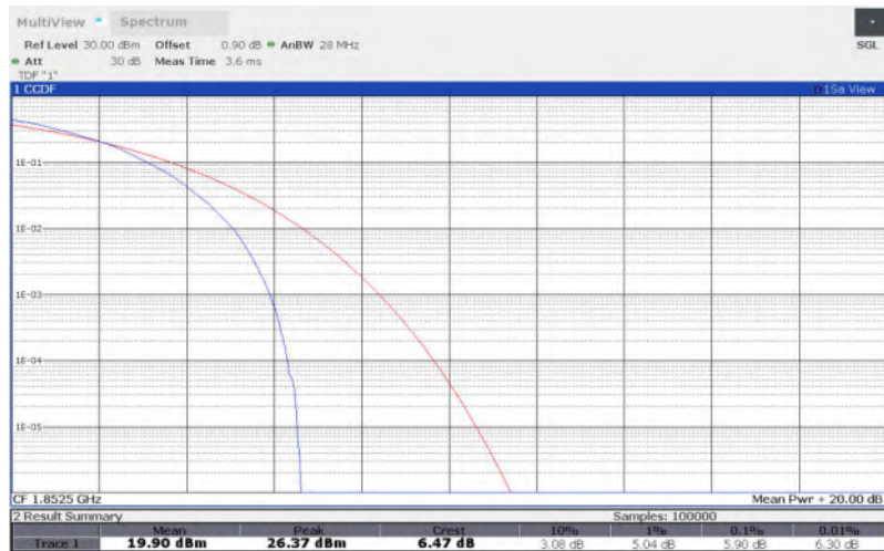
LTE Band 2 , 5MHz Bandwidth,QPSK
