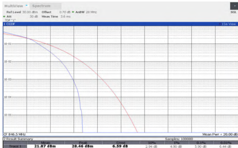
LTE Band 5 , 5MHz Bandwidth,64QAM
