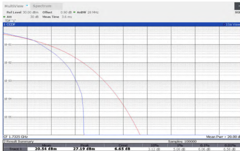
LTE Band 4 , 3MHz Bandwidth,64QAM
