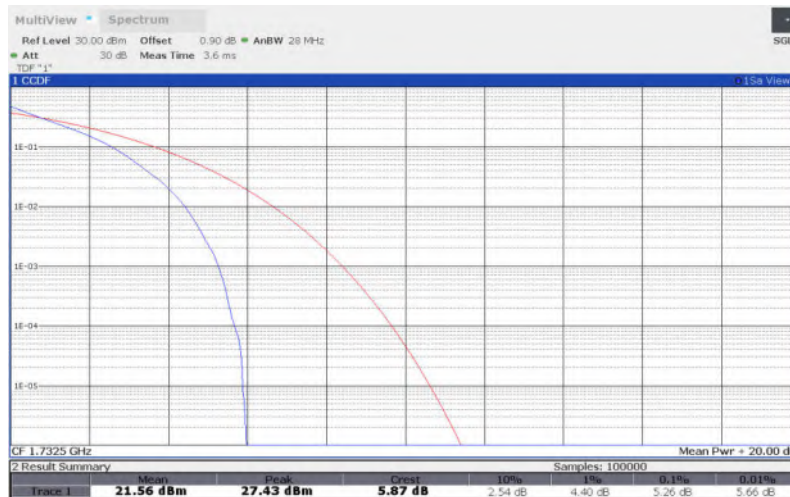
LTE Band 4 , 5MHz Bandwidth,16QAM
