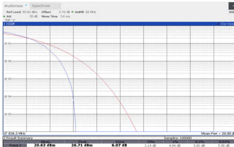
LTE Band 5 , 3MHz Bandwidth,QPSK
