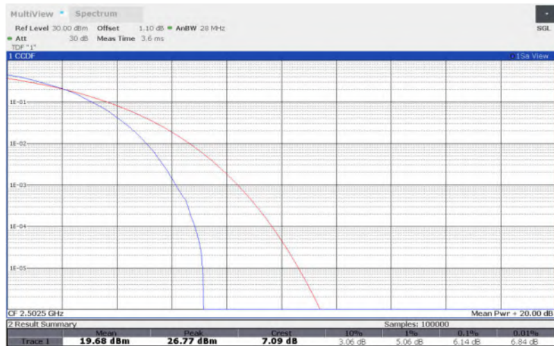
LTE Band 7 , 5MHz Bandwidth,QPSK
