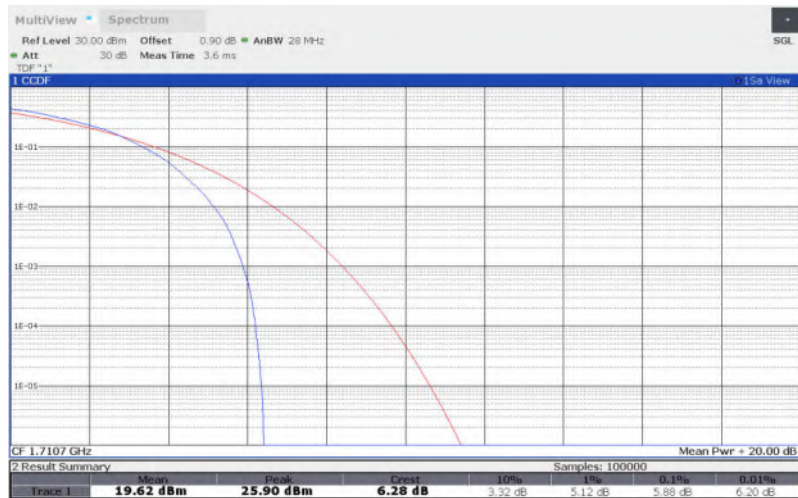
LTE Band 4 , 1.4MHz Bandwidth,QPSK
