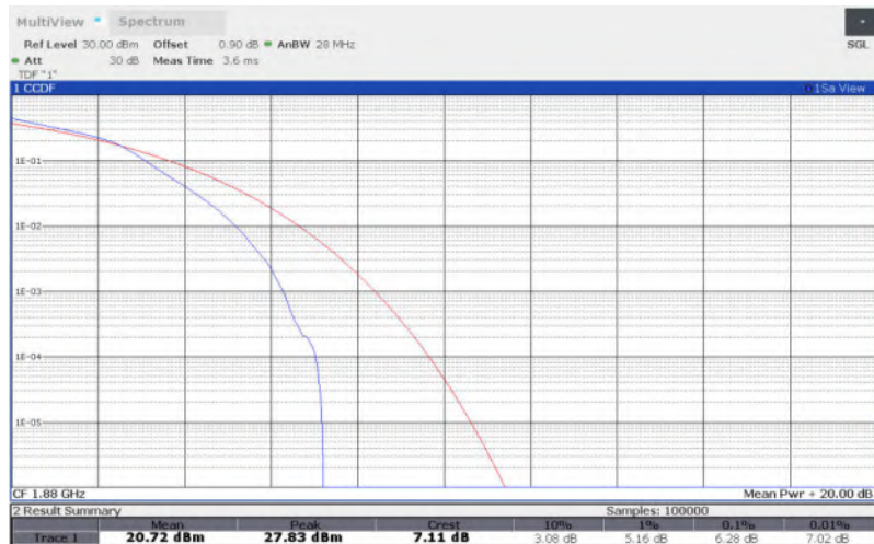
LTE Band 2 , 1.4MHz Bandwidth,64QAM
