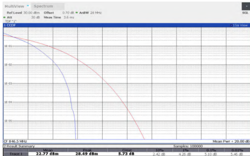
LTE Band 5 , 5MHz Bandwidth,16QAM
