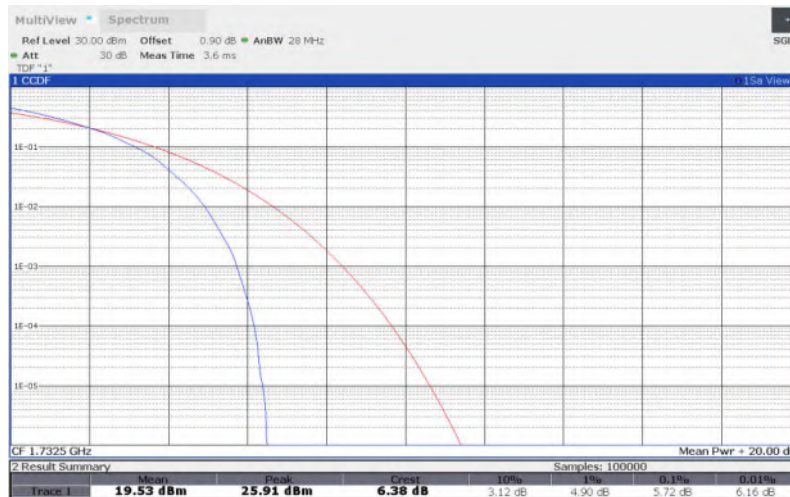
LTE Band 4 , 10MHz Bandwidth,QPSK
