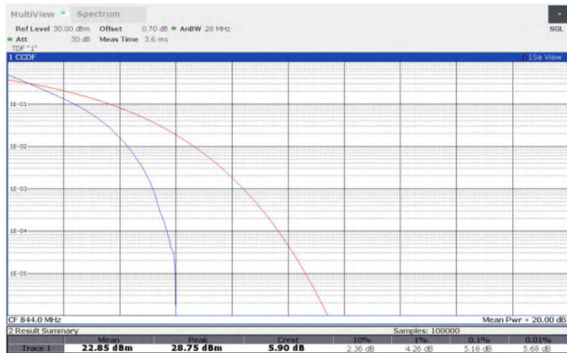
LTE Band 5 , 10MHz Bandwidth,16QAM
