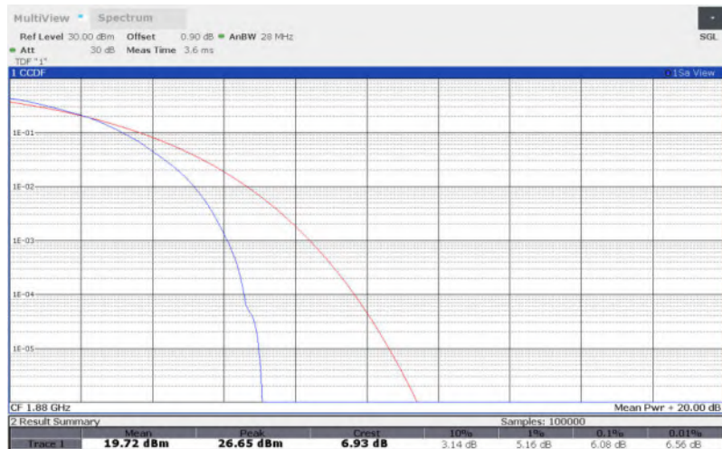
LTE Band 2 , 3MHz Bandwidth,QPSK
