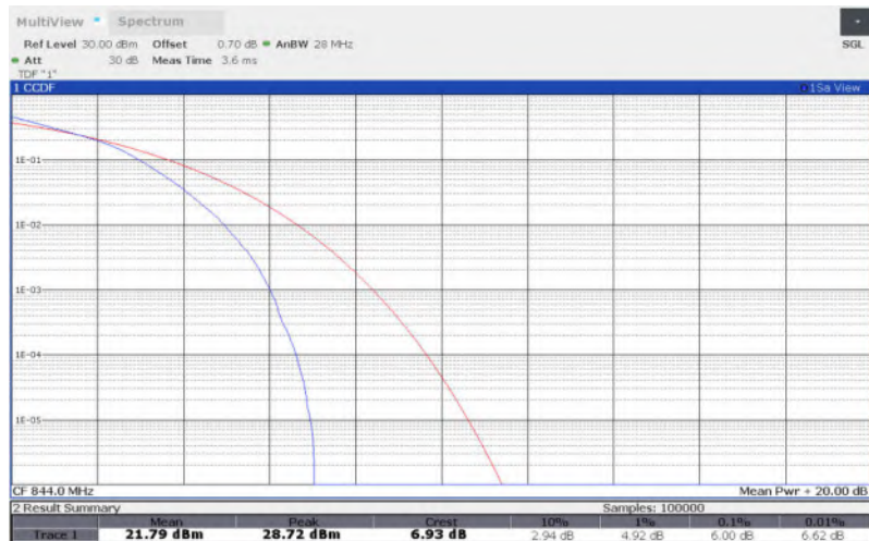
LTE Band 5 , 10MHz Bandwidth,64QAM
