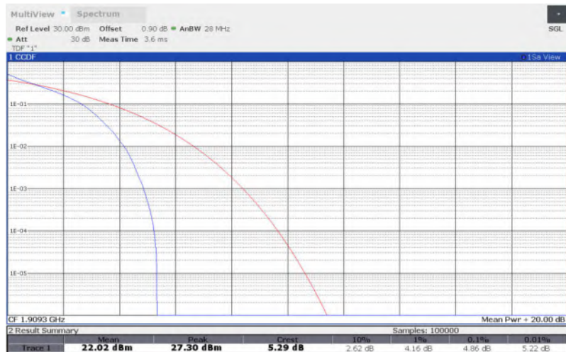
LTE Band 2 , 1.4MHz Bandwidth,16QAM
