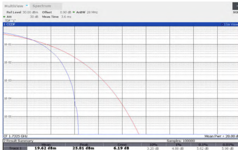
LTE Band 4 , 3MHz Bandwidth,QPSK
