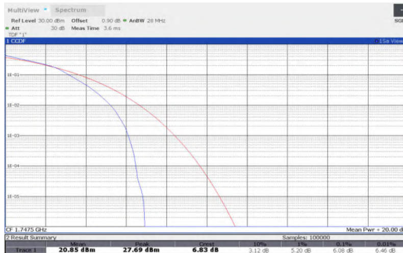
LTE Band 4 , 15MHz Bandwidth,64QAM
