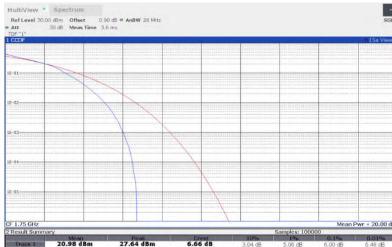
LTE Band 4 , 10MHz Bandwidth,64QAM
