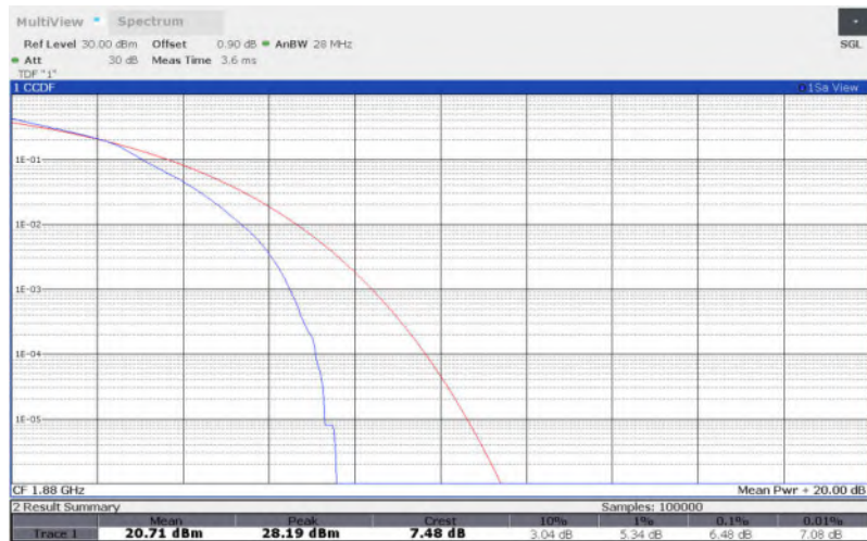
LTE Band 2 , 15MHz Bandwidth,64QAM
