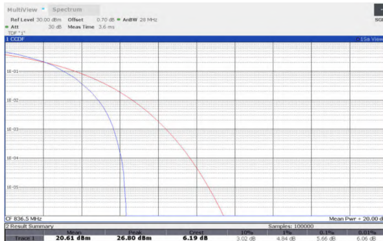
LTE Band 5 , 5MHz Bandwidth,QPSK
