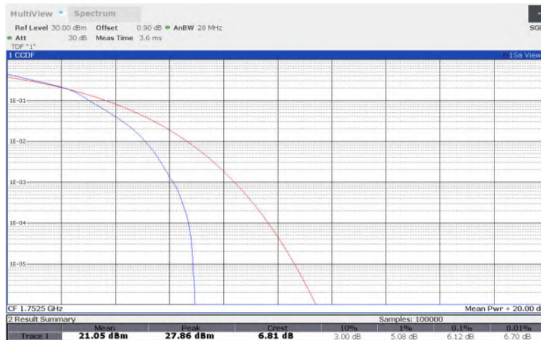
LTE Band 4 , 5MHz Bandwidth,64QAM
