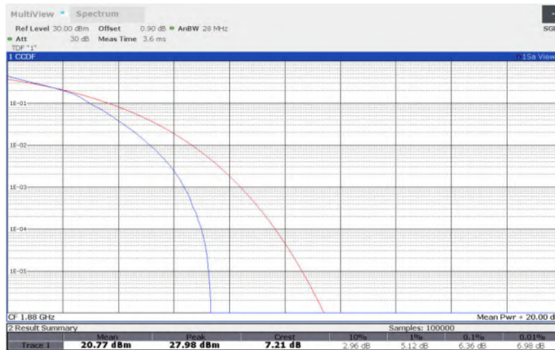
LTE Band 2 , 10MHz Bandwidth,64QAM
