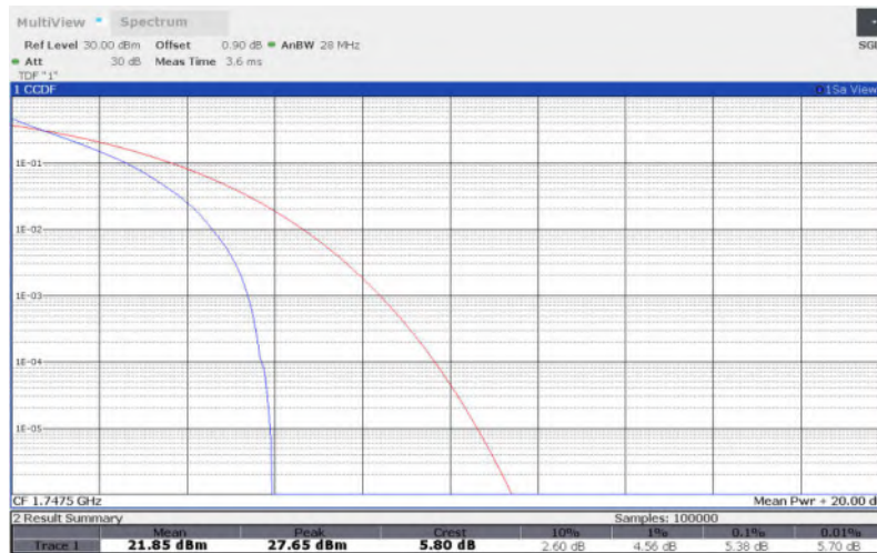
LTE Band 4 , 15MHz Bandwidth,16QAM
