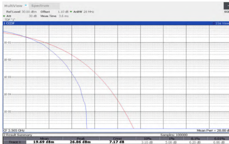
LTE Band 7 , 10MHz Bandwidth,QPSK
