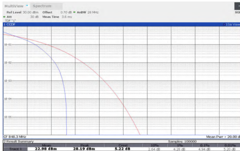
LTE Band 5 , 1.4MHz Bandwidth,16QAM
