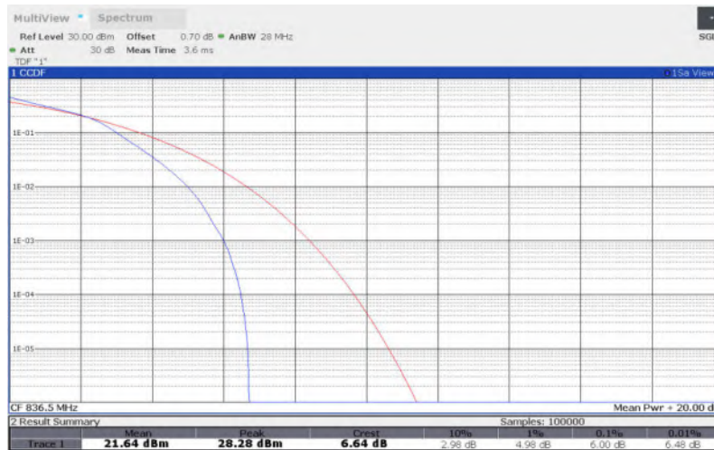
LTE Band 5 , 3MHz Bandwidth,64QAM
