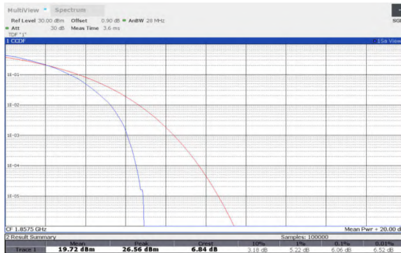
LTE Band 2 , 15MHz Bandwidth,QPSK
