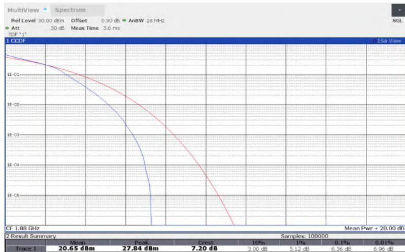
LTE Band 2 , 3MHz Bandwidth,64QAM
