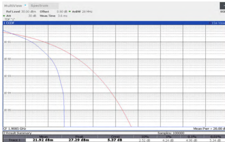
LTE Band 2 , 3MHz Bandwidth,16QAM
