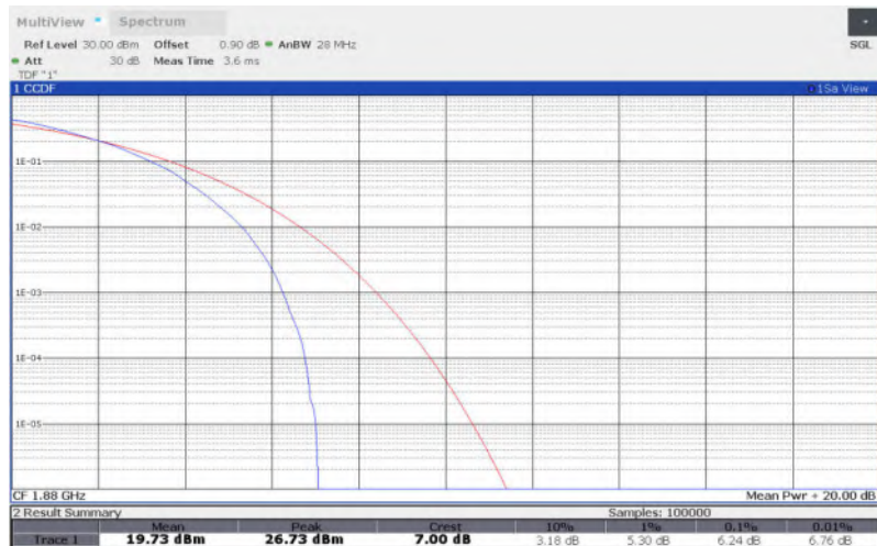
LTE Band 2 , 15MHz Bandwidth,QPSK
