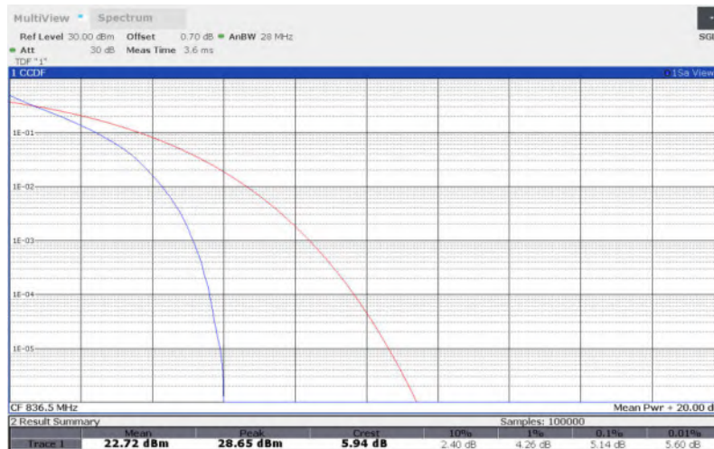
LTE Band 5 , 10MHz Bandwidth,16QAM
