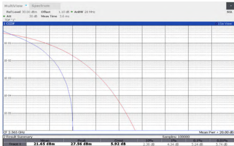
LTE Band 7 , 10MHz Bandwidth,16QAM
