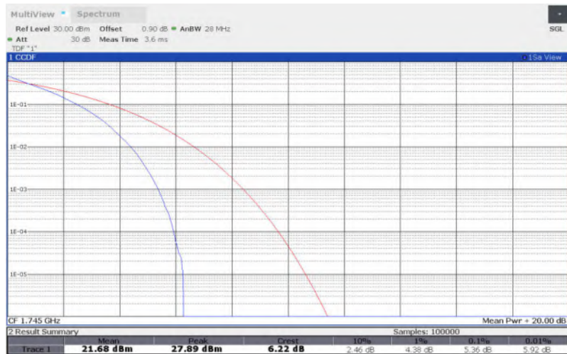
LTE Band 4 , 20MHz Bandwidth,16QAM
