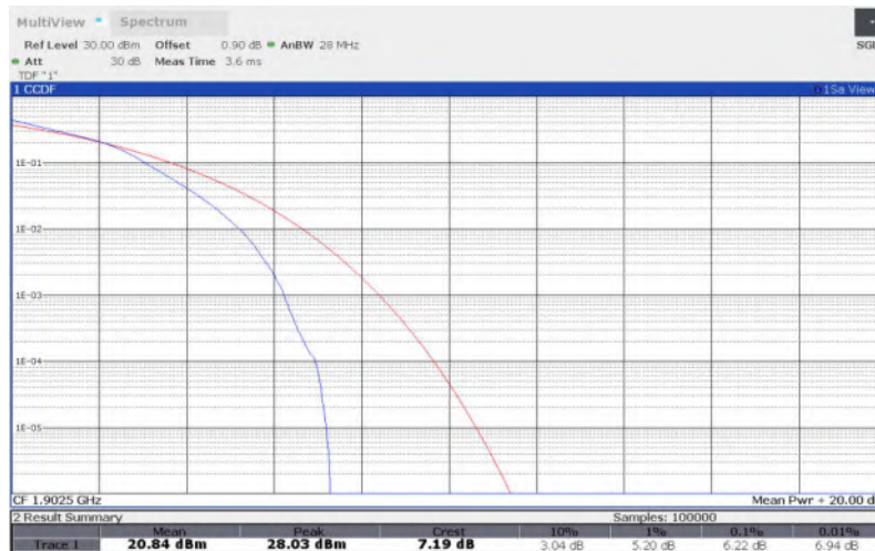
LTE Band 2 , 15MHz Bandwidth,64QAM
