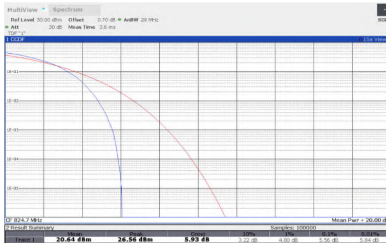
LTE Band 5 , 1.4MHz Bandwidth,QPSK
