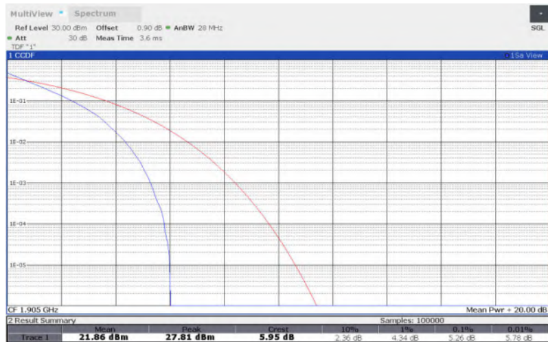
LTE Band 2 , 10MHz Bandwidth,16QAM
