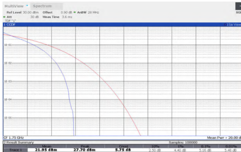
LTE Band 4 , 10MHz Bandwidth,16QAM
