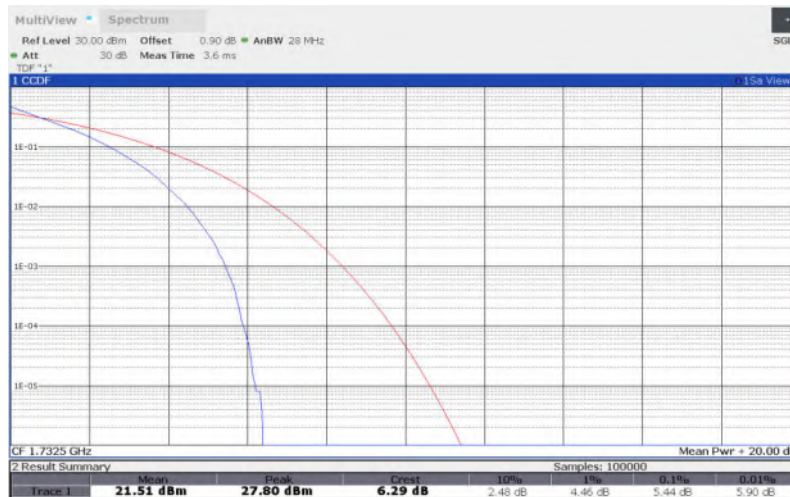
LTE Band 4 , 20MHz Bandwidth,16QAM
