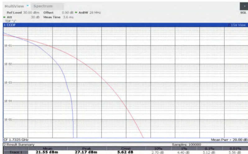
LTE Band 4 , 1.4MHz Bandwidth,16QAM
