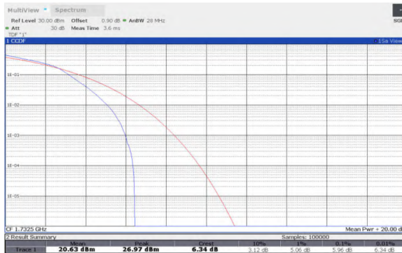
LTE Band 4 , 1.4MHz Bandwidth,64QAM
