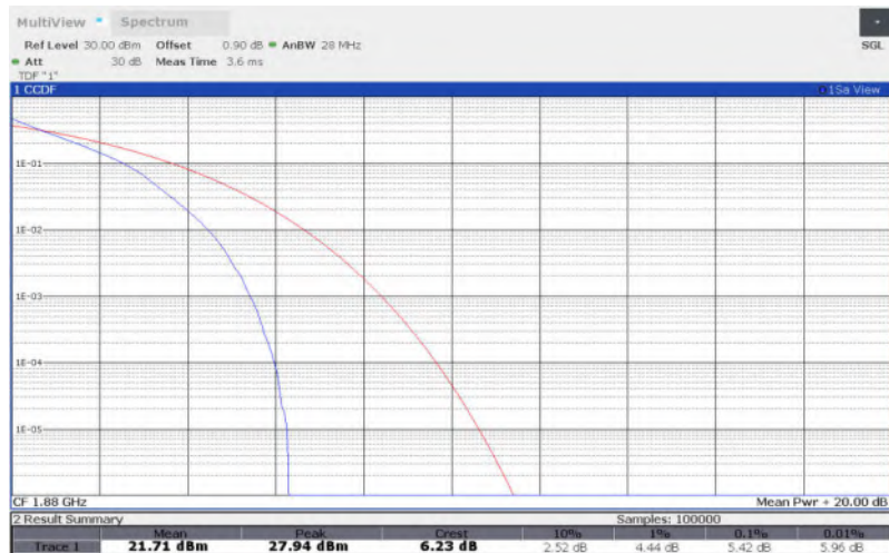
LTE Band 2 , 3MHz Bandwidth,16QAM
