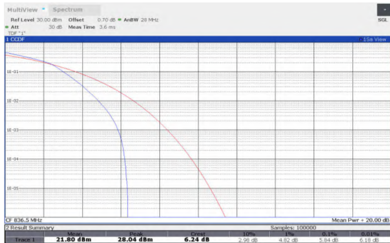
LTE Band 5 , 1.4MHz Bandwidth,64QAM
