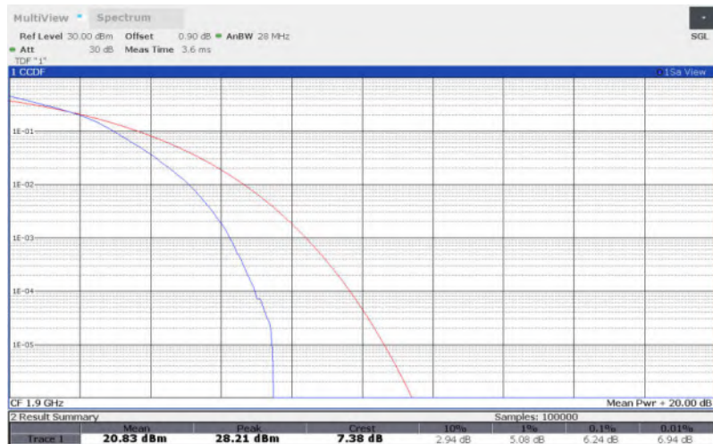
LTE Band 2 , 20MHz Bandwidth,64QAM
