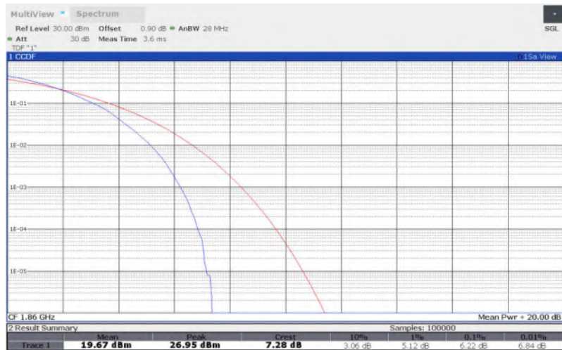
LTE Band 2 , 20MHz Bandwidth,QPSK
