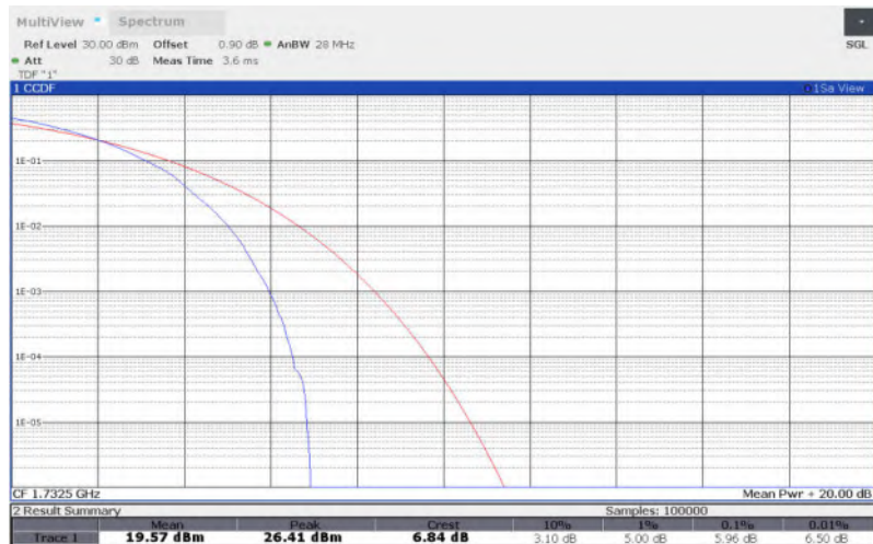
LTE Band 4 , 20MHz Bandwidth,QPSK
