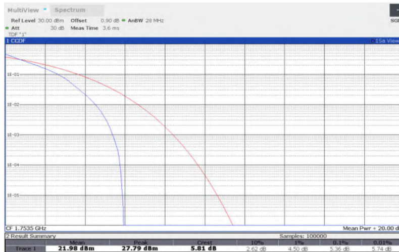
LTE Band 4 , 3MHz Bandwidth,16QAM
