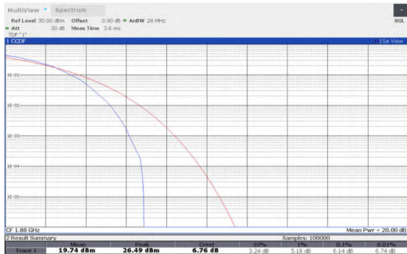
LTE Band 2 , 1.4MHz Bandwidth,QPSK
