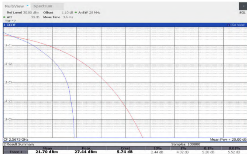
LTE Band 7 , 5MHz Bandwidth,16QAM
