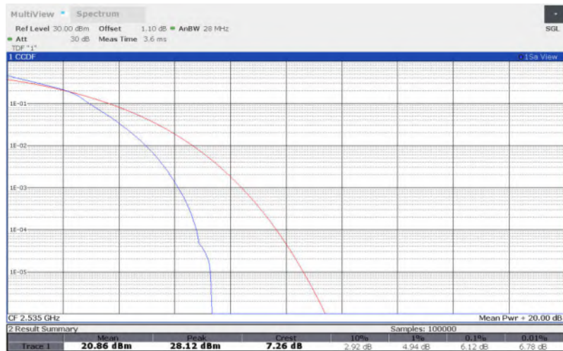
LTE Band 7 , 5MHz Bandwidth,64QAM
