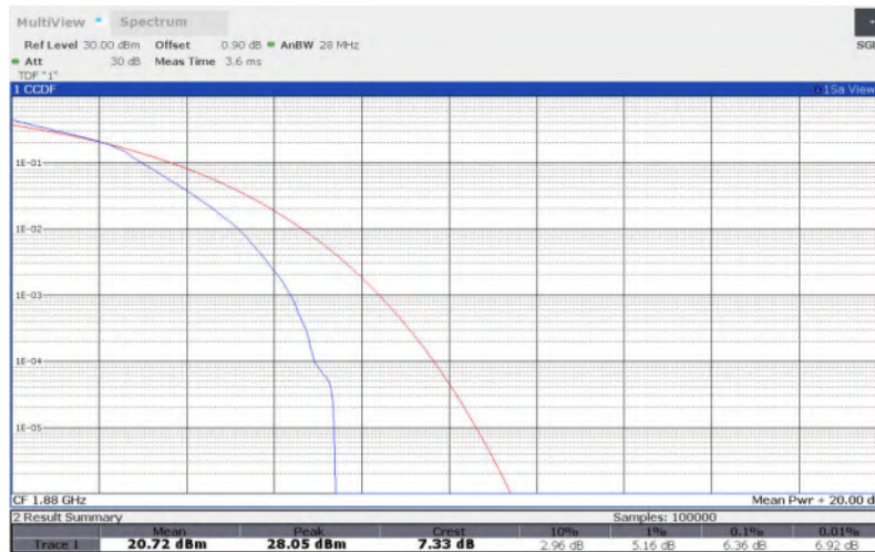
LTE Band 2 , 5MHz Bandwidth,64QAM
