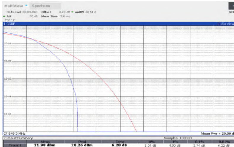
LTE Band 5 , 1.4MHz Bandwidth,64QAM
