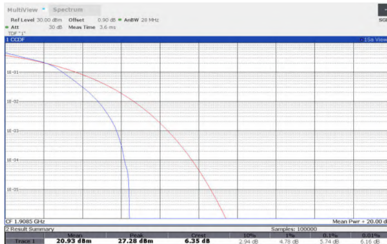
LTE Band 2 , 3MHz Bandwidth,64QAM
