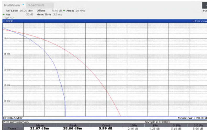
LTE Band 5 , 5MHz Bandwidth,16QAM
