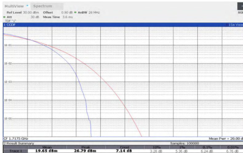
LTE Band 4 , 15MHz Bandwidth,QPSK
