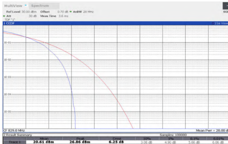
LTE Band 5 , 10MHz Bandwidth,QPSK
