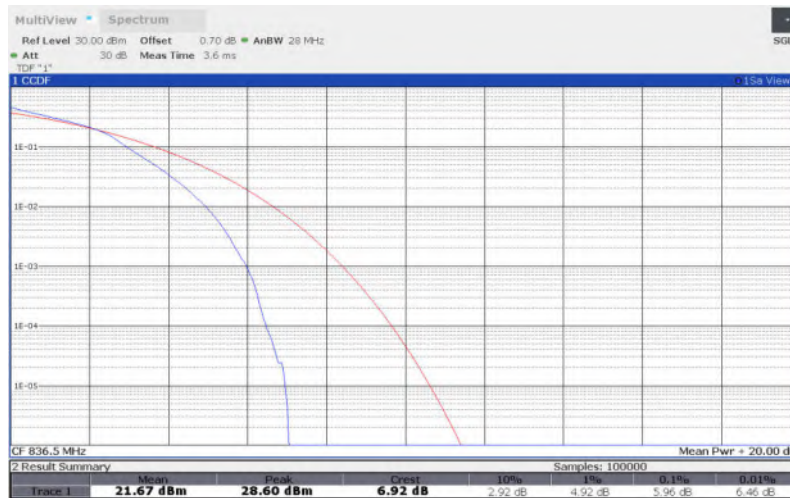
LTE Band 5 , 5MHz Bandwidth,64QAM
