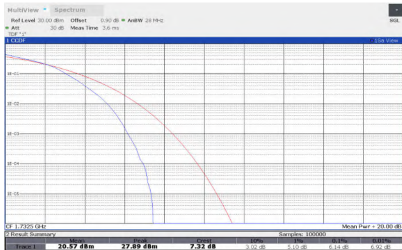
LTE Band 4 , 20MHz Bandwidth,64QAM
