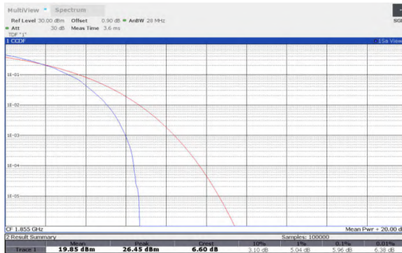
LTE Band 2 , 10MHz Bandwidth,QPSK
