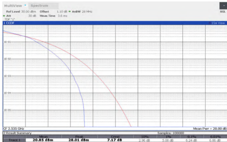
LTE Band 7 , 10MHz Bandwidth,64QAM
