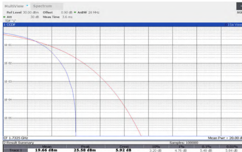
LTE Band 4 , 1.4MHz Bandwidth,QPSK
