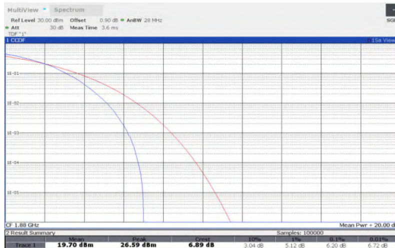
LTE Band 2 , 5MHz Bandwidth,QPSK
