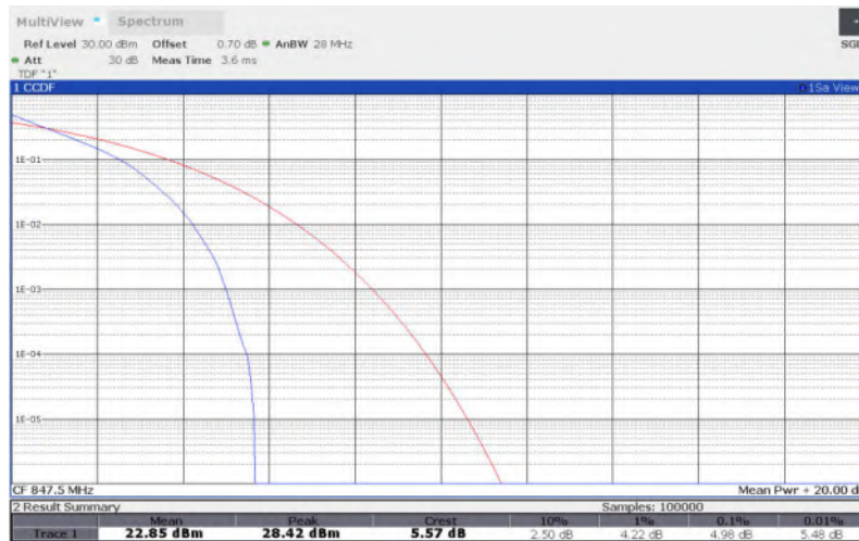
LTE Band 5 , 3MHz Bandwidth,16QAM
