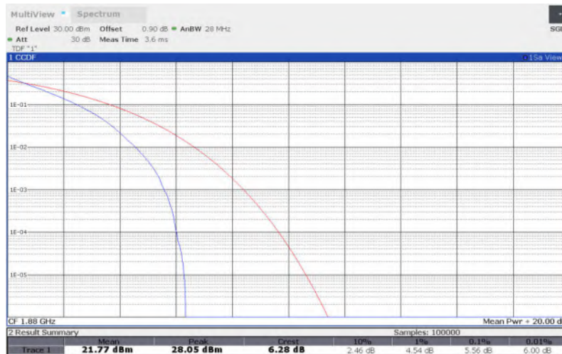
LTE Band 2 , 10MHz Bandwidth,16QAM
