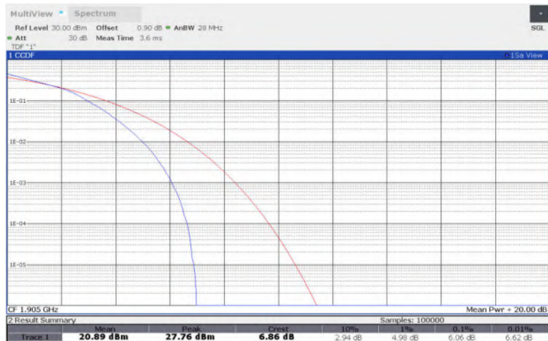
LTE Band 2 , 10MHz Bandwidth,64QAM
