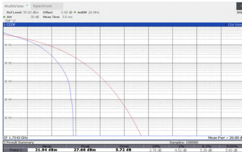
LTE Band 4 , 1.4MHz Bandwidth,16QAM
