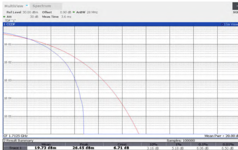
LTE Band 4 , 5MHz Bandwidth,QPSK
