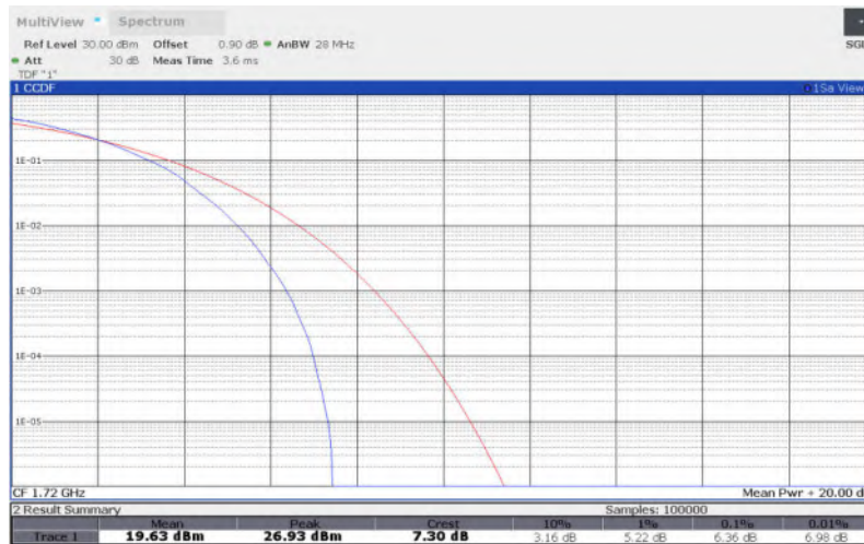
LTE Band 4 , 20MHz Bandwidth,QPSK
