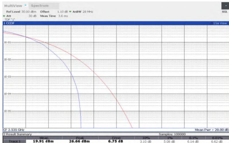
LTE Band 7 , 10MHz Bandwidth,QPSK
