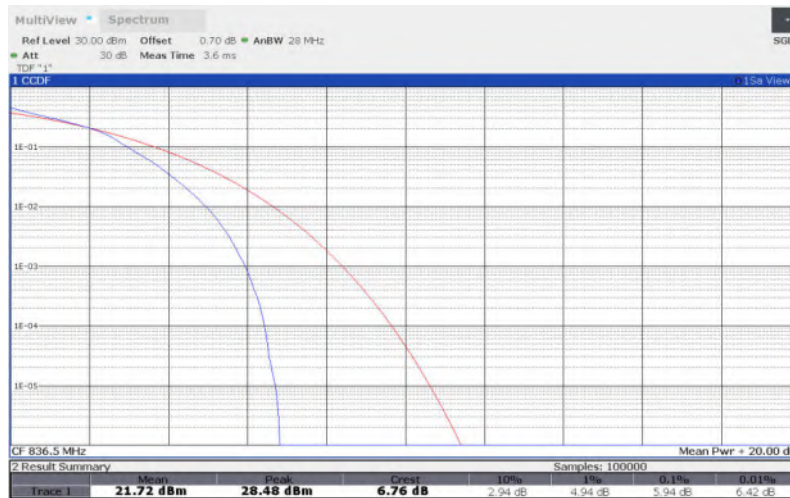
LTE Band 5 , 10MHz Bandwidth,64QAM
