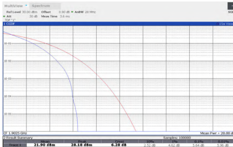
LTE Band 2 , 15MHz Bandwidth,16QAM
