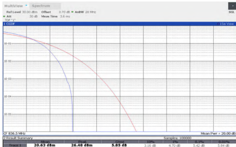
LTE Band 5 , 1.4MHz Bandwidth,QPSK
