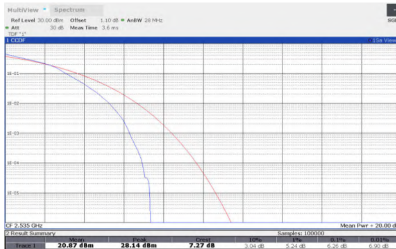
LTE Band 7 , 15MHz Bandwidth,64QAM
