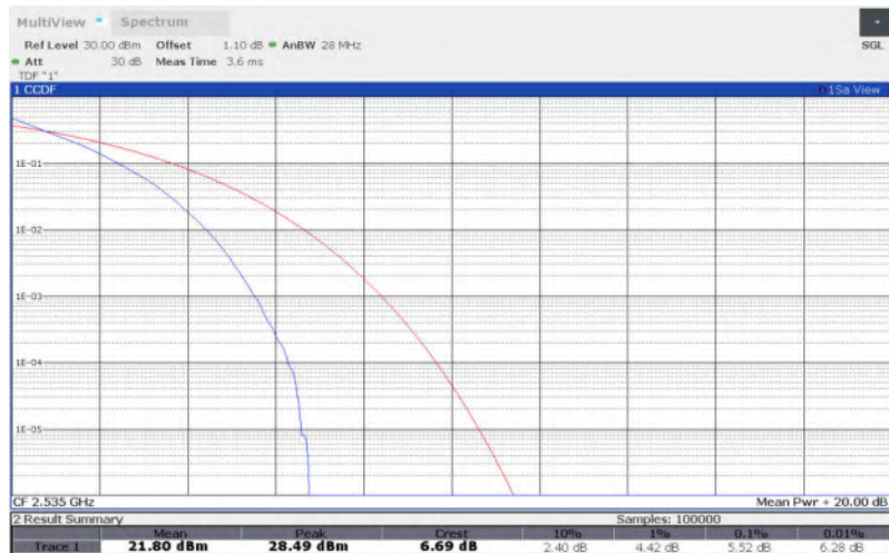
LTE Band 7 , 20MHz Bandwidth,16QAM
