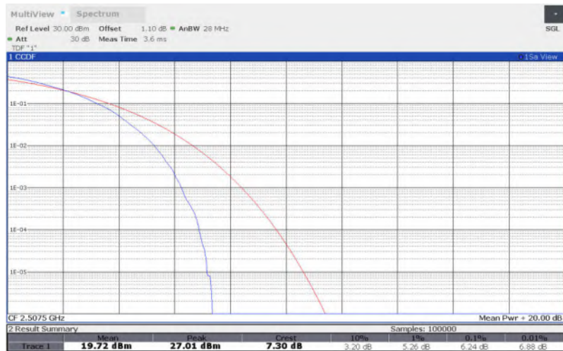
LTE Band 7 , 15MHz Bandwidth,QPSK
