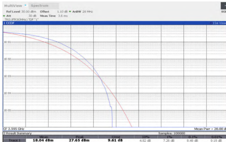
LTE Band 38 , 5MHz Bandwidth,QPSK
