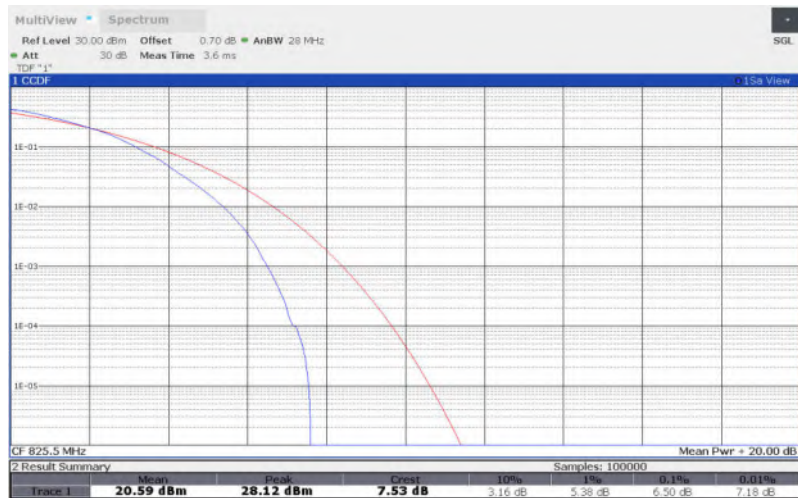
LTE Band 26 , 3MHz Bandwidth,QPSK
