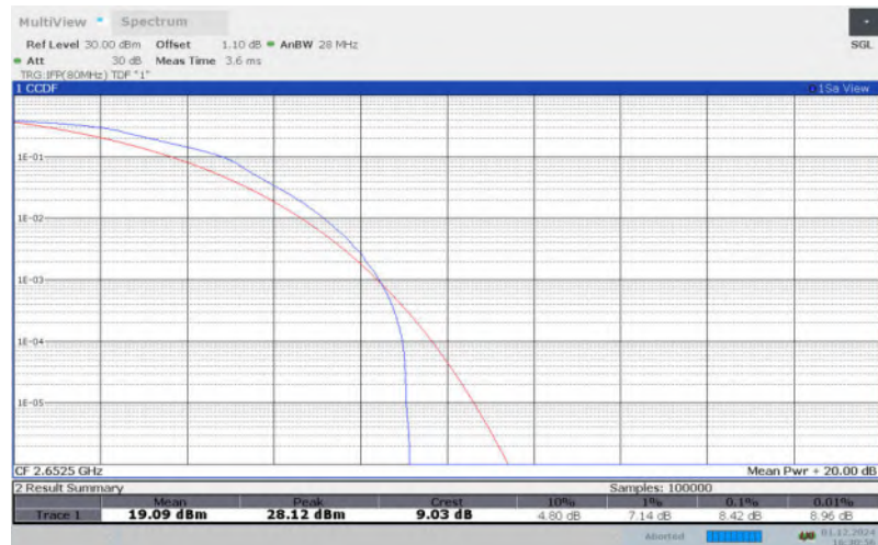
LTE Band 41 , 5MHz Bandwidth,64QAM
