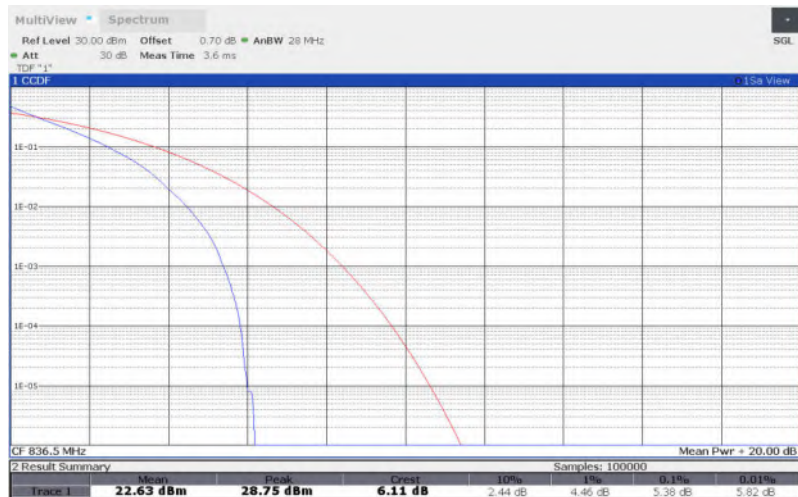
LTE Band 26 , 10MHz Bandwidth,16QAM
