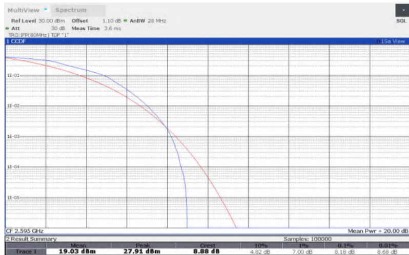
LTE Band 38 , 10MHz Bandwidth,64QAM
