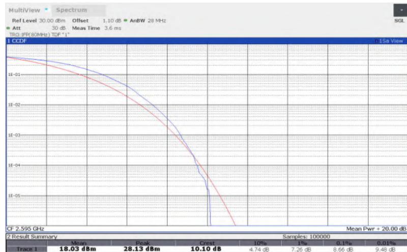
LTE Band 38 , 20MHz Bandwidth,QPSK
