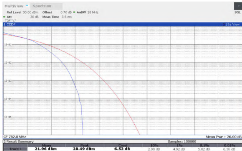
LTE Band 13 , 10MHz Bandwidth,64QAM
