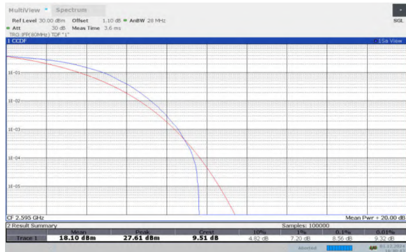
LTE Band 41 , 5MHz Bandwidth,QPSK
