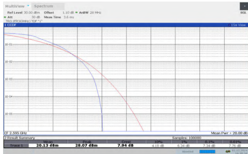
LTE Band 41 , 5MHz Bandwidth,16QAM
