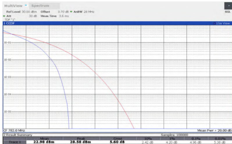
LTE Band 13 , 10MHz Bandwidth,16QAM
