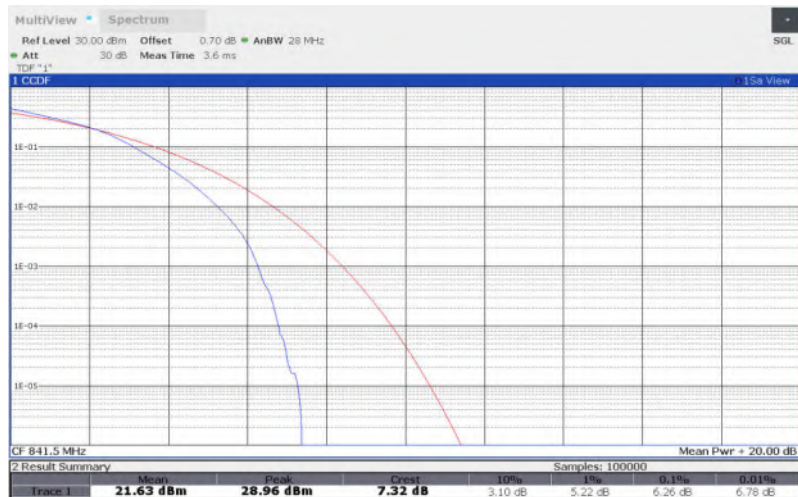
LTE Band 26 , 15MHz Bandwidth,64QAM
