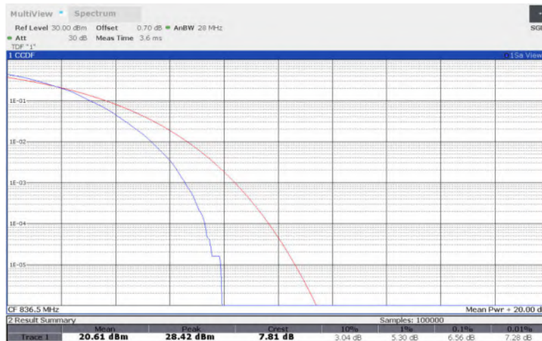
LTE Band 26 , 5MHz Bandwidth,QPSK
