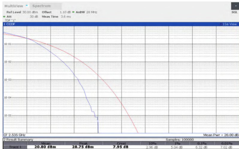
LTE Band 7 , 20MHz Bandwidth,64QAM
