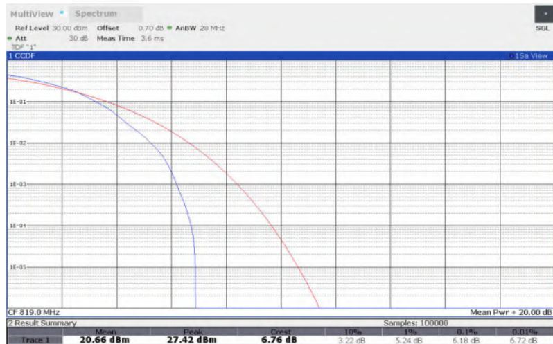
LTE Band 26 , 1.4MHz Bandwidth,QPSK
