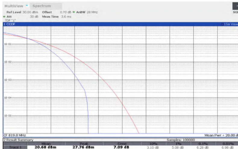
LTE Band 26 , 3MHz Bandwidth,QPSK
