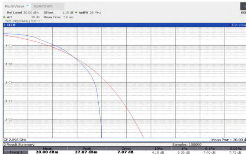
LTE Band 38 , 5MHz Bandwidth,16QAM
