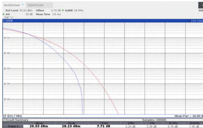
LTE Band 26 , 1.4MHz Bandwidth,QPSK
