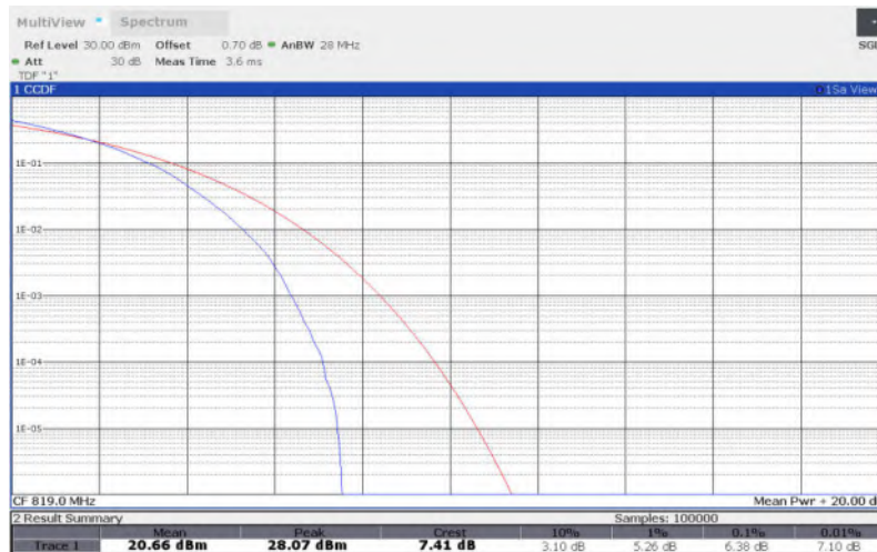
LTE Band 26 , 10MHz Bandwidth,QPSK
