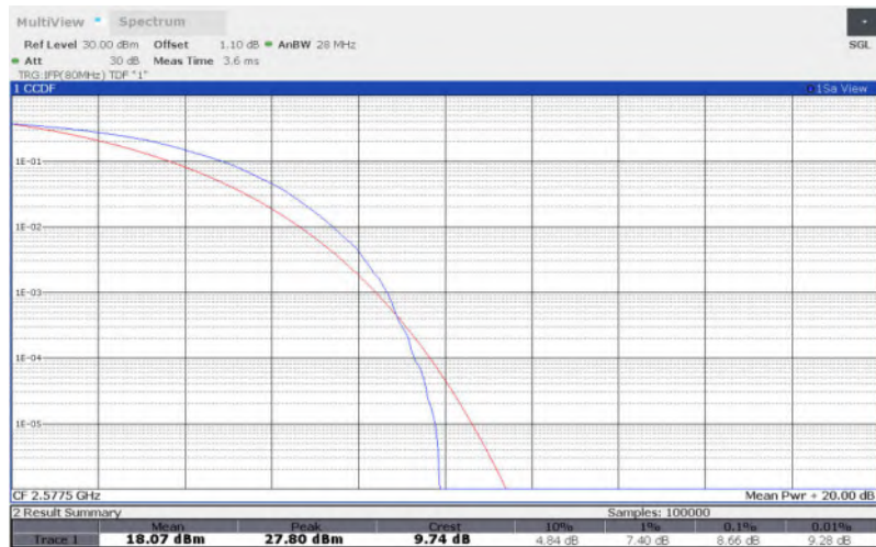
LTE Band 38 , 15MHz Bandwidth,QPSK
