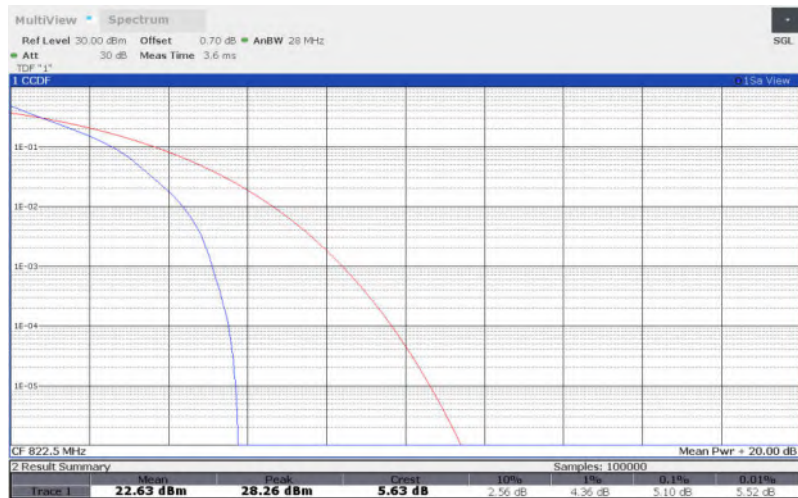
LTE Band 26 , 3MHz Bandwidth,16QAM
