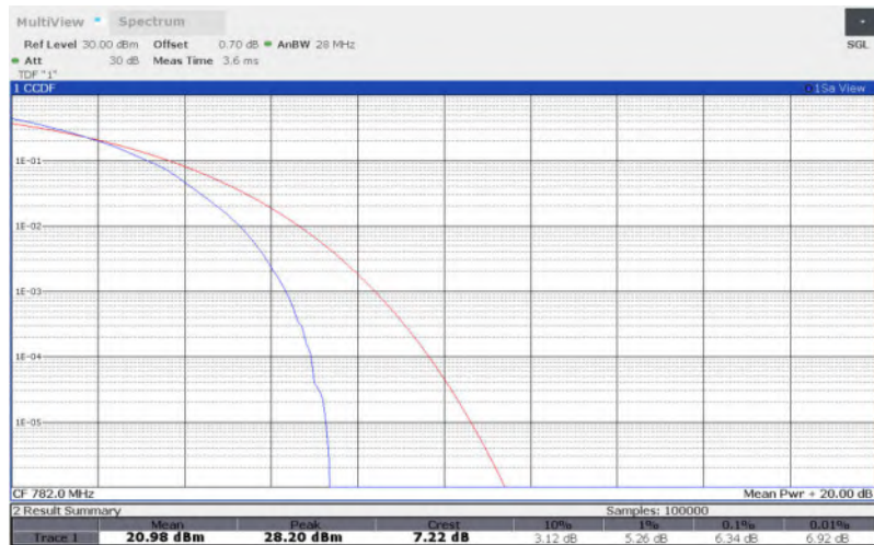
LTE Band 13 , 10MHz Bandwidth,QPSK
