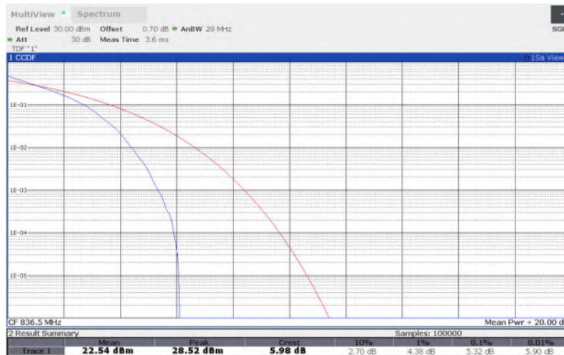
LTE Band 26 , 1.4MHz Bandwidth,16QAM
