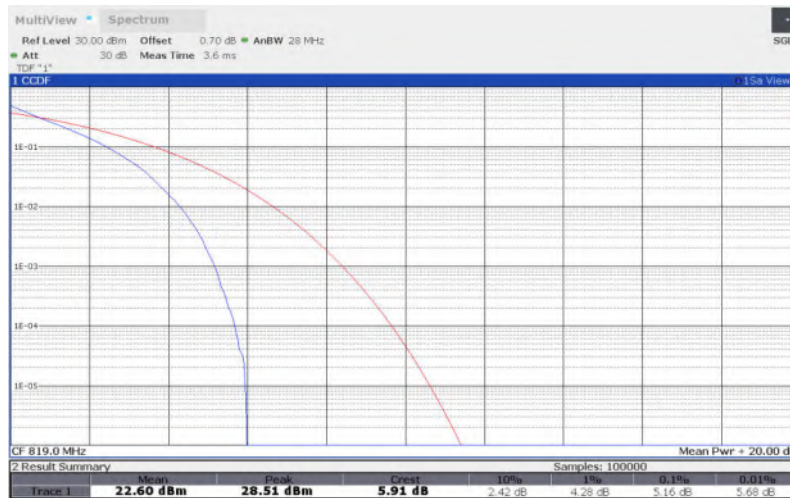
LTE Band 26 , 10MHz Bandwidth,16QAM
