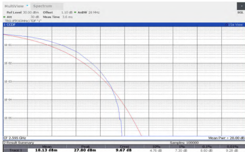
LTE Band 38 , 10MHz Bandwidth,QPSK
