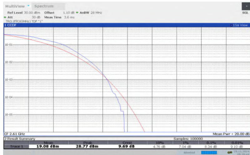
LTE Band 38 , 20MHz Bandwidth,64QAM
