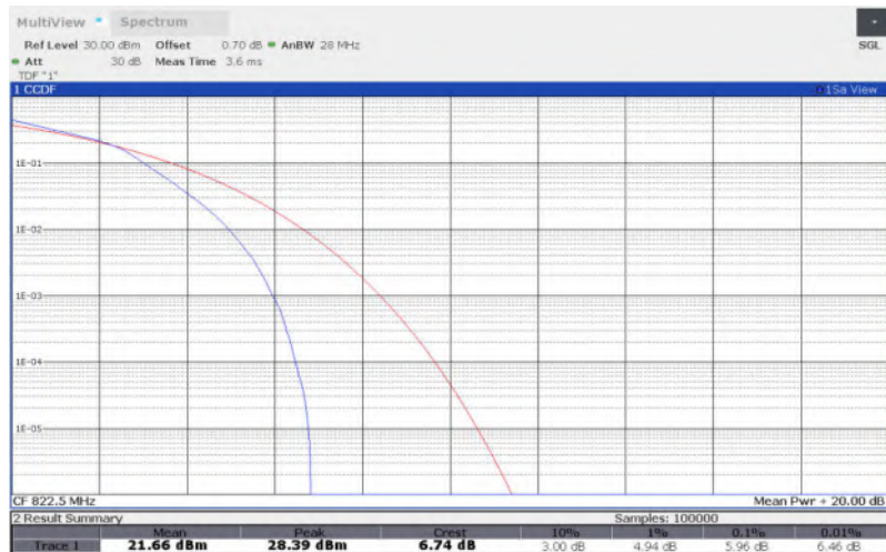
LTE Band 26 , 3MHz Bandwidth,64QAM
