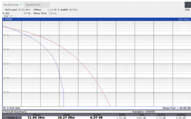
LTE Band 7 , 15MHz Bandwidth,16QAM
