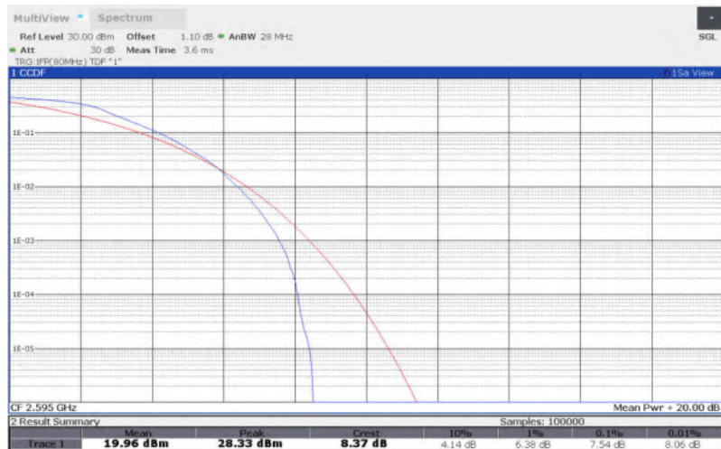
LTE Band 38 , 20MHz Bandwidth,16QAM
