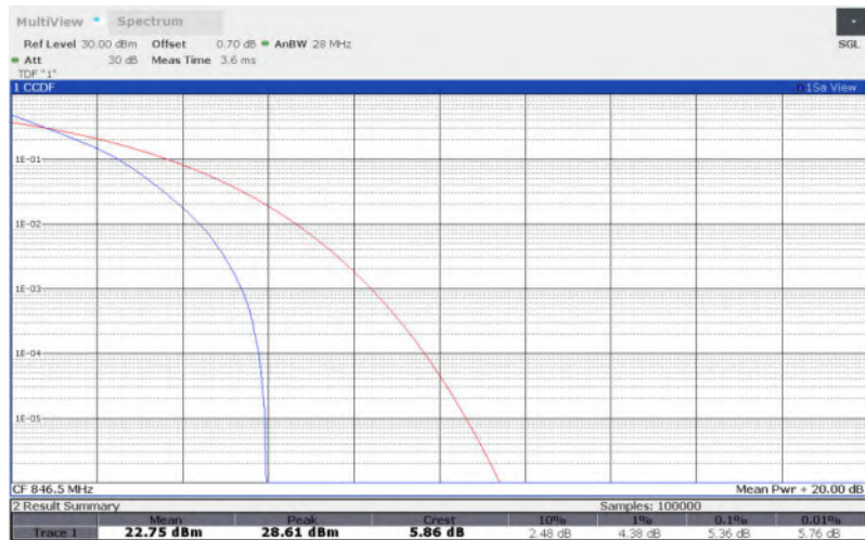
LTE Band 26 , 5MHz Bandwidth,16QAM
