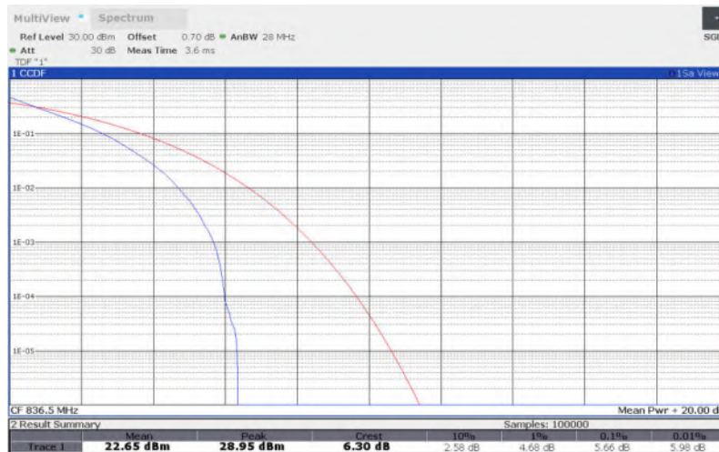
LTE Band 26 , 15MHz Bandwidth,16QAM
