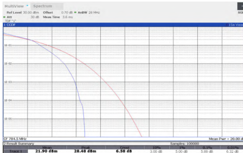
LTE Band 13 , 5MHz Bandwidth,64QAM
