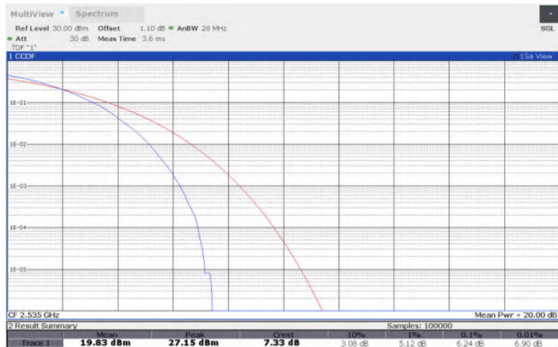
LTE Band 7 , 20MHz Bandwidth,QPSK
