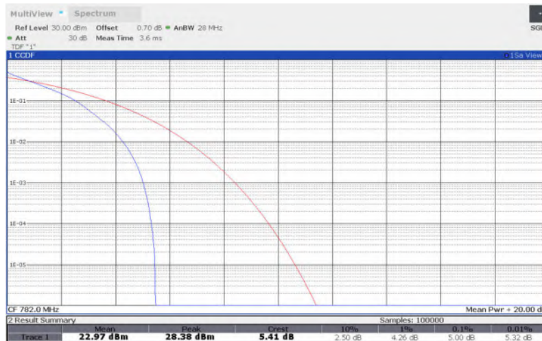
LTE Band 13 , 5MHz Bandwidth,16QAM
