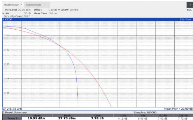
LTE Band 38 , 5MHz Bandwidth,16QAM
