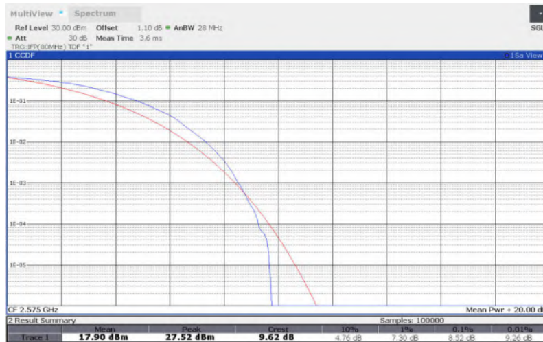
LTE Band 38 , 10MHz Bandwidth,QPSK
