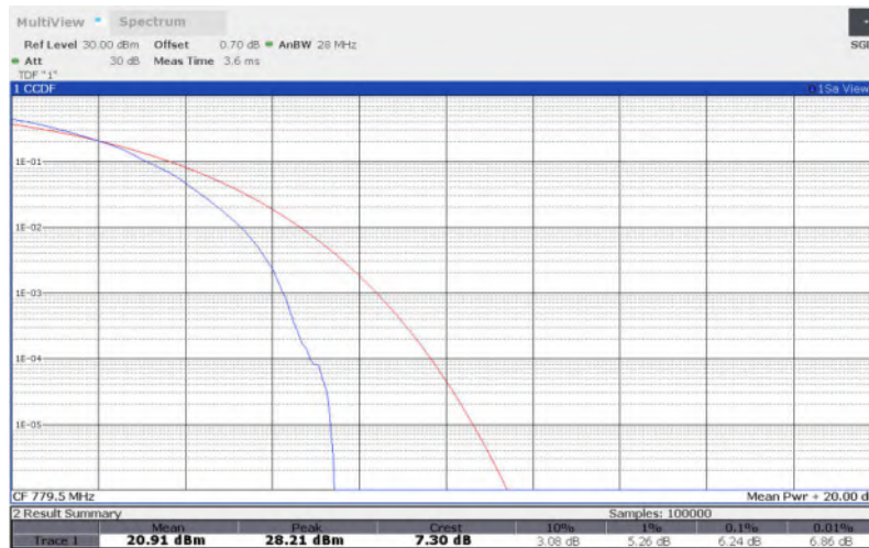
LTE Band 13 , 5MHz Bandwidth,QPSK
