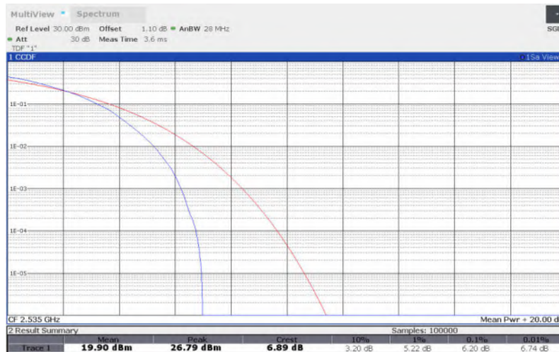
LTE Band 7 , 15MHz Bandwidth,QPSK
