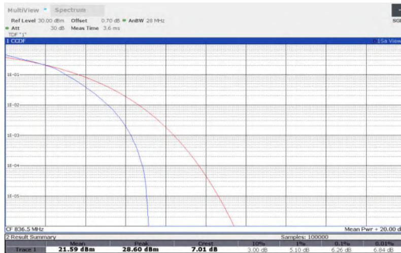
LTE Band 26 , 10MHz Bandwidth,64QAM
