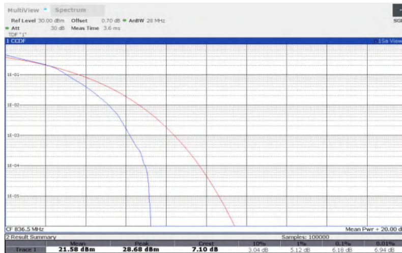
LTE Band 26 , 3MHz Bandwidth,64QAM
