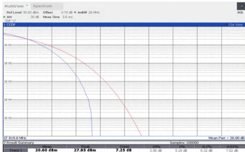
LTE Band 26 , 5MHz Bandwidth,QPSK
