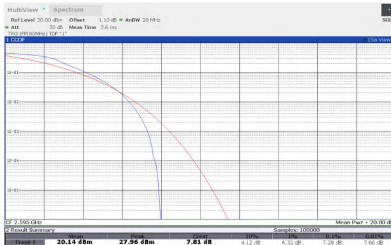
LTE Band 38 , 10MHz Bandwidth,16QAM
