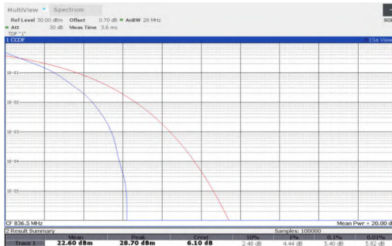
LTE Band 26 , 5MHz Bandwidth,16QAM
