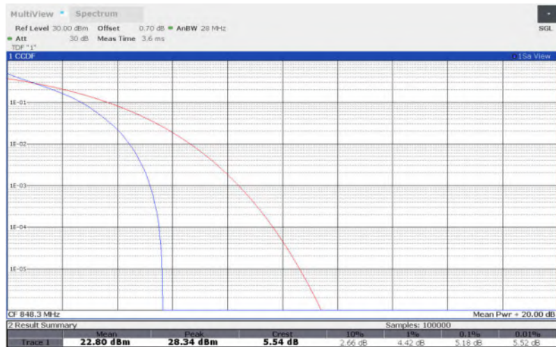
LTE Band 26 , 1.4MHz Bandwidth,16QAM
