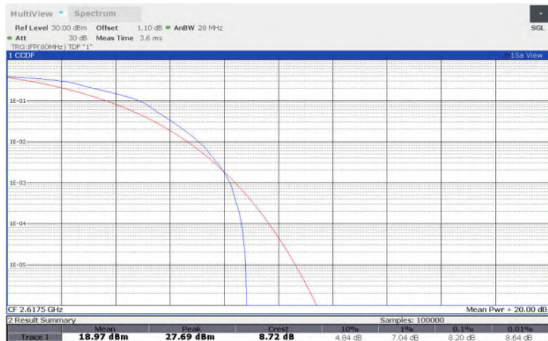
LTE Band 38 , 5MHz Bandwidth,64QAM
