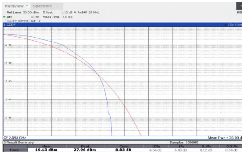
LTE Band 38 , 5MHz Bandwidth,64QAM
