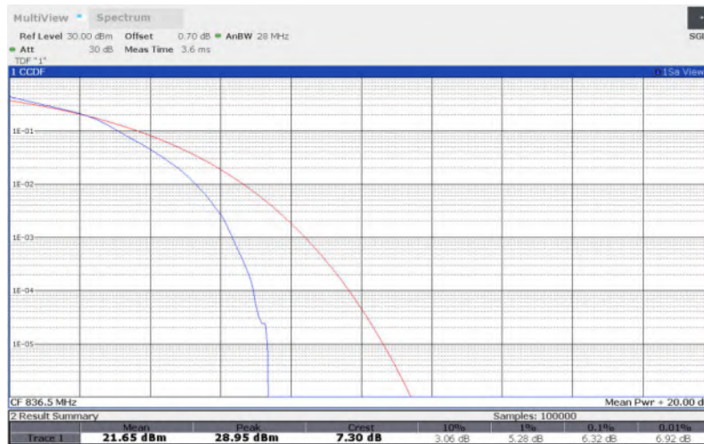
LTE Band 26 , 15MHz Bandwidth,64QAM
