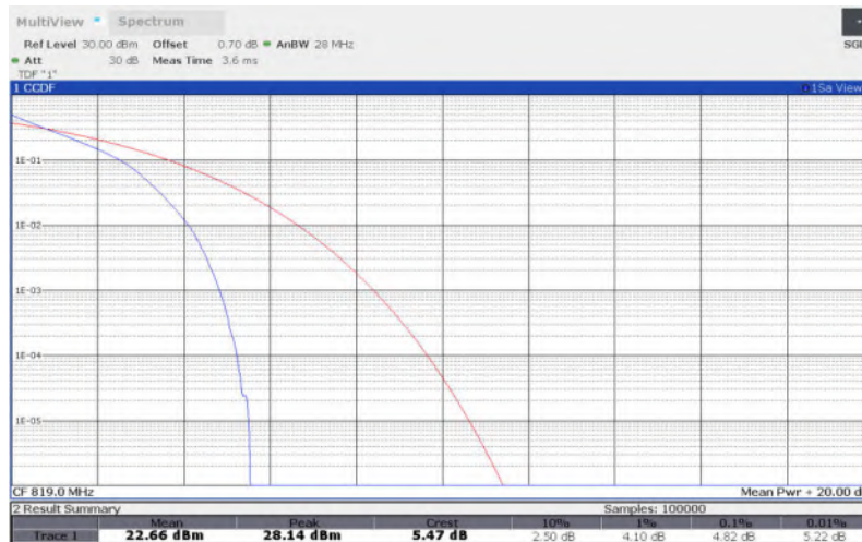
LTE Band 26 , 3MHz Bandwidth,16QAM
