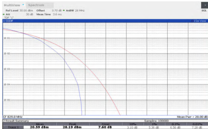
LTE Band 26 , 10MHz Bandwidth,QPSK
