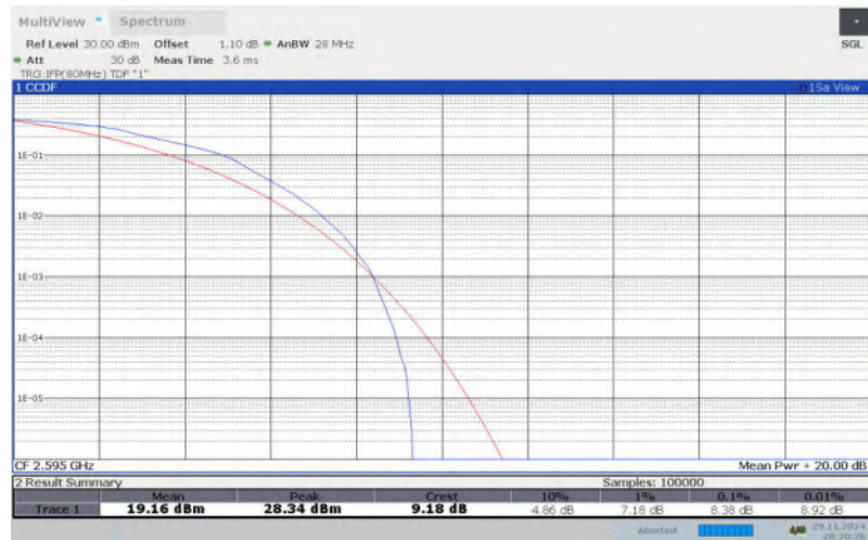
LTE Band 38 , 15MHz Bandwidth,64QAM
