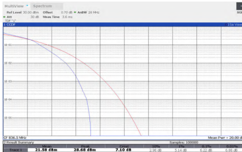
LTE Band 26 , 5MHz Bandwidth,64QAM
