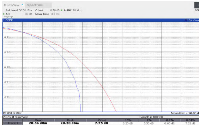
LTE Band 26 , 15MHz Bandwidth,QPSK
