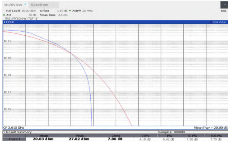
LTE Band 38 , 10MHz Bandwidth,16QAM
