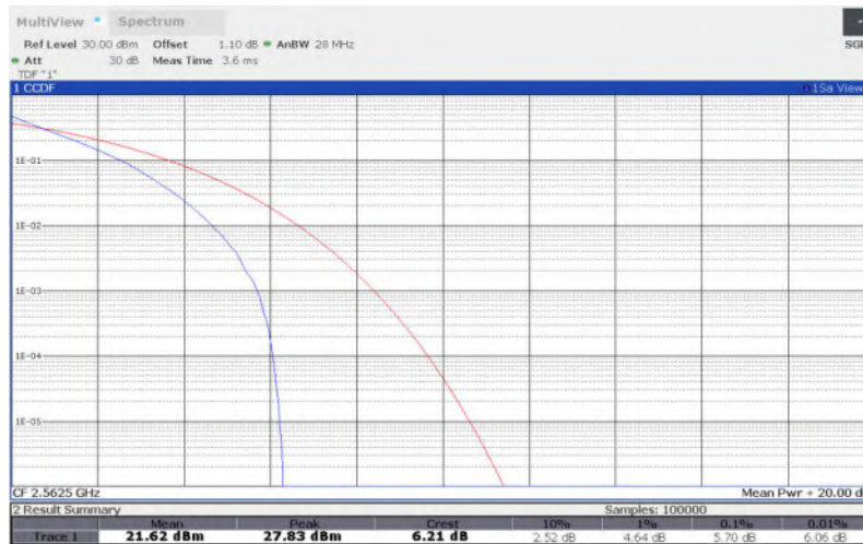
LTE Band 7 , 15MHz Bandwidth,16QAM
