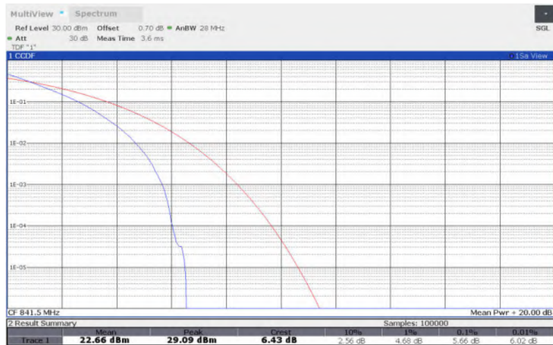
LTE Band 26 , 15MHz Bandwidth,16QAM
