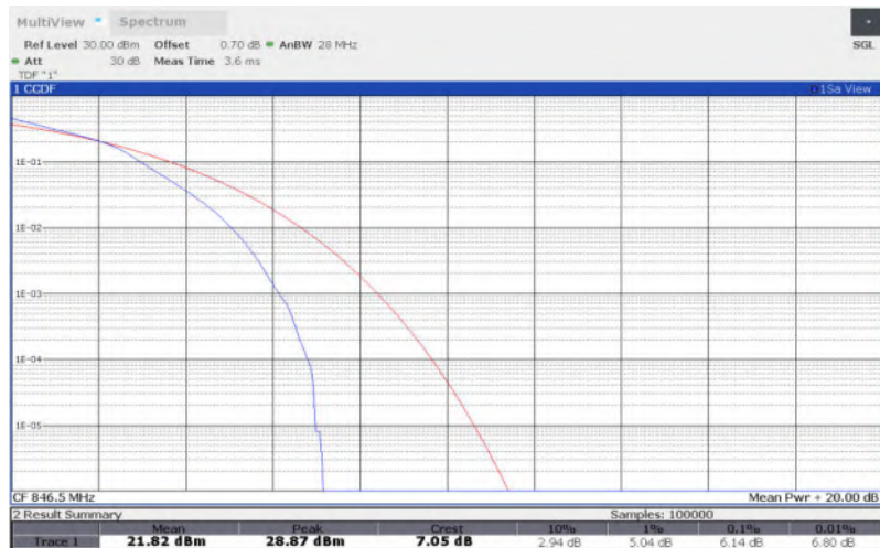
LTE Band 26 , 5MHz Bandwidth,64QAM
