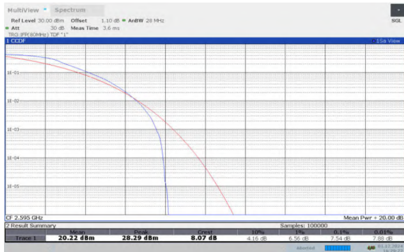
LTE Band 38 , 15MHz Bandwidth,16QAM
