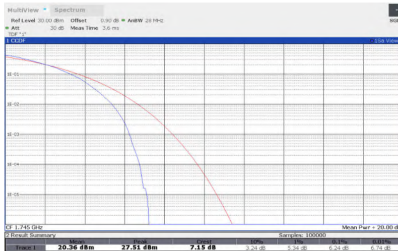
LTE Band 66 , 15MHz Bandwidth,256QAM
