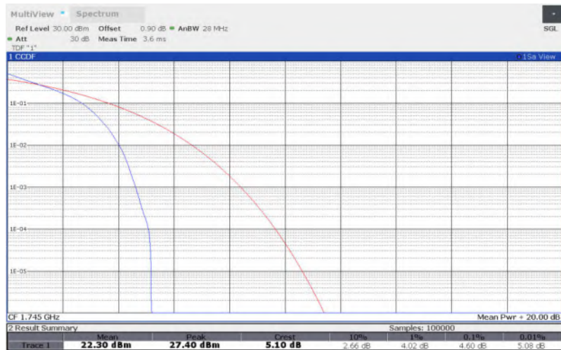
LTE Band 66 , 1.4MHz Bandwidth,16QAM
