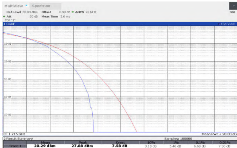
LTE Band 66 , 10MHz Bandwidth,256QAM
