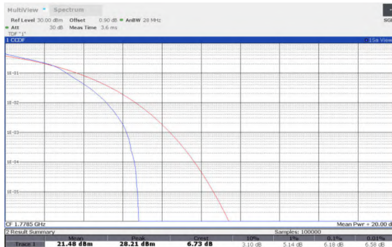
LTE Band 66 , 3MHz Bandwidth,64QAM
