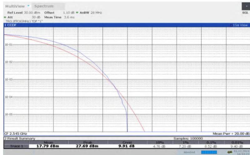
LTE Band 41 , 20MHz Bandwidth,QPSK
