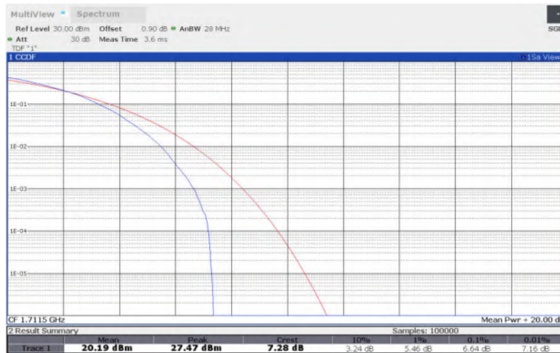
LTE Band 66 , 3MHz Bandwidth,256QAM
