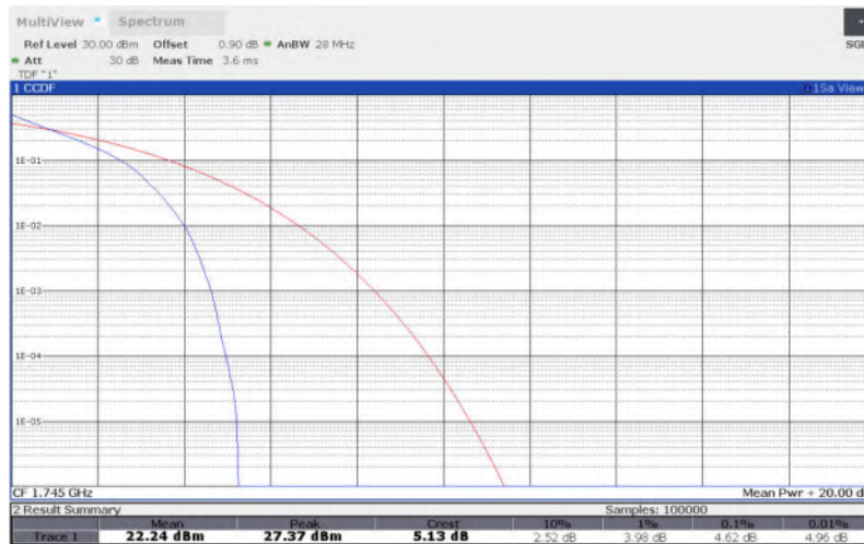
LTE Band 66 , 3MHz Bandwidth,16QAM
