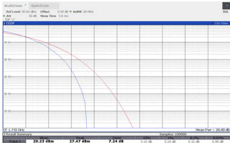
LTE Band 66 , 20MHz Bandwidth,QPSK
