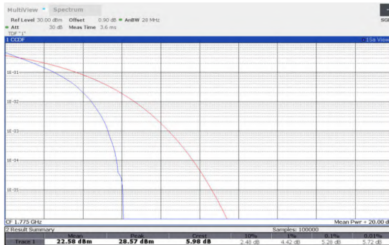
LTE Band 66 , 10MHz Bandwidth,16QAM
