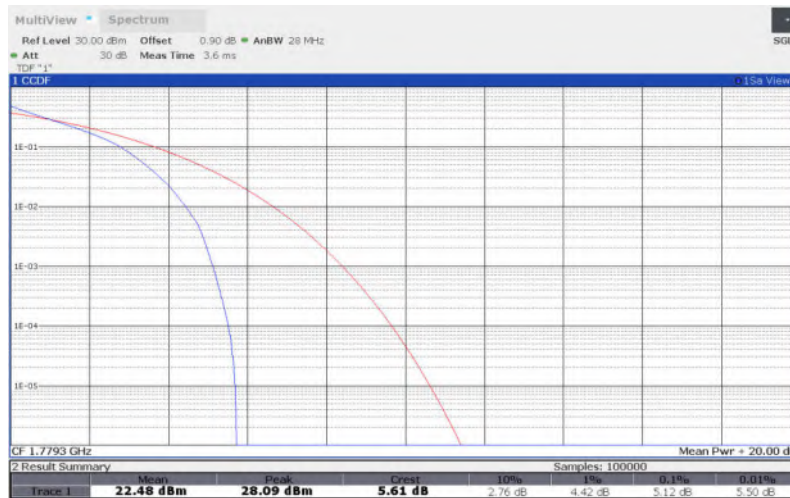
LTE Band 66 , 1.4MHz Bandwidth,16QAM
