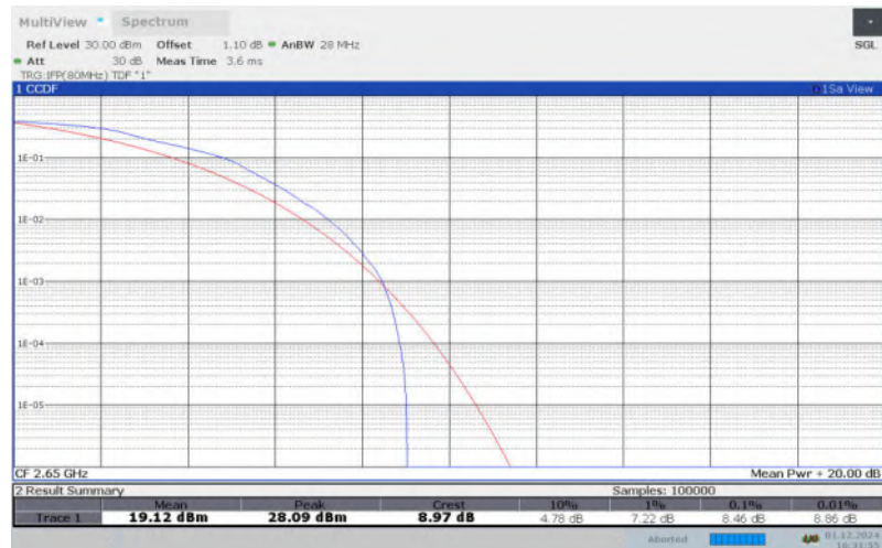
LTE Band 41 , 10MHz Bandwidth,64QAM
