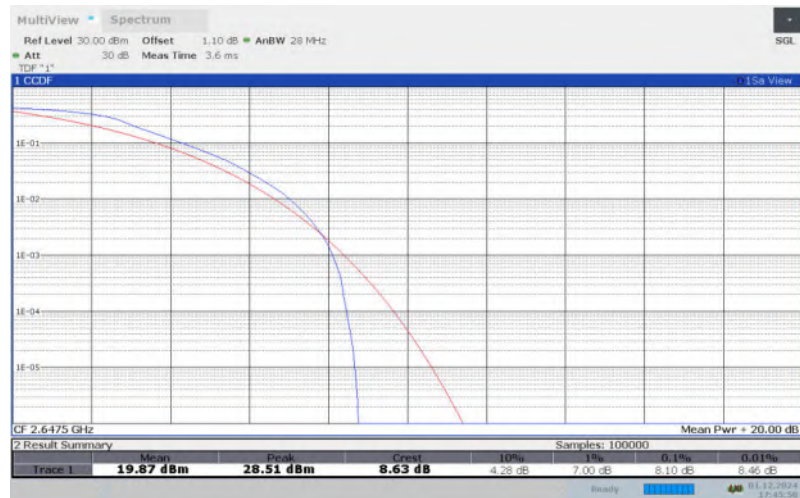
LTE Band 41 , 15MHz Bandwidth,16QAM
