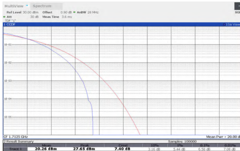
LTE Band 66 , 5MHz Bandwidth,256QAM
