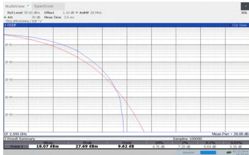
LTE Band 41 , 10MHz Bandwidth,QPSK
