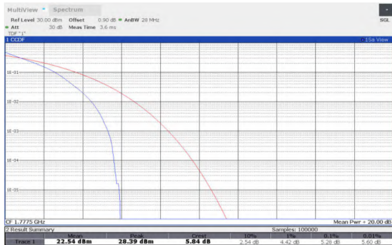
LTE Band 66 , 5MHz Bandwidth,16QAM
