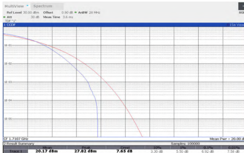
LTE Band 66 , 1.4MHz Bandwidth,QPSK
