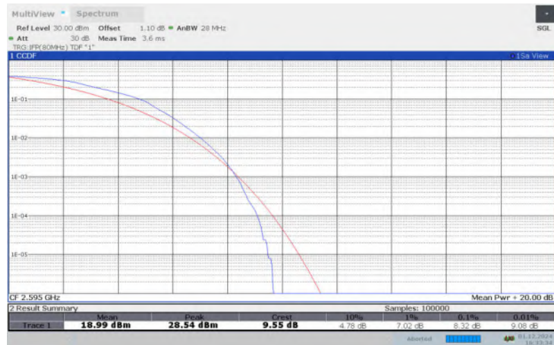
LTE Band 41 , 20MHz Bandwidth,64QAM
