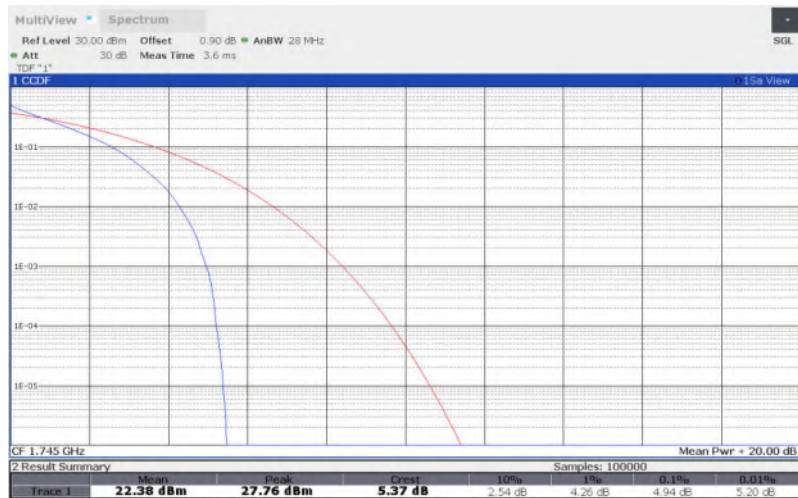
LTE Band 66 , 15MHz Bandwidth,16QAM
