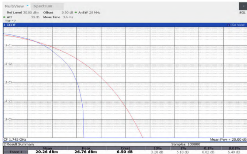
LTE Band 66 , 1.4MHz Bandwidth,256QAM
