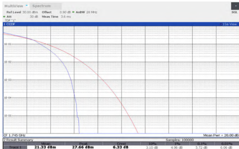
LTE Band 66 , 15MHz Bandwidth,64QAM
