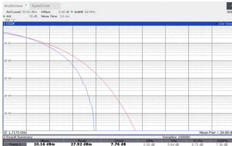
LTE Band 66 , 15MHz Bandwidth,QPSK
