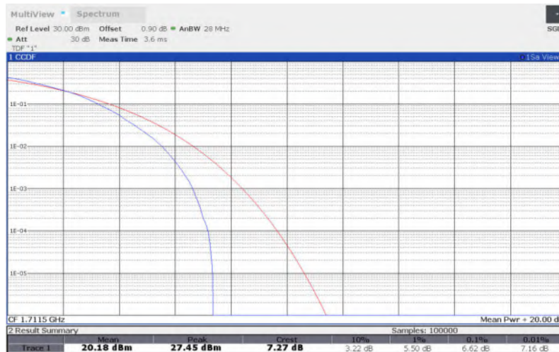
LTE Band 66 , 3MHz Bandwidth,QPSK
