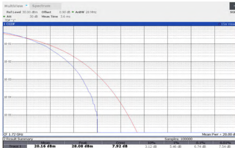
LTE Band 66 , 20MHz Bandwidth,QPSK
