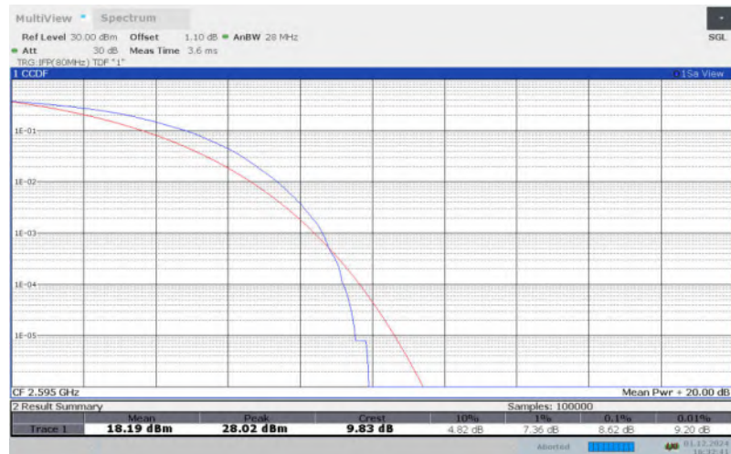
LTE Band 41 , 15MHz Bandwidth,QPSK
