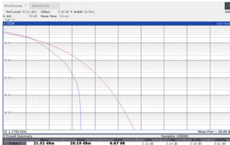
LTE Band 66 , 1.4MHz Bandwidth,64QAM
