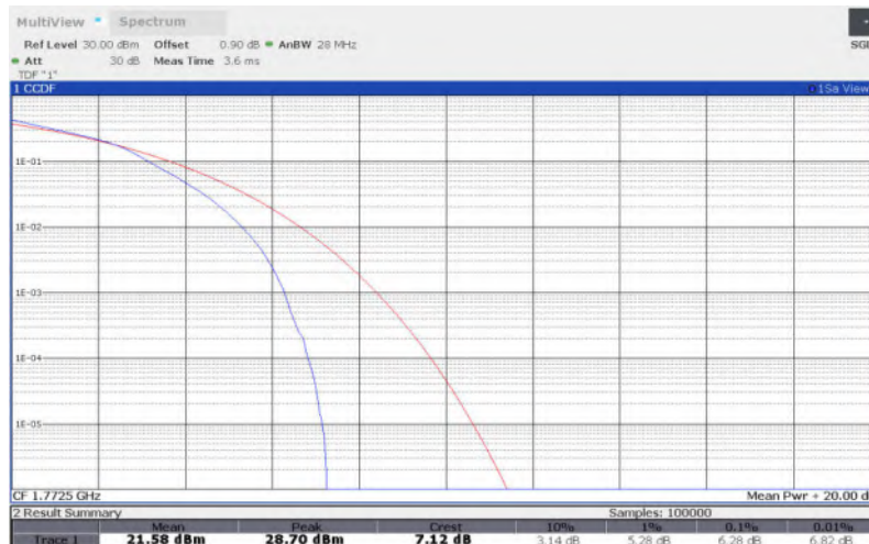
LTE Band 66 , 15MHz Bandwidth,64QAM
