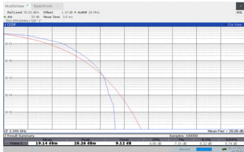
LTE Band 41 , 15MHz Bandwidth,64QAM
