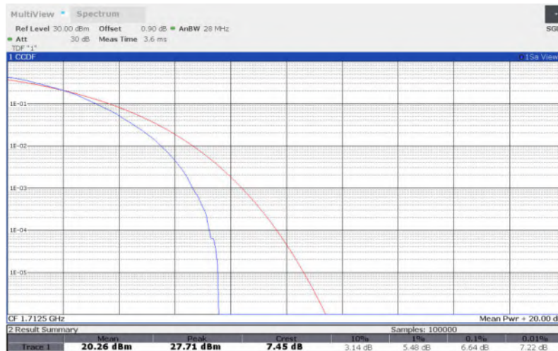
LTE Band 66 , 5MHz Bandwidth,QPSK
