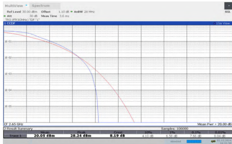
LTE Band 41 , 10MHz Bandwidth,16QAM
