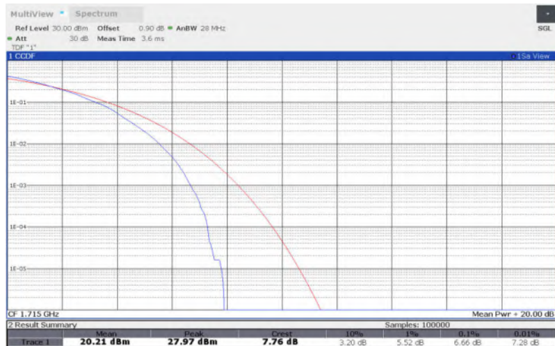
LTE Band 66 , 10MHz Bandwidth,QPSK
