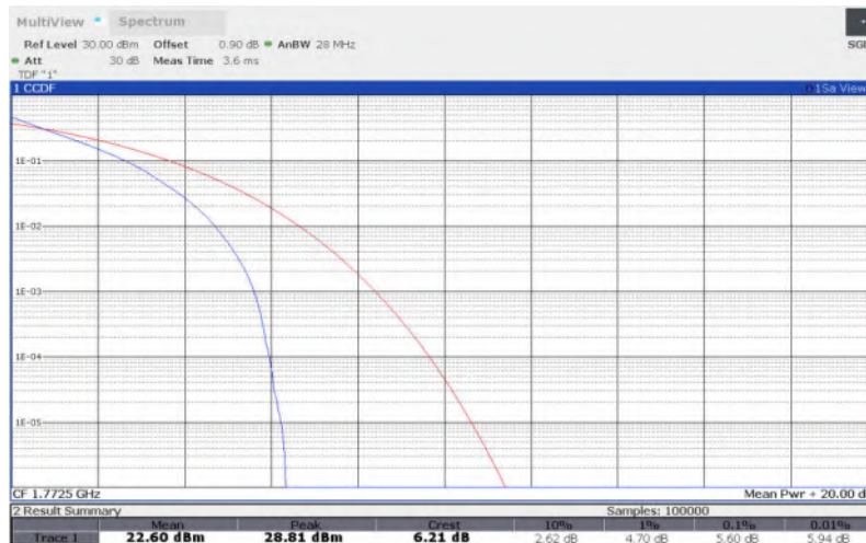
LTE Band 66 , 15MHz Bandwidth,16QAM
