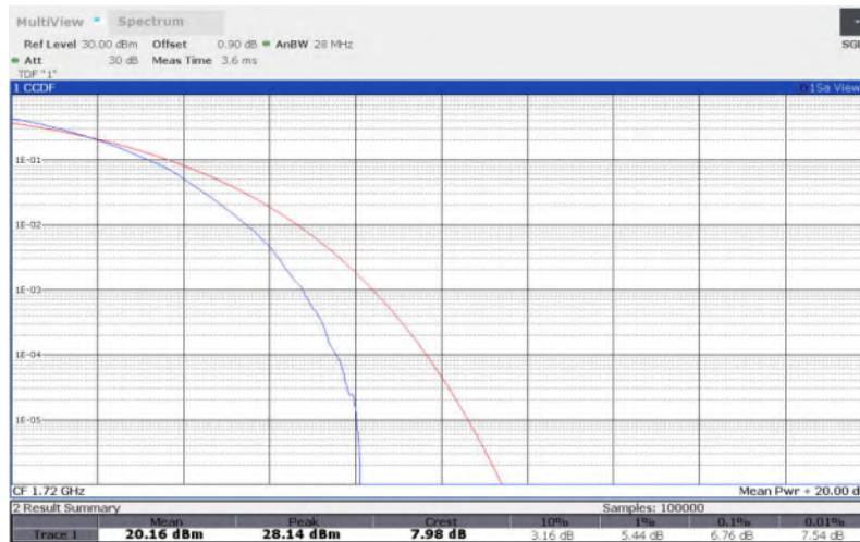
LTE Band 66 , 20MHz Bandwidth,256QAM
