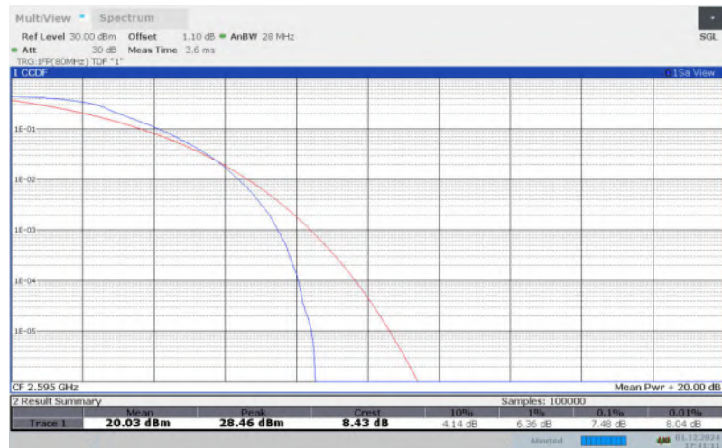
LTE Band 41 , 20MHz Bandwidth,16QAM
