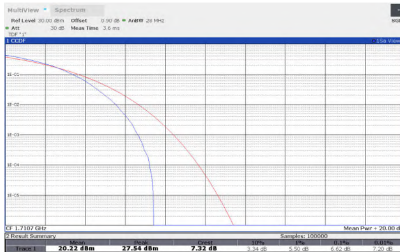
LTE Band 66 , 1.4MHz Bandwidth,256QAM
