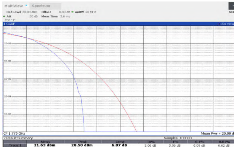
LTE Band 66 , 10MHz Bandwidth,64QAM
