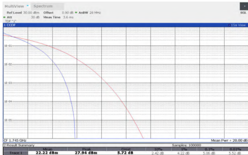
LTE Band 66 , 20MHz Bandwidth,16QAM
