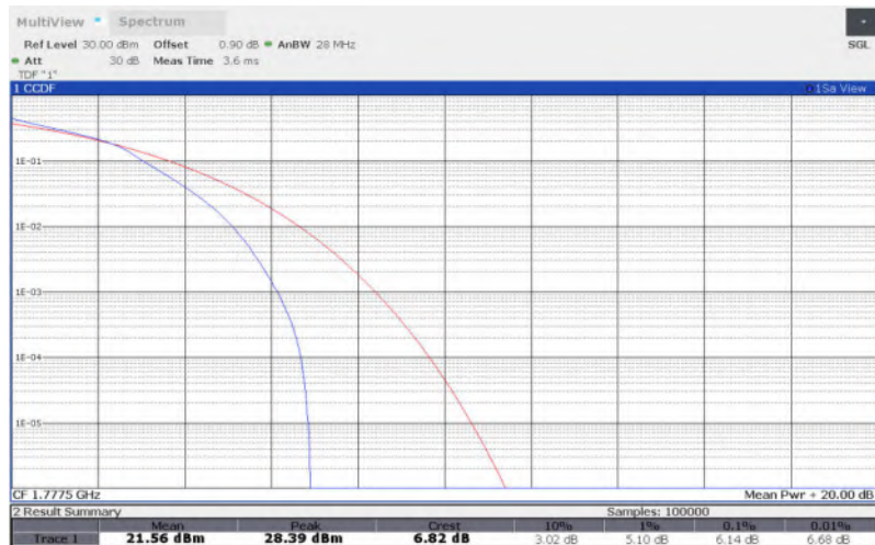
LTE Band 66 , 5MHz Bandwidth,64QAM
