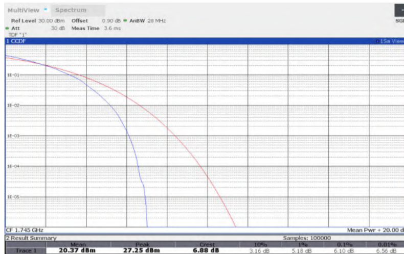
LTE Band 66 , 10MHz Bandwidth,256QAM
