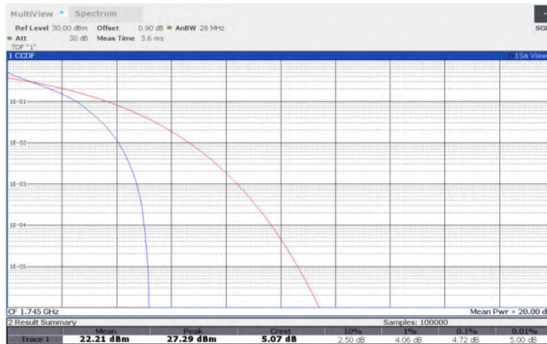
LTE Band 66 , 5MHz Bandwidth,16QAM
