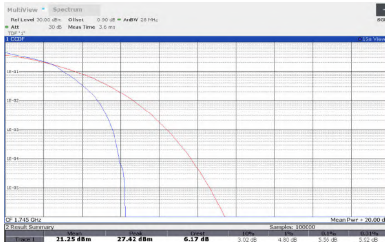
LTE Band 66 , 5MHz Bandwidth,64QAM
