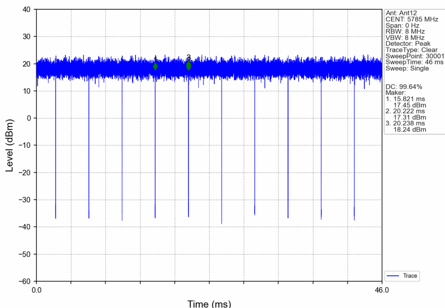
802.11ax(HEW20)_MCH_5785MHz_RU242_Left_Ant12_NTNV
