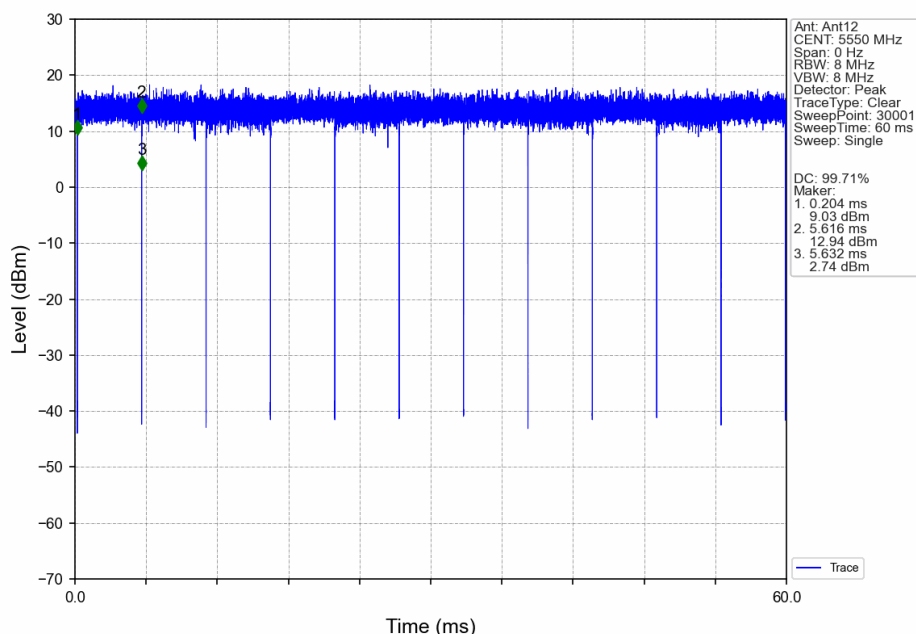
802.11n(HT40)_MCH_5550MHz_Ant12_NTNV
