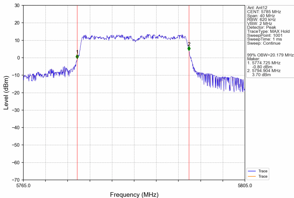
802.11ax(HEW20)_MCH_5785MHz_RU242_Left_Ant12_NTNV
