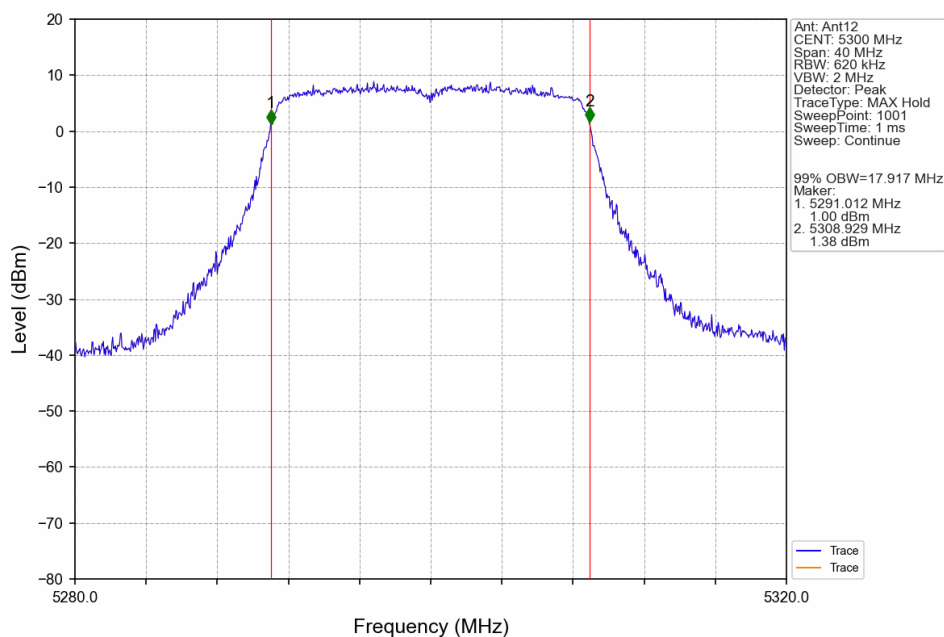
802.11ac(VHT20)_MCH_5300MHz_Ant12_NTNV
