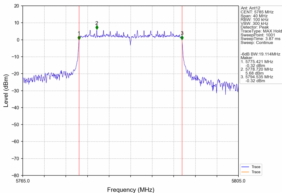
802.11ax(HEW20)_MCH_5785MHz_RU242_Left_Ant12_NTNV
