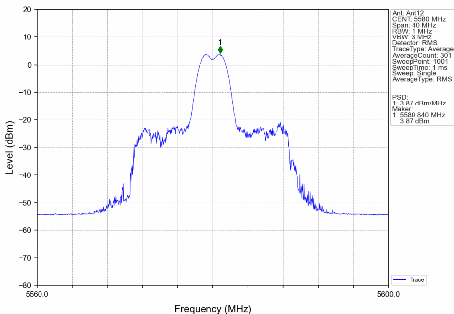
802.11ax(HEW20)_MCH_5580MHz_RU26_Mid_Ant12_NTNV
