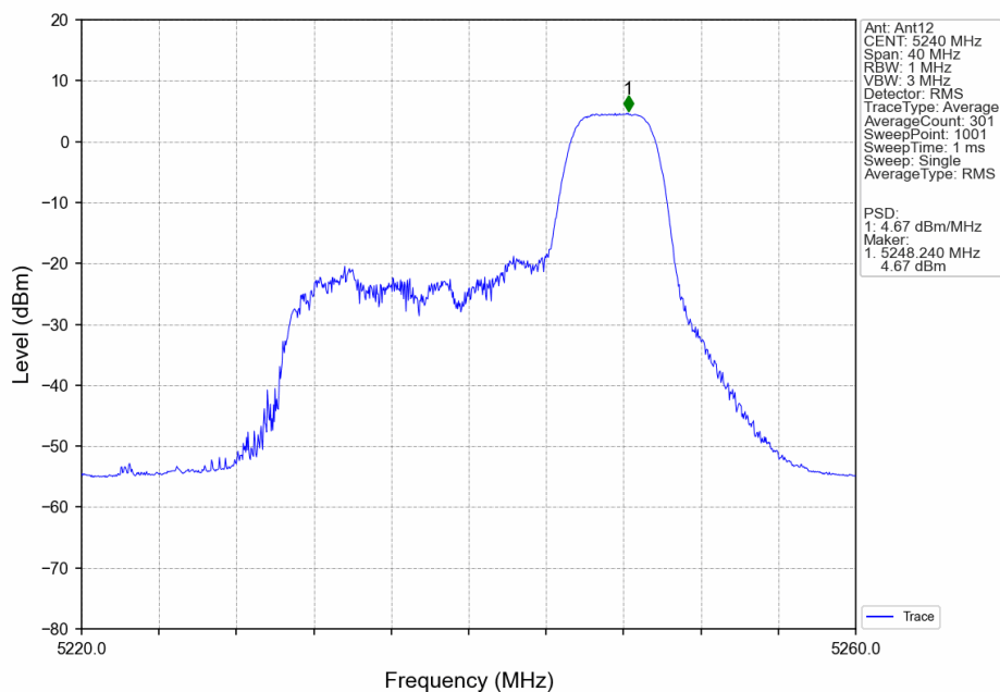
802.11ax(HEW20)_HCH_5240MHz_RU106_Right_Ant12_NTNV
