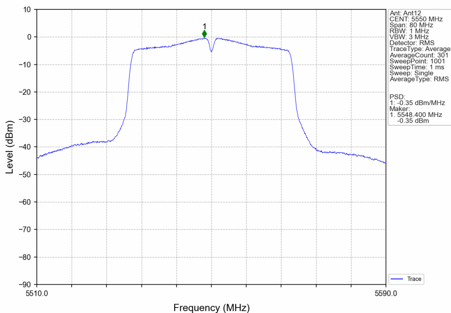
802.11ac(VHT40)_MCH_5550MHz_Ant12_NTNV
