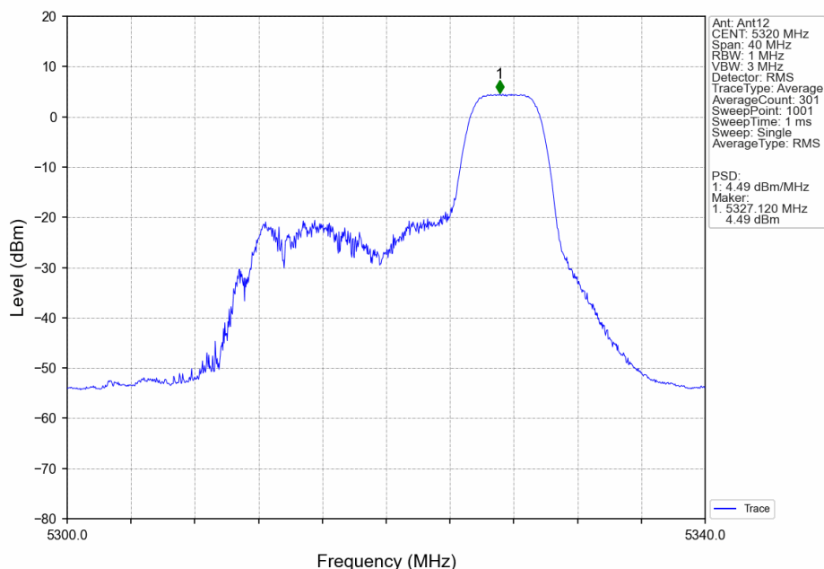
802.11ax(HEW20)_HCH_5320MHz_RU106_Right_Ant12_NTNV
