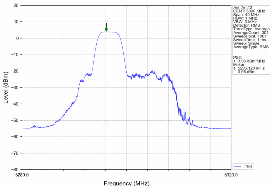
802.11ax(HEW20)_MCH_5300MHz_RU106_Left_Ant12_NTNV
