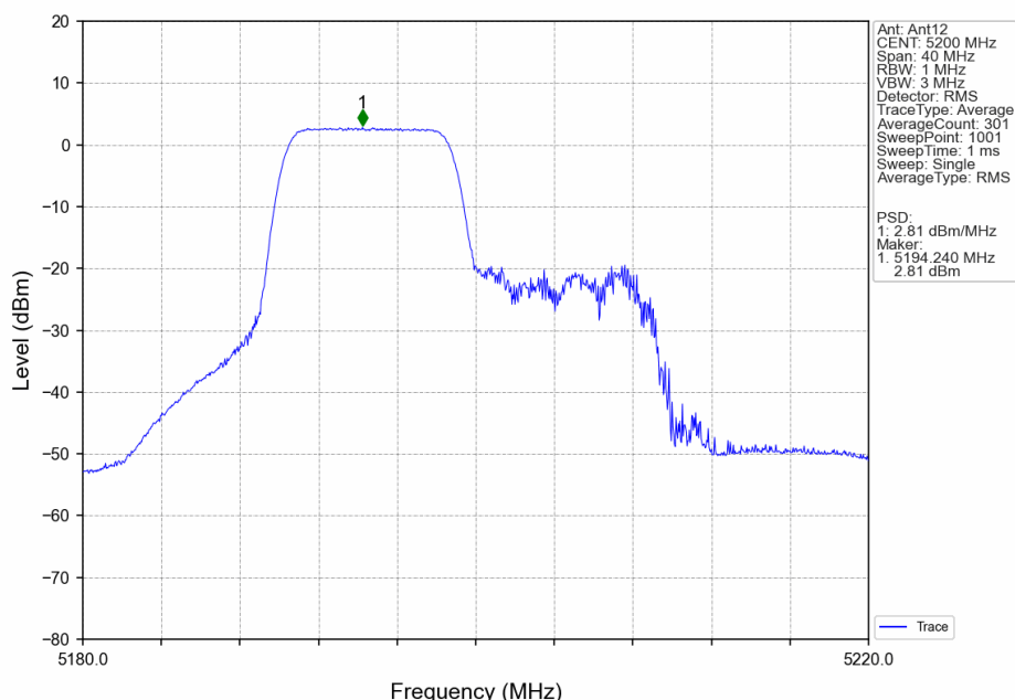
802.11ax(HEW20)_MCH_5200MHz_RU106_Left_Ant12_NTNV
