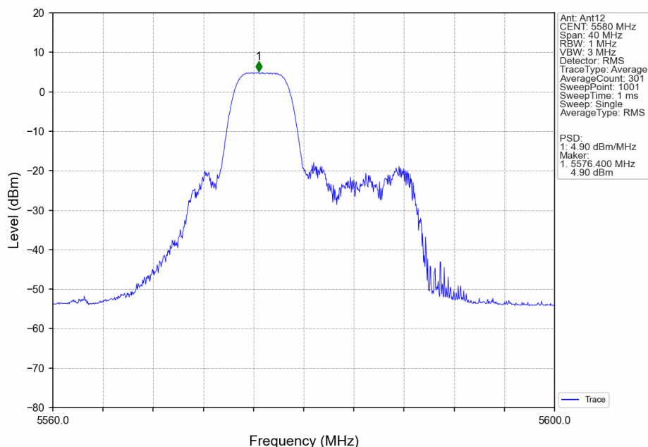
802.11ax(HEW20)_MCH_5580MHz_RU106_Left_Ant12_NTNV
