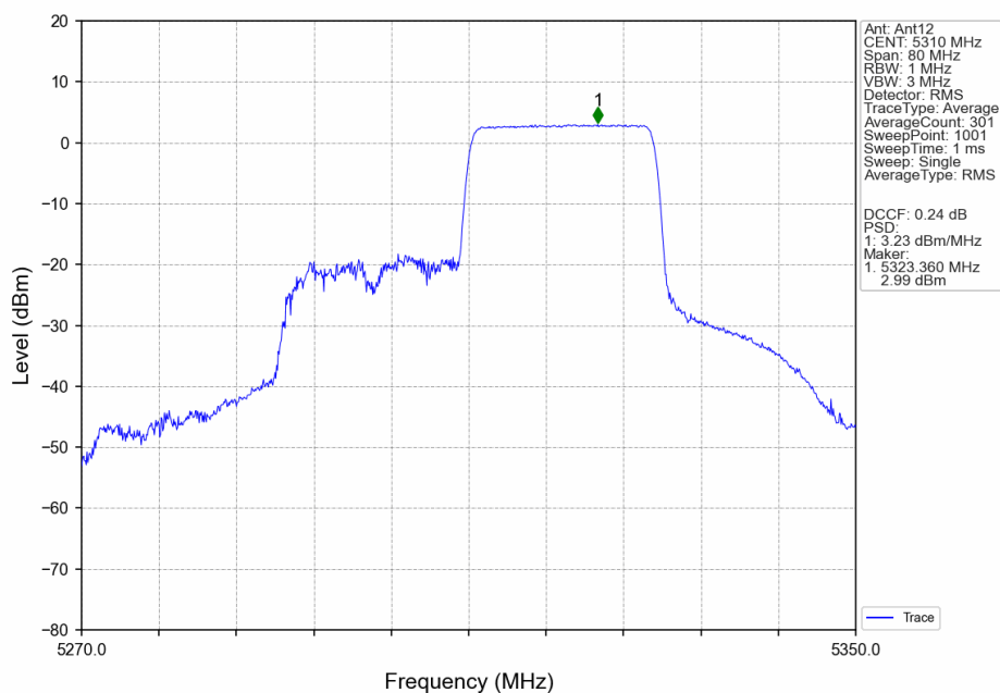
802.11ax(HEW40)_HCH_5310MHz_RU242_Right_Ant12_NTNV
