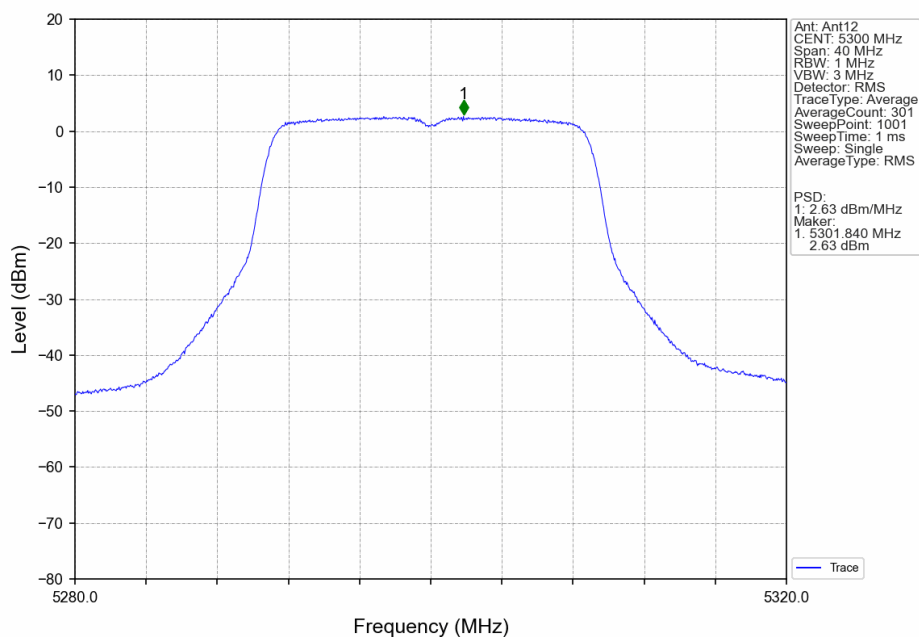
802.11ac(VHT20)_MCH_5300MHz_Ant12_NTNV
