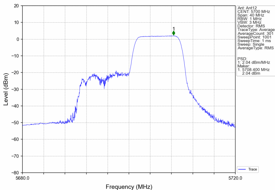
802.11ax(HEW20)_HCH_5700MHz_RU106_Right_Ant12_NTNV
