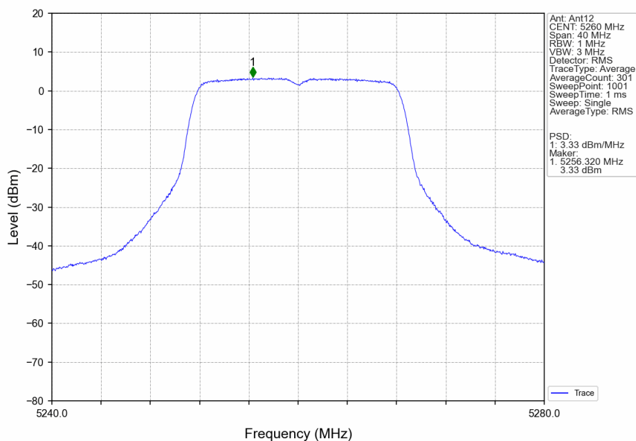
802.11a_LCH_5260MHz_Ant12_NTNV
