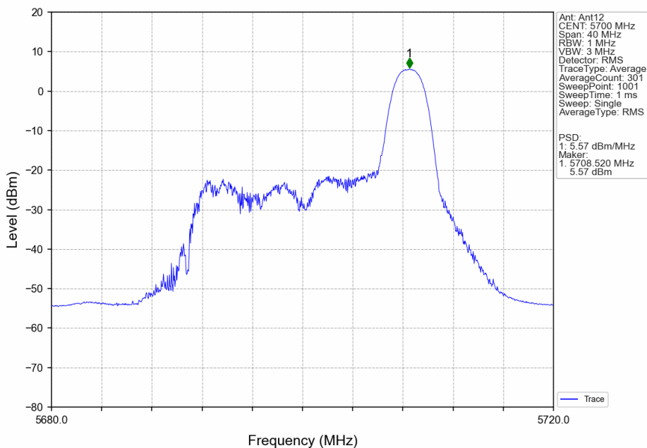
802.11ax(HEW20)_HCH_5700MHz_RU26_Right_Ant12_NTNV
