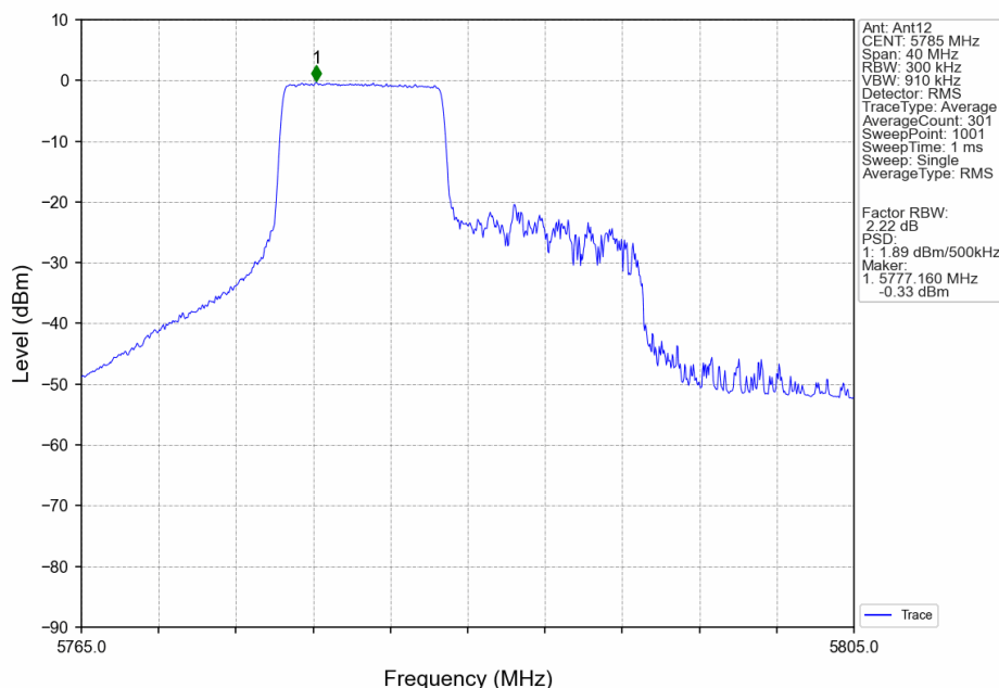
802.11ax(HEW20)_MCH_5785MHz_RU242_Left_Ant12_NTNV
