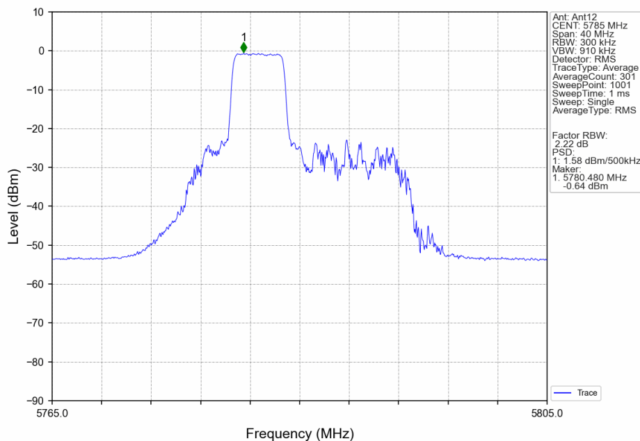
802.11ax(HEW20)_MCH_5785MHz_RU52_Mid_Ant12_NTNV
