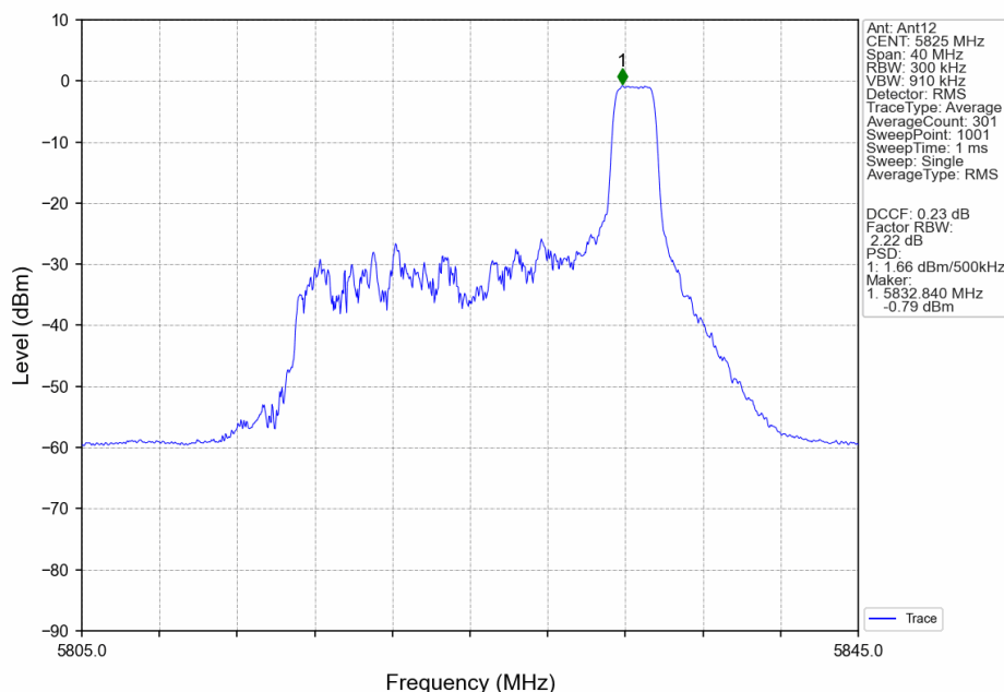
802.11ax(HEW20)_HCH_5825MHz_RU52_Right_Ant12_NTNV
