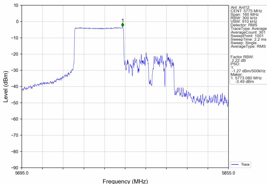
802.11ax(HEW80)_MCH_5775MHz_RU484_Right_Ant12_NTNV
